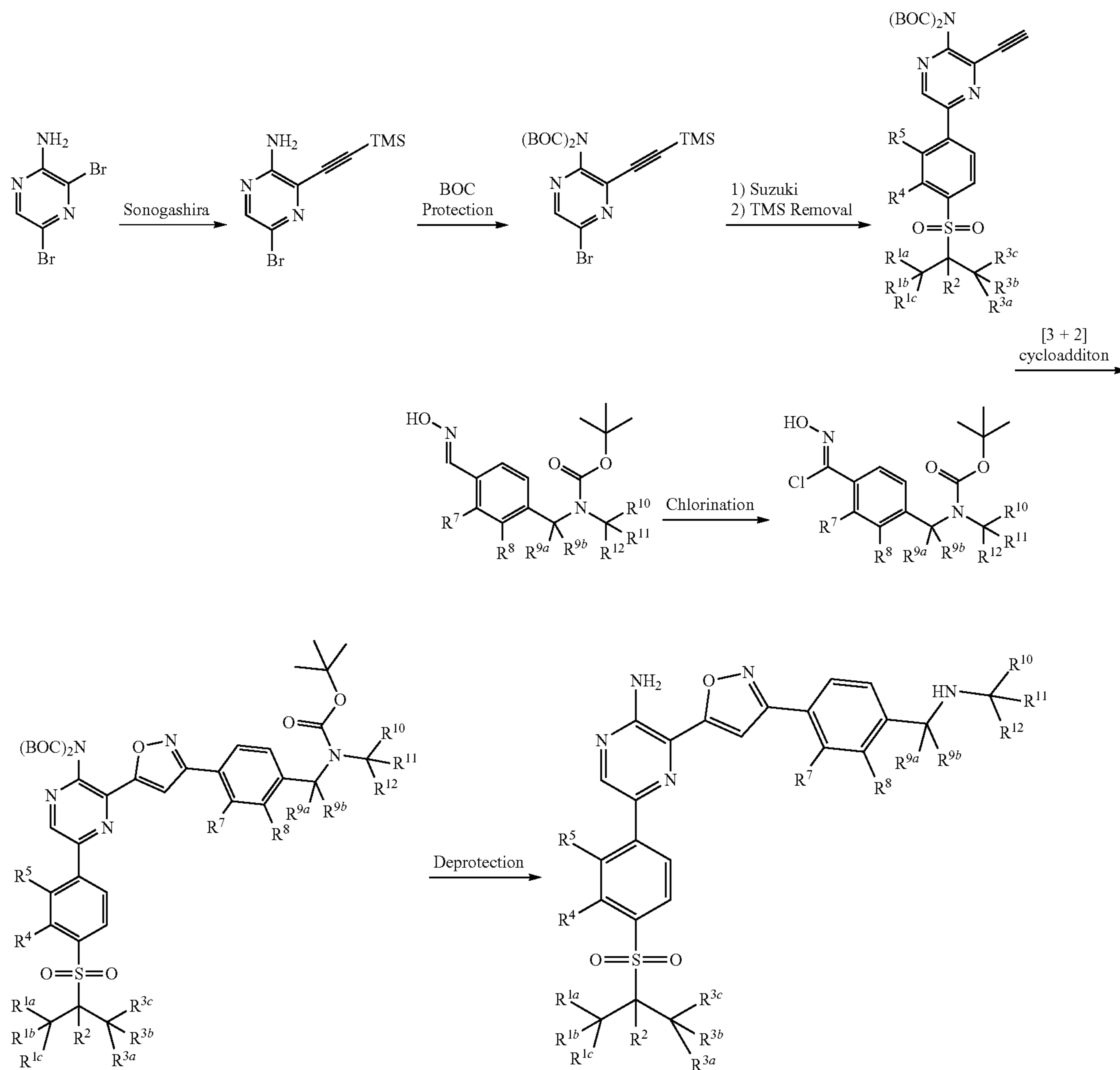
SCHEME P: Formation of isoxazole derivatives
