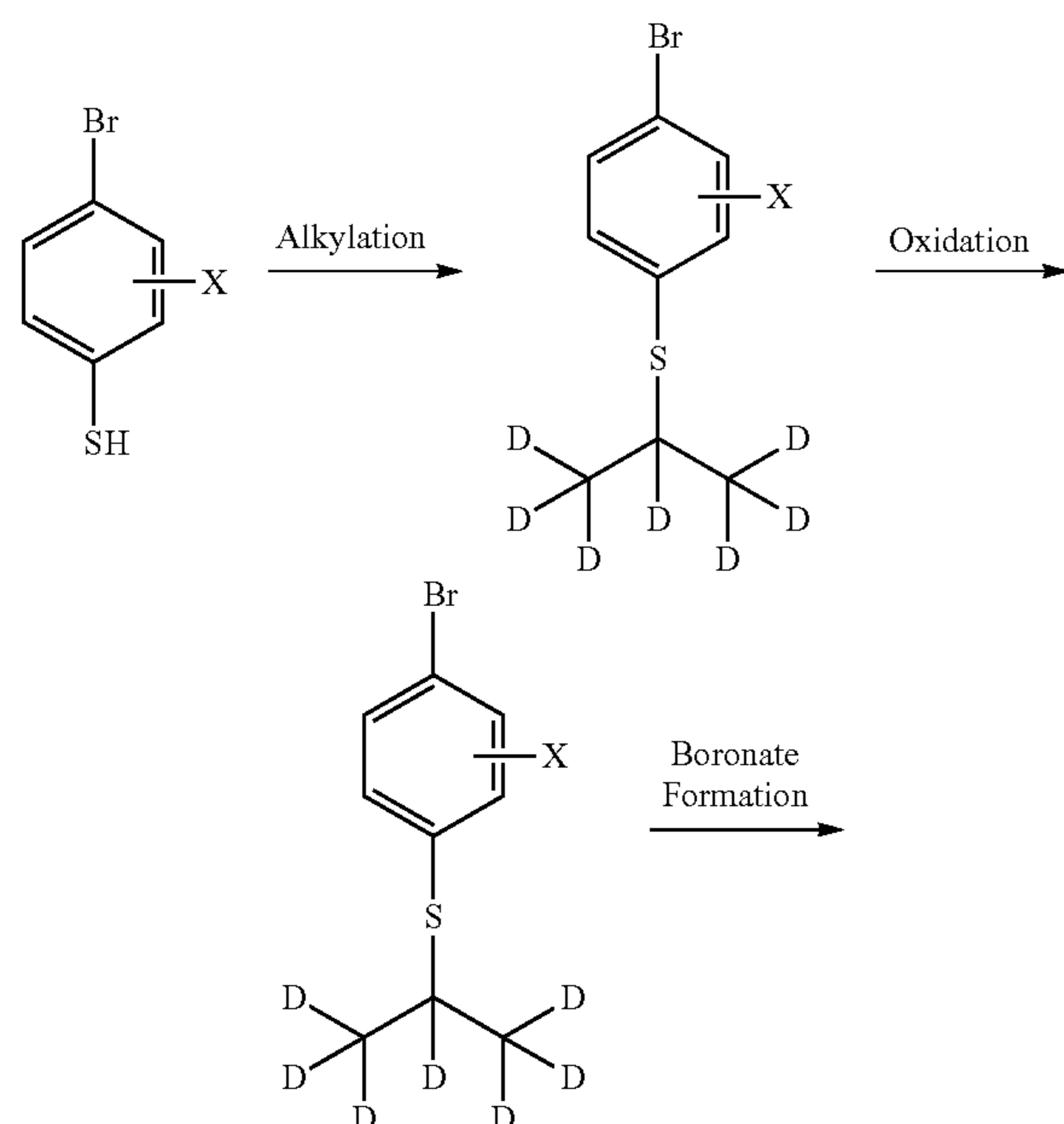
SCHEME F: Formation of aryl ring deuterated boronate
