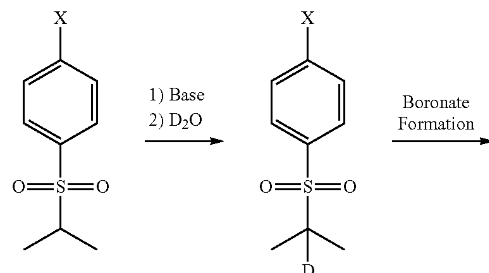
SCHEME B: Formation of d1-boronate
