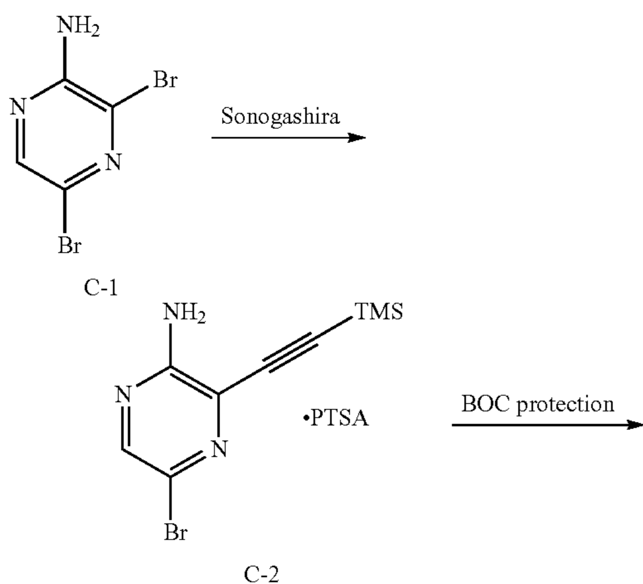
Scheme CC: Synthesis of Intermediate A-4-ii
