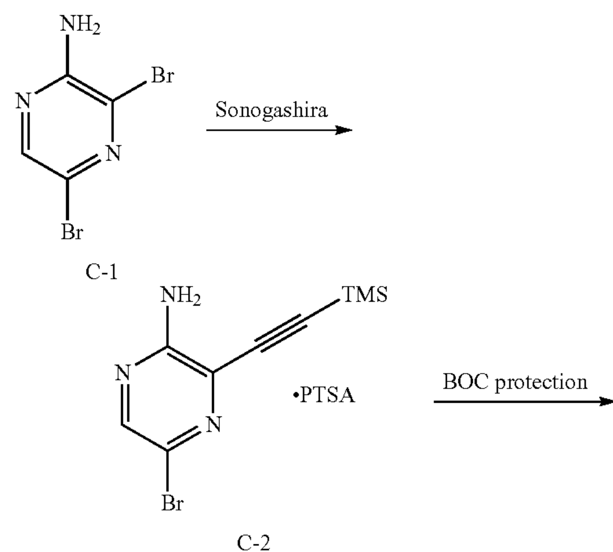
Scheme CC: Synthesis of Intermediate A-4-ii
