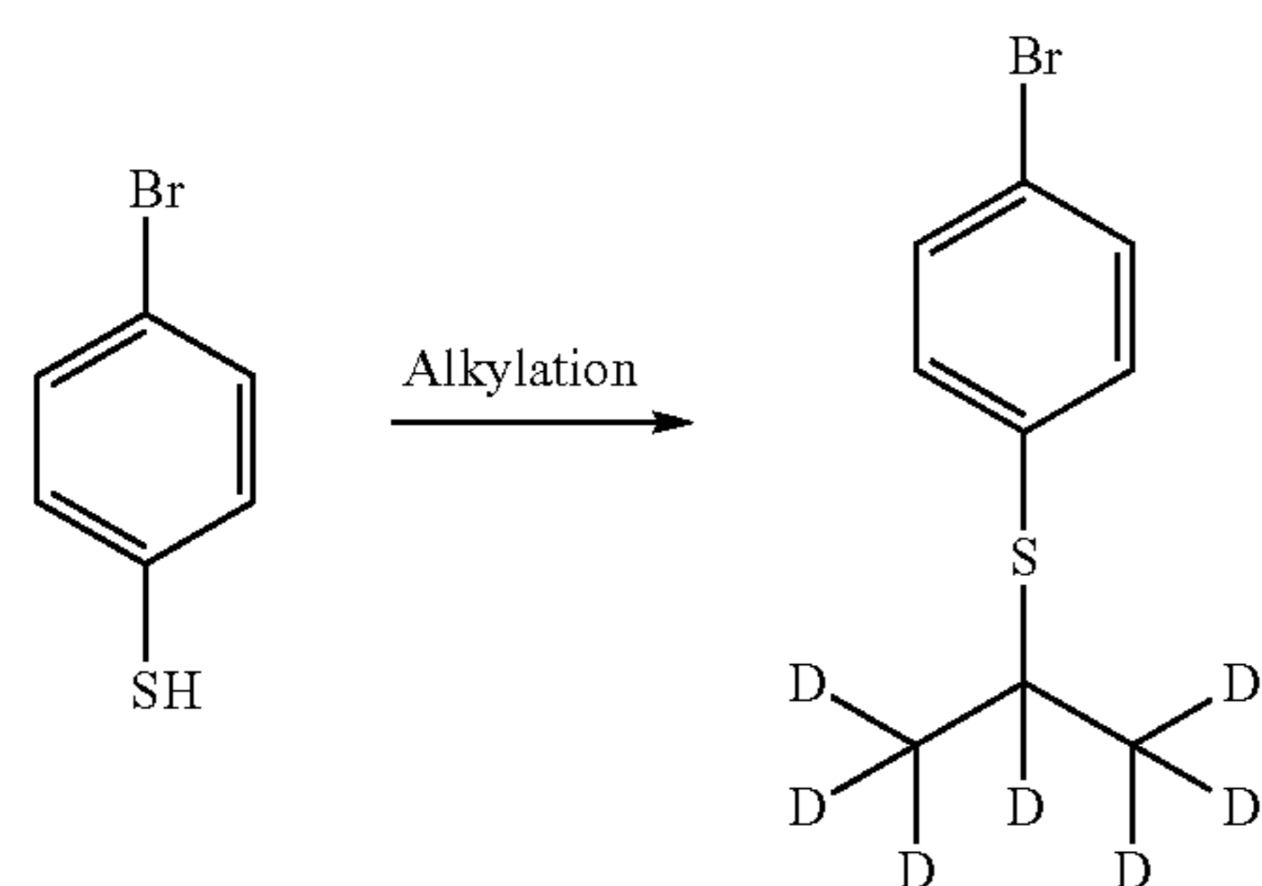
SCHEME D: Formation of d7-boronate
