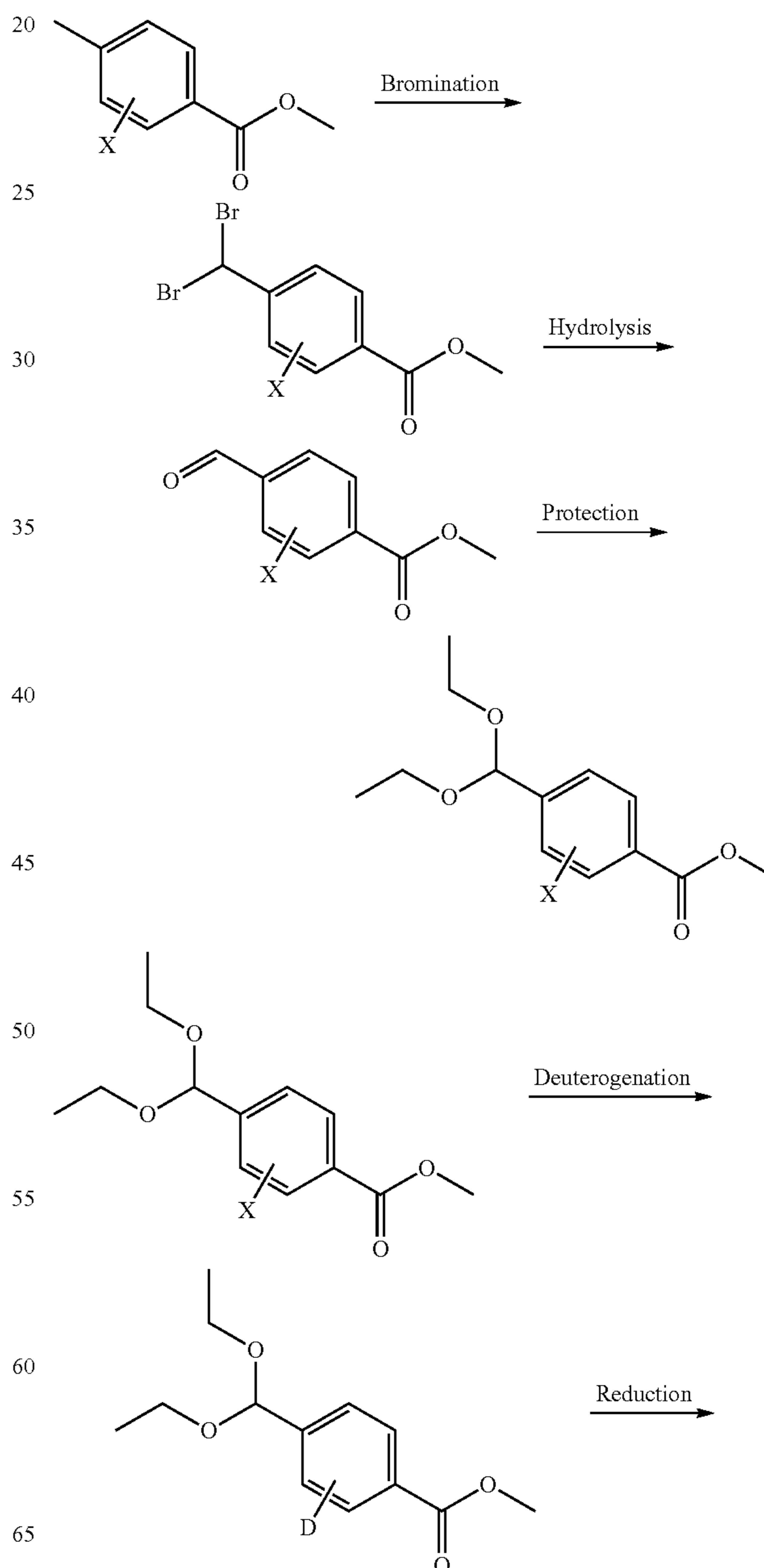
SCHEME H: Formation of aryl ring deuterated oxime intermediates
