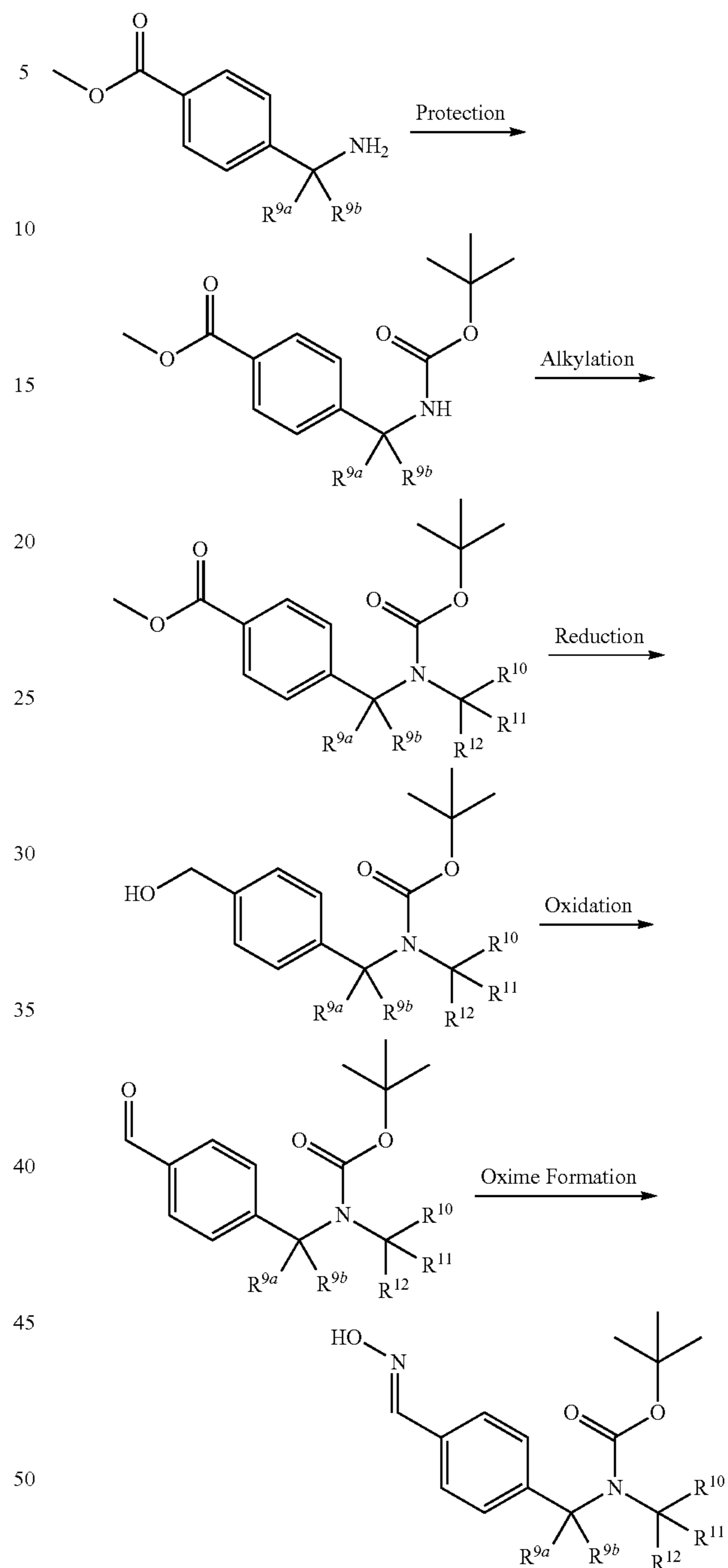
SCHEME O: Formation of deuterated oxime intermediates
