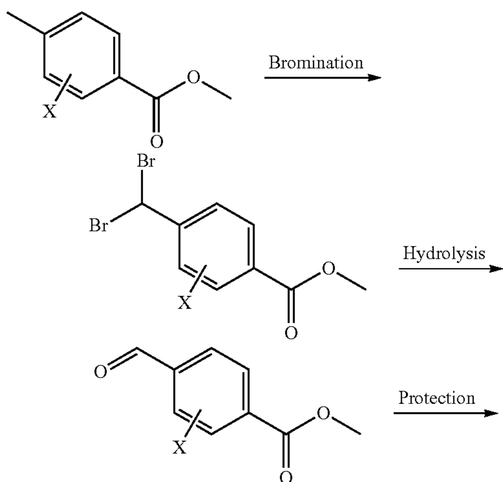
SCHEME J: Formation of aryl ring deuterated oxime intermediates
