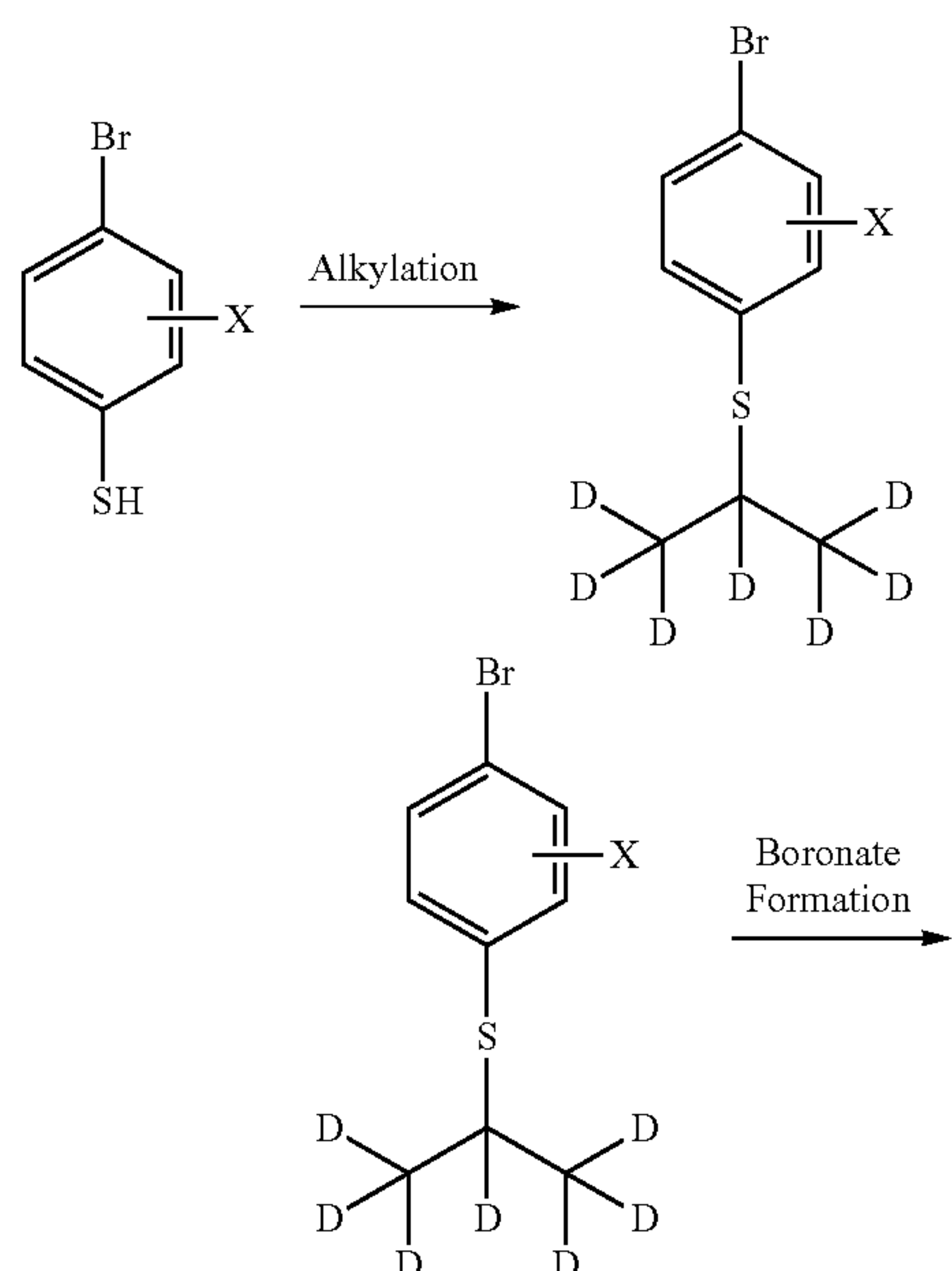
SCHEME F: Formation of aryl ring deuterated boronate
