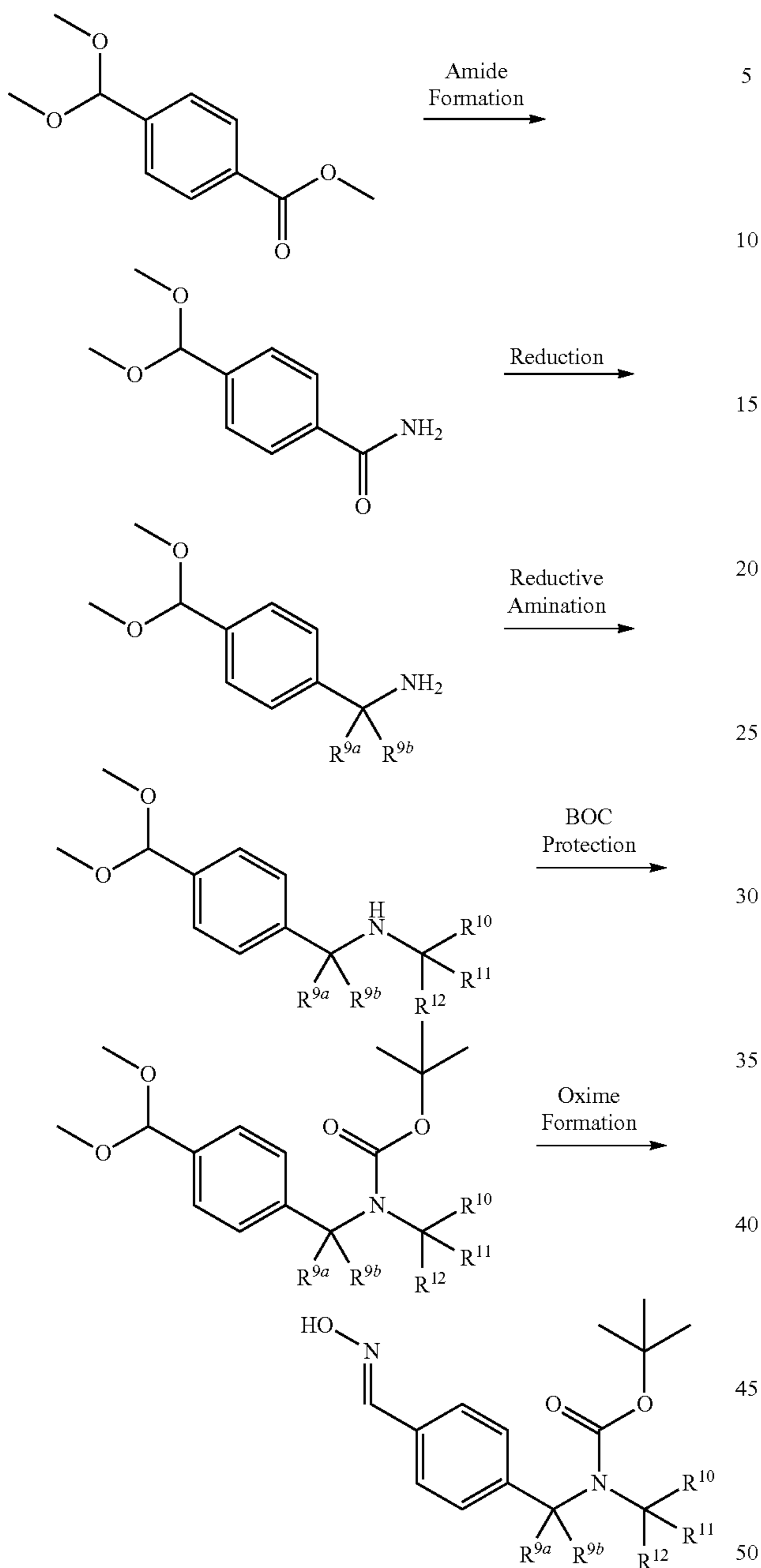
SCHEME N: Formation of deuterated oxime intermediates
