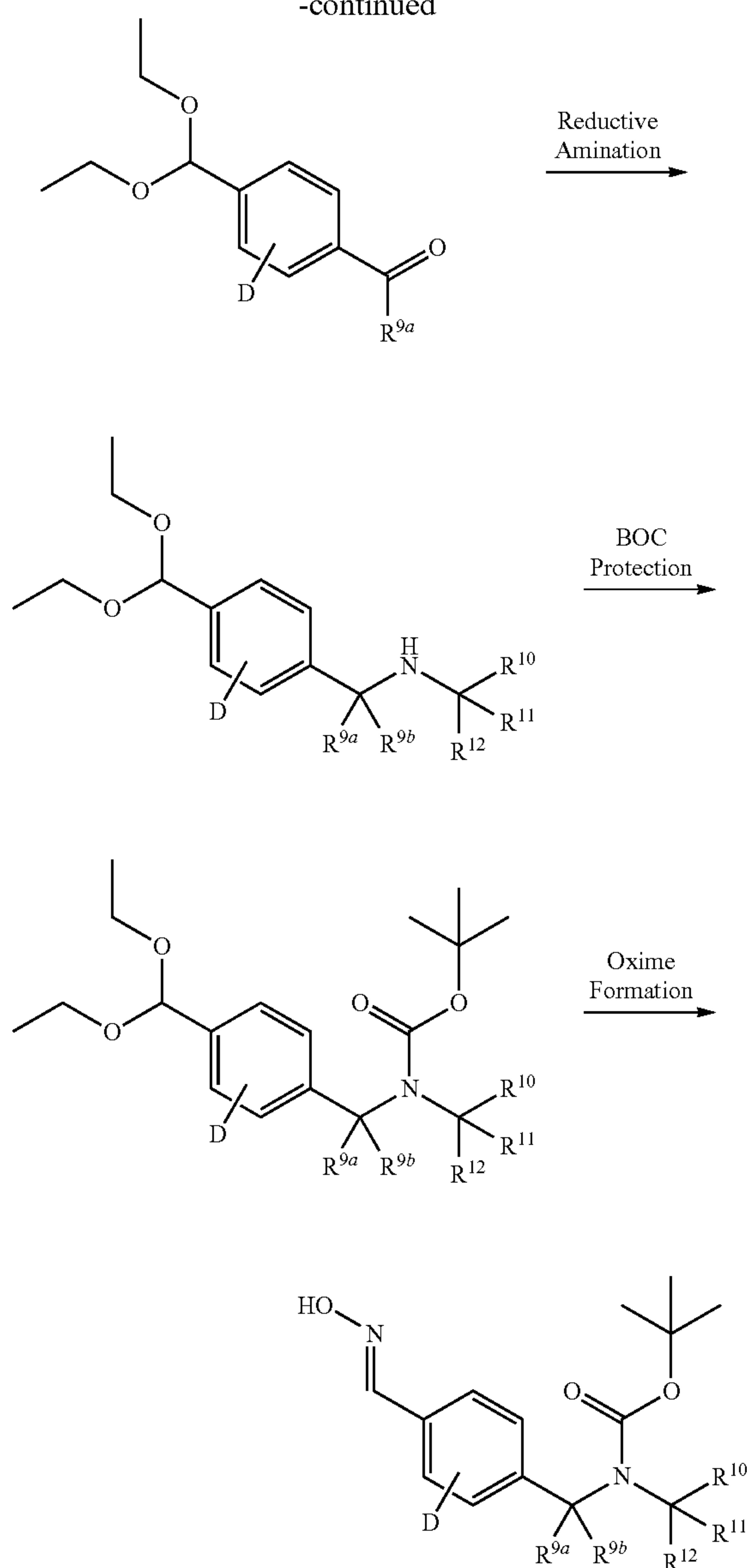
5 SCHEME I: Formation of aryl ring deuterated oxime intermediates
