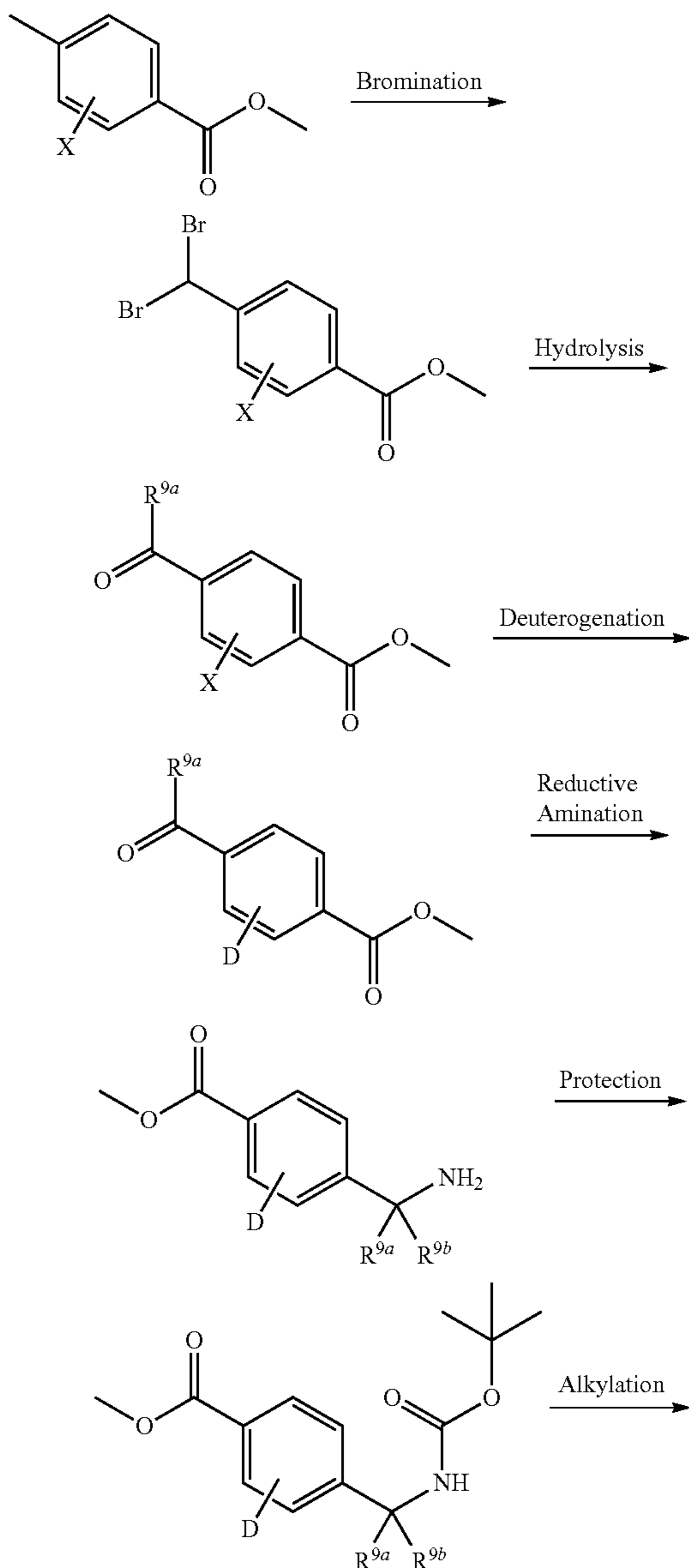
SCHEME K: Formation of aryl ring deuterated oxime intermediates
