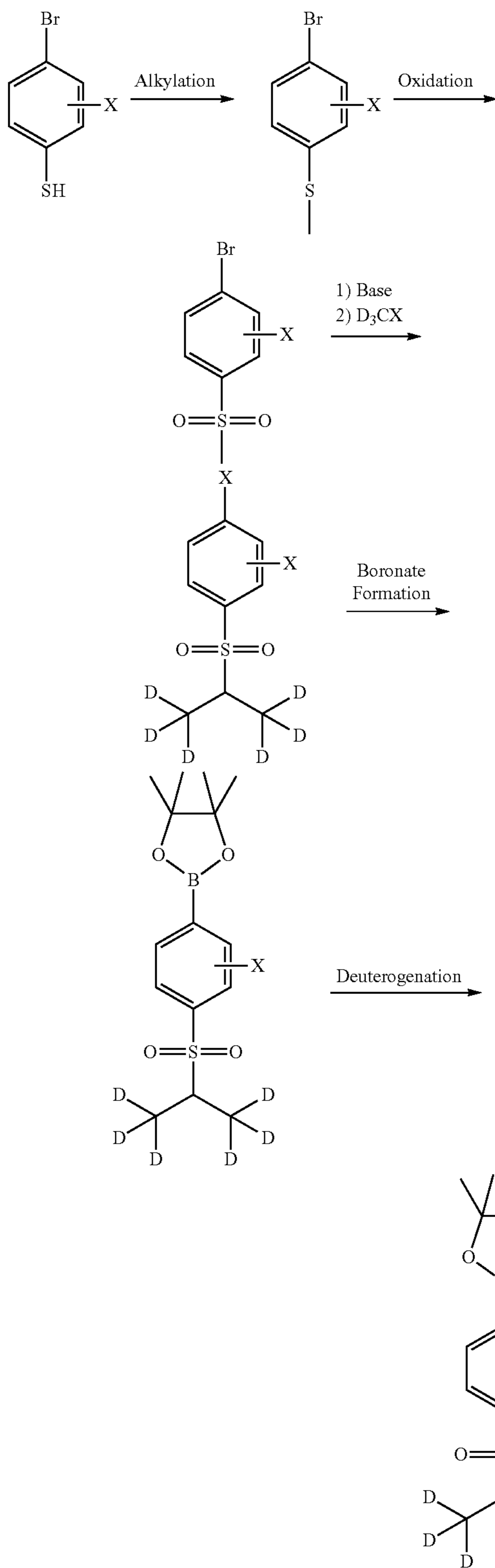
SCHEME G: Formation of aryl ring deuterated boronate
