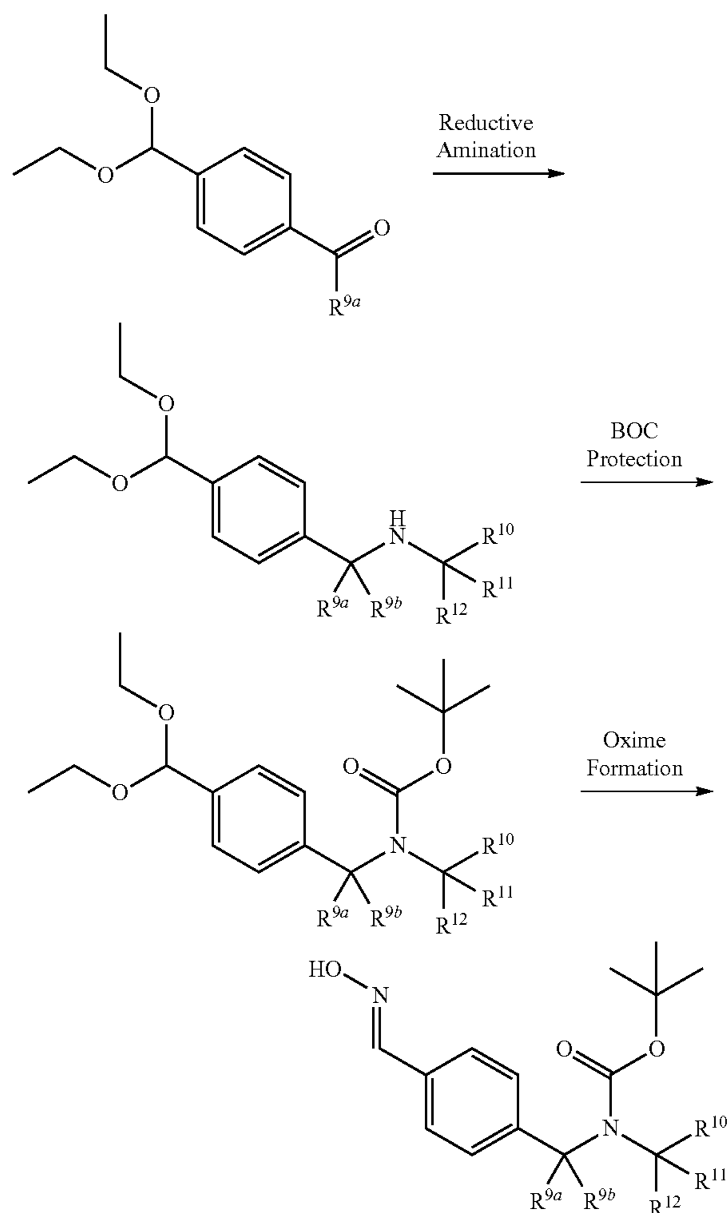
SCHEME L: Formation of deuterated oxime intermediates
