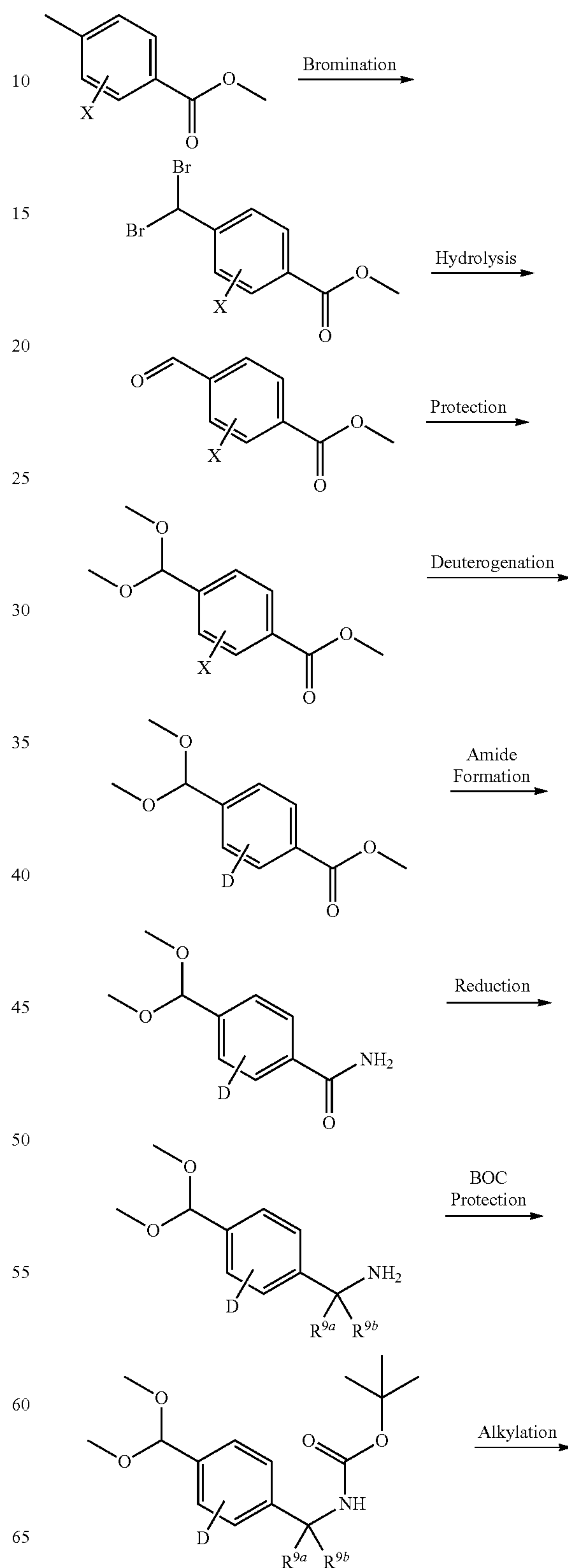
5 SCHEME I: Formation of aryl ring deuterated oxime intermediates
