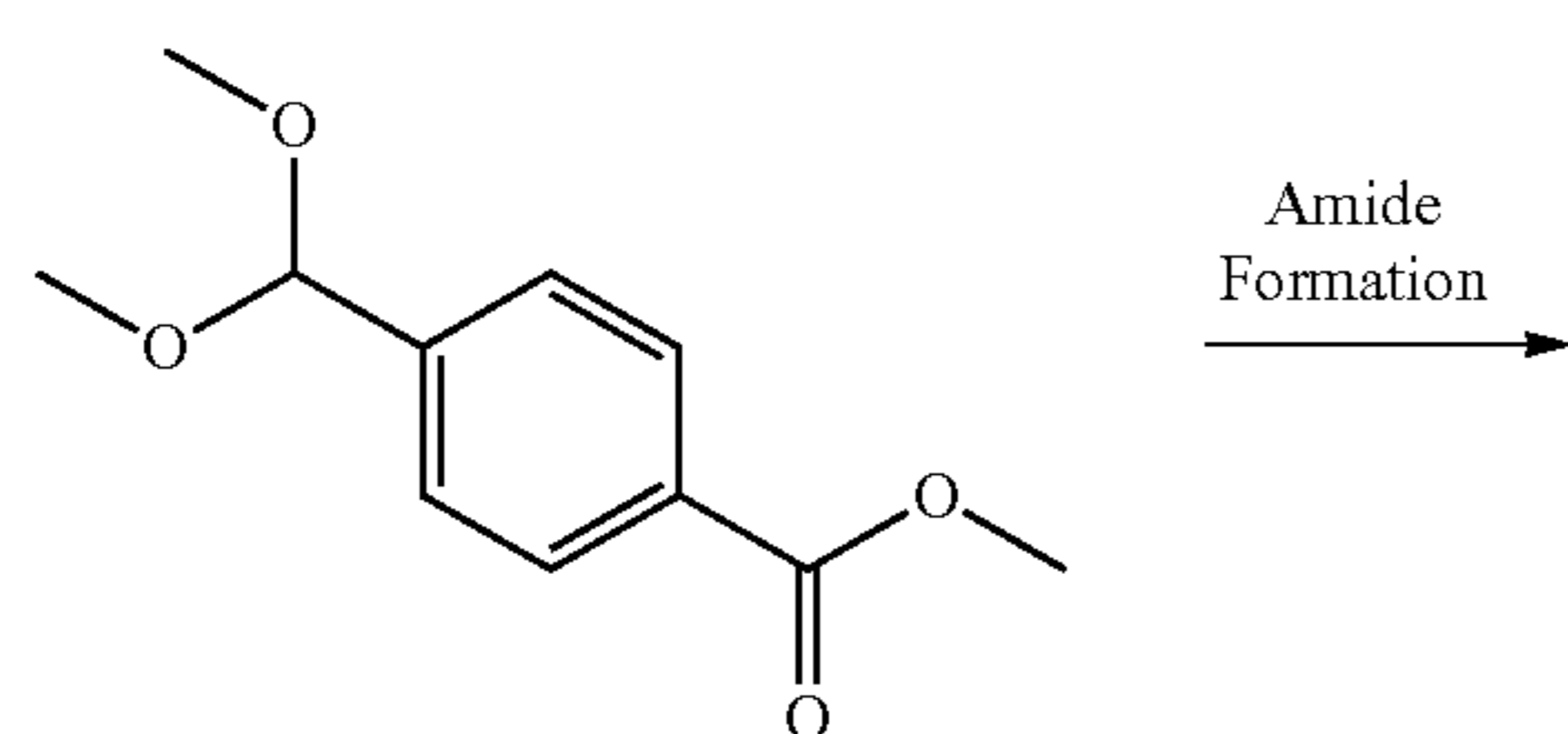
SCHEME M: Formation of deuterated oxime intermediates
