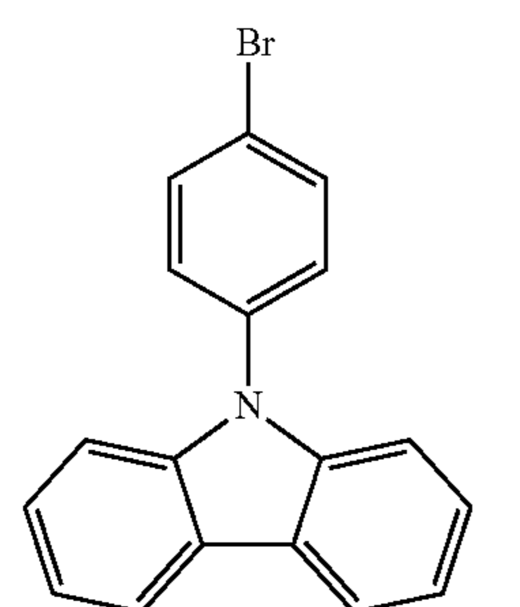
9-(4-bromophenyl)-9H-carbazole
