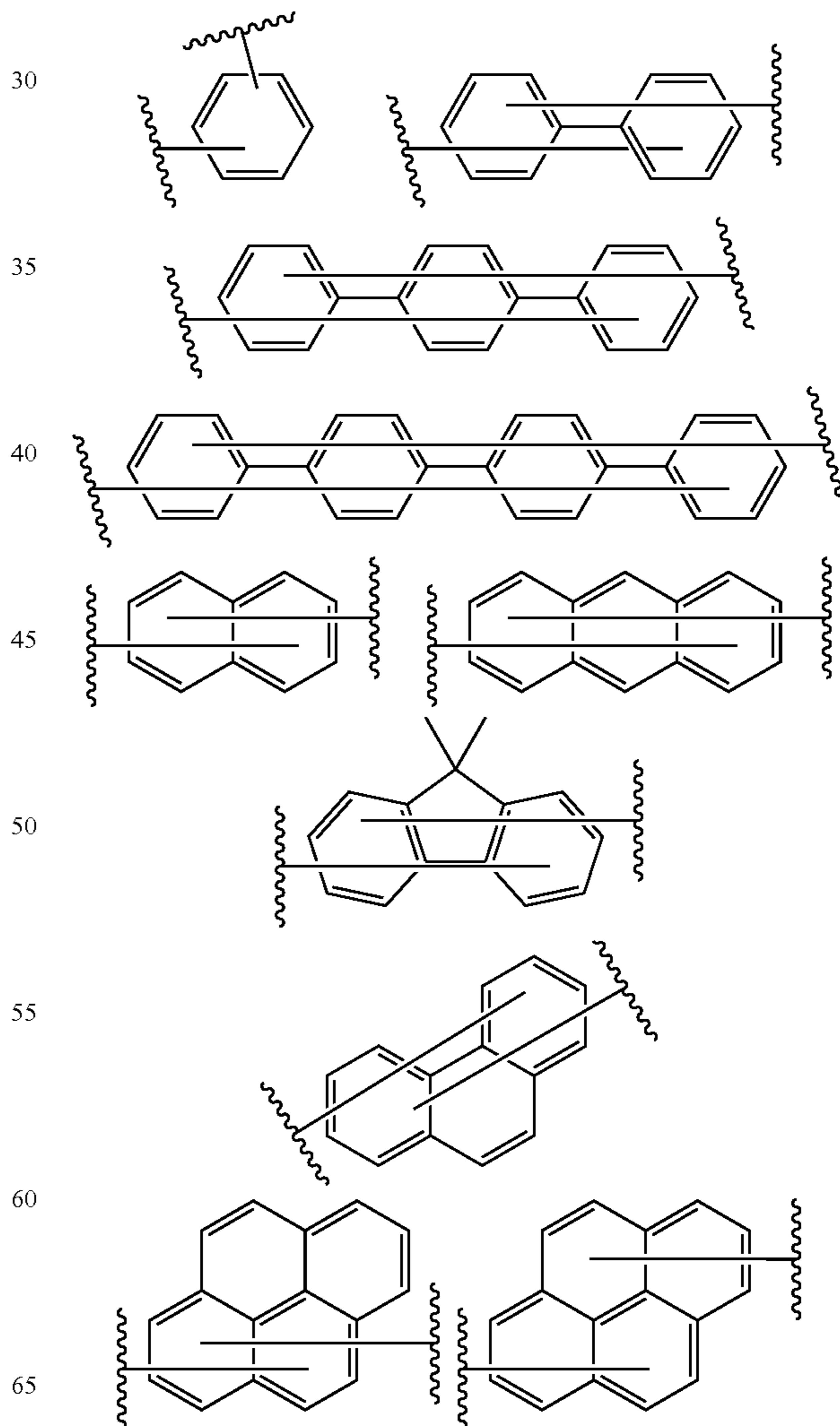
[Chemical Formula 9]
