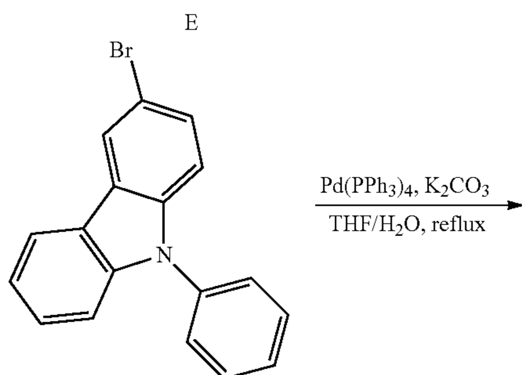
3-bromo-9-phenyl-9H-carbazole
