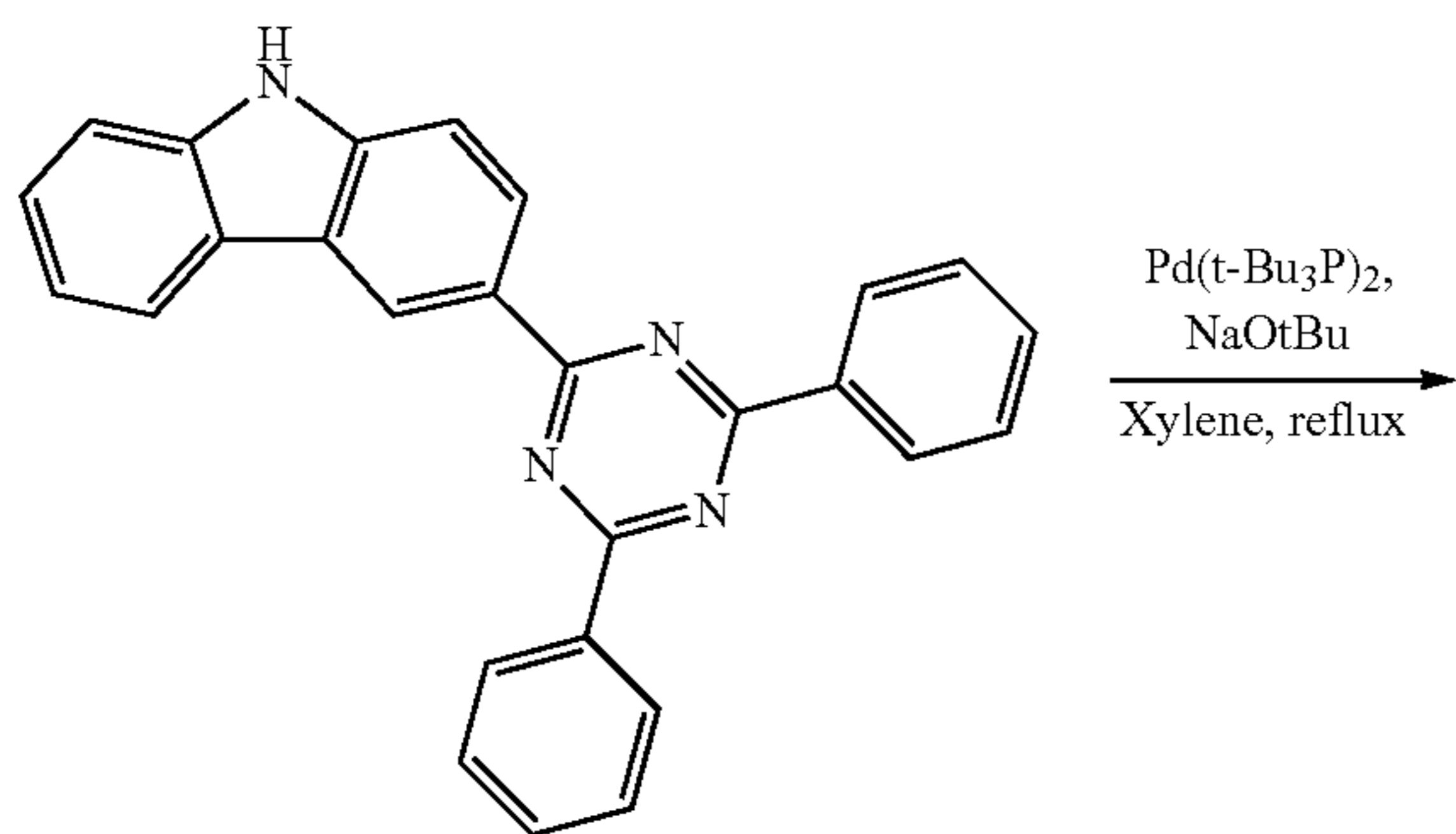
3-(4,6-diphenyl-1,3,5-triazin-2-yl)-9H-carbazole
