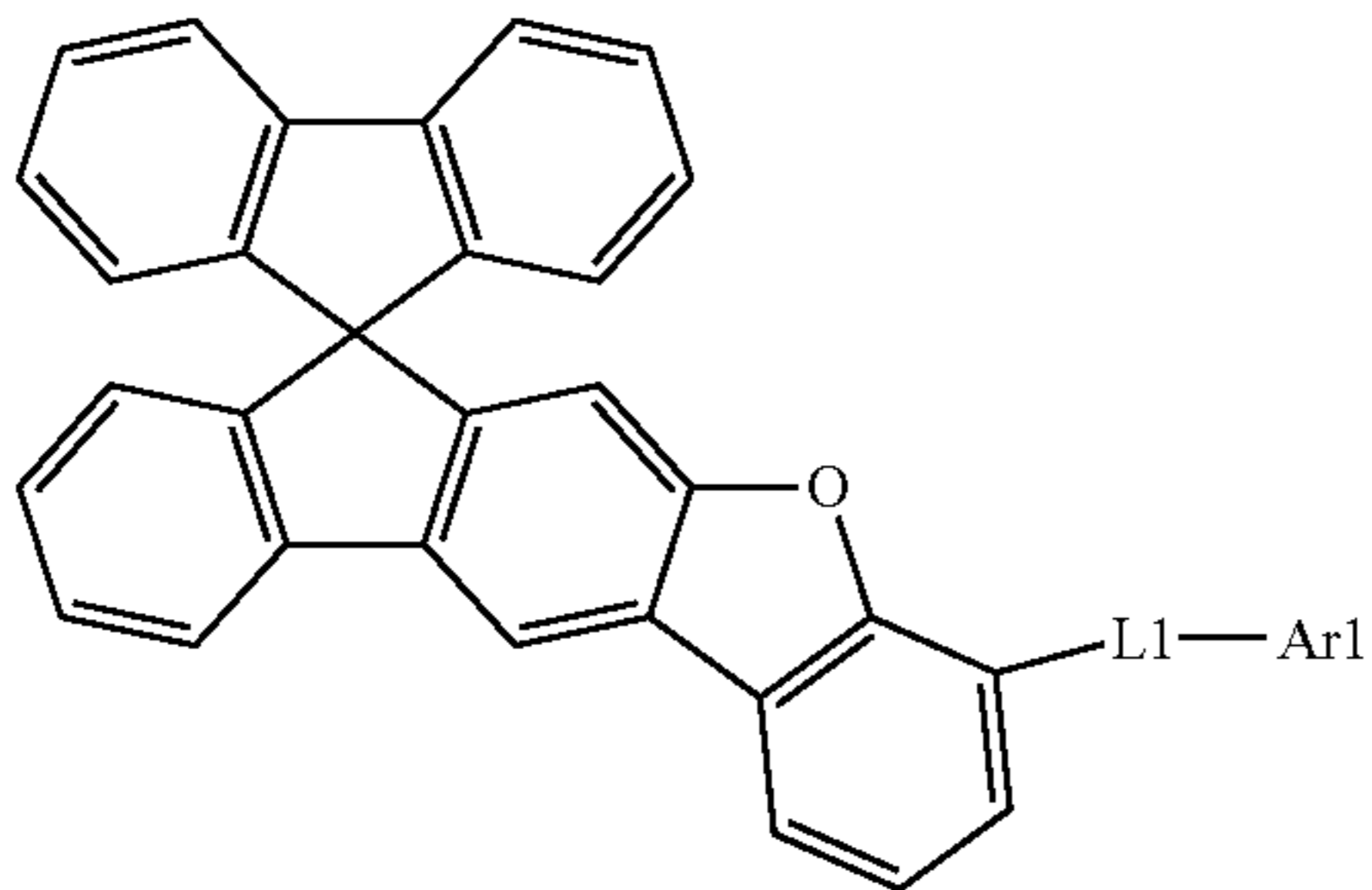
[Chemical Formula 8]
