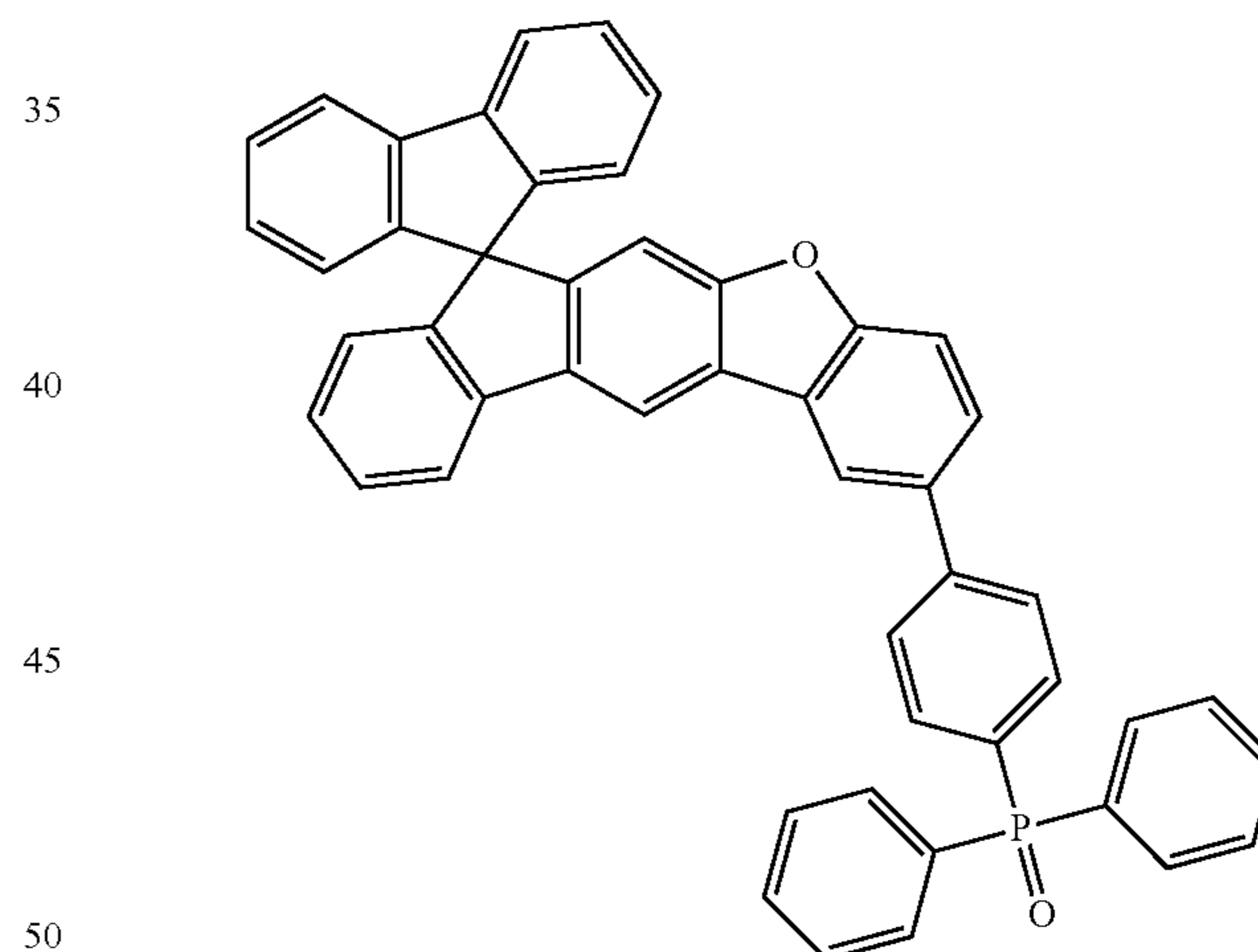
(4-bromophenyl)diphenylphosphine oxide
