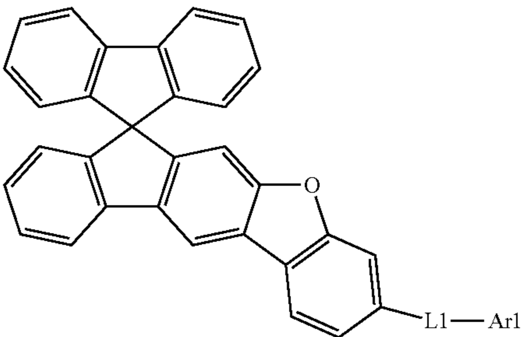
[Chemical Formula 9]
