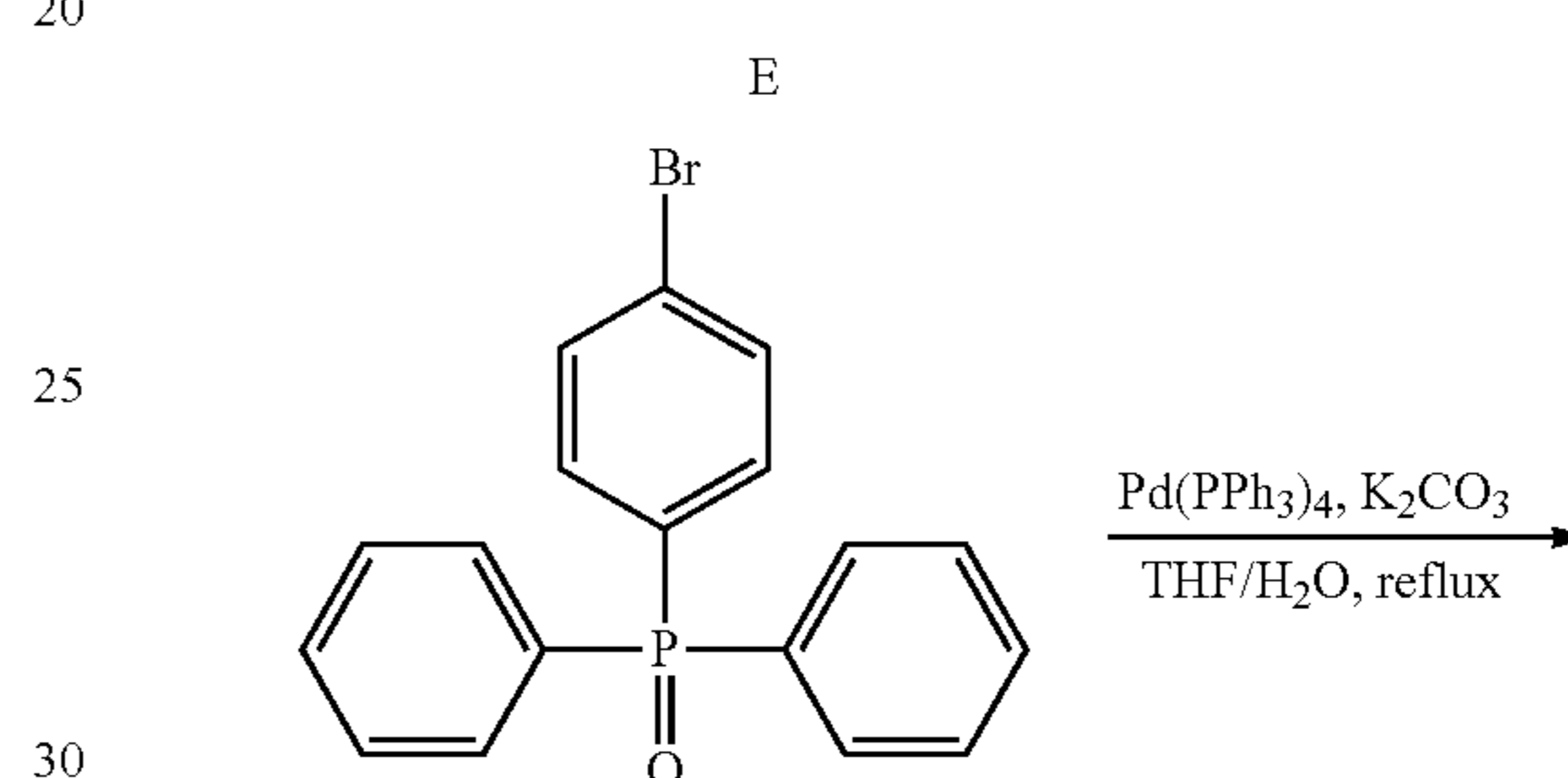
(4-bromophenyl)diphenylphosphine oxide
