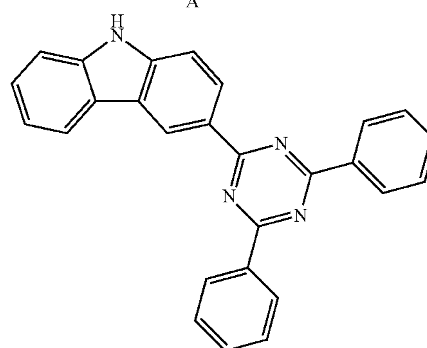
3-(4,6-diphenyl-1,3,5-triazin-2-yl)-9H-carbazole
