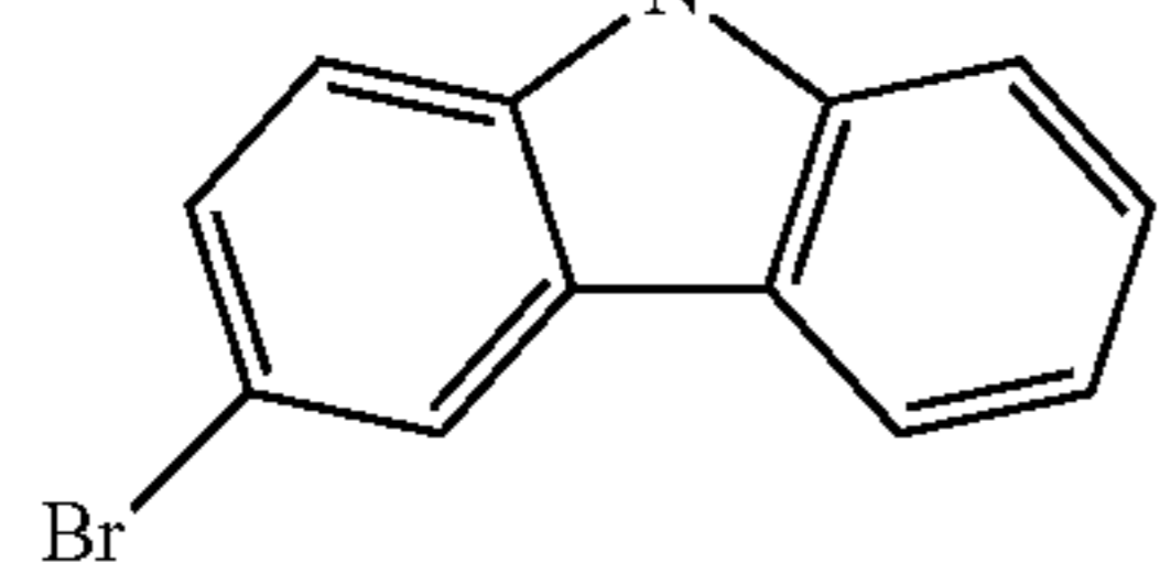
3-bromo-9-(4,6-diphenyl-1,3,5-triazin-2-yl)-9H-carbazole
