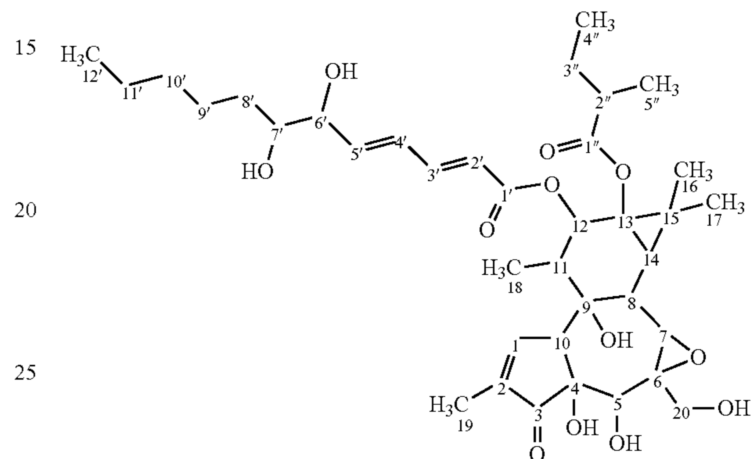
Compound 10: 12-[(2E,4E)-6-oxohexa-2,4-dienyl]-13-(2-methylbutanoyl)-6,7-epoxy-4,5,9,12,13,20-hexahydroxy-1-tiglaen-3-one
