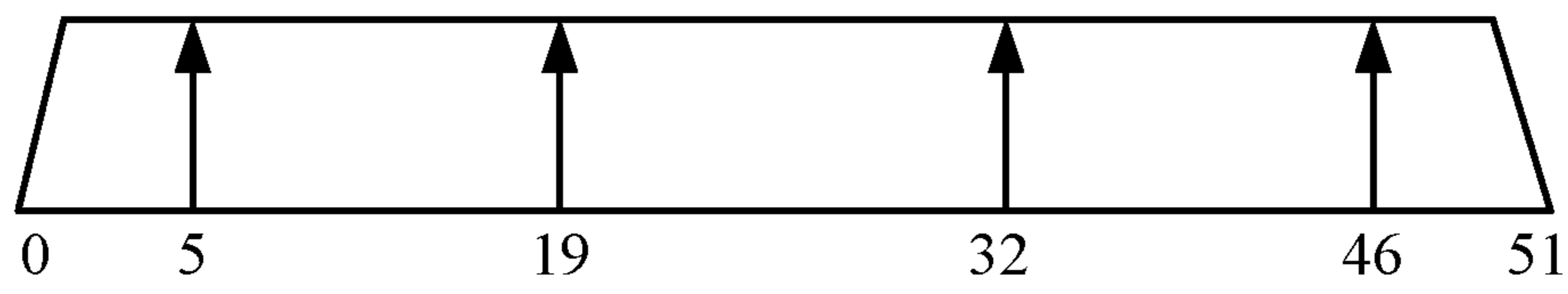
11a 52-tone pilot structure
