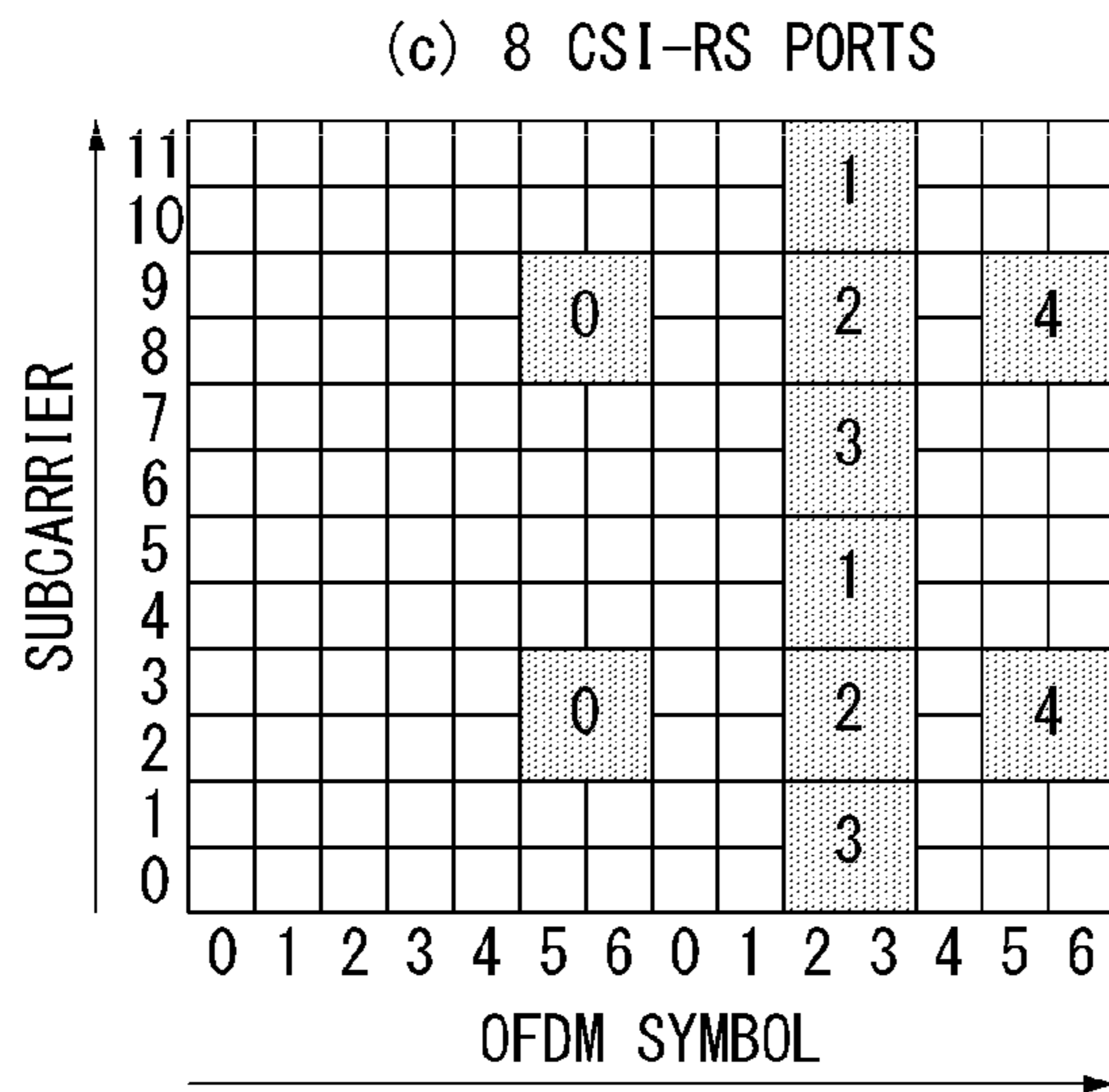
i :CSI-RS CONFIGURATION AVAILABLE FOR 8 CSI-RS PORTS
