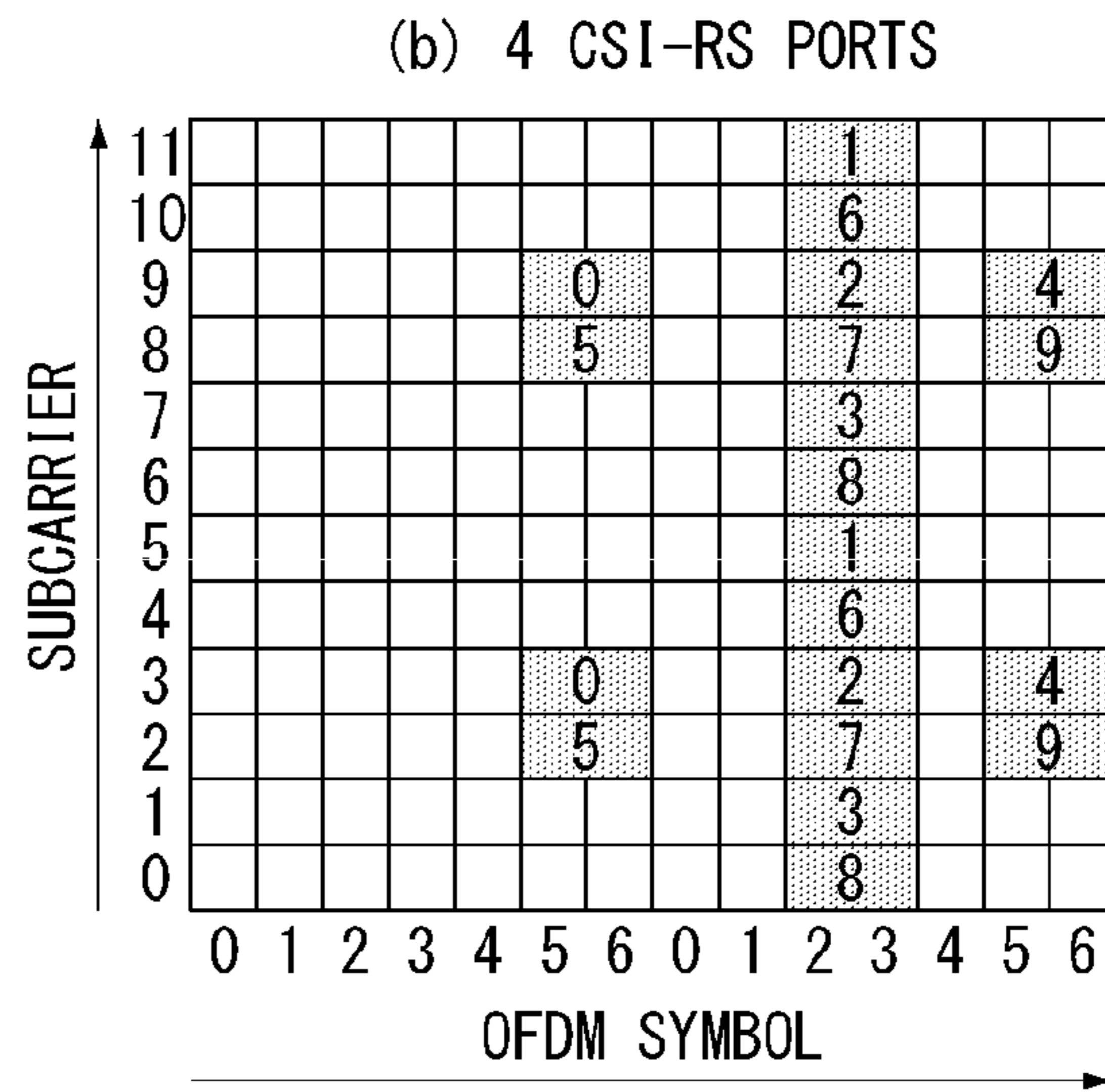
i :CSI-RS CONFIGURATION AVAILABLE FOR 4 CSI-RS PORTS
