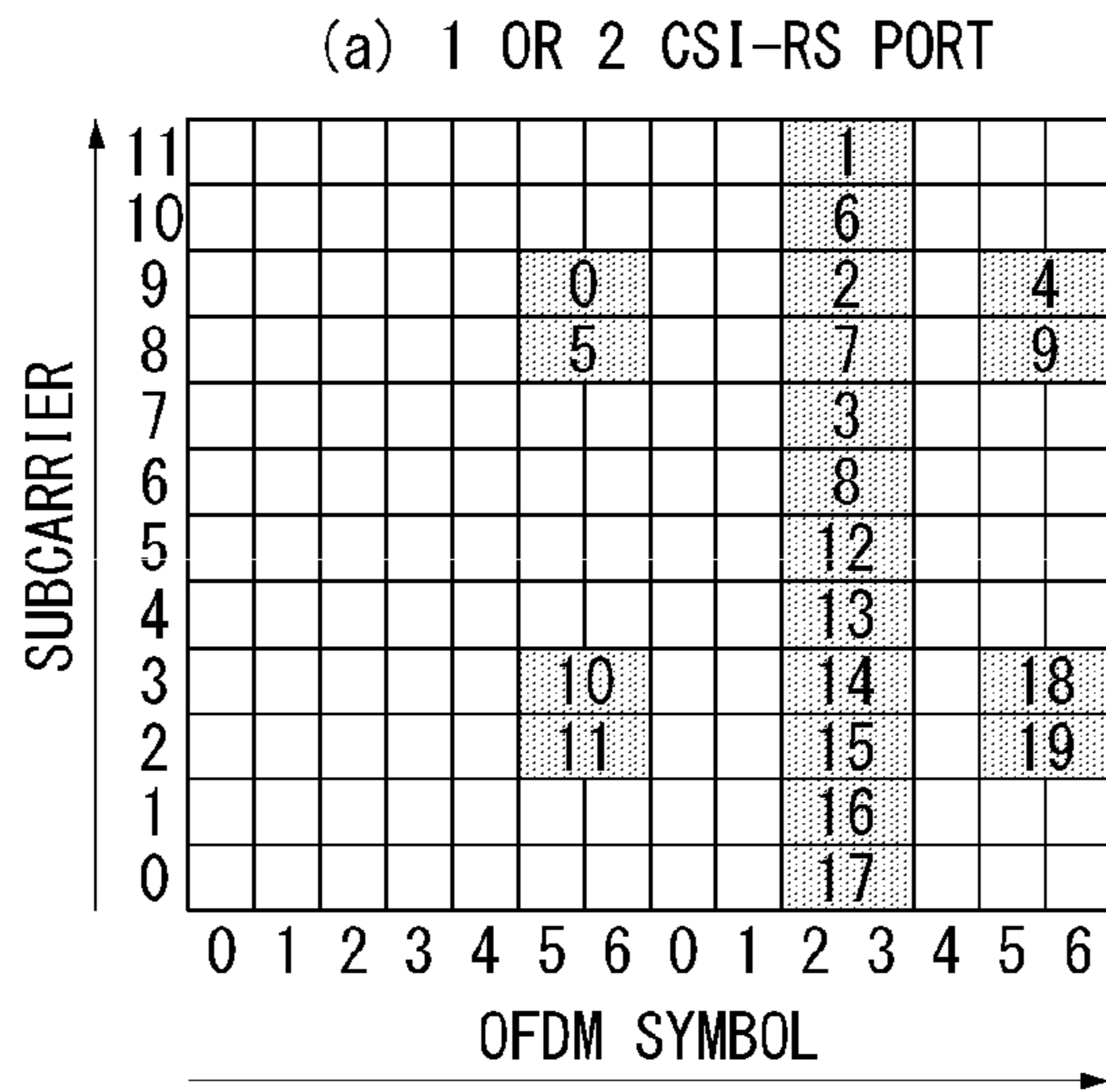
i :CSI-RS CONFIGURATION AVAILABLE FOR 1 OR 2 CSI-RS PORT
