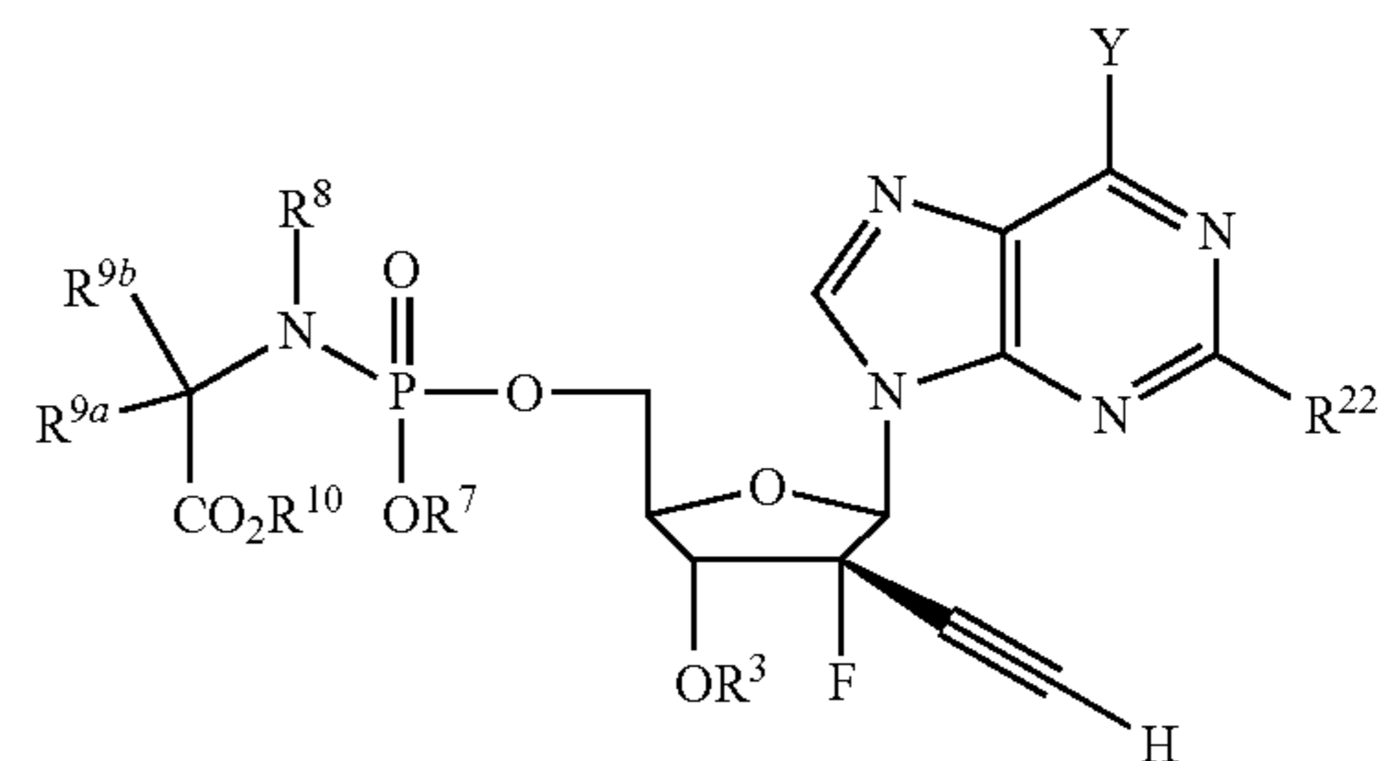
Formula V
