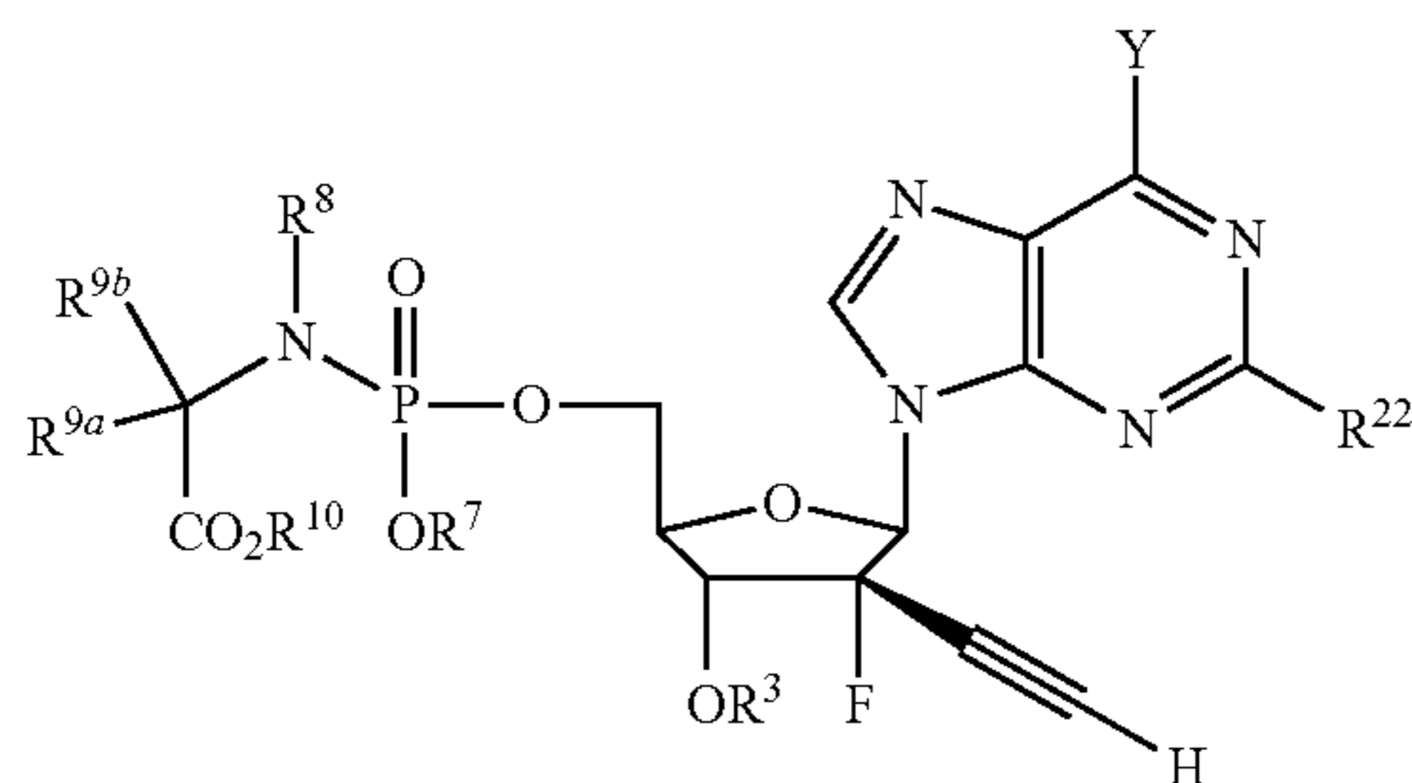
Formula V
