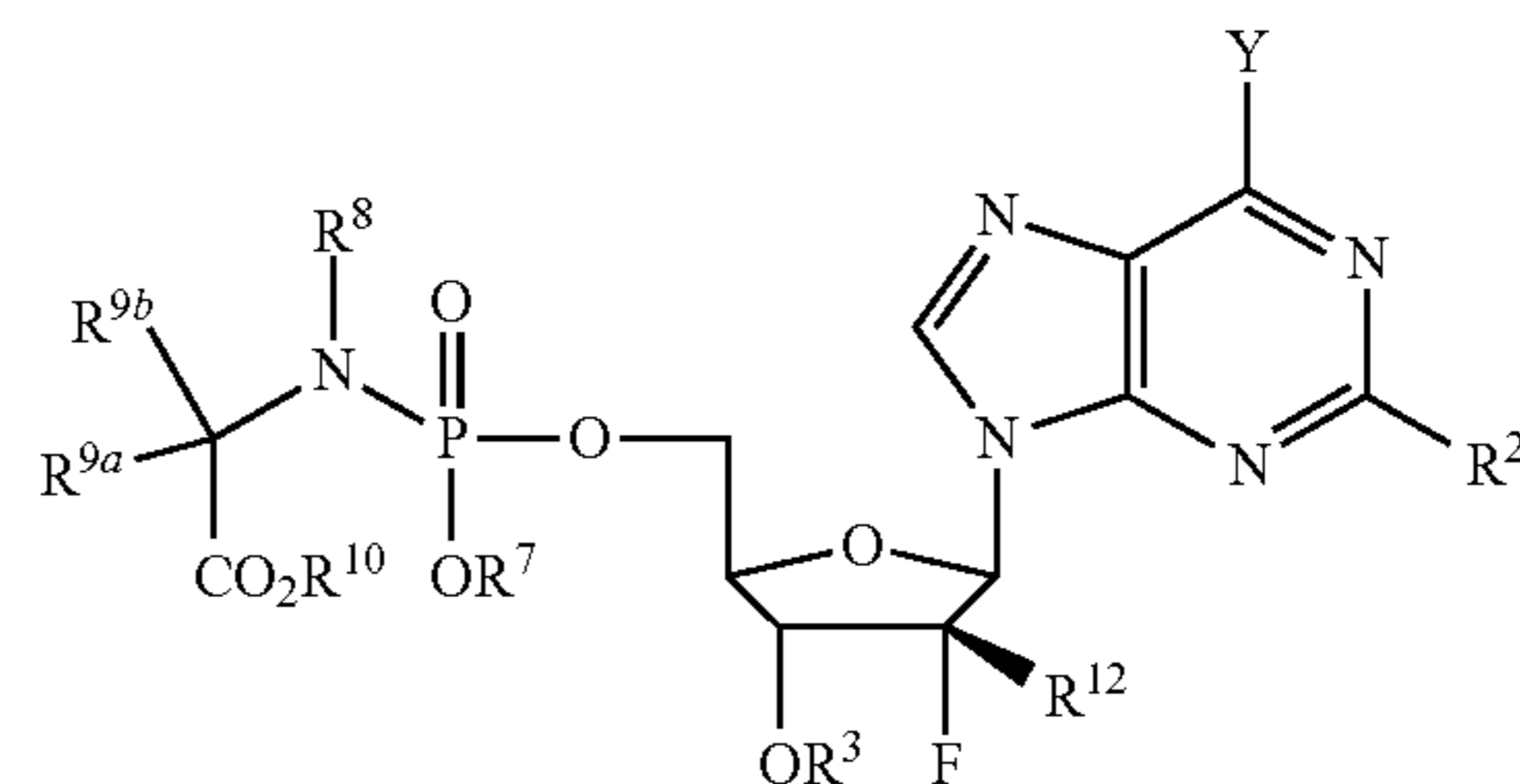
Formula III
