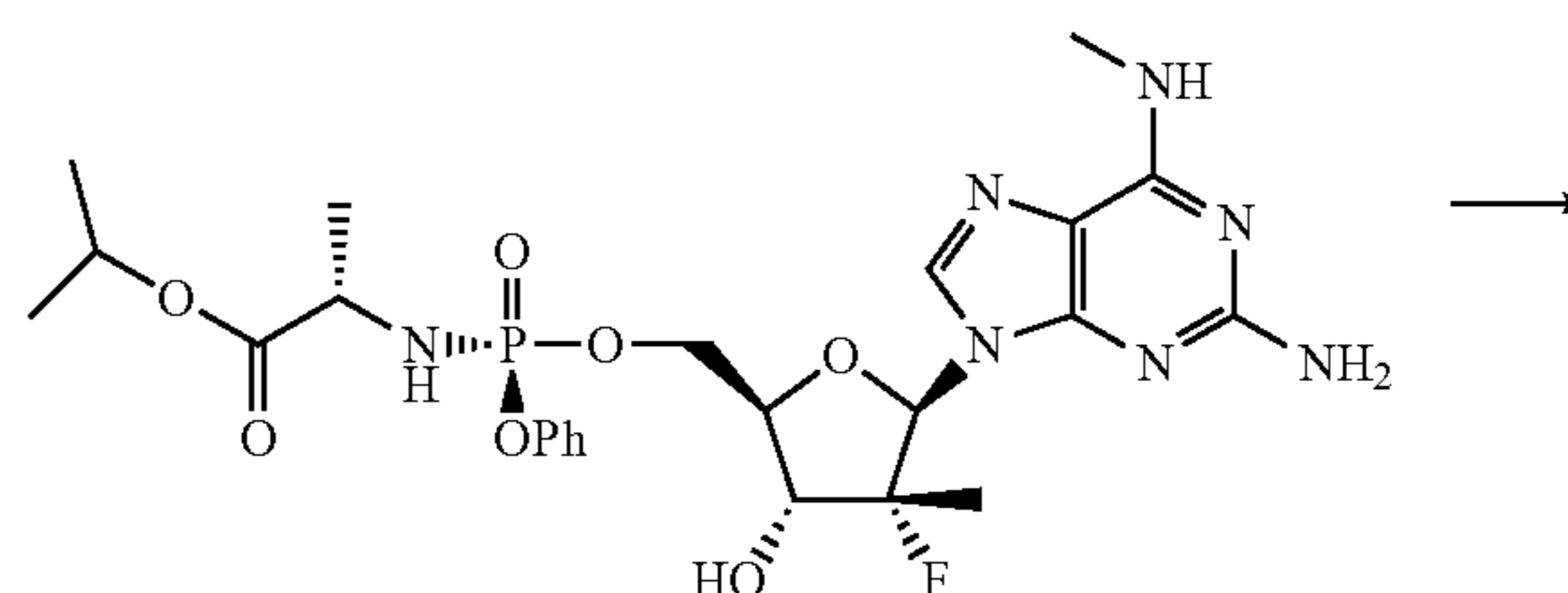
Scheme 1
