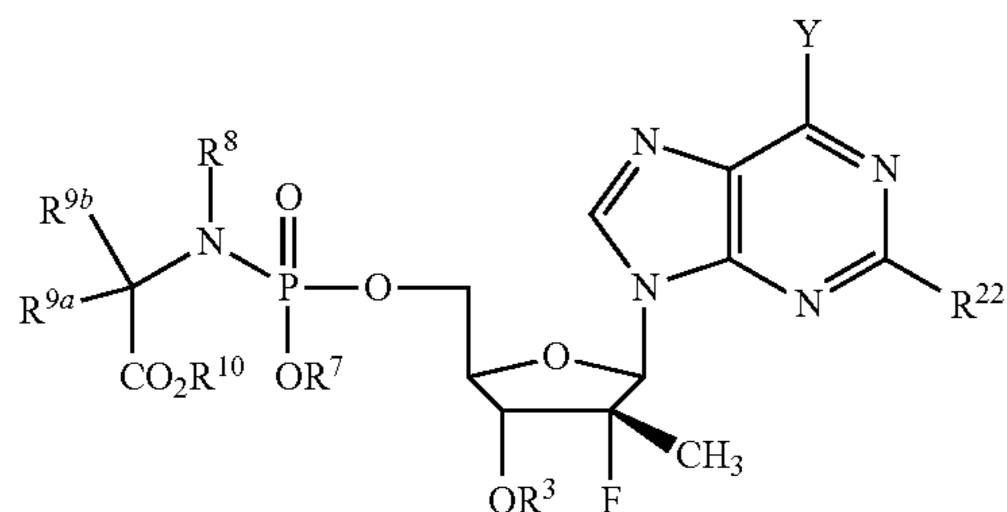
Formula IV
