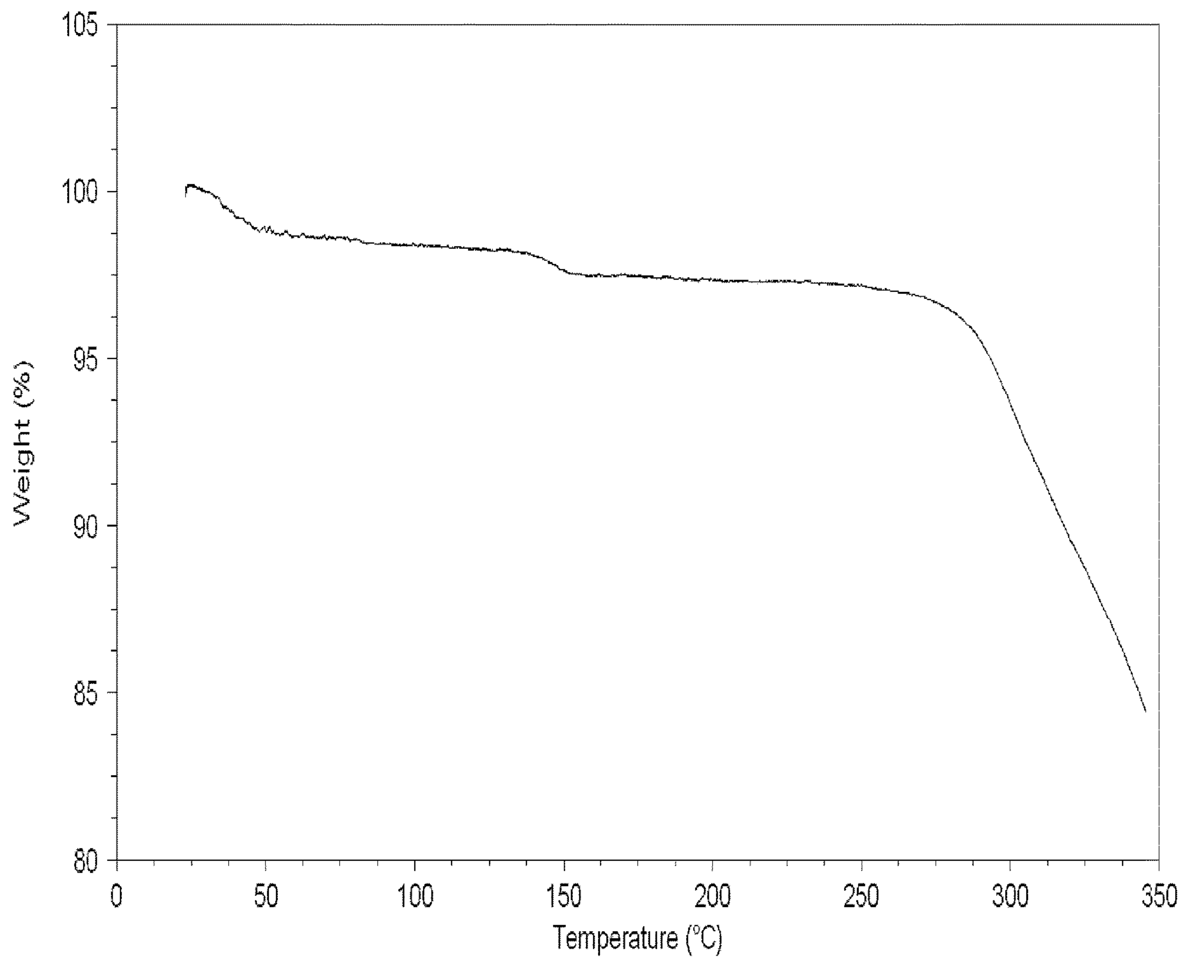
FIGURE 2d: TGA Compound I-1 (anhydrous form B)
