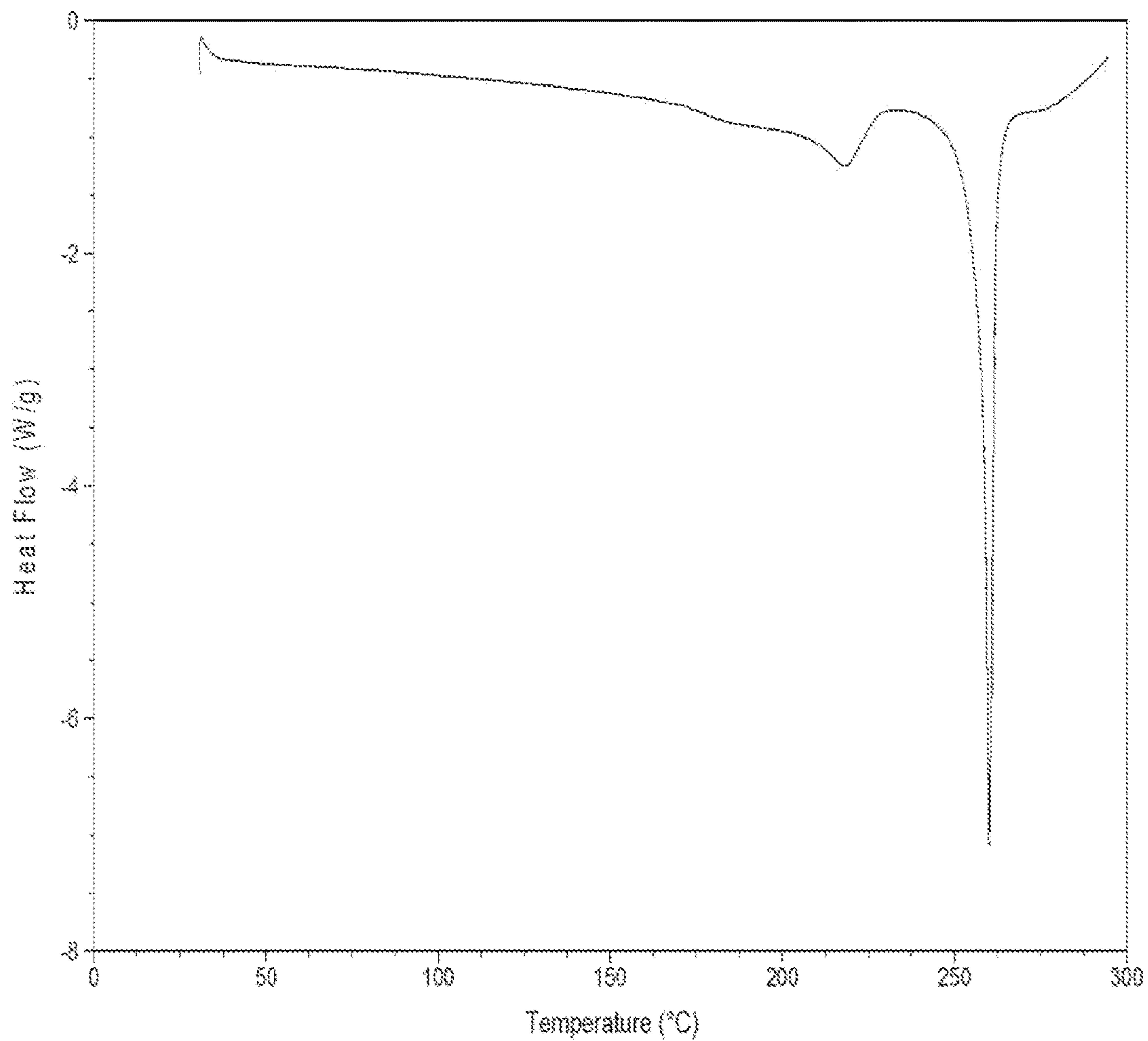
FIGURE 3a: DSC Compound I-1 (ethanol solvate)
