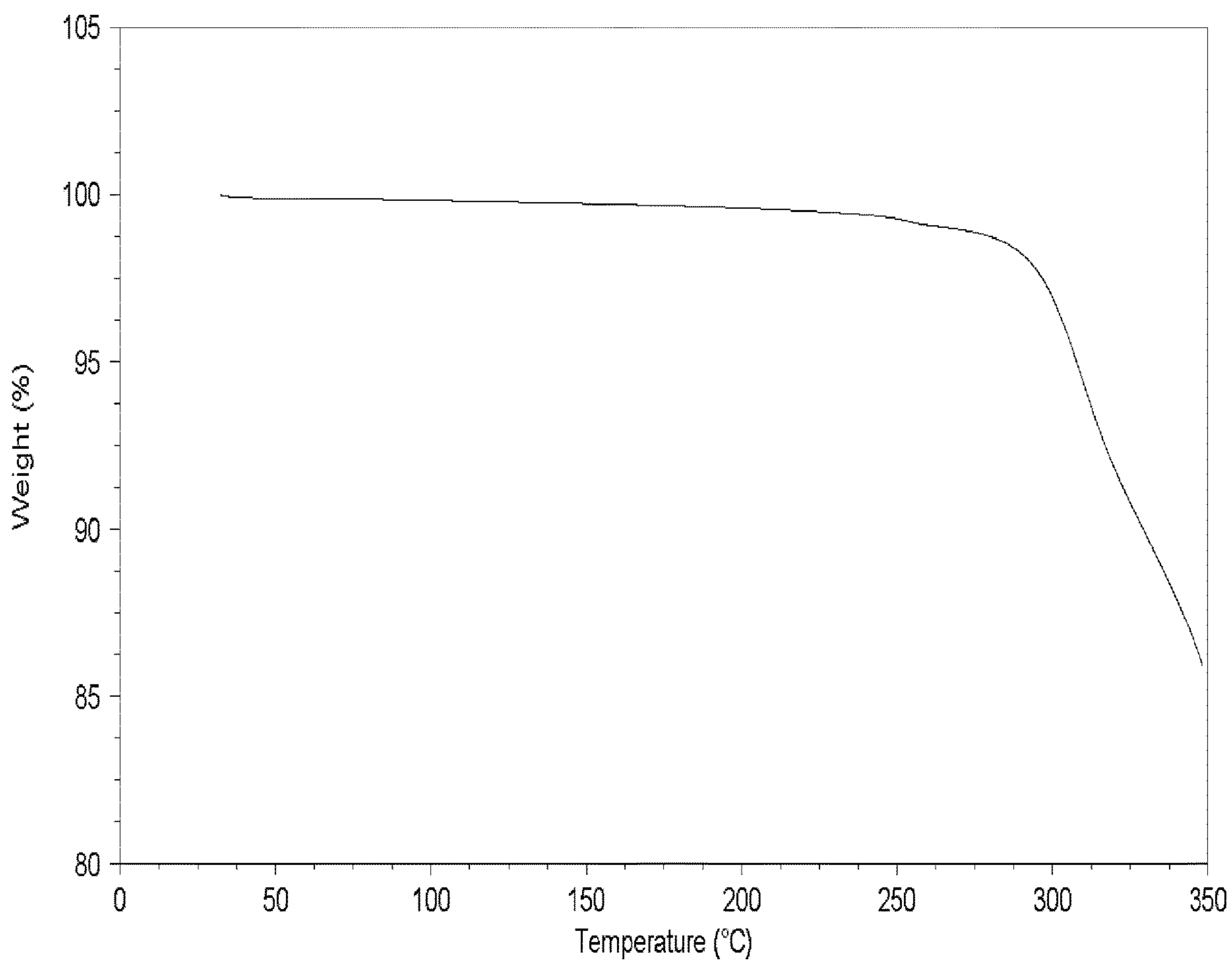
FIGURE 2c: TGA Compound I-1 (anhydrous form A)
