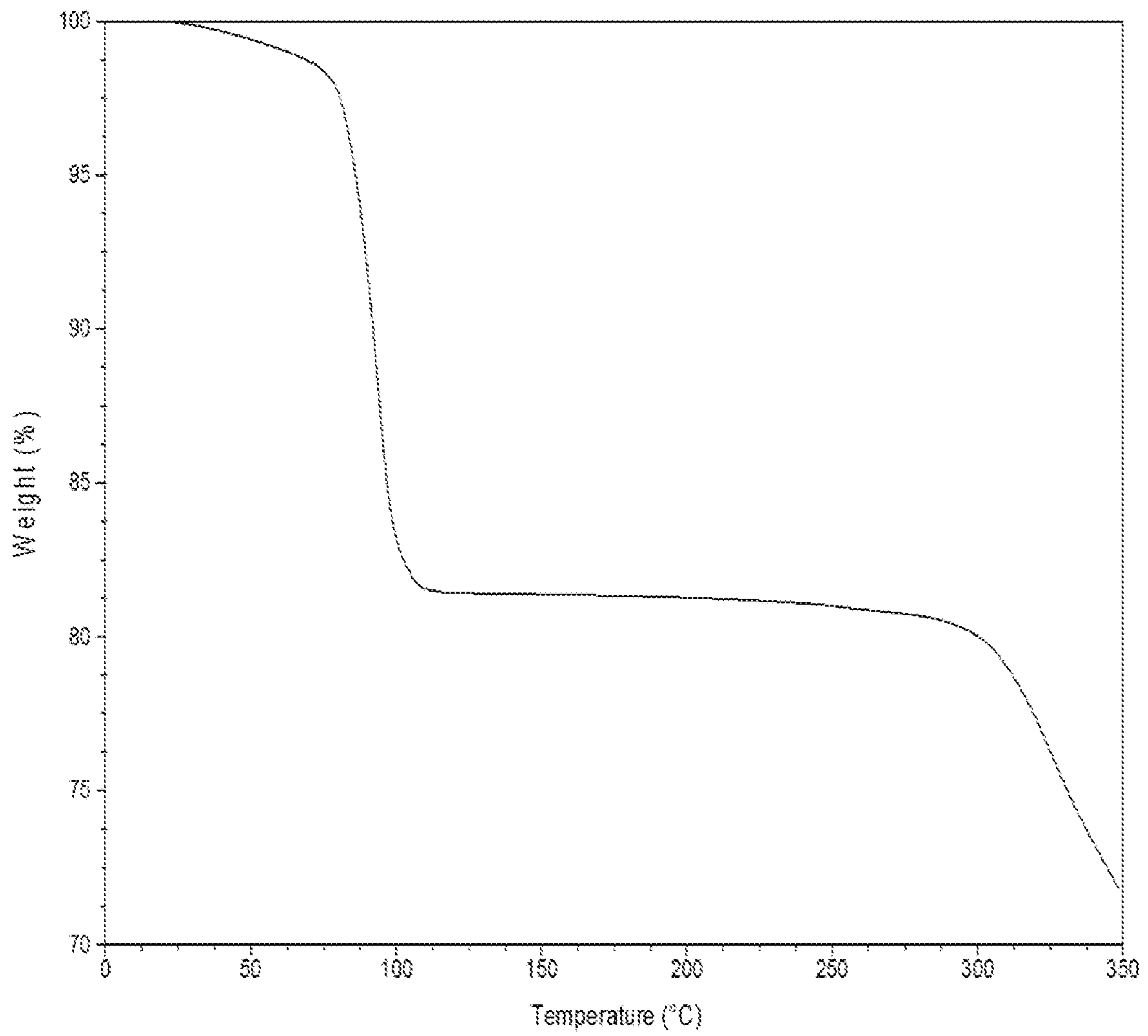
FIGURE 2h: TGA Compound I-1 (DMAC solvate)
