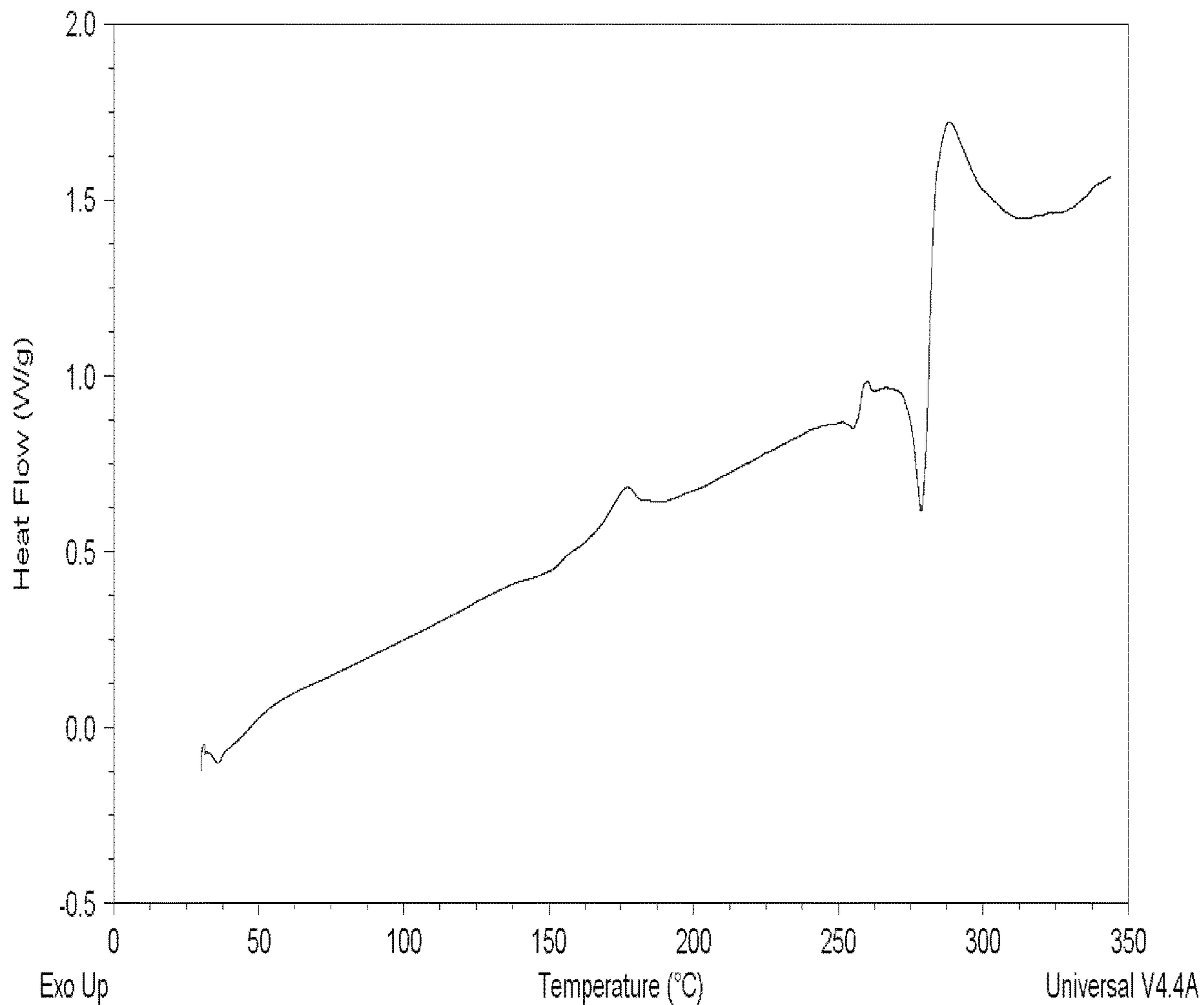
FIGURE 3d: DSC Compound I-1 (anhydrous form B)
