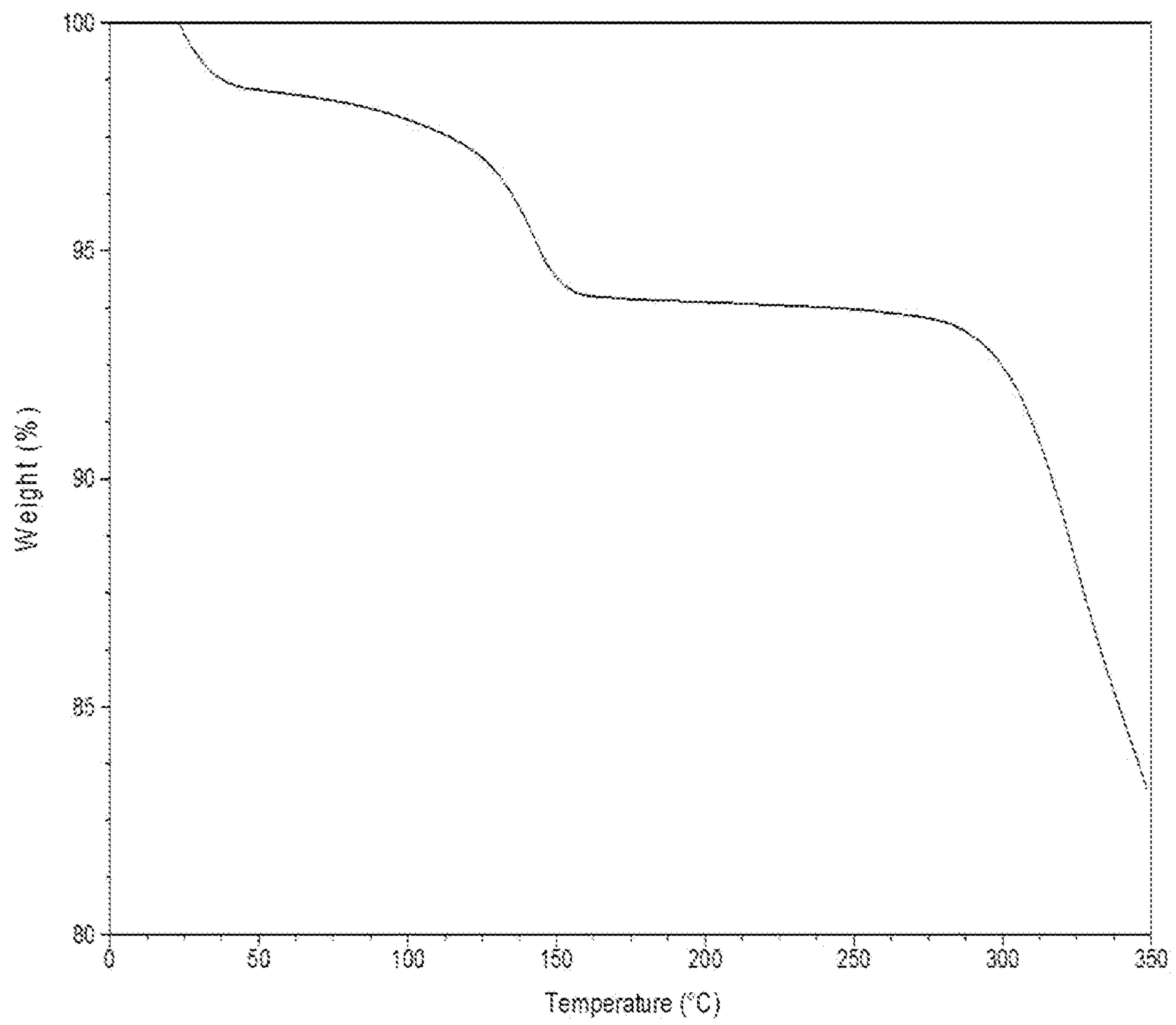
FIGURE 2i: TGA Compound I-1 (acetone solvate)
