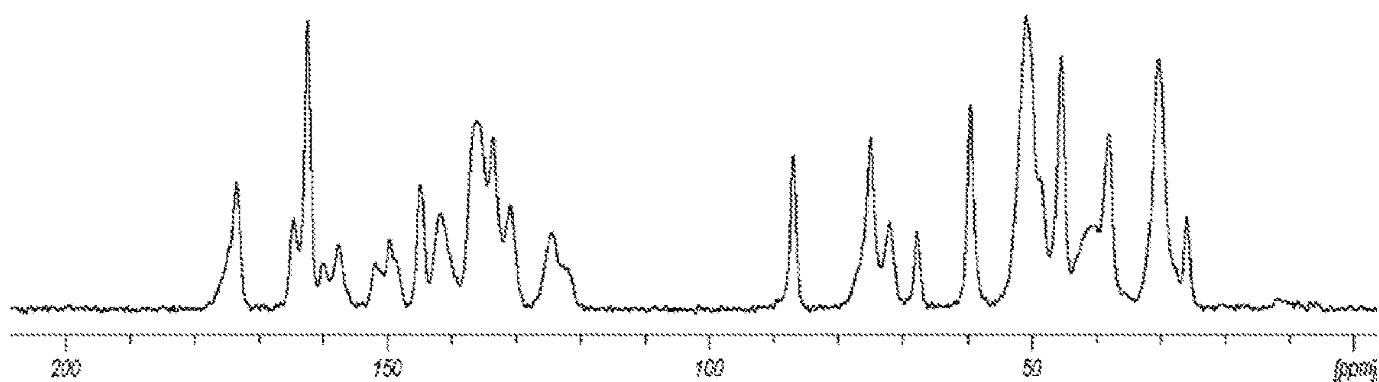
FIGURE 4d: Solid State ^{13}\text{C} NMR Spectrum of Compound I-1 (anhydrous form B)
