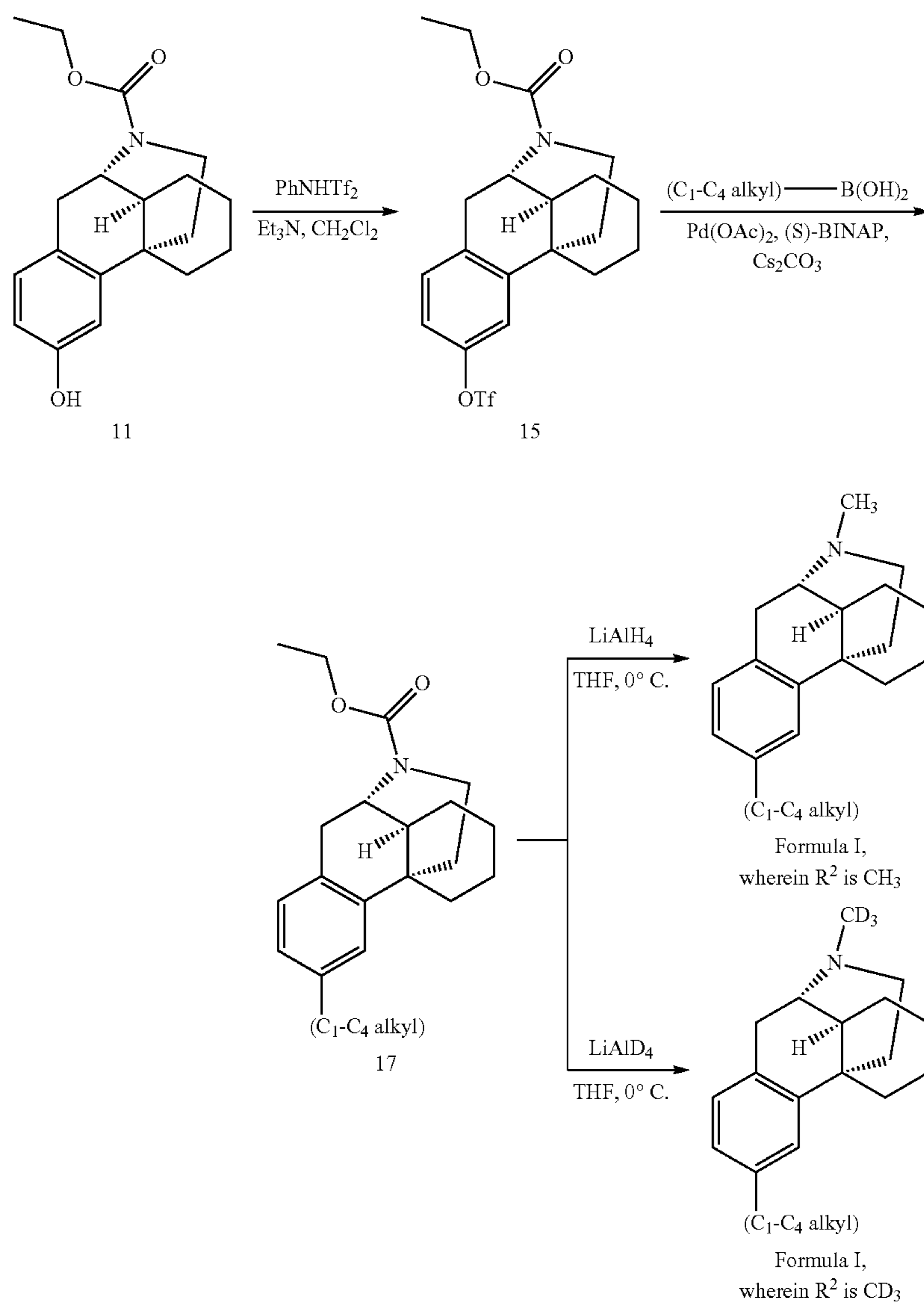
Scheme 2. Synthesis of a Compound of Formula I ( R^1 is -(C_1-C_4) alkyl)
