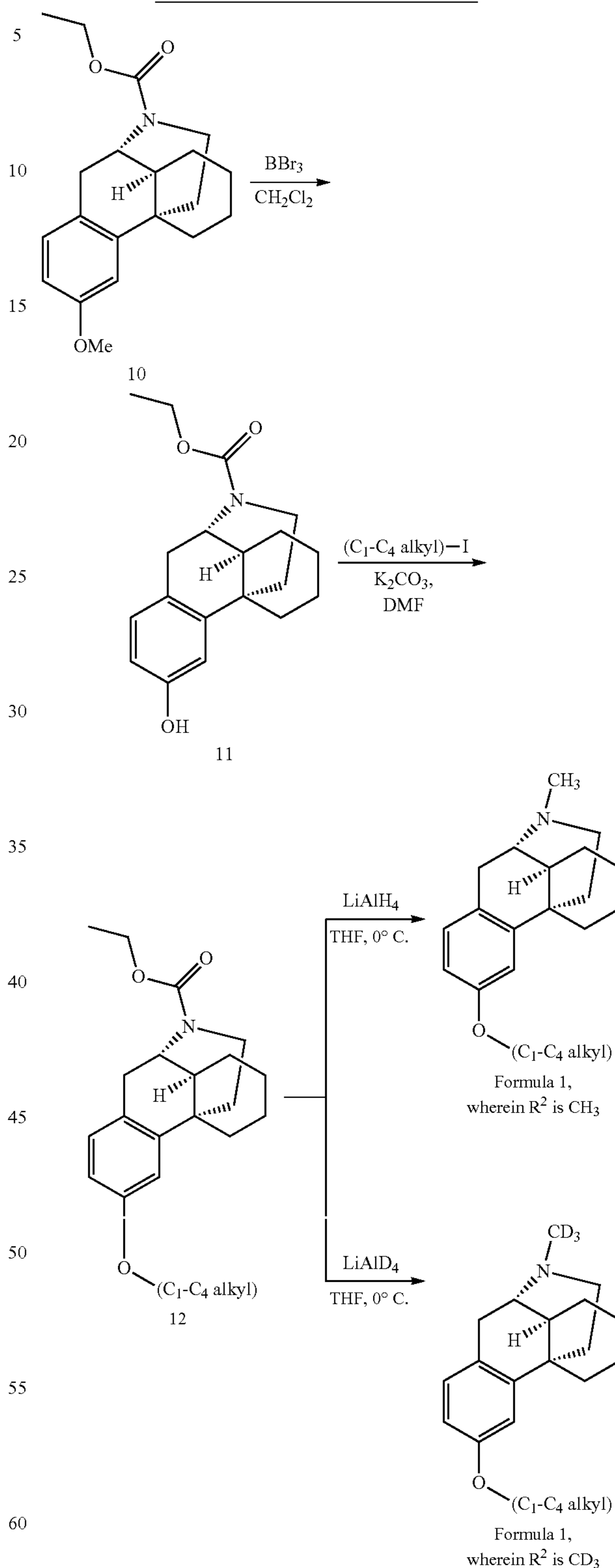
Scheme 1. Synthesis of a Compound of Formula I (R 1 is —O—(C 1 -C 4 )alkyl)
