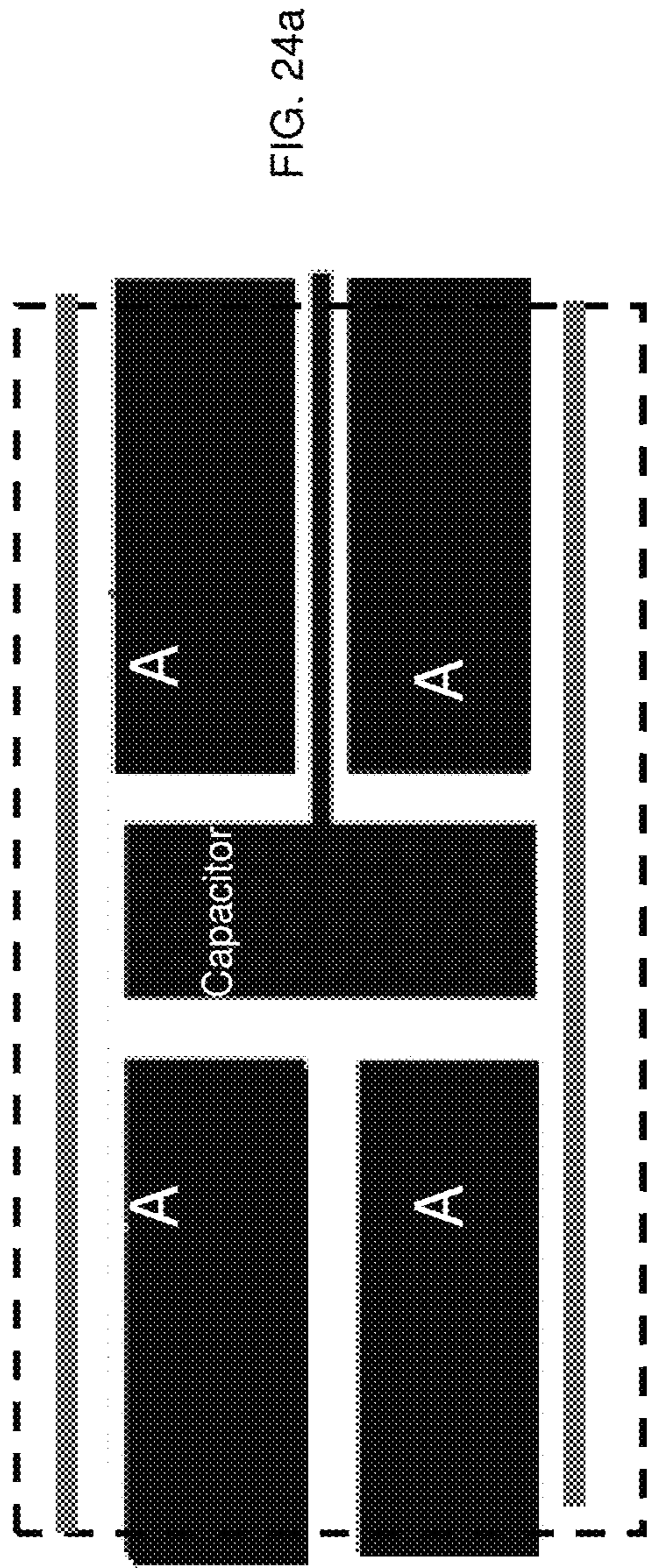
Beam actuation and capacitor or contact area
