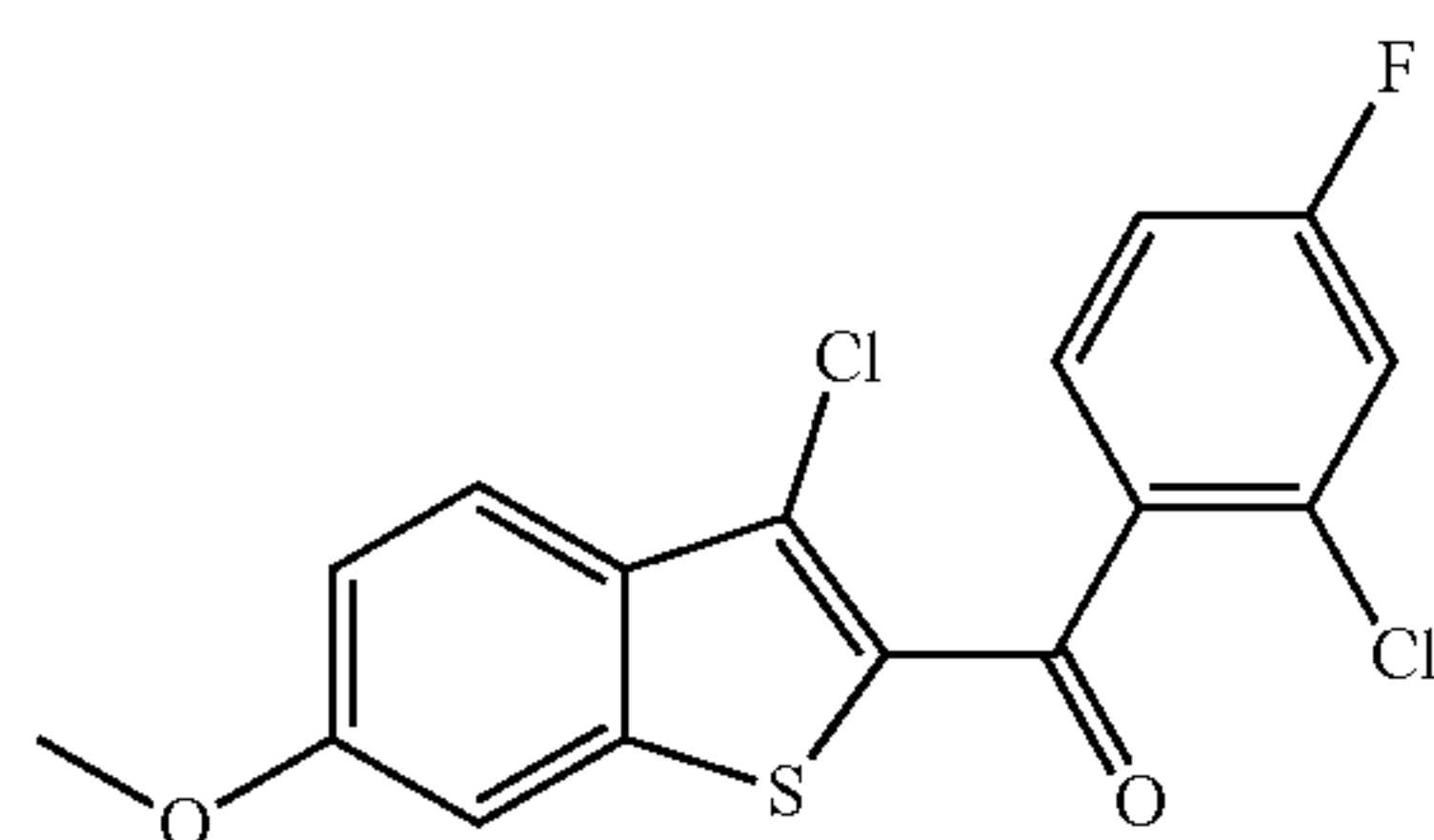
(2-Chloro-4-fluorophenyl)(3-chloro-6-methoxybenzo[b]thiophen-2-yl)methanone
