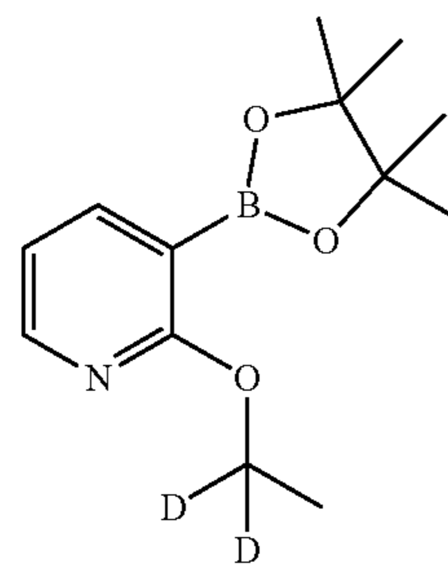
2-(Ethoxy-1,1-d 2 )-3-(4,4,5,5,-tetramethyl-1,3,2-dioxaboran-2yl)pyridine Prepared from 3-bromo-2-(ethoxy-1,1-d 2 )pyridine.
