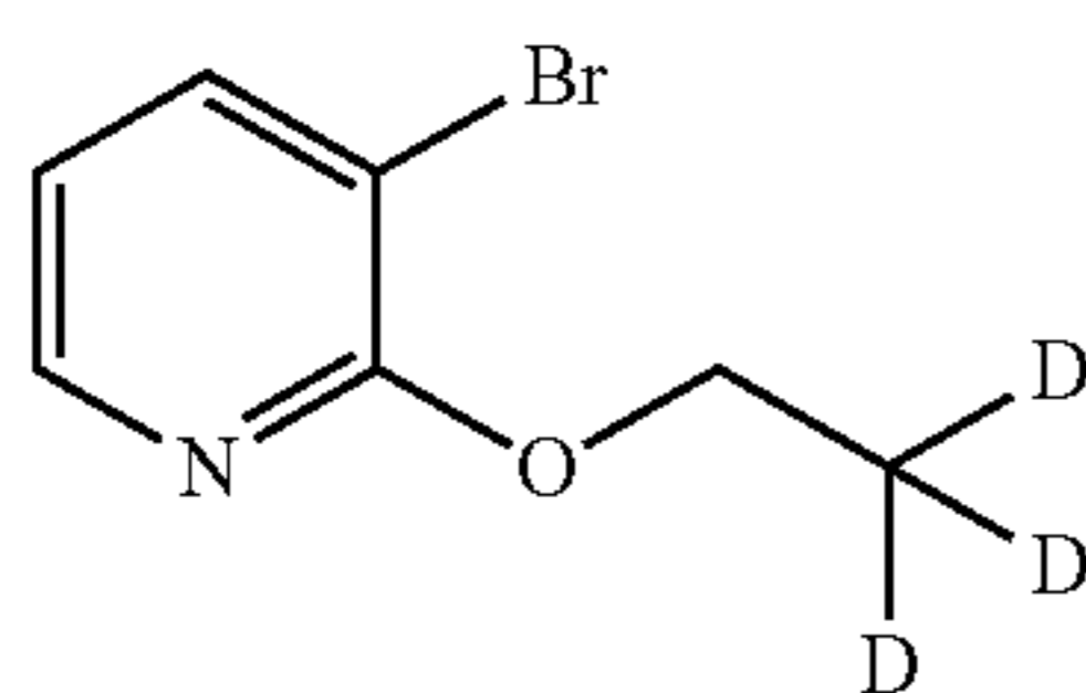
3-bromo-2-(ethoxy-2,2,2-d 3 )pyridine Prepared from 3-bromo-2-fluoropyridine and ethanol-2,2,2-d 3
