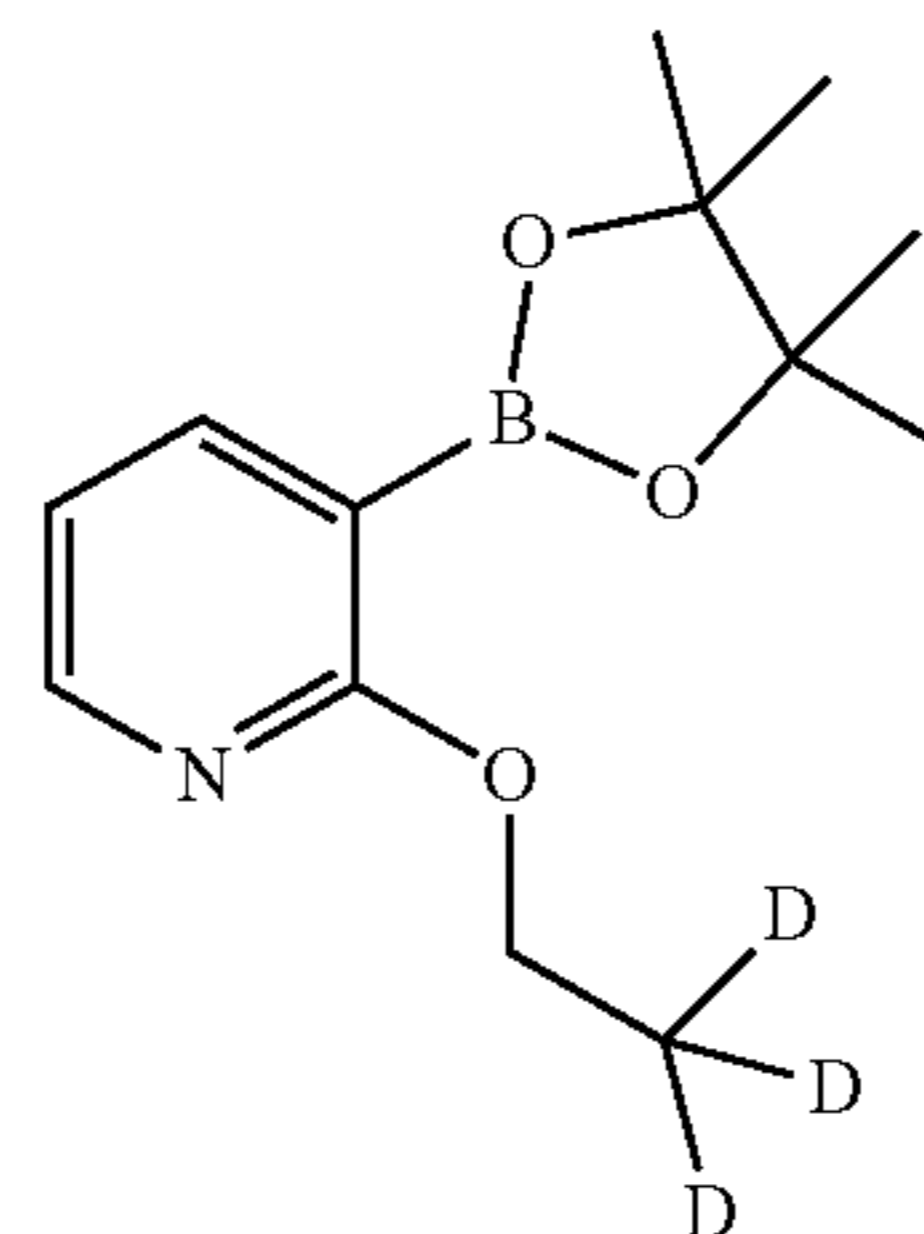
2-(Ethoxy-2,2,2-d 3 )-3-(4,4,5,5,-tetramethyl-1,3,2-dioxaboran-2yl)pyridine Prepared from 3-bromo-2-(ethoxy-2,2,2-d 3 )pyridine.
