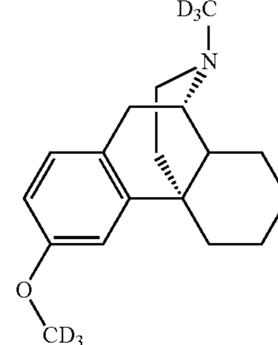
d6-dextromethorphan
