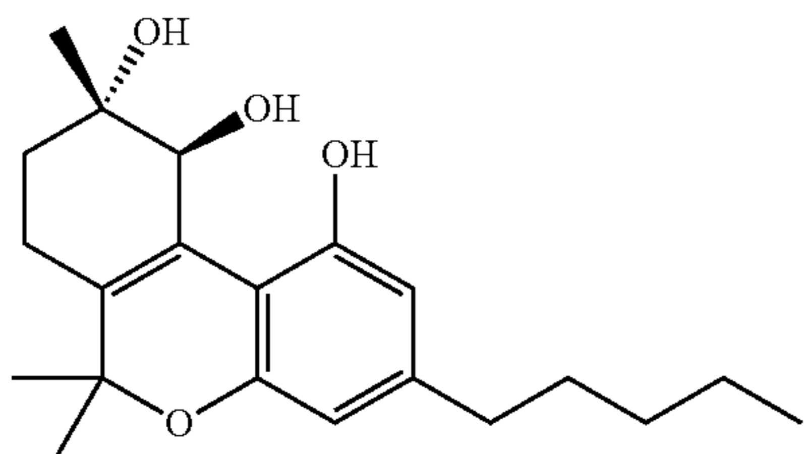
(-)-(9S, 10S)-trans-cannabitrinol [(-)-trans-CBT]
