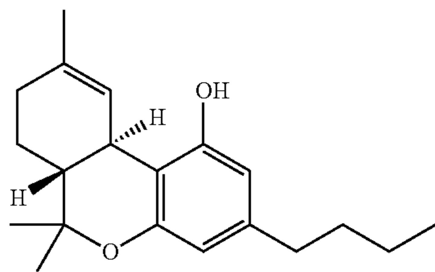
\Delta^9 -tetrahydrocannabinol-C 4 [THC-C 4 ]
