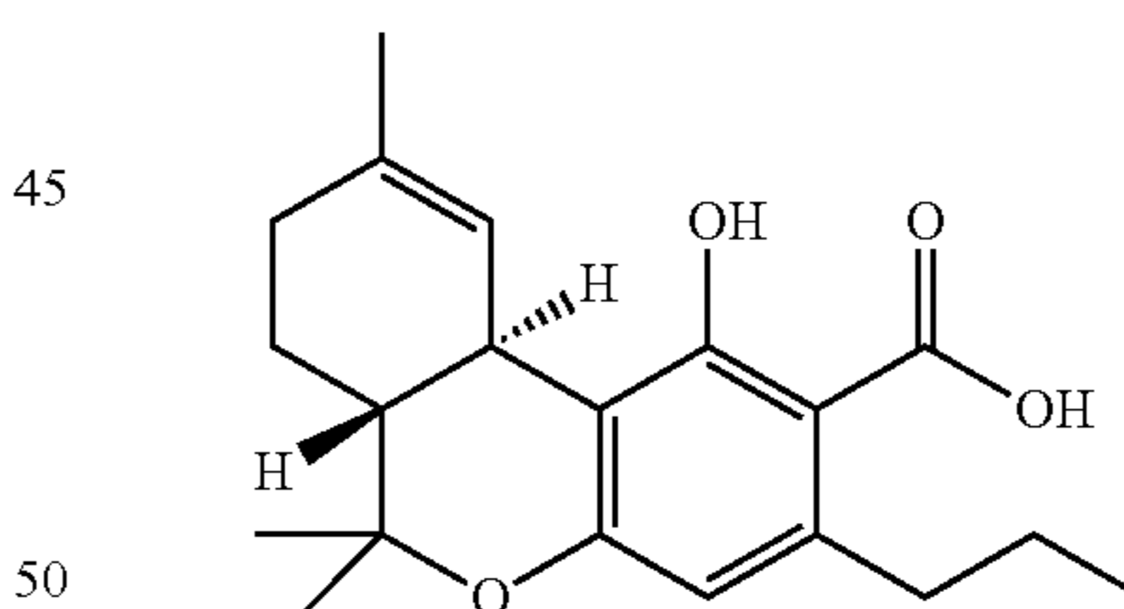
\Delta^9 -tetrahydrocannabivarinic acid A [ \Delta^9 -THCVA A]
