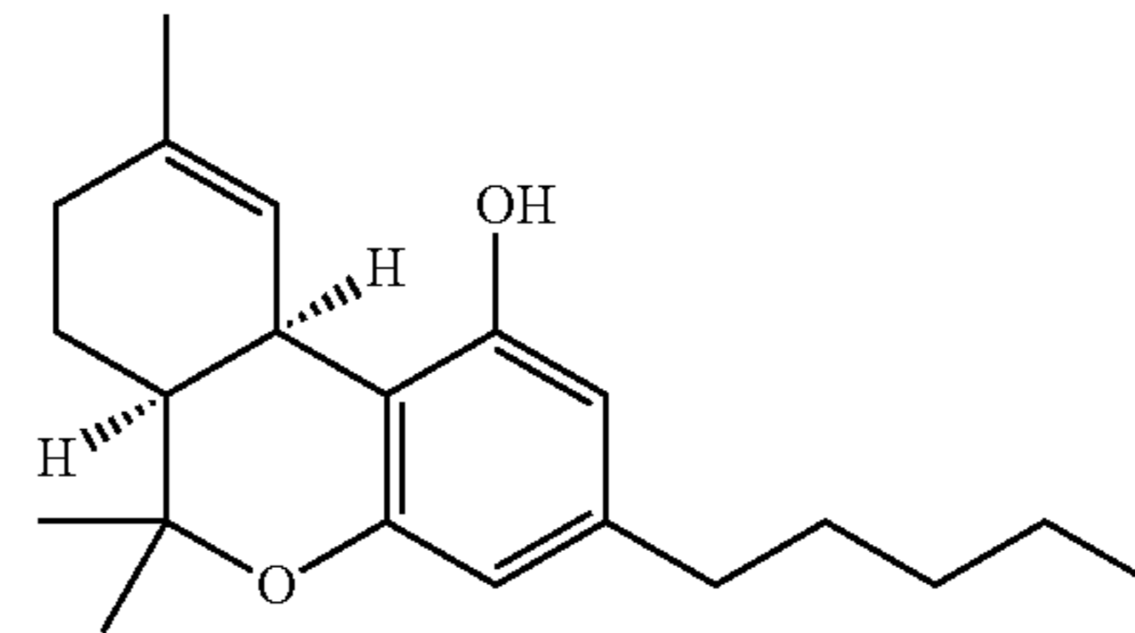
(-)-(6aS, 10aR)- \Delta^9 - tetrahydrocannabinol [cis- \Delta^9 -THC]
