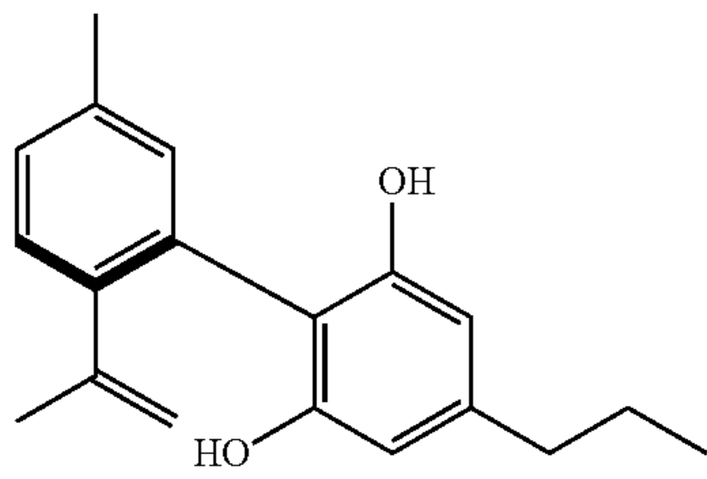
cannabinodivarin [CBND-C 3 ]
