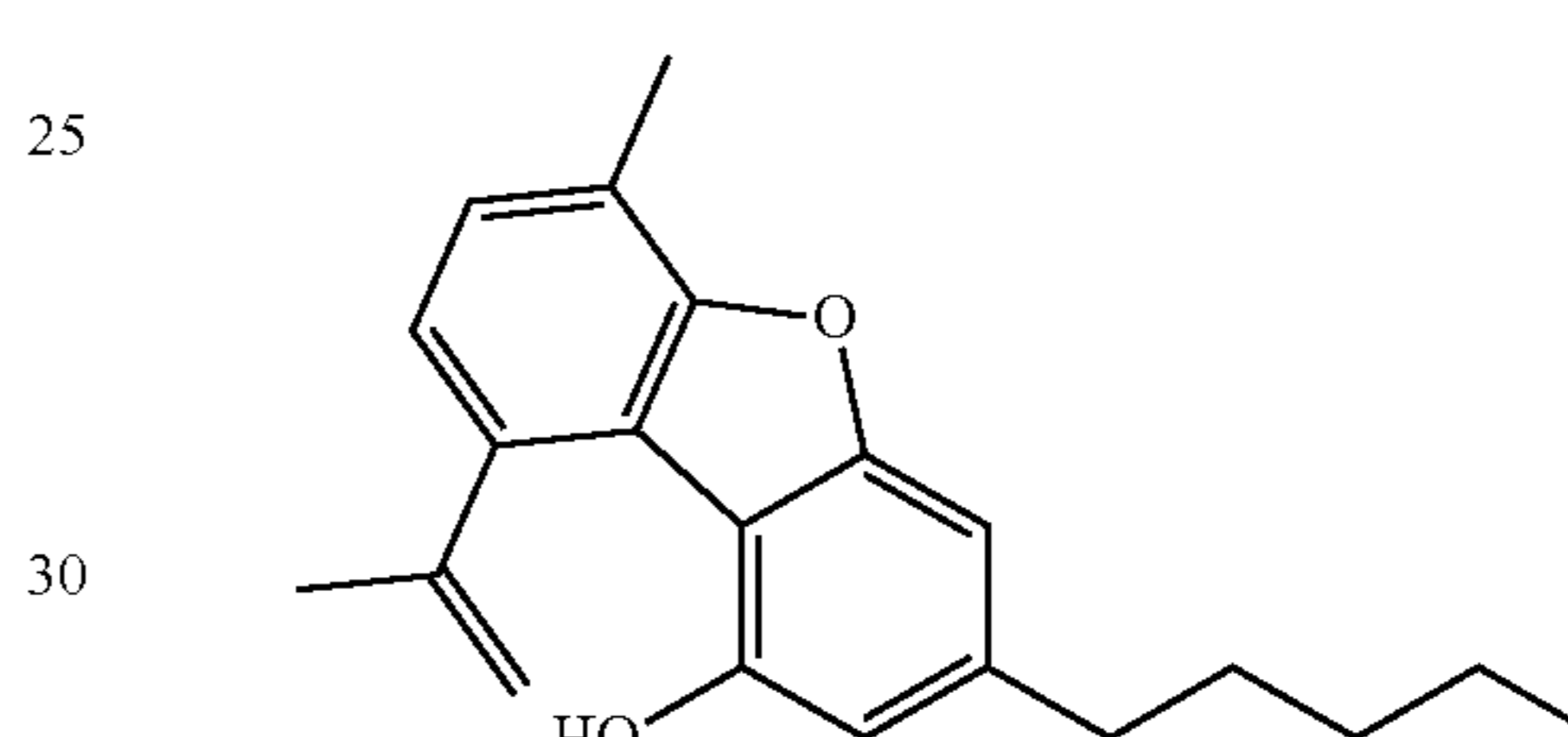
dehydrocannabifuran [DCBF]
