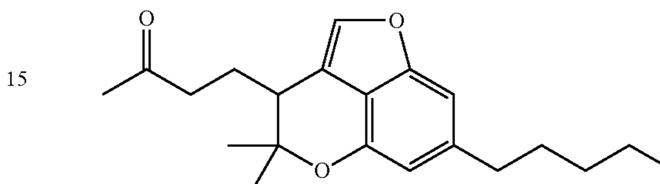
cannabicooumaronone [CBCON]
