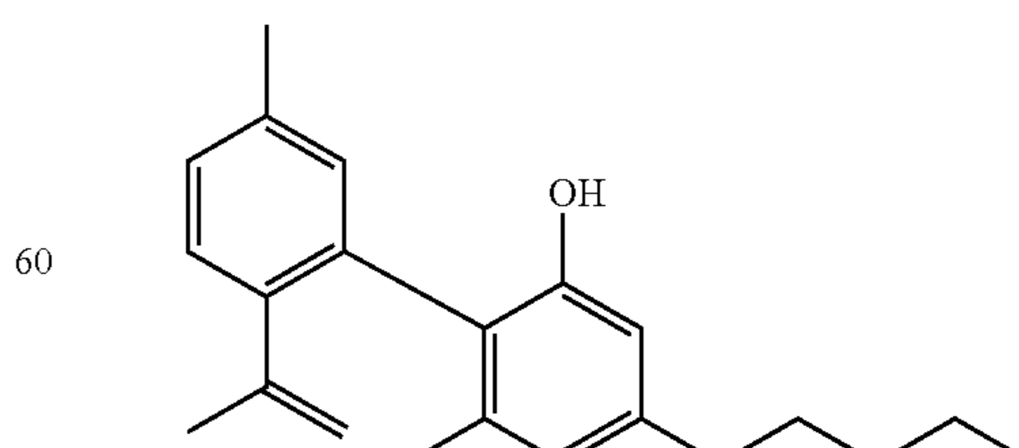
cannabinodiol [CBND]
