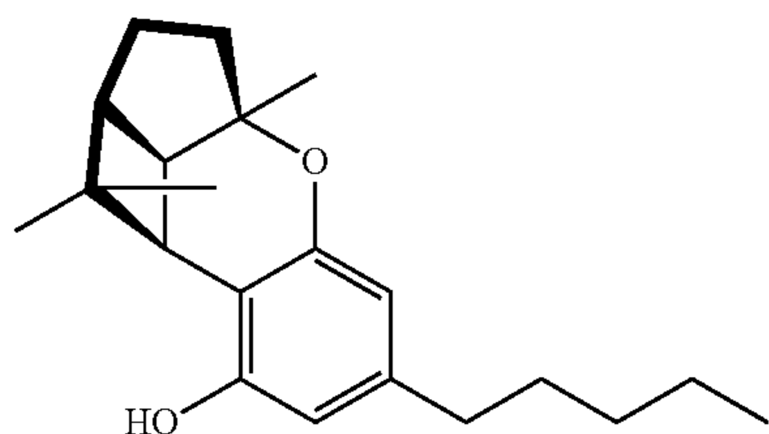
(±)-(1aS, 3aR, 8bR, 8cR)- cannabicyclol [CBL]
