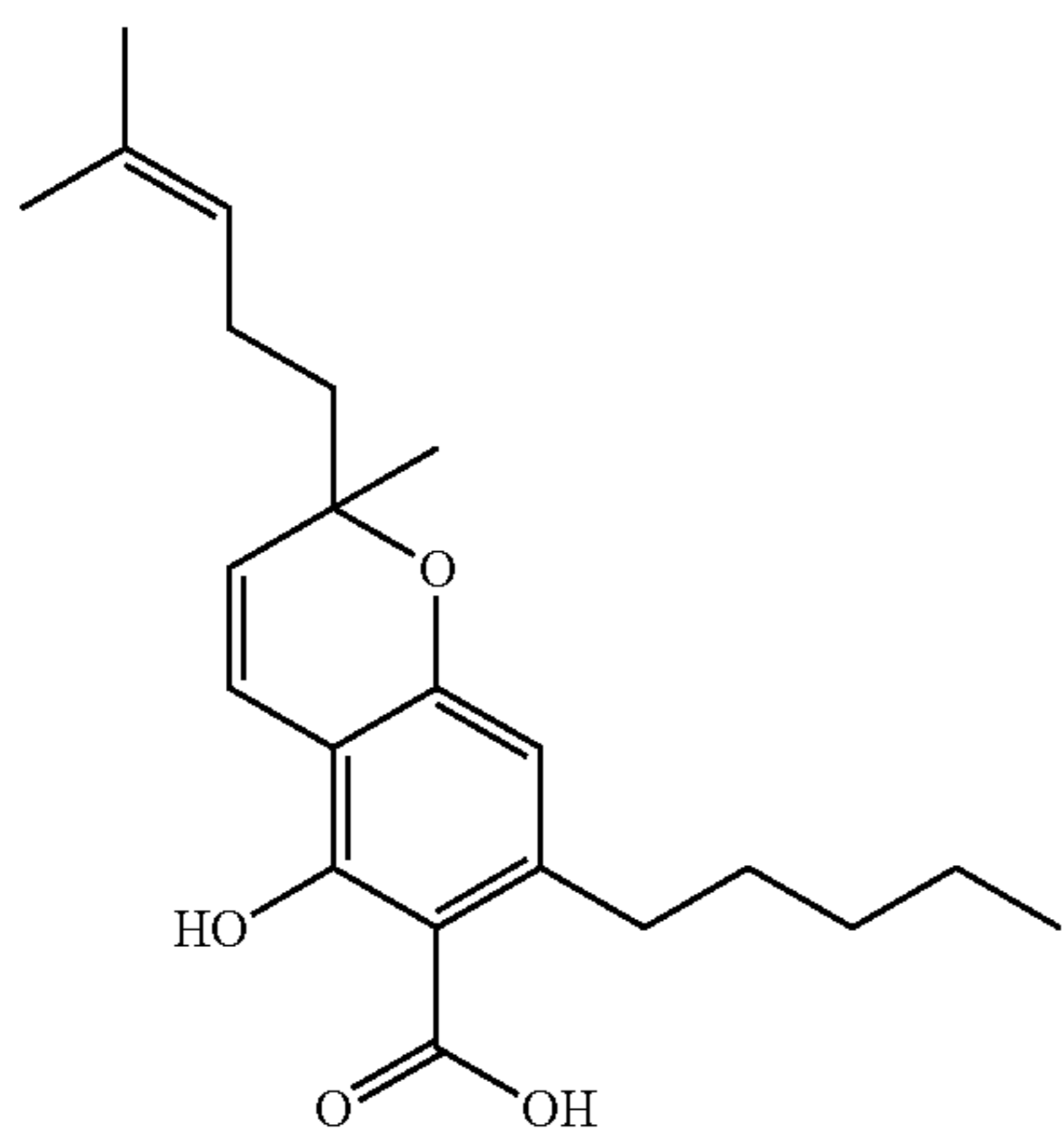
(±)-cannabichromenic acid A [CBCA-C 5 A]
