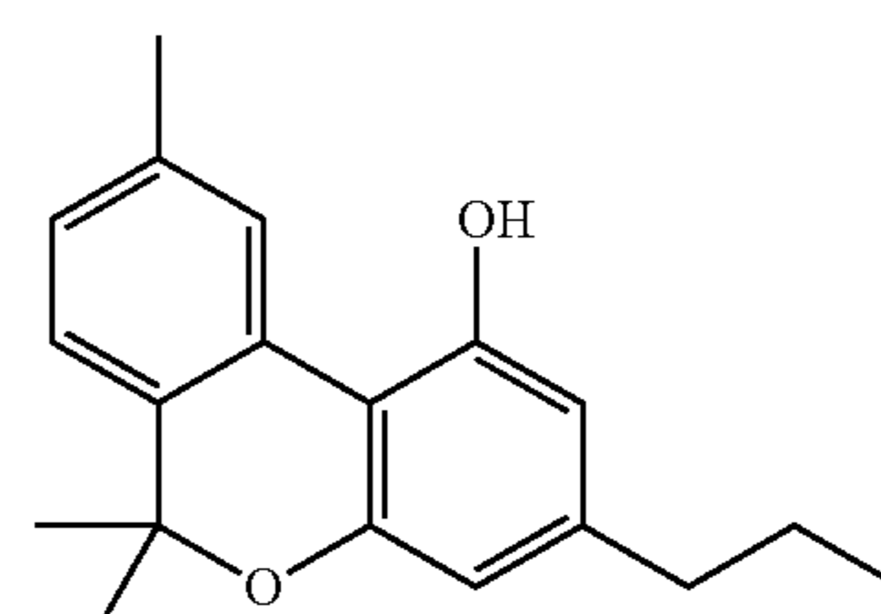
cannabivarin [CBN-C 3 ]
