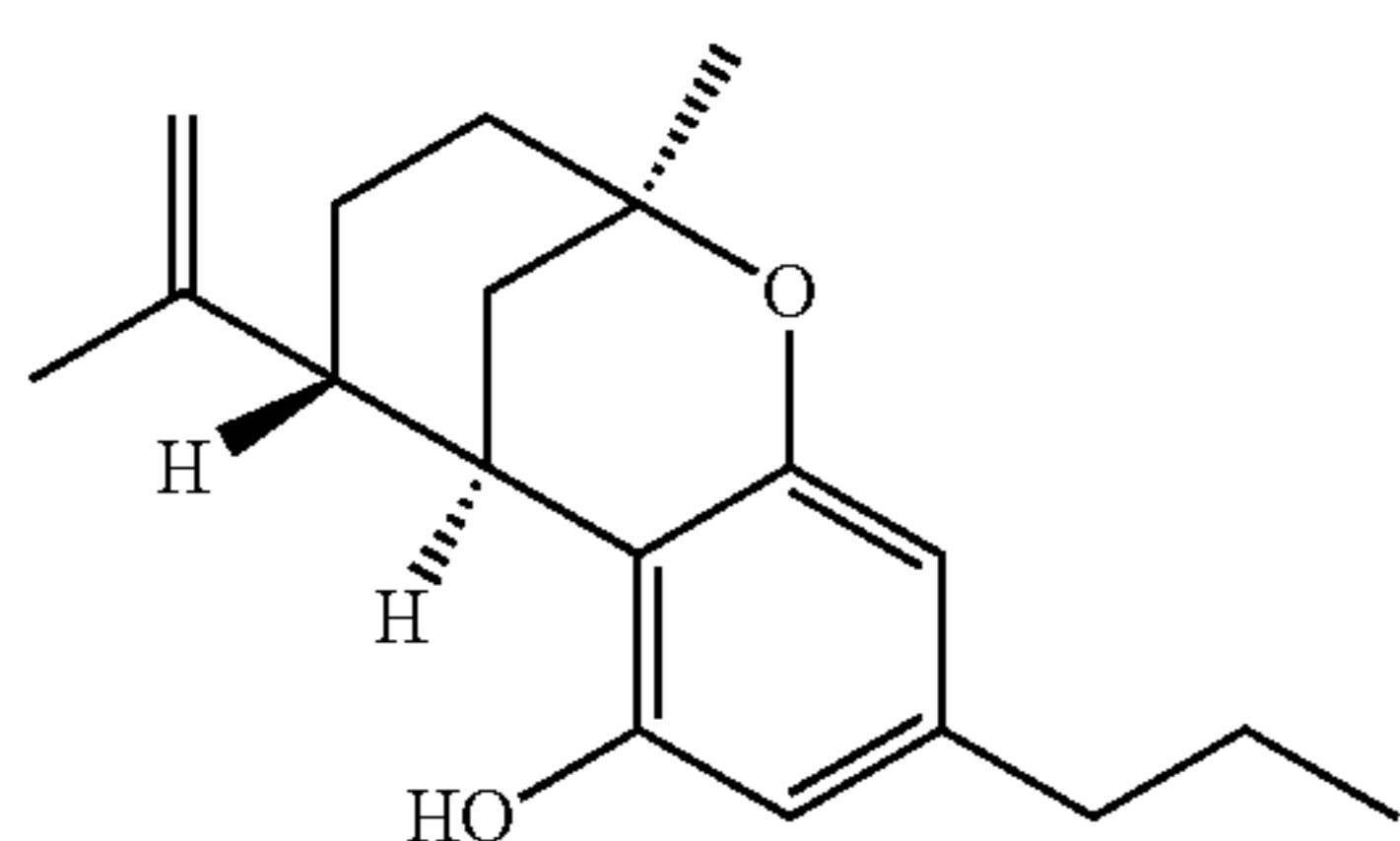
(-)- \Delta^7 -1,2-trans-(1R, 3R, 6R)- isotetrahydrocannabivarin
