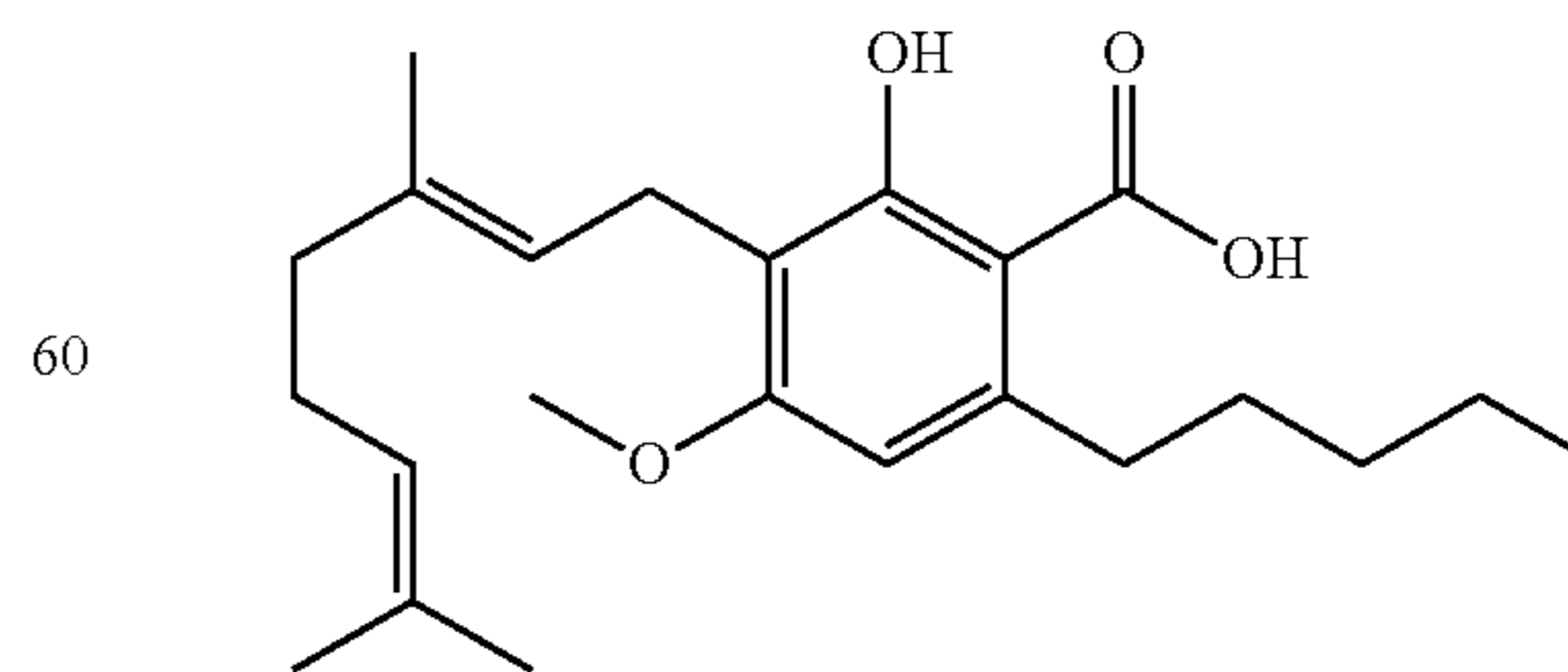
cannabigerolic acid A monomethyl ether [(E)-CBGAM-C 5 A]
