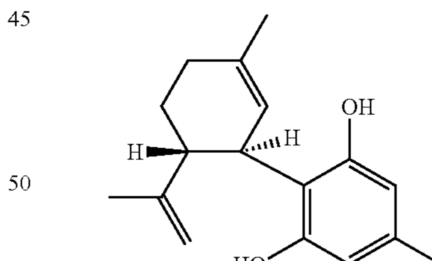
cannabidiolcol [CBD-D 1 ]
