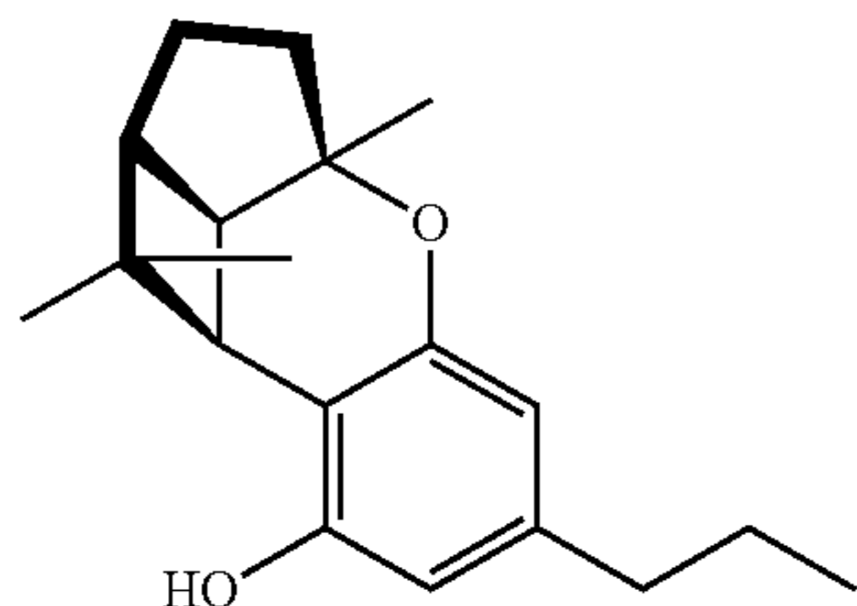
(±)-(1aS, 3aR, 8bR, 8cR)- cannabicyclovarin [CBLV]
