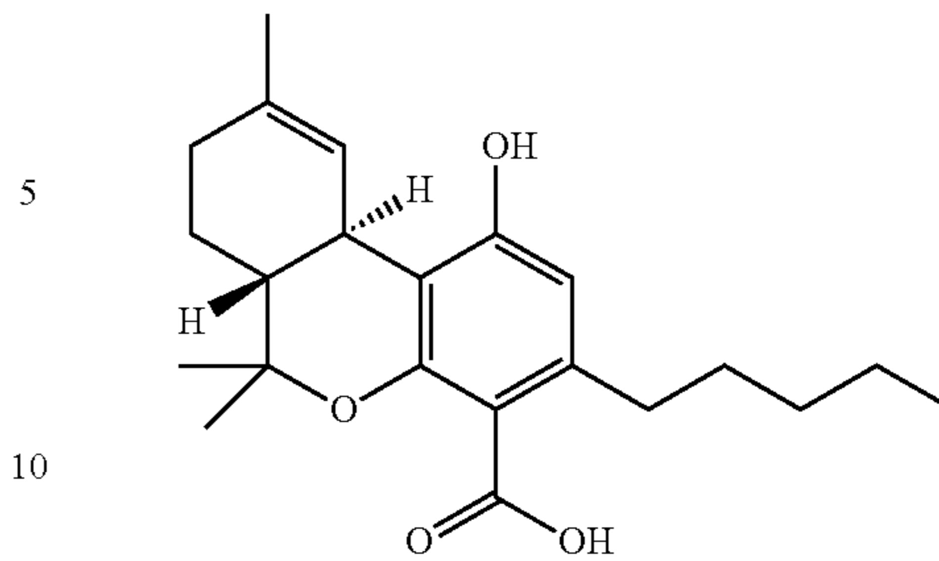
\Delta^9 -tetrahydrocannabinolic acid B [ \Delta^9 -THCA B]
