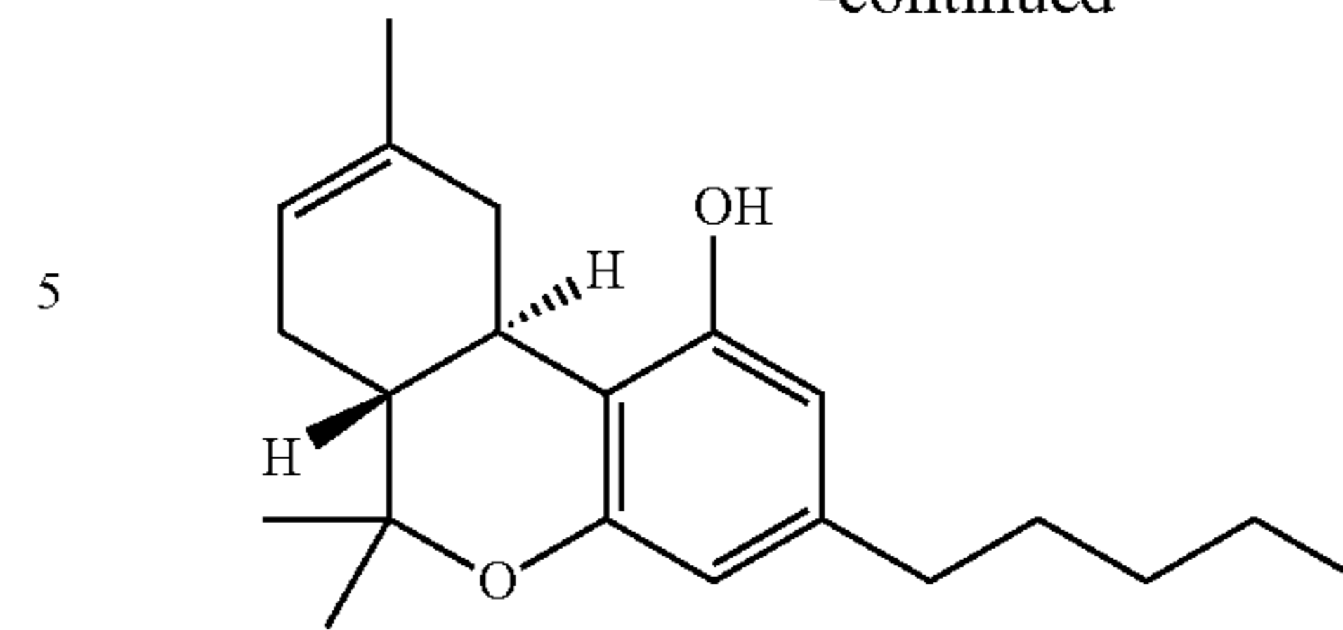
(-)- \Delta^8 -trans-(6aR, 10aR)- \Delta^8 - \Delta^8 - tetrahydrocannabinol [ \Delta^8 -THC]
