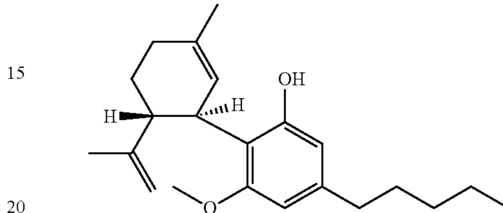
cannabidiol monomethyl ether [CBDM]
