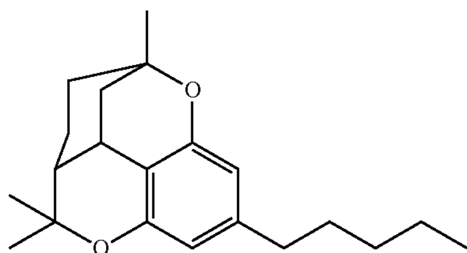
cannabicitran [CBT]
