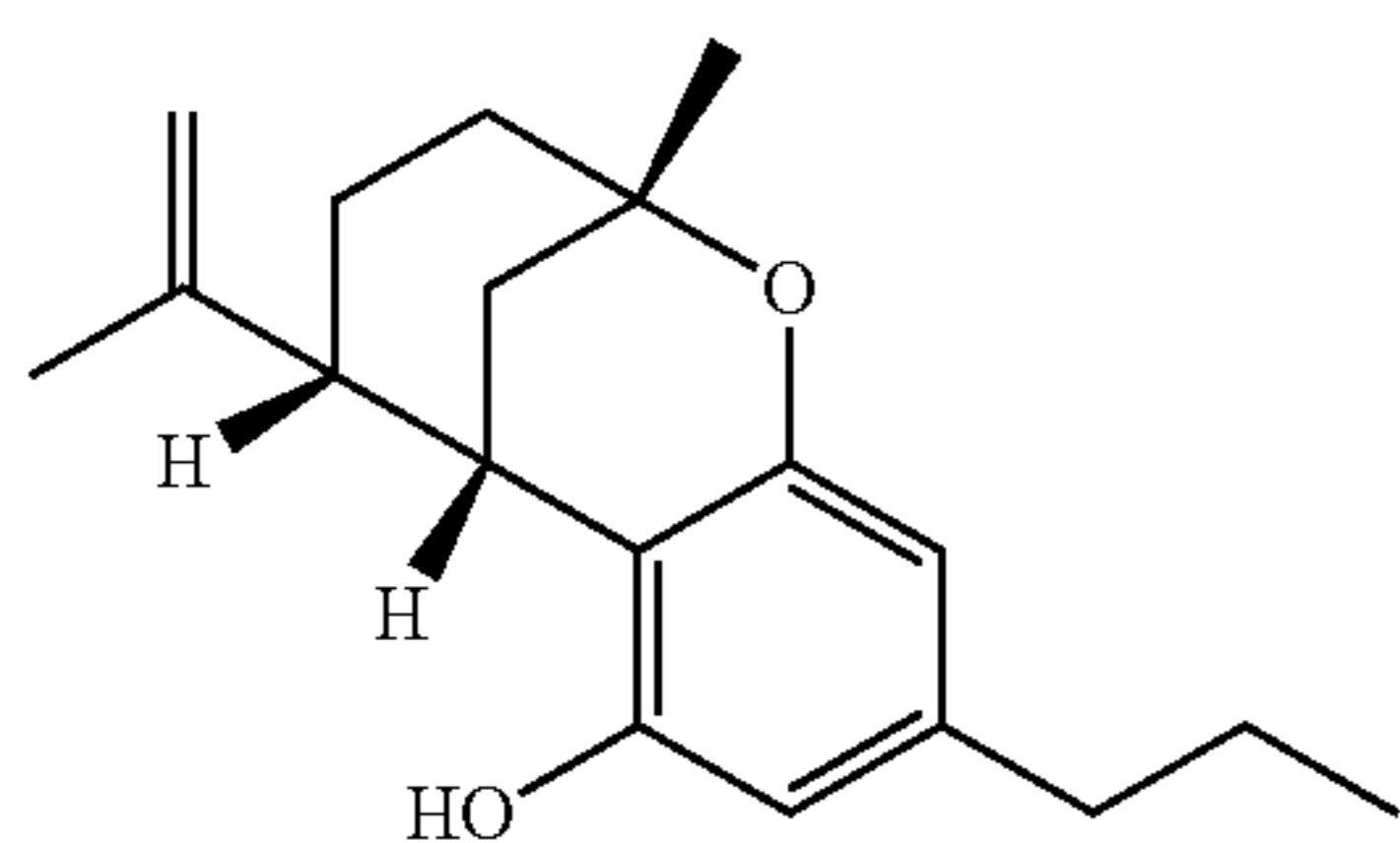
(±)- \Delta^7 -1,2-cis-(1S, 3S, 6R)- isotetrahydrocannabivarin
