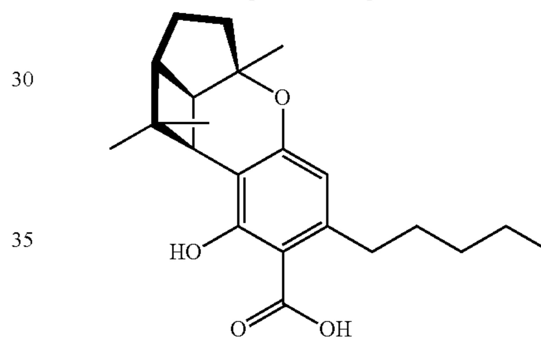
(±)-(1aS, 3aR, 8bR, 8cR)-cannabicyclolic [CBLA A]
