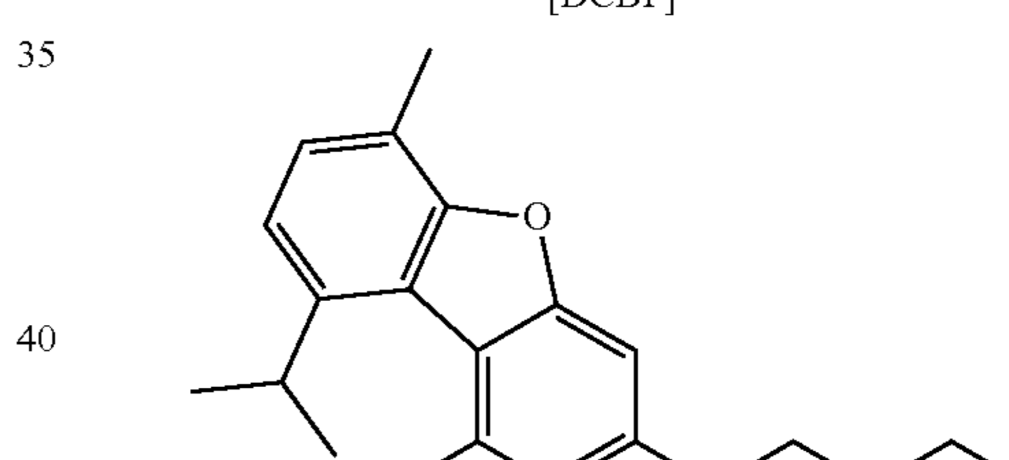
cannabifuran [CBF]
