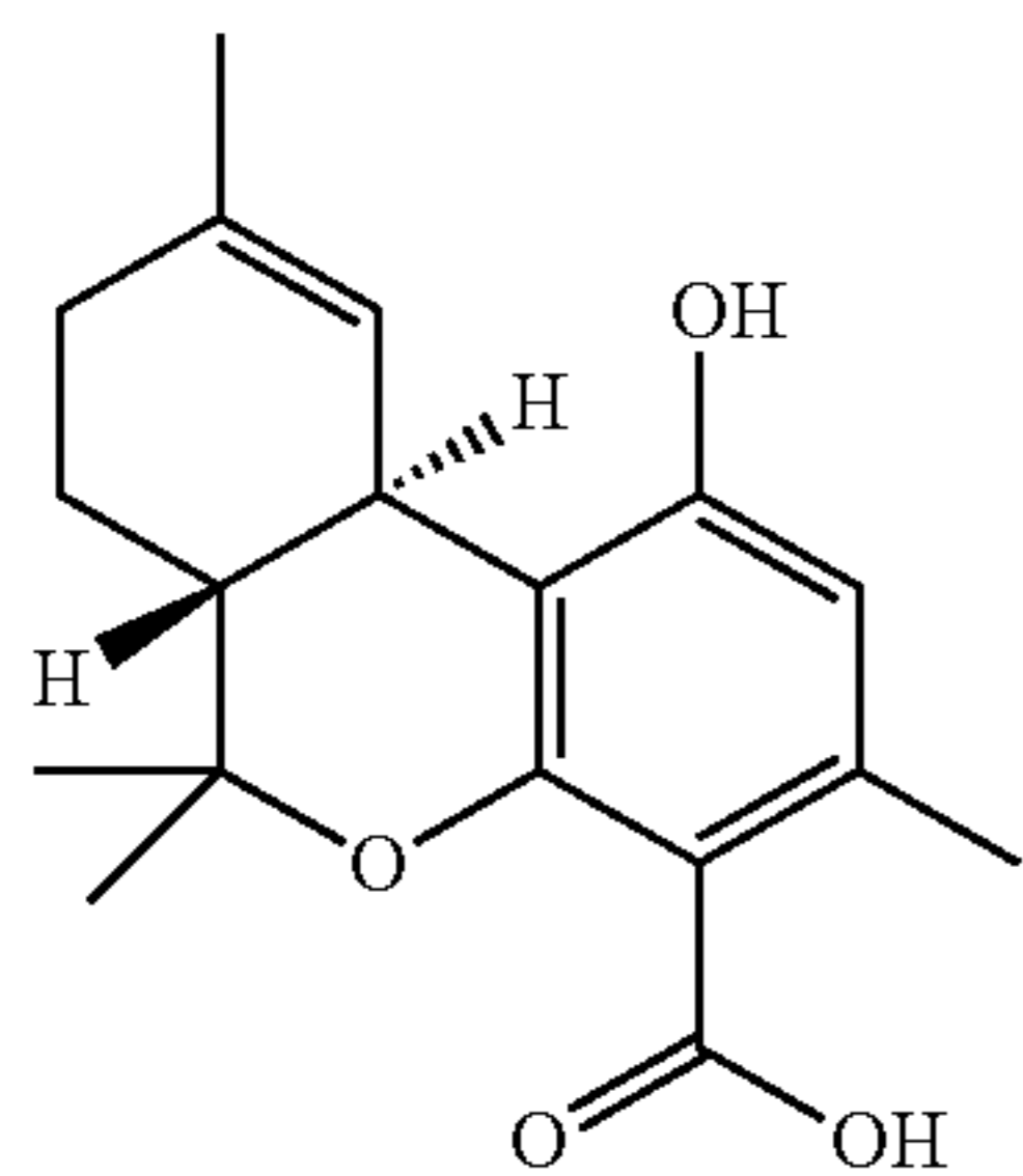
\Delta^9 -tetrahydrocannabinolic acid B [ \Delta^9 -THCOA B]
