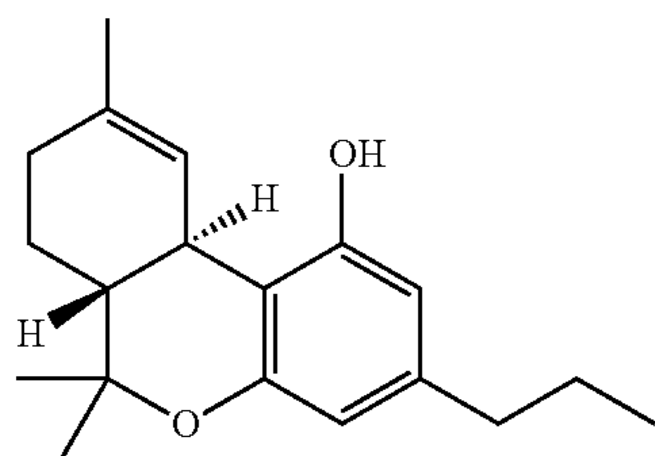
\Delta^9 -tetrahydrocannabivarin [THCV]
