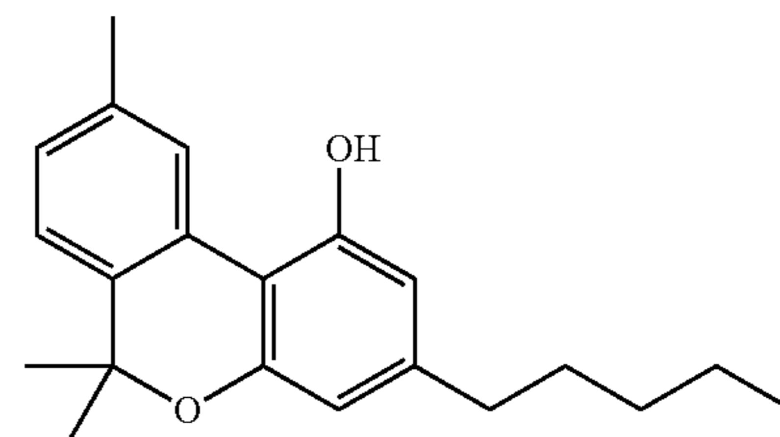
cannabinol [CBN]
