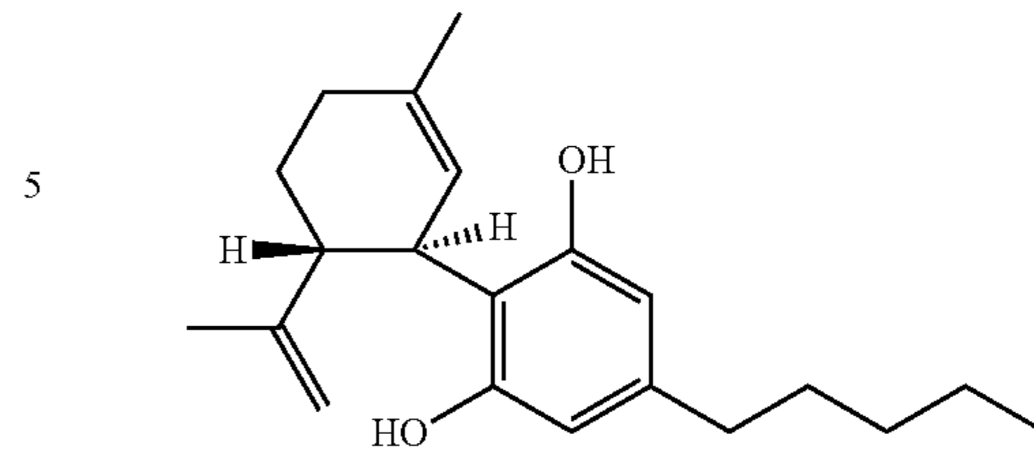
(-)-cannabidiol [CBD]
