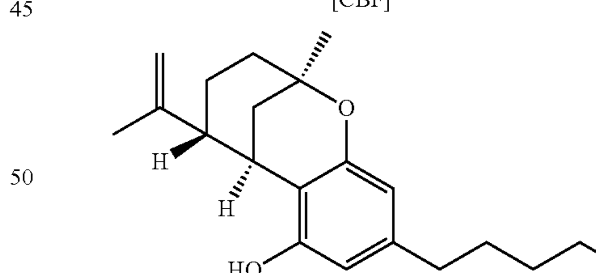
(-)-Δ 7 -trans-(1R, 3R, 6R)- isotetrahydrocannabinol
