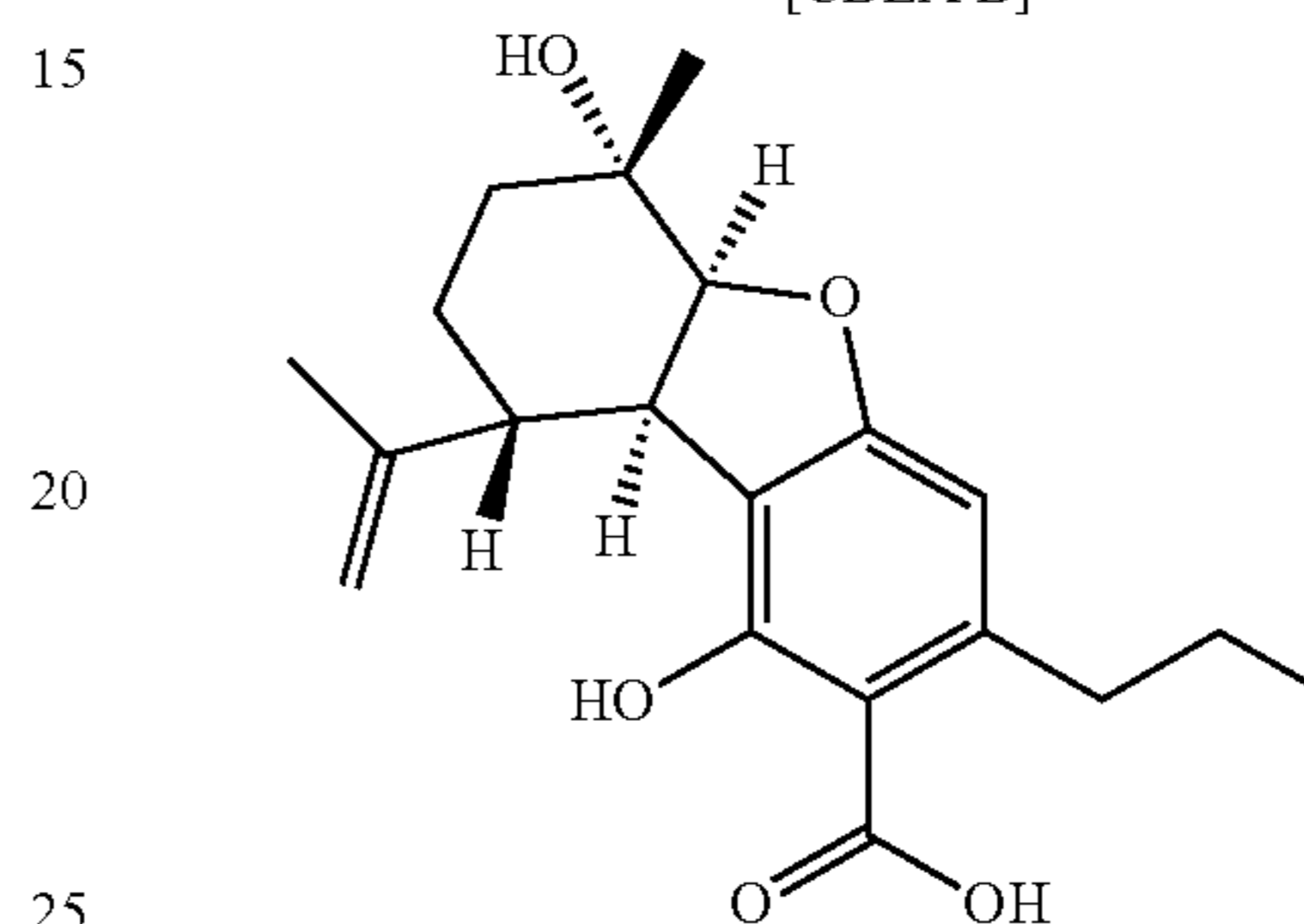
(5aS, 6S, 9R, 9aR)-C 3 -cannabielsoic acid B [CBEA-C 3 B]
