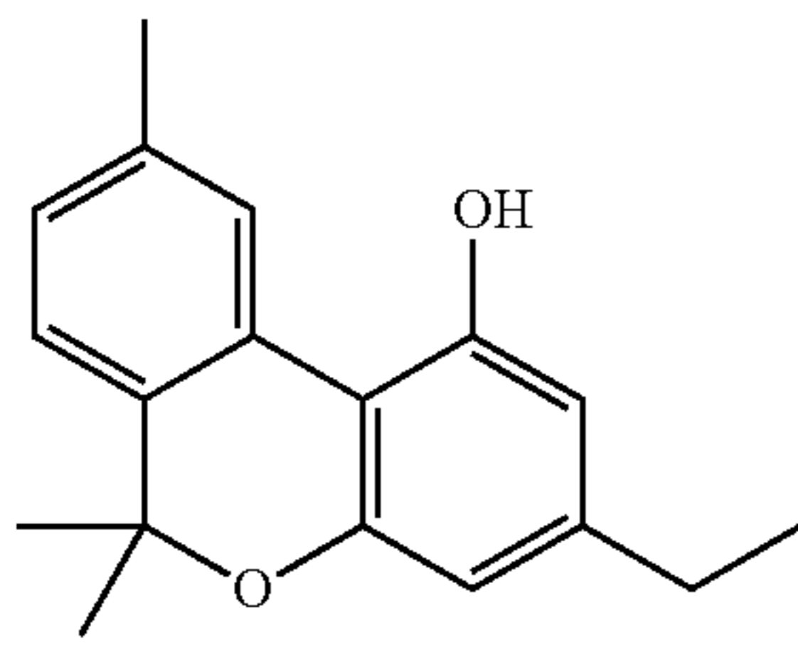
cannabinol-C 2 [CBN-C 2 ]
