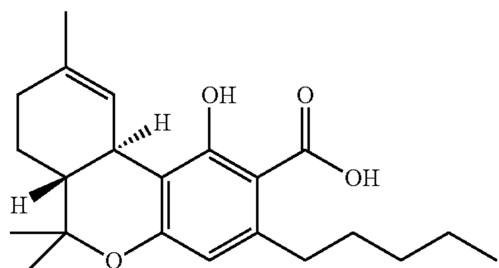
\Delta^9 -tetrahydrocannabinolic acid A [ \Delta^9 -THCA A]
