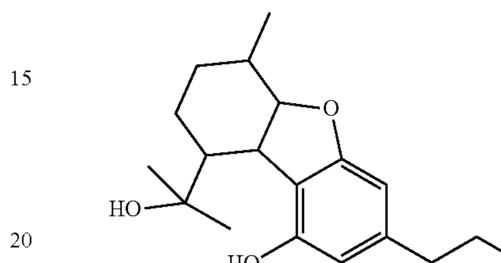
cannabiglendo-C 3 [OH-iso-HHCV-C 3 ]
