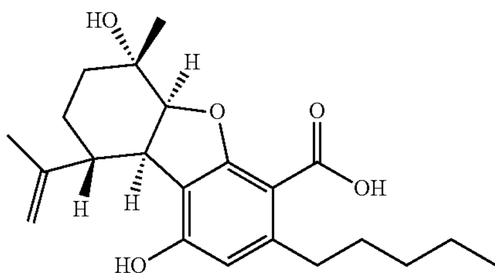
(5aS, 6S, 9R, 9aR)-cannabielsoic acid A [CBEA A]
