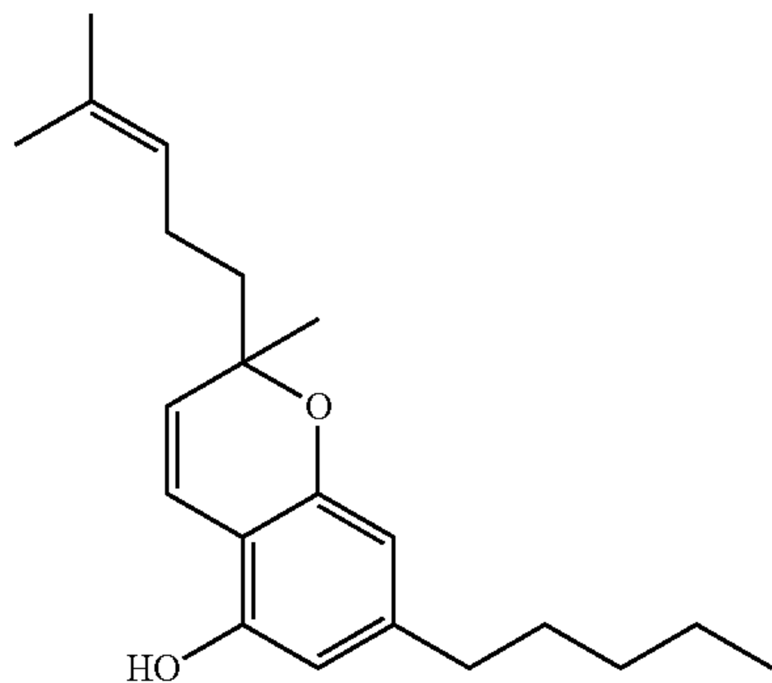
(±)-cannabichromene [CBC]
