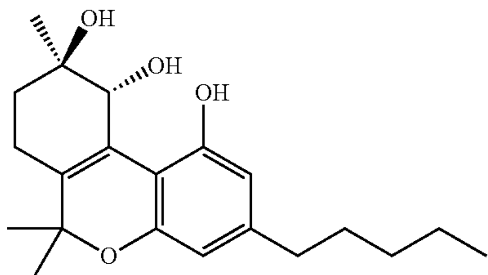
(-)-(9R, 10R)-trans-cannabitrinol [(-)-trans-CBT]
