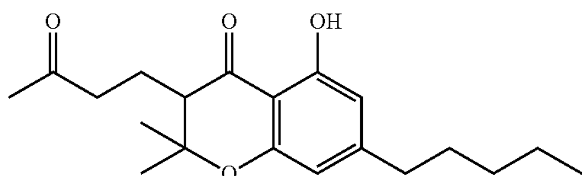
cannabichromanone [CBCN]
