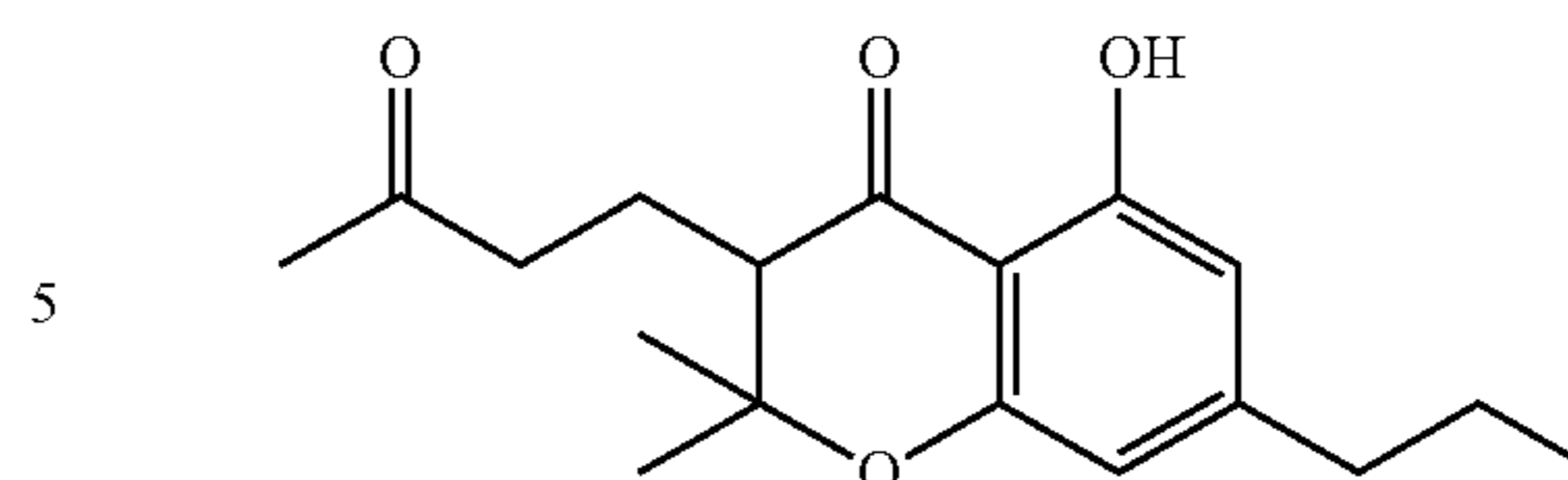
cannabichromanone-C 3 [CBCN-C 3 ]
