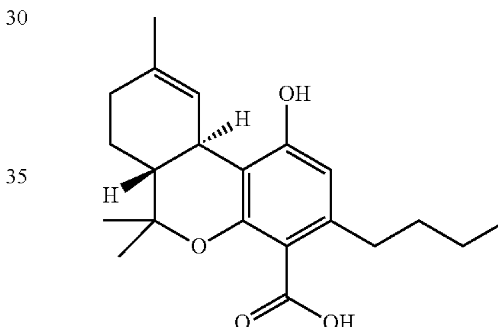
\Delta^9 -tetrahydrocannabinolic acid-C 4 B [ \Delta^9 -THCA-C 4 B]
