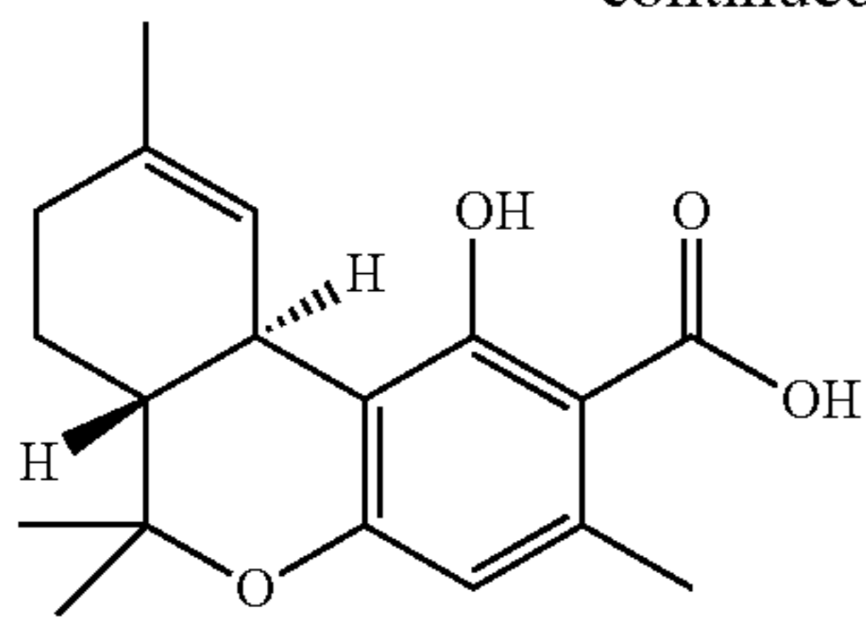
\Delta^9 -tetrahydrocannabinolic acid A [ \Delta^9 -THCOA A]
