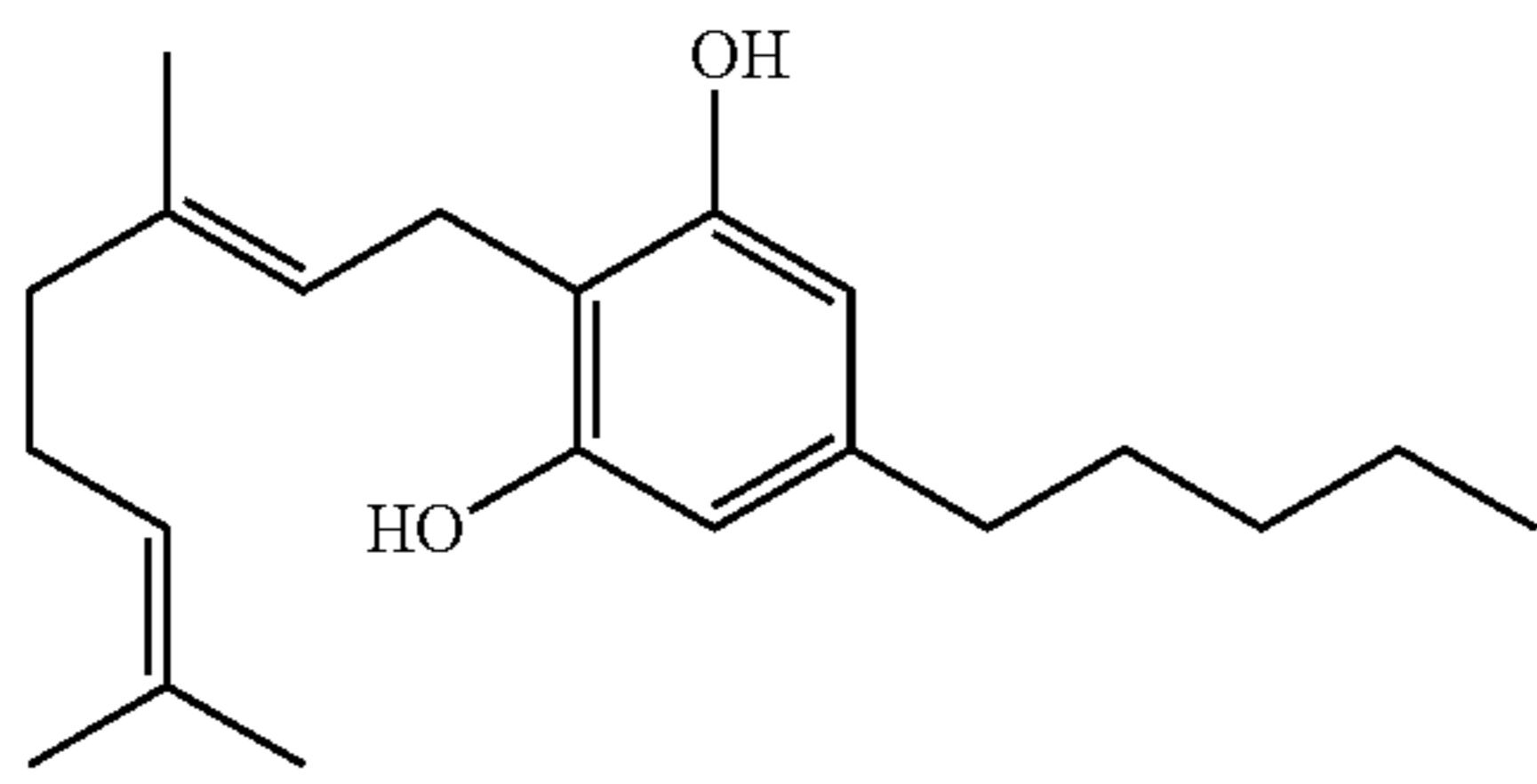
cannabigerol [CBG]
