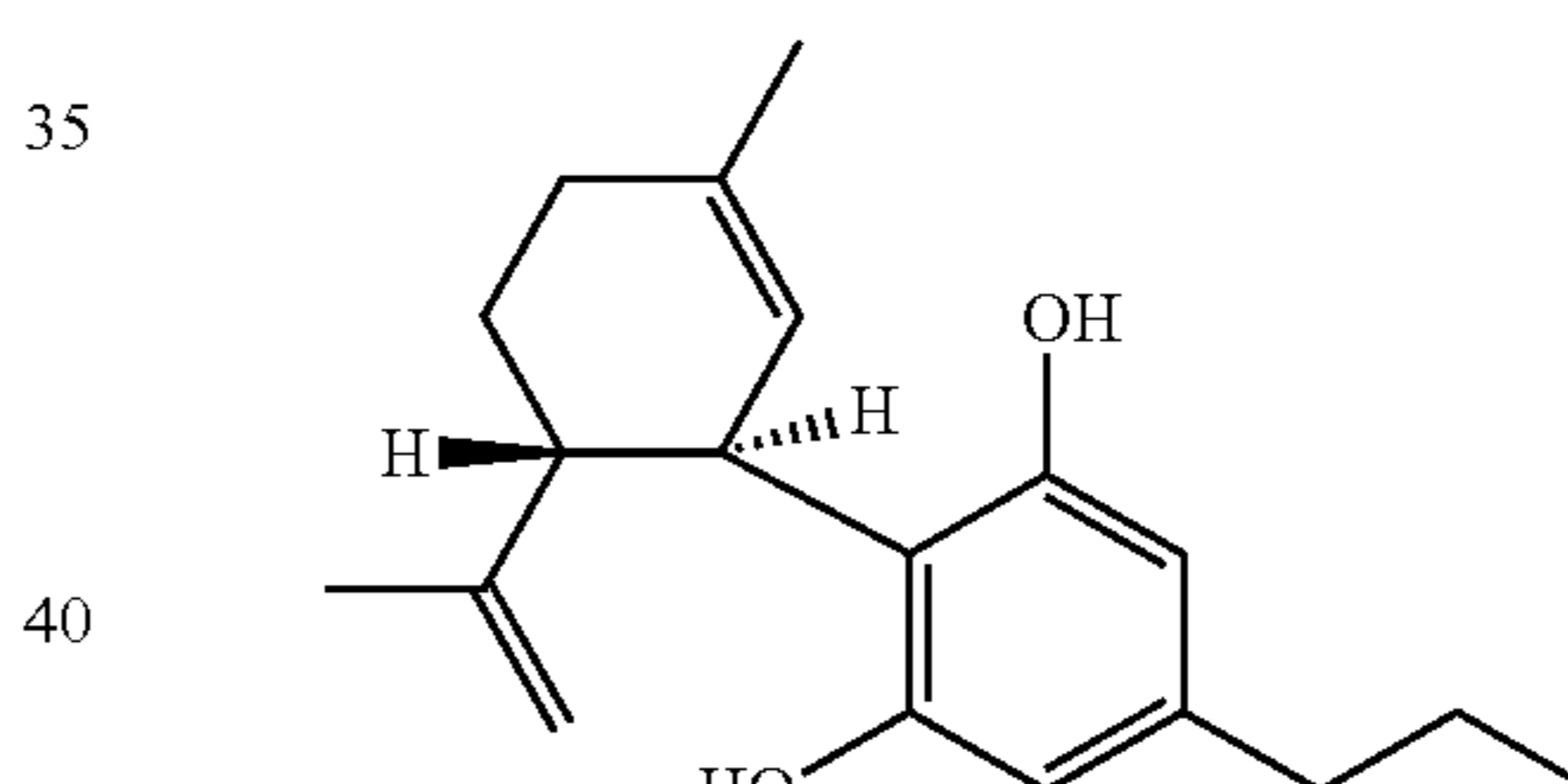
(-)-cannabidivarin [CBDV]
