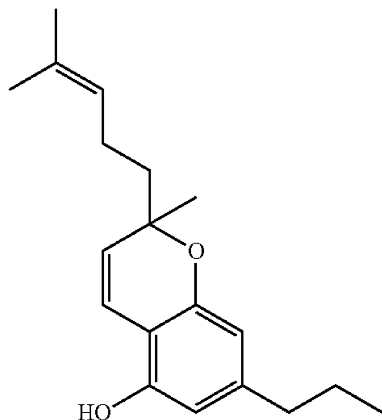
(±)-cannabichromevarin [CBCV]
