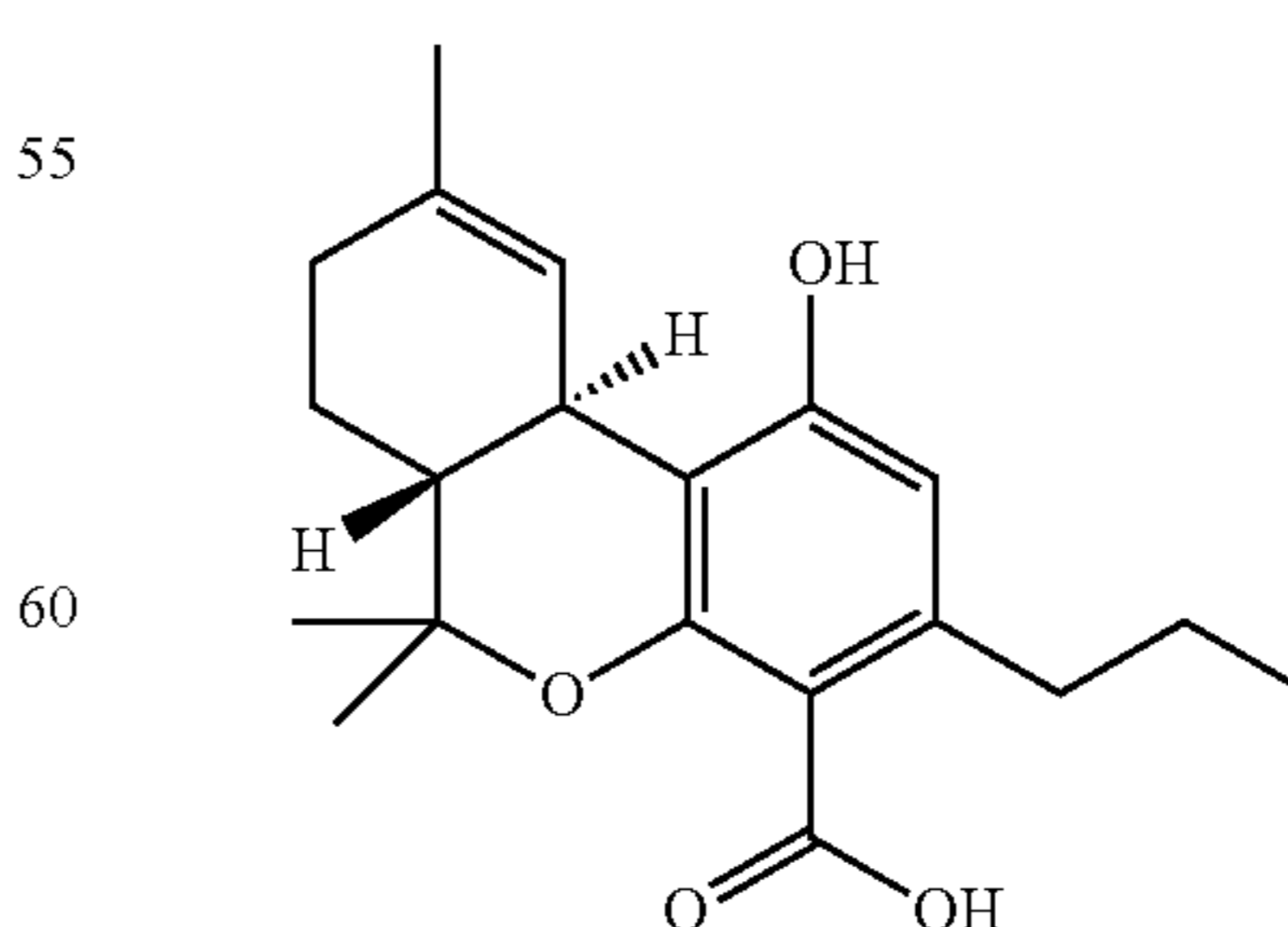
\Delta^9 -tetrahydrocannabivarinic acid B [ \Delta^9 -THCVA B]
