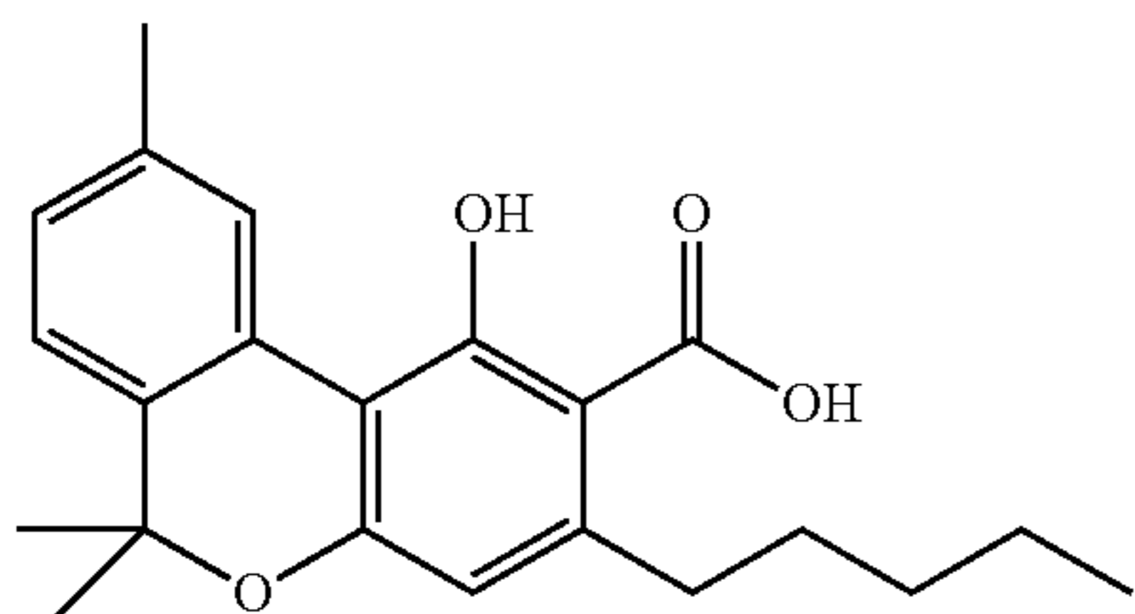
cannabinolic acid A [CBNA A]
