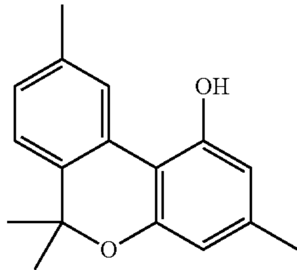
cannabiorcol [CBN-C 1 ]
