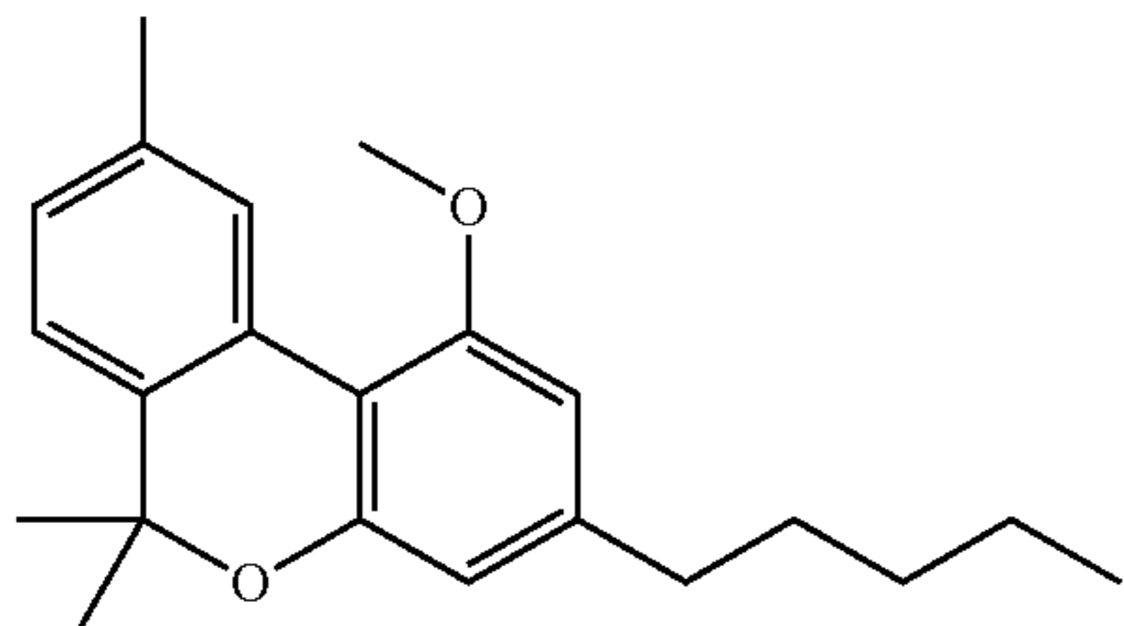
cannabinol methyl ether [CBNM]
