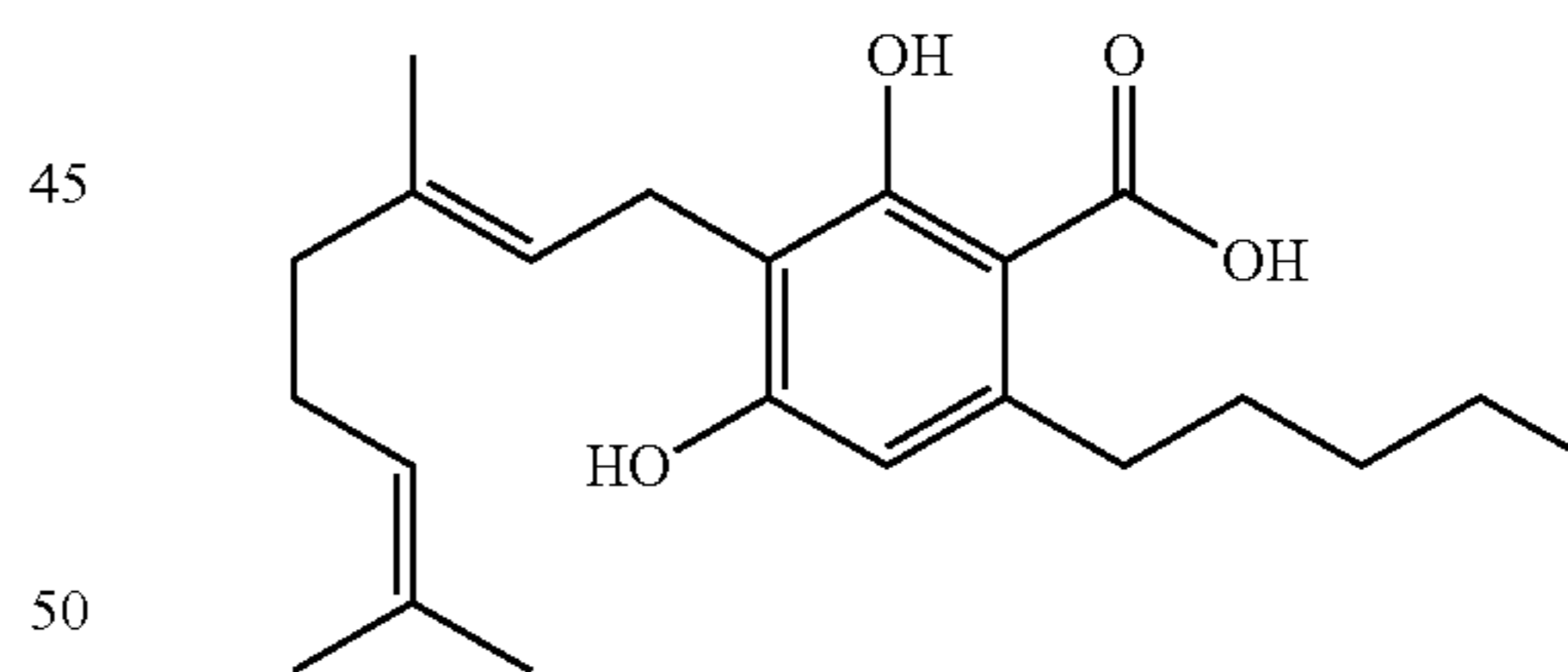
cannabigerolic acid A [(E)-CBGA-C 5 A]
