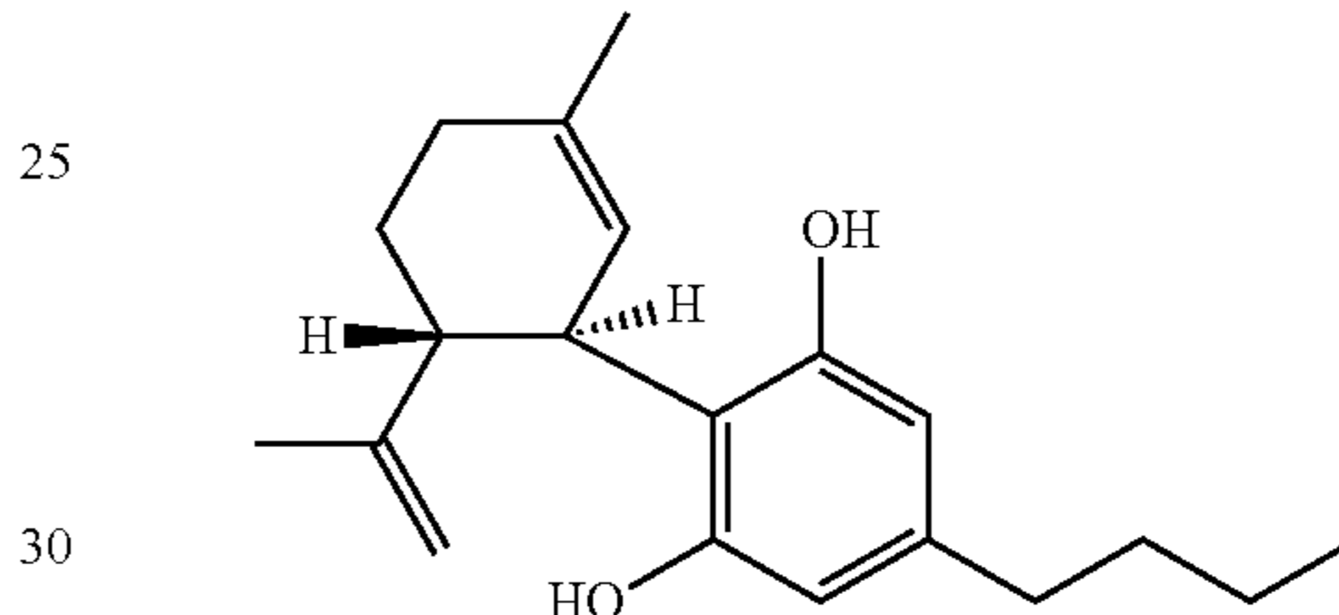
cannabidiol-C 4 [CBD-C 4 ]
