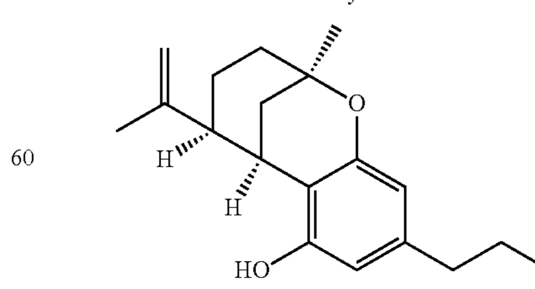
(±)-Δ 7 -1,2-cis-(1R, 3R, 6S)- isotetrahydrocannabivarin
