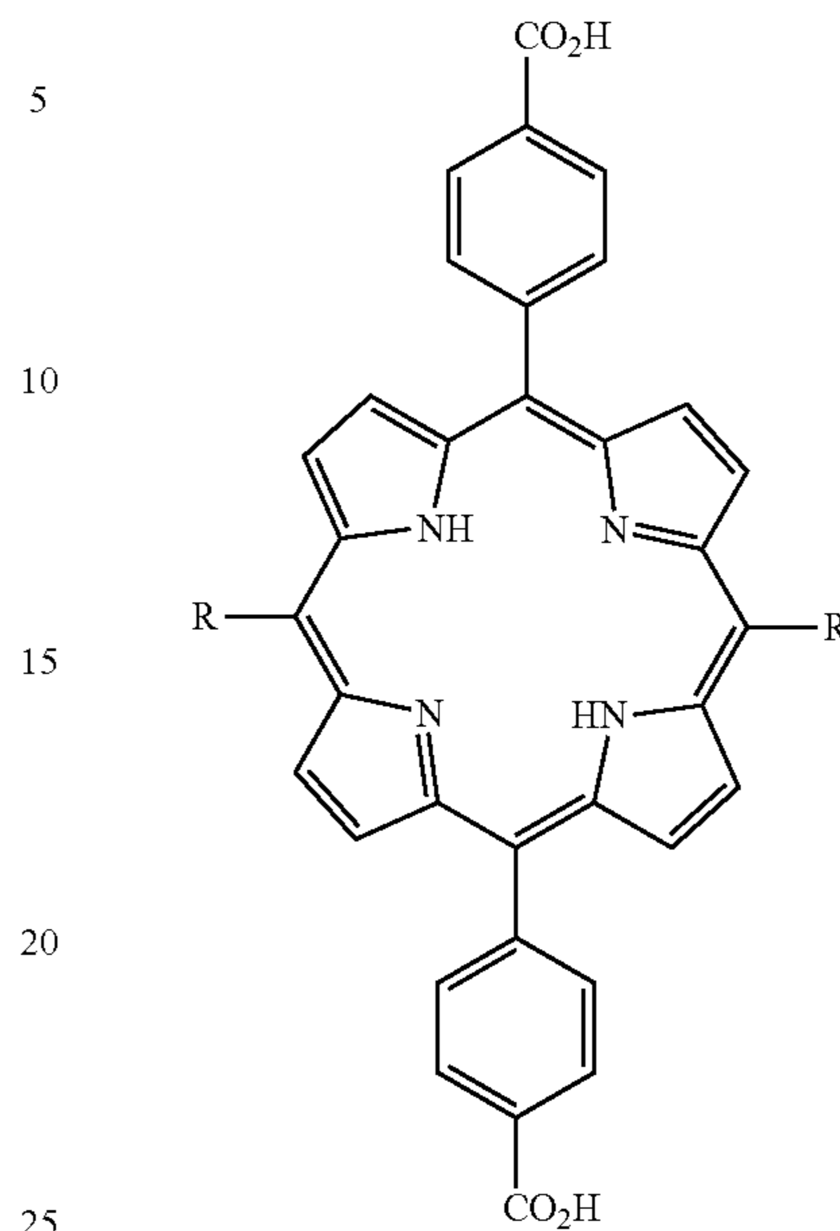
Scheme 1. Exemplary DBP, DBC, and DBCC ligands.
