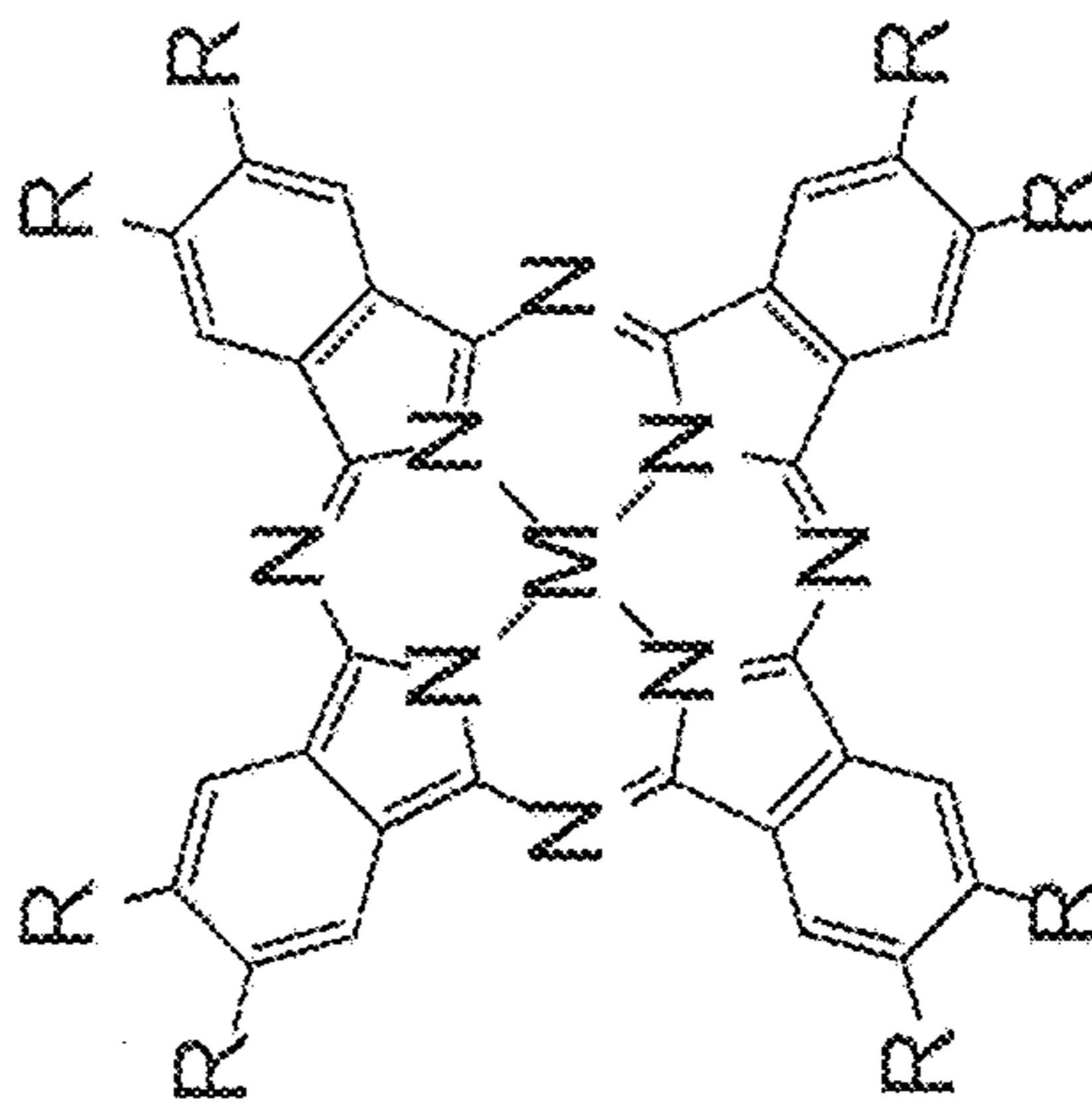
5,10,15,20-tetra(p-pyridyl)porphyrin
