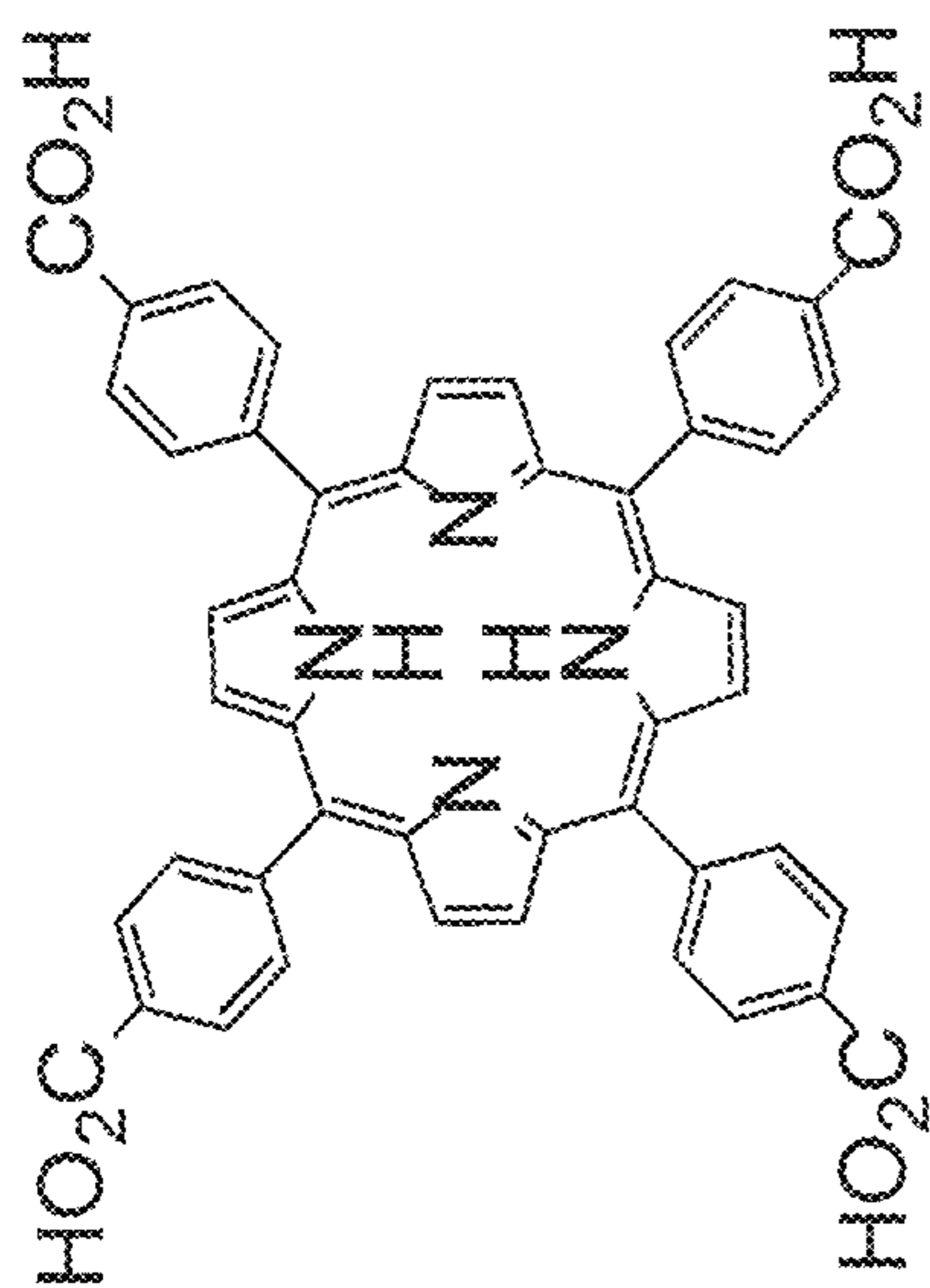
5,10,15,20-tetra(p-carboxylphenyl)porphyrin
