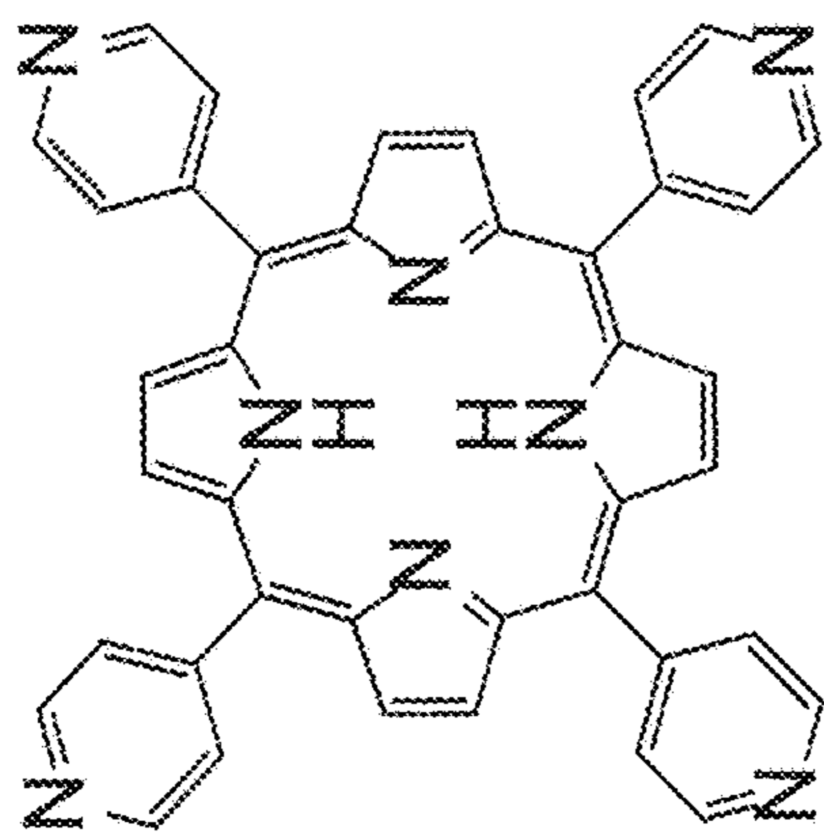
5,10,15,20-tetra(p-pyridyl)porphyrin
