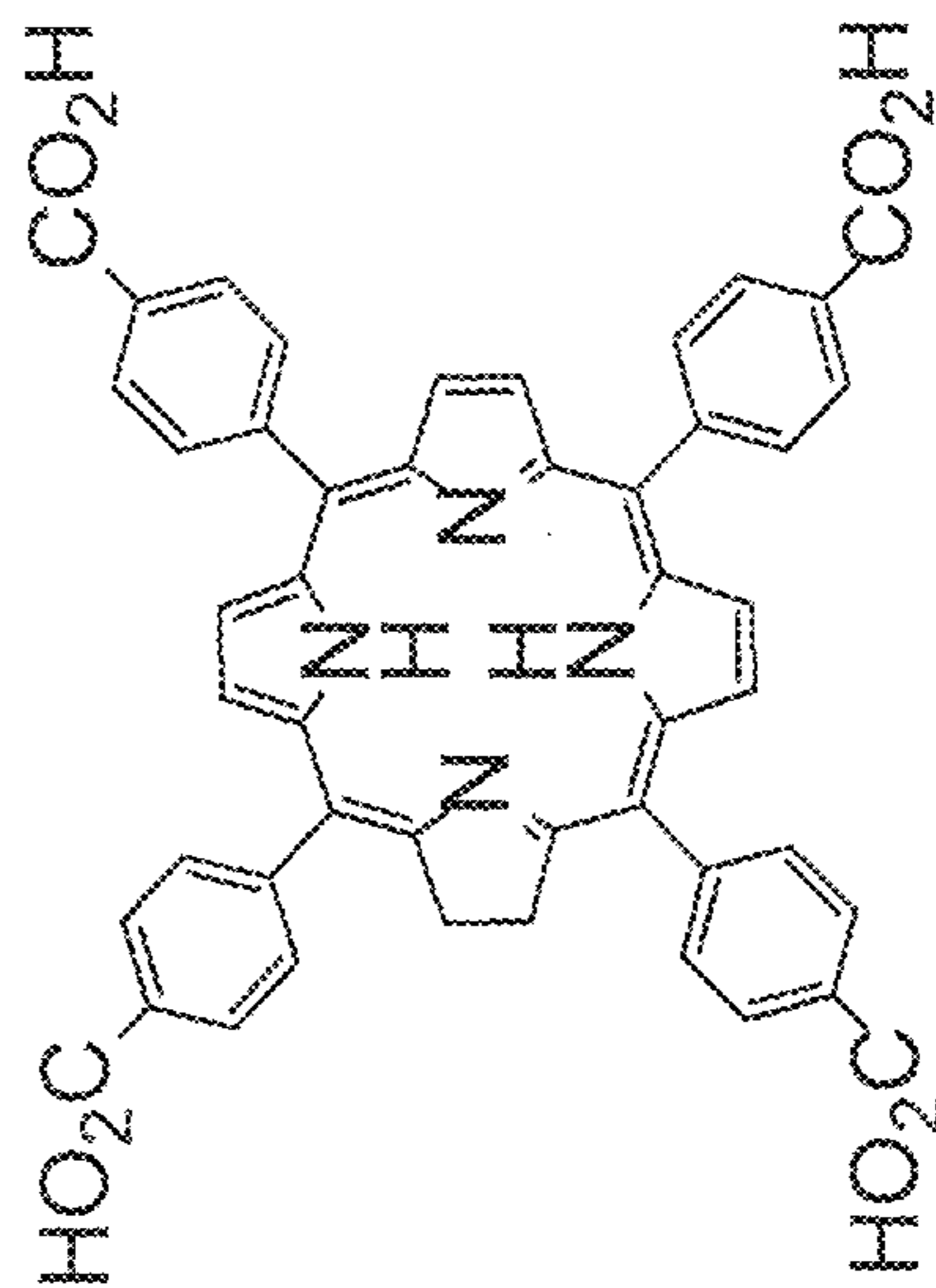
5,10,15,20-tetra(3',5'-dicarboxylphenyl)porphyrin
