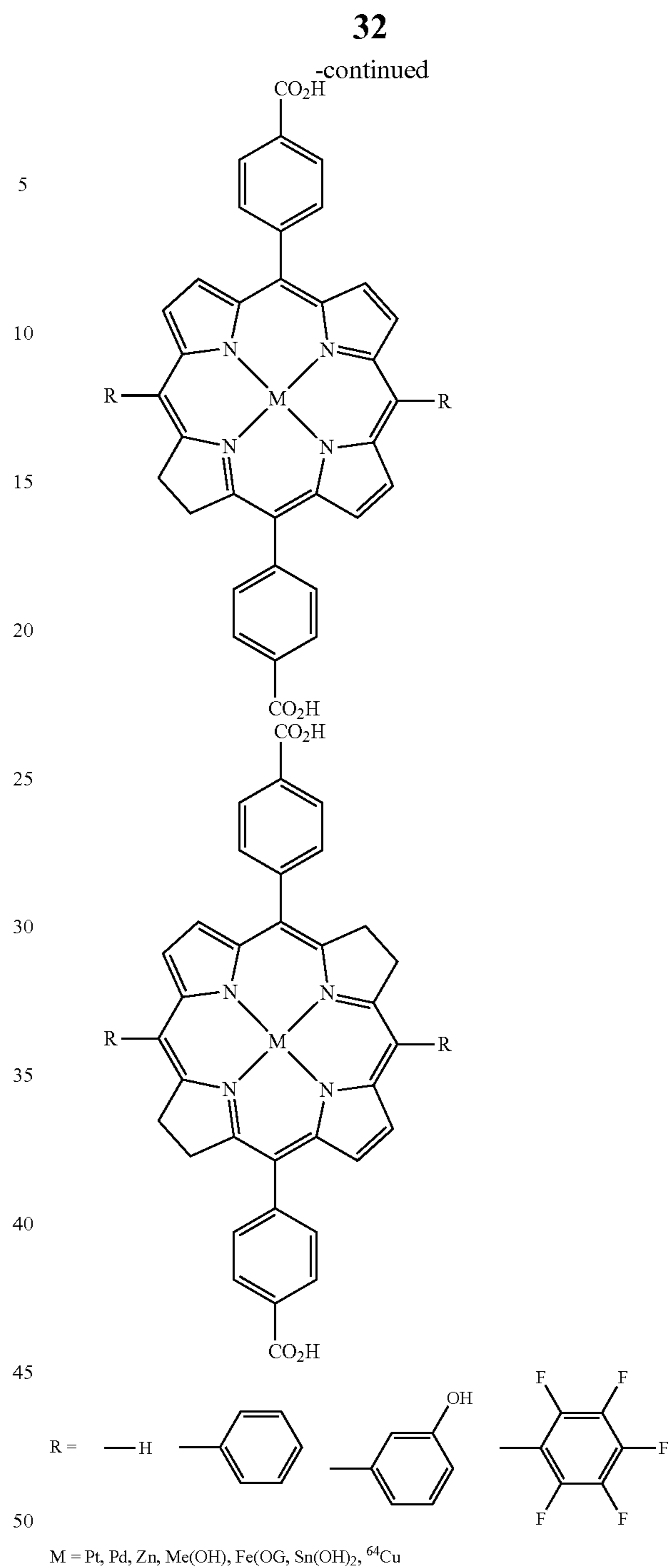
Scheme 2. Exemplary Metal Complex DBP, DBC, and DBCC ligands.
