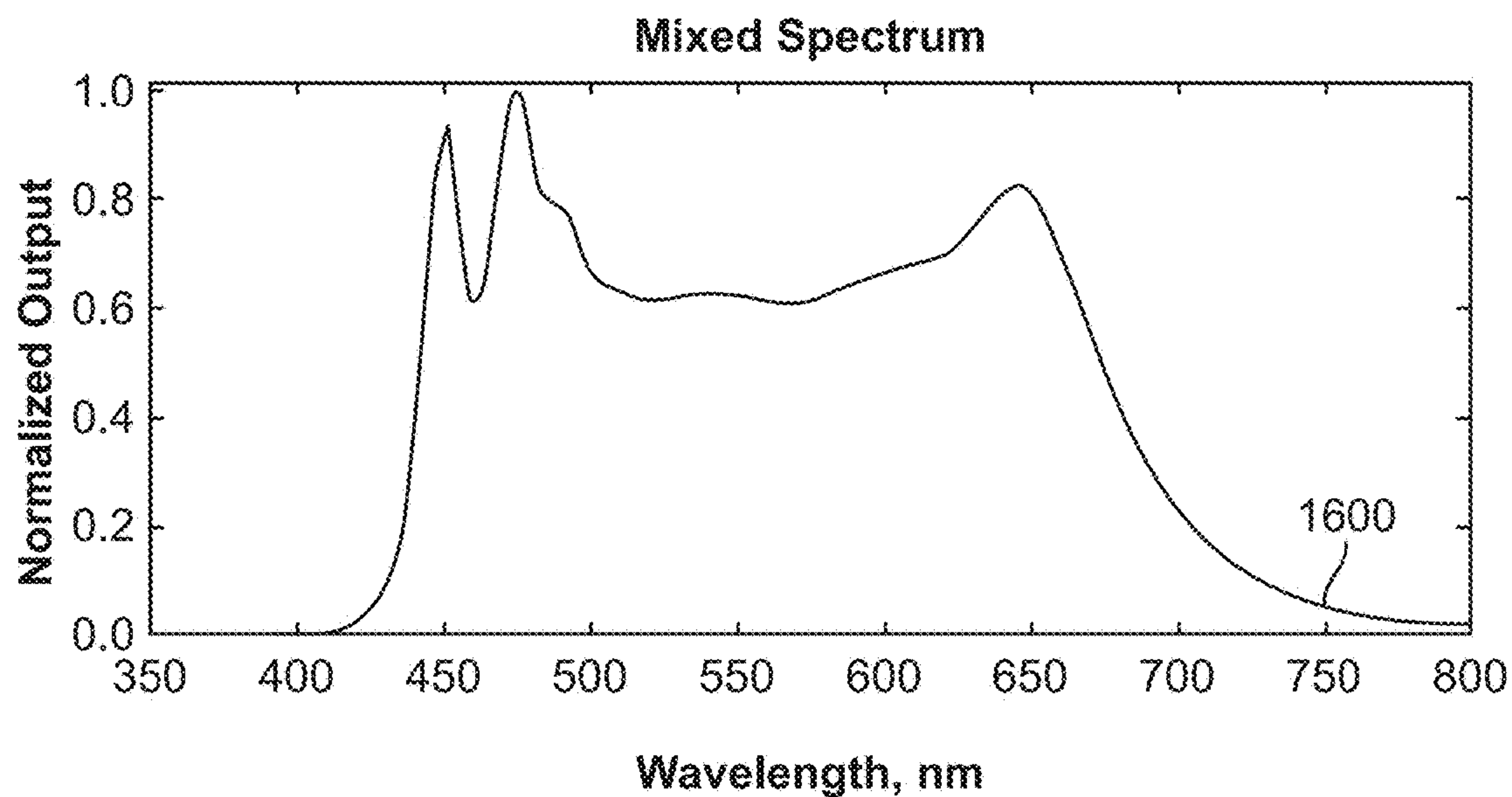
5000K Ch1: Normalized Output vs. Wavelength (nm)
