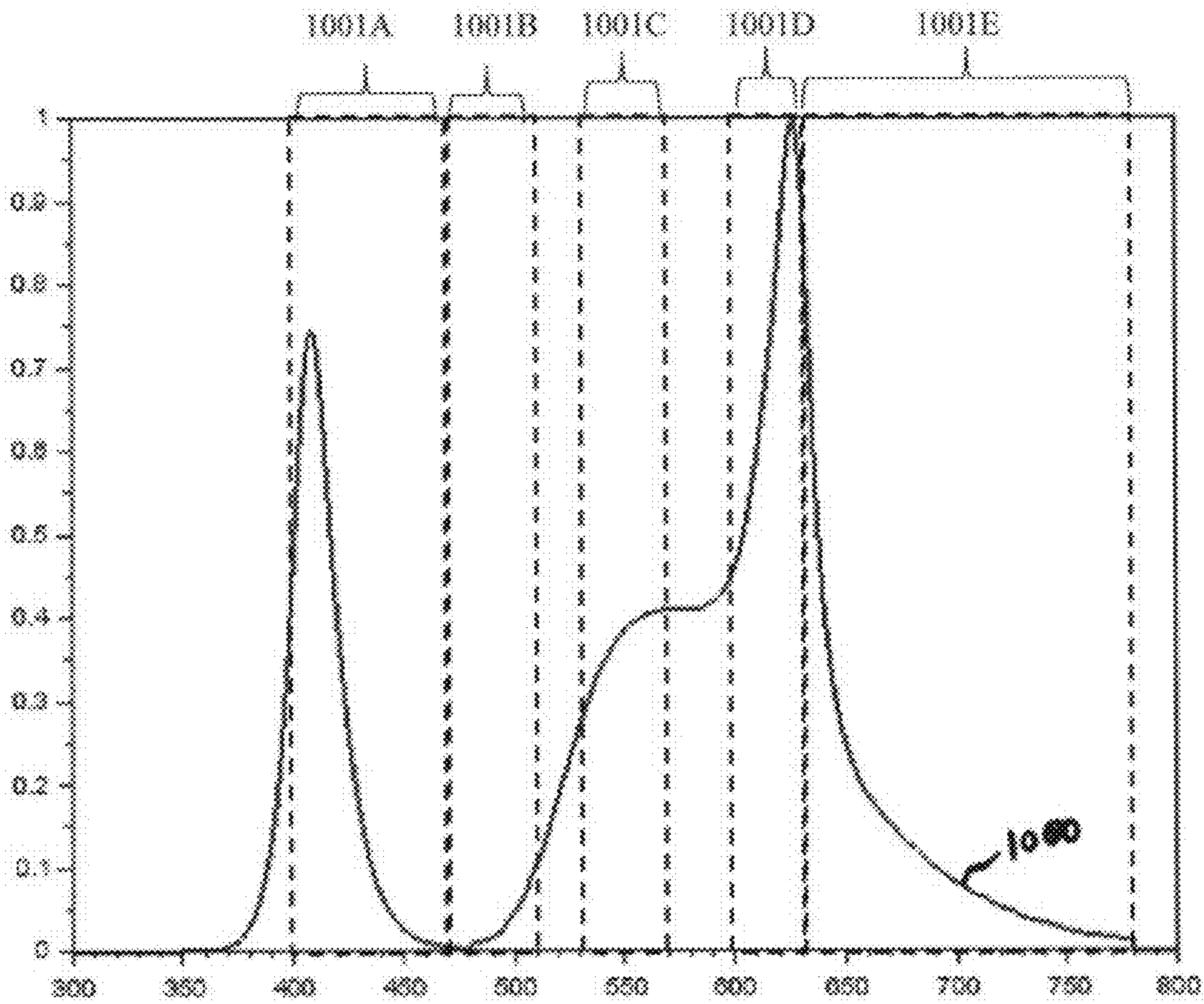
2400K Ch3: Normalized Output vs. Wavelength (nm)
