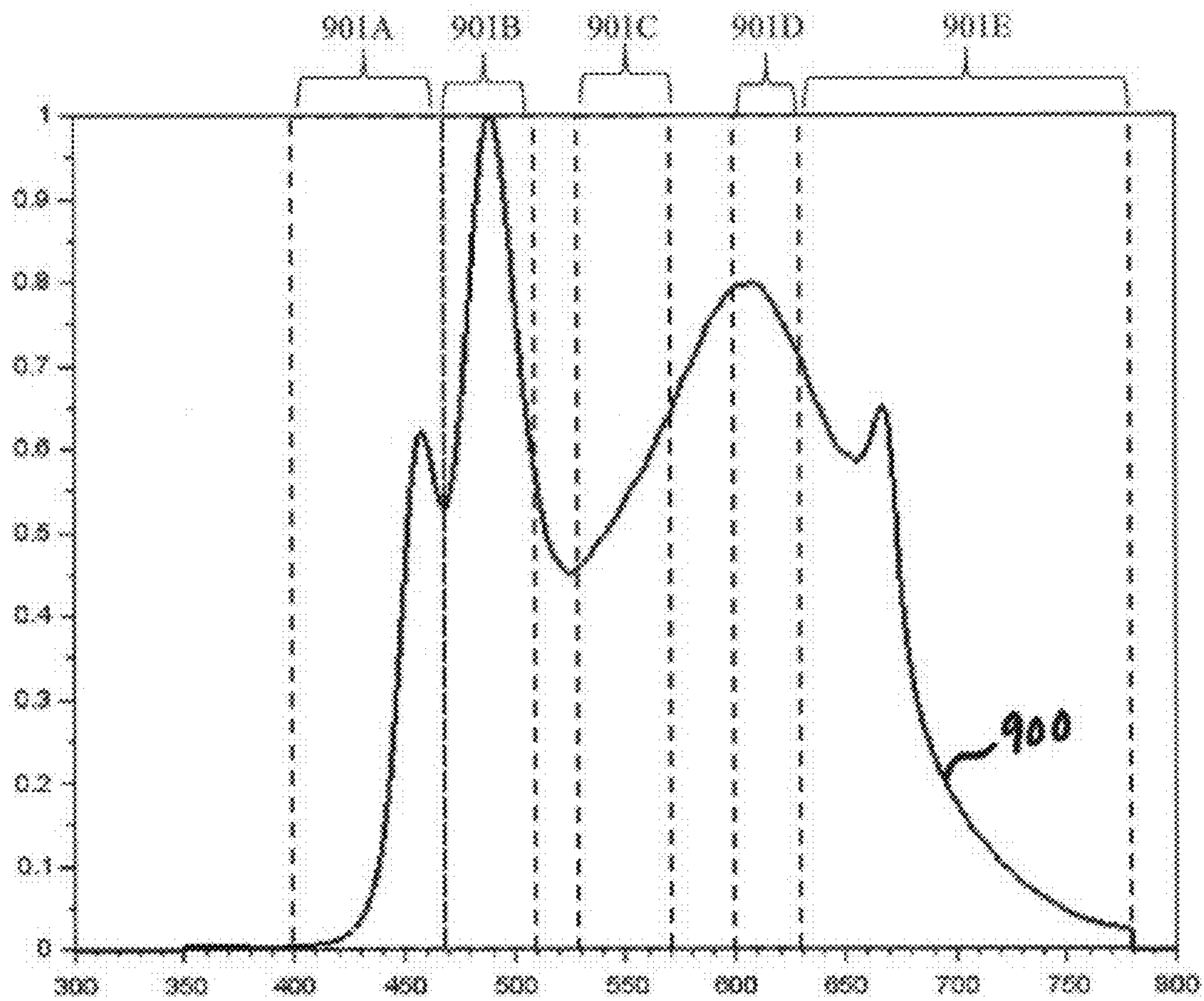
4000K Ch4: Normalized Output vs. Wavelength (nm)
