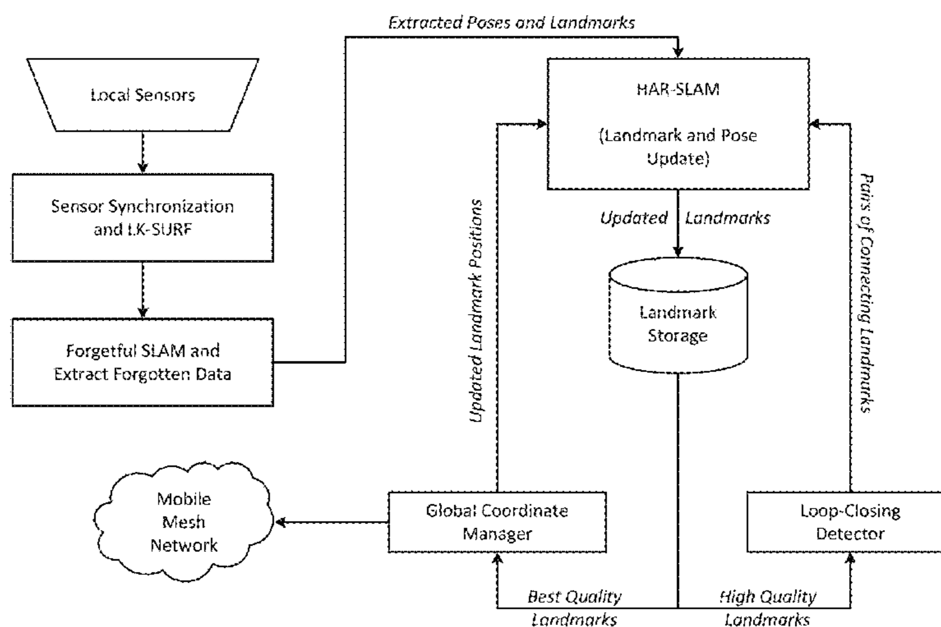
Diagram of Cooperative LP-SLAM
