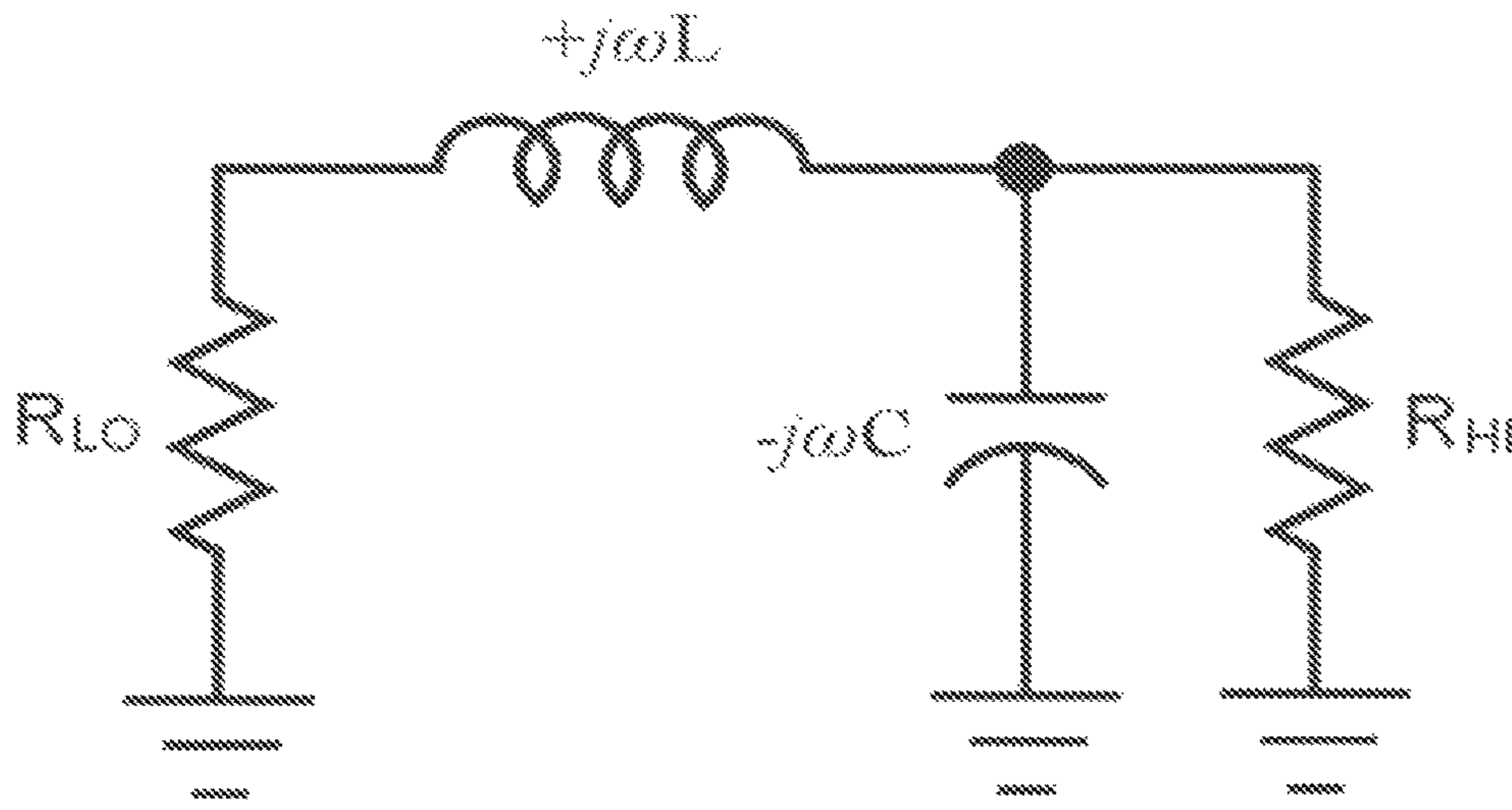
L-Matching network.
