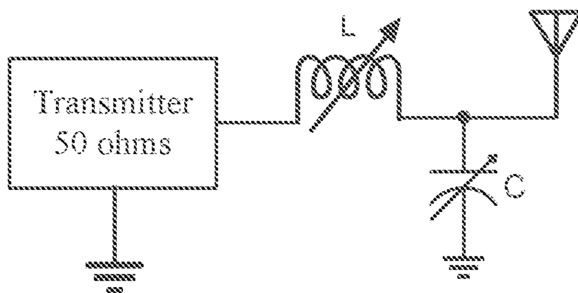
FIGURE 2 (Prior Art)
