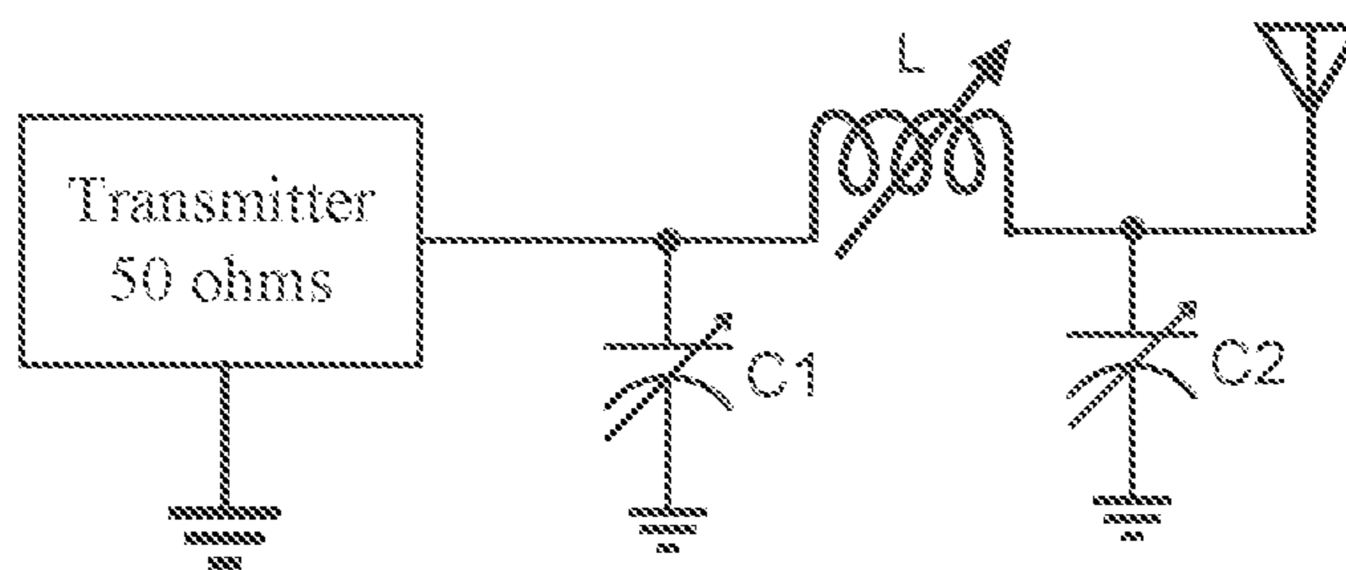
FIGURE 3 (Prior Art)
