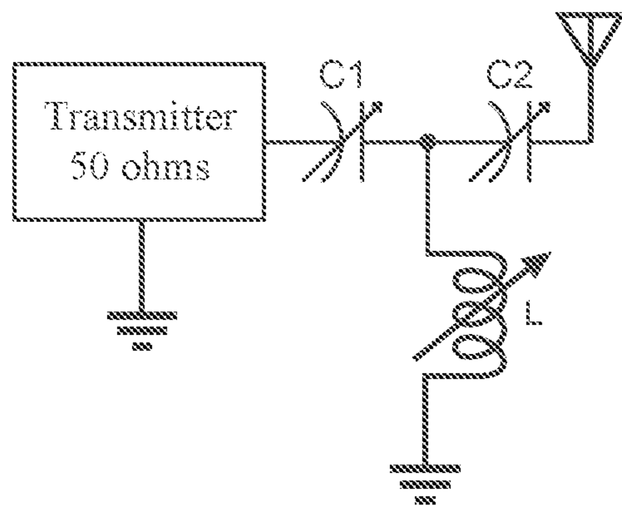
FIGURE 1 (Prior Art)
