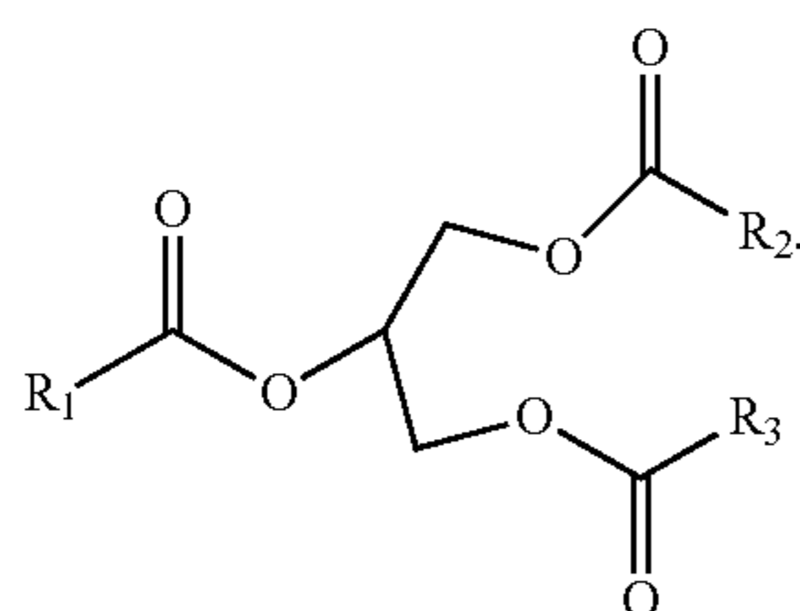
Structure of triglyceride
