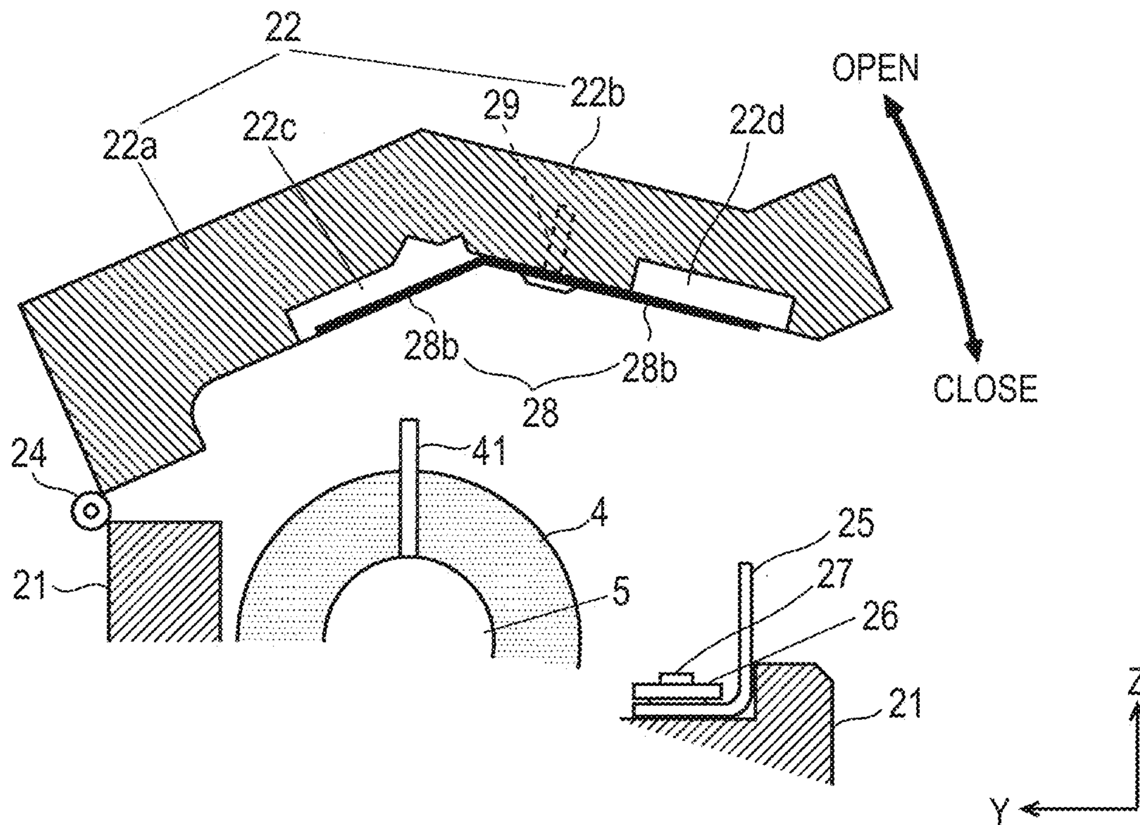
(a) OPEN STATE OF UPPER HOLDER
