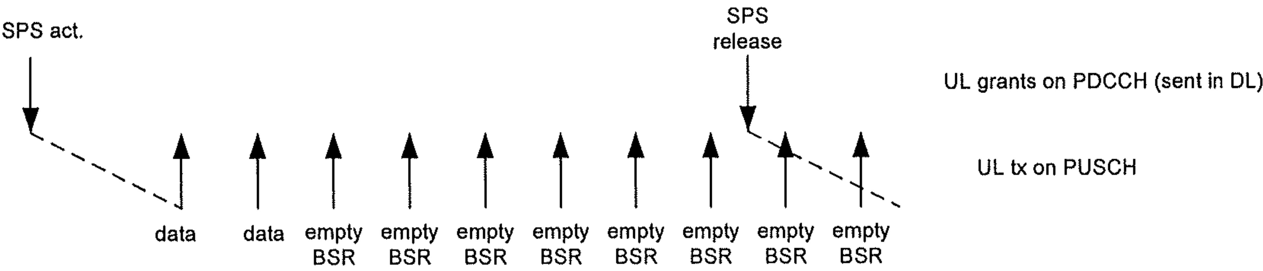
Fig. 1 (Prior Art)
