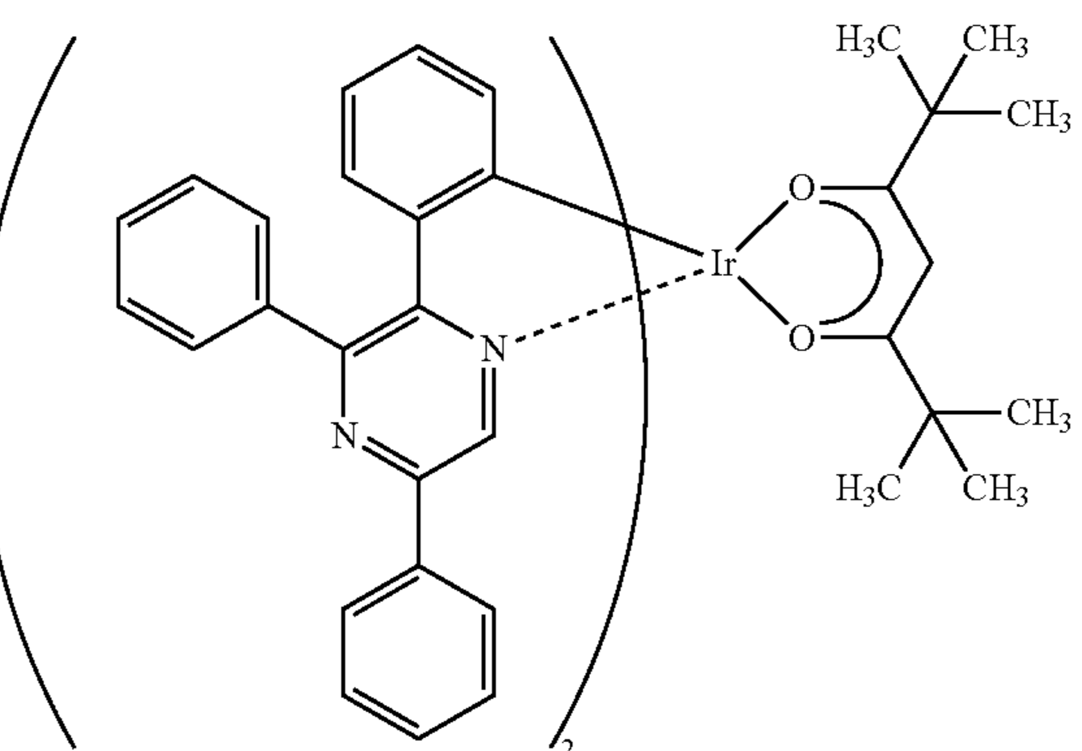
Ir(tppr) 2 (dpm)
