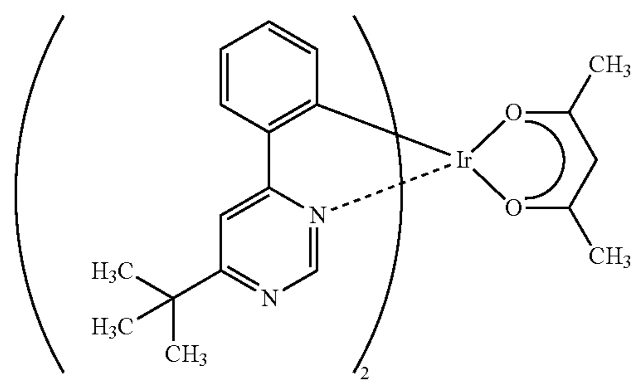
Ir(tBuppm) 2 (acac)
