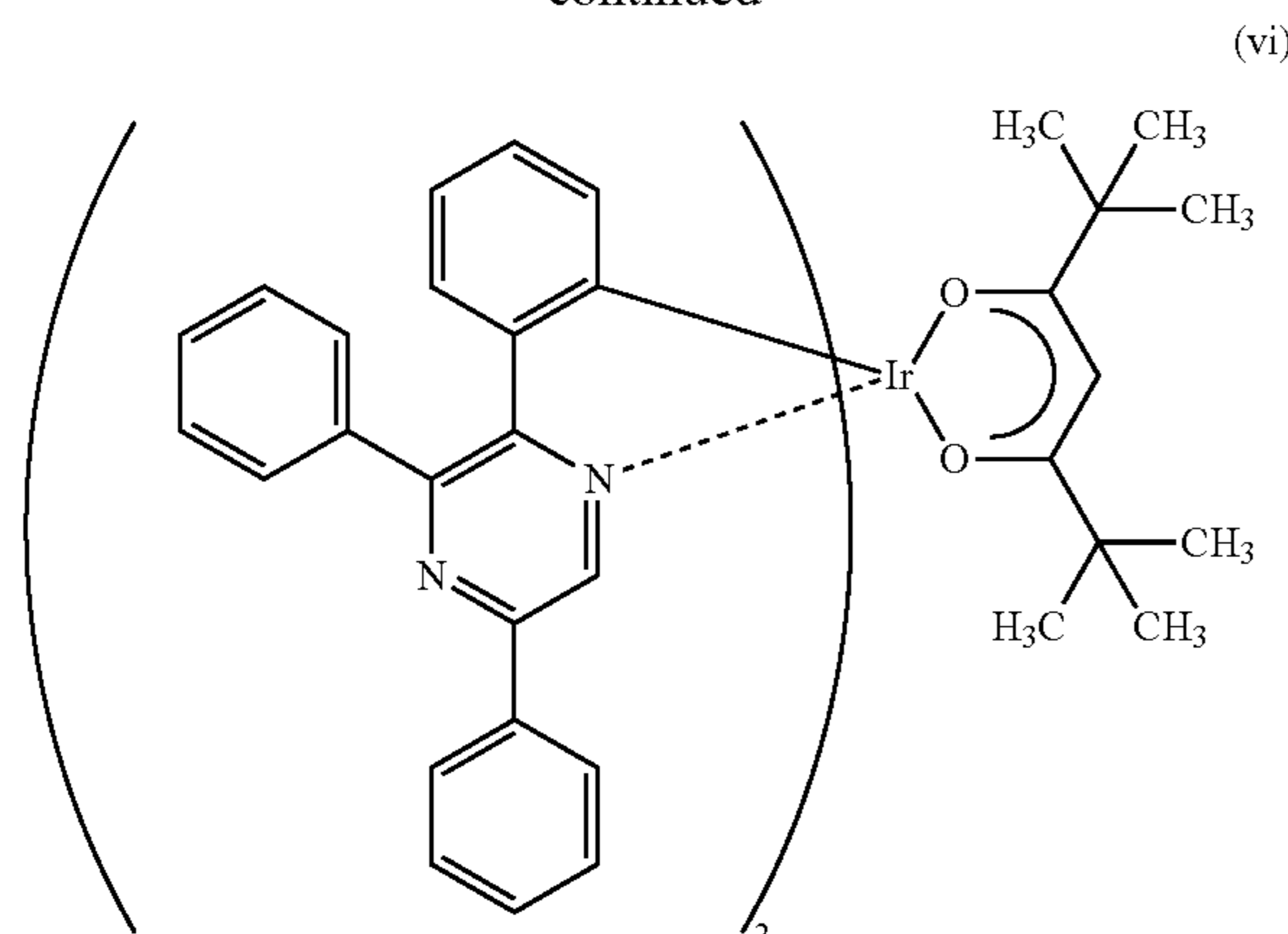
Ir(tppr) 2 (dpm)
