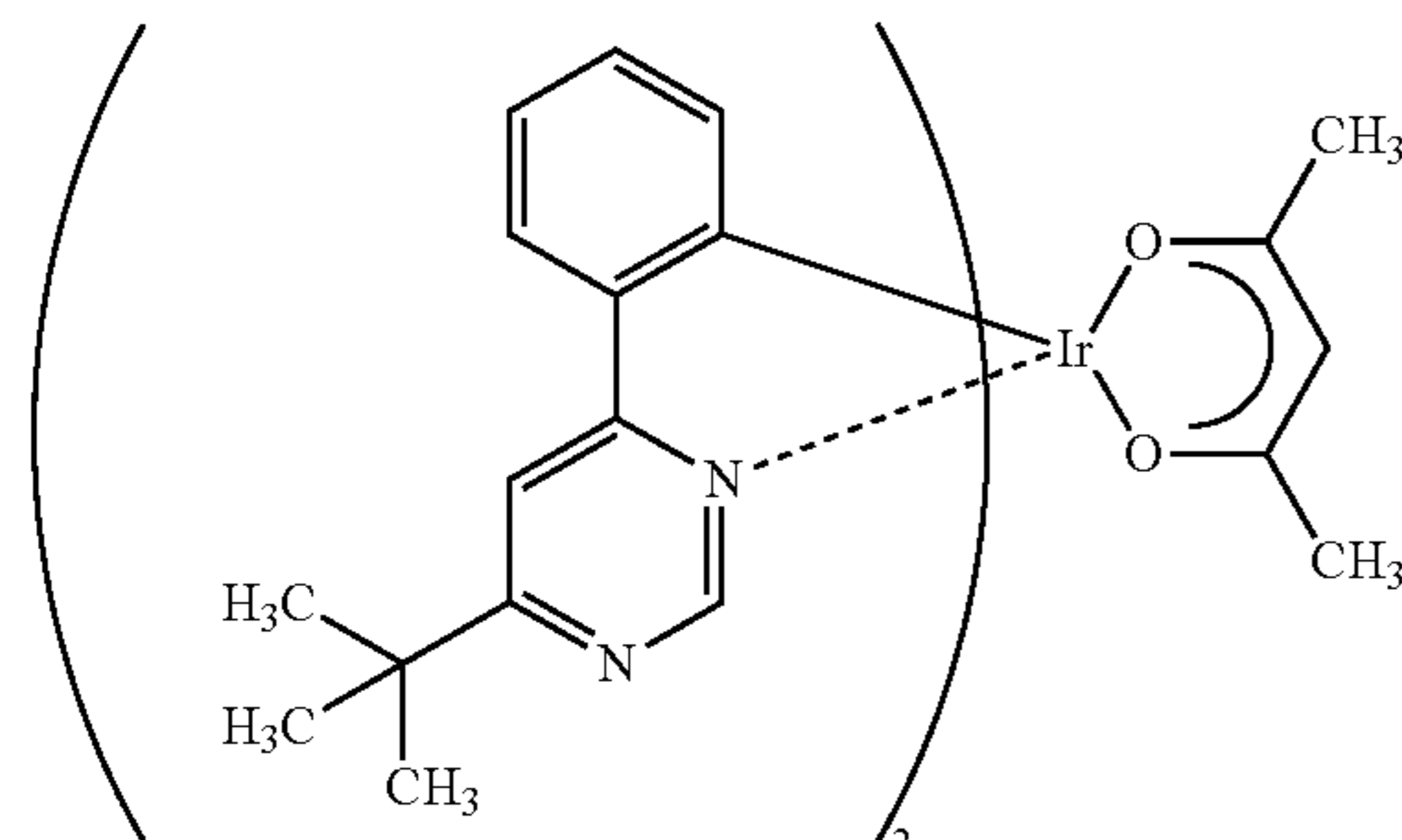
Ir(tBuppm) 2 (acac)
