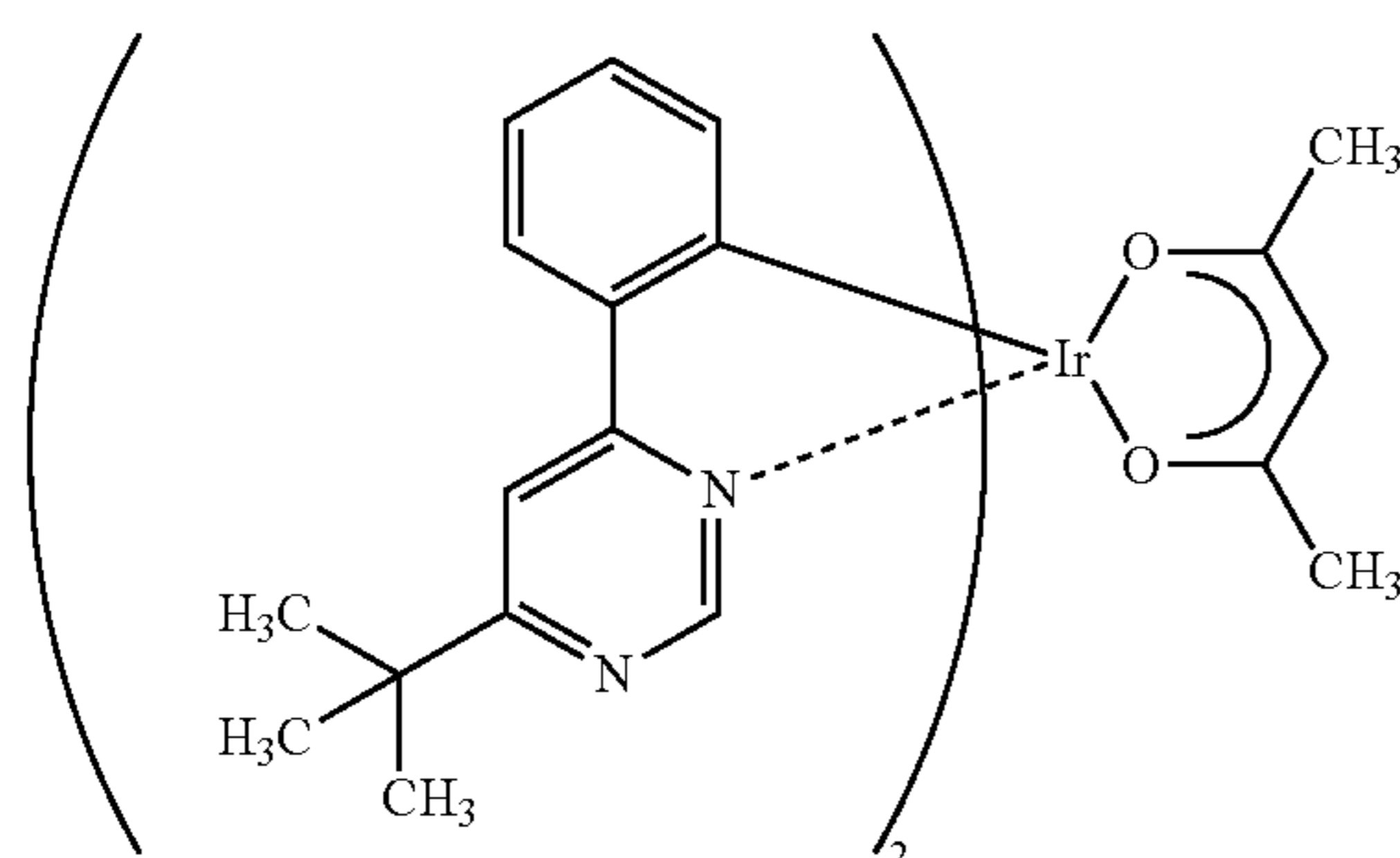
Ir(tBuppm) 2 (acac)
