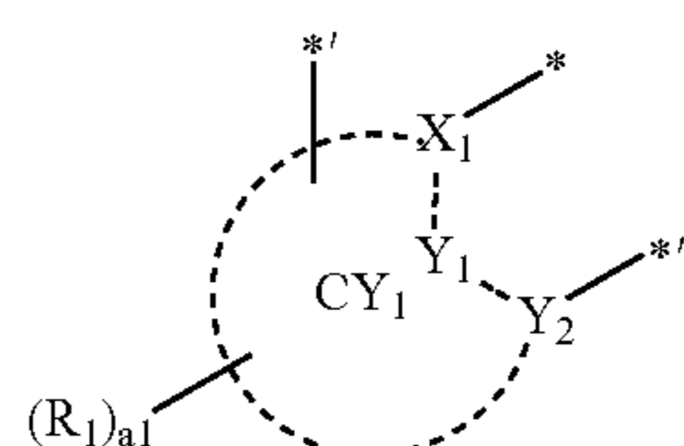
25 Formula A2-1
