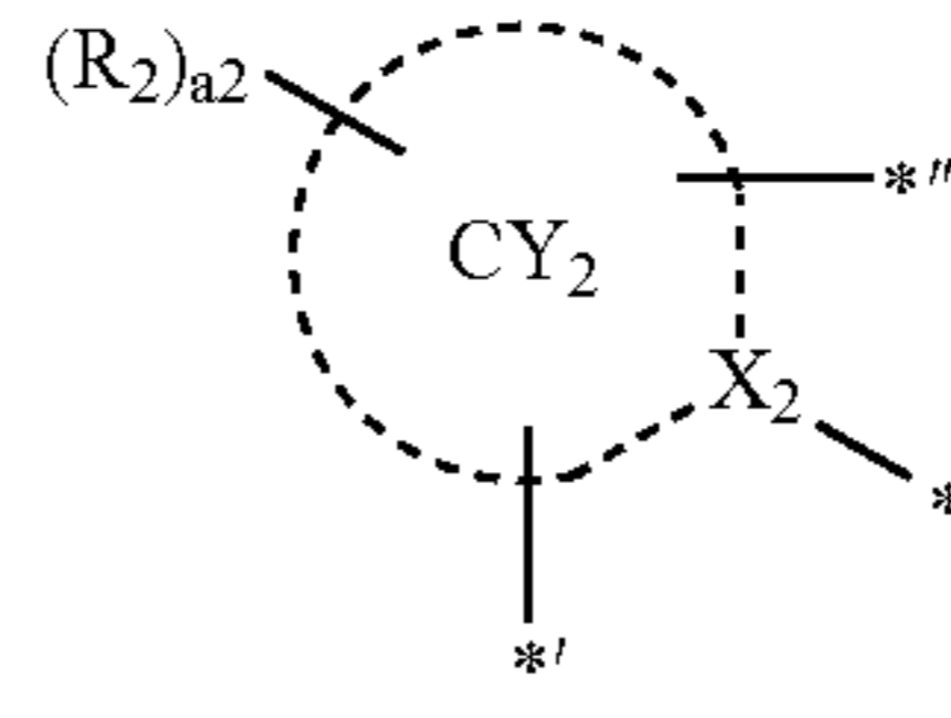
30 Formula A2-2
