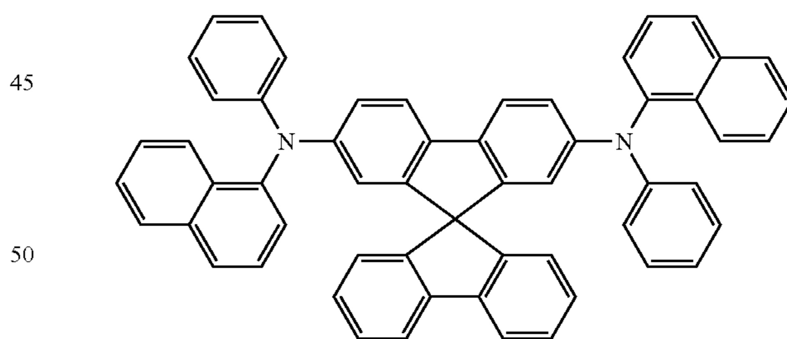
Spiro-NPB
