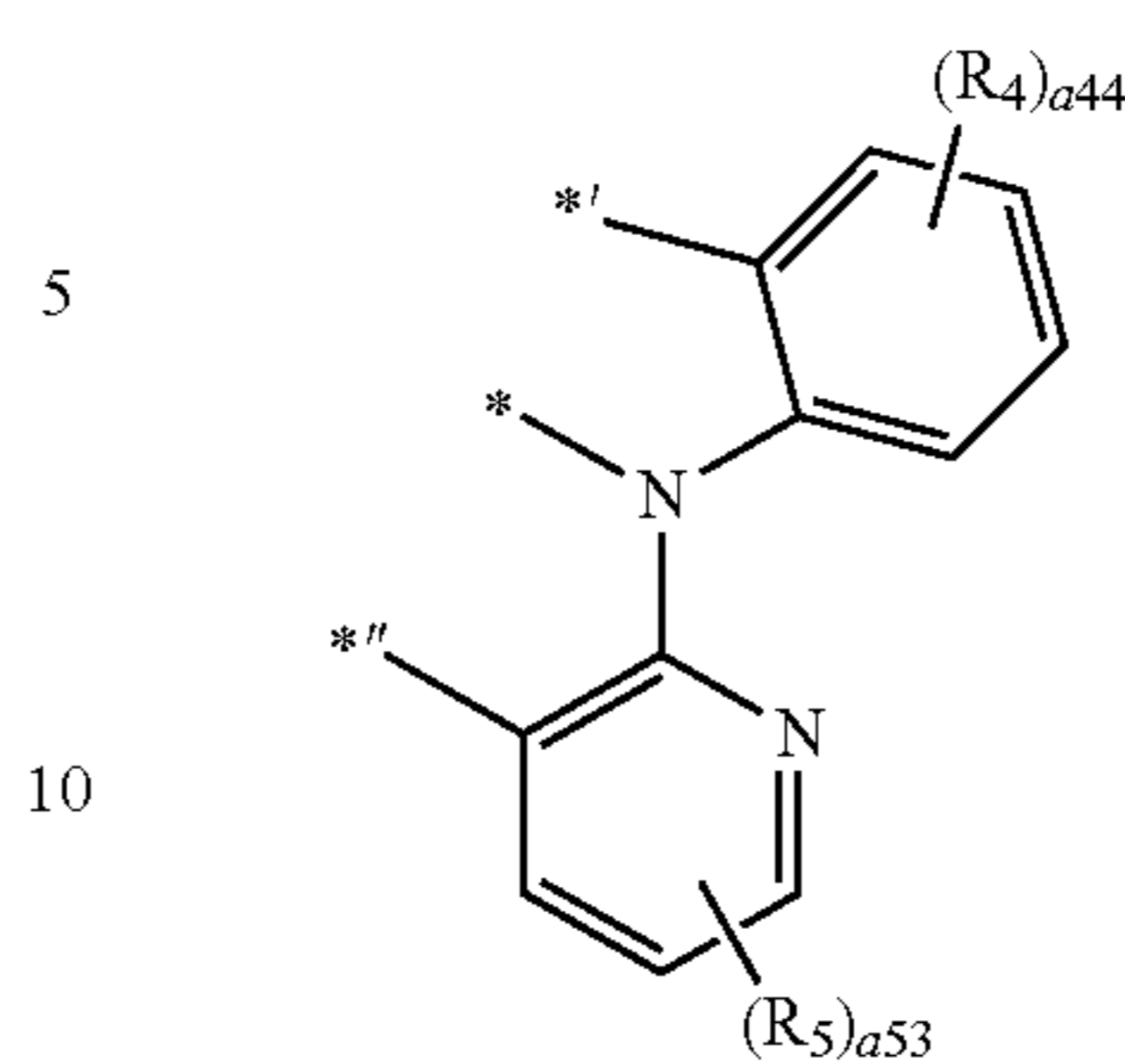
Formula A4-1(1)
