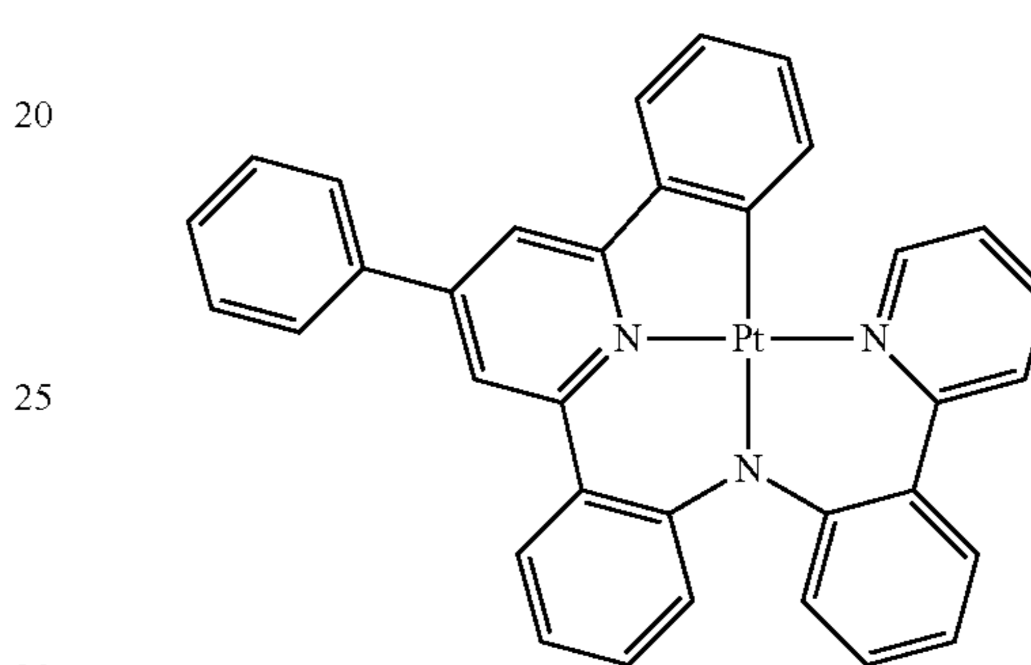
Formula 1-4
