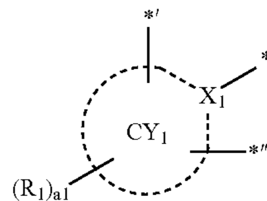
15 Formula A1-2
