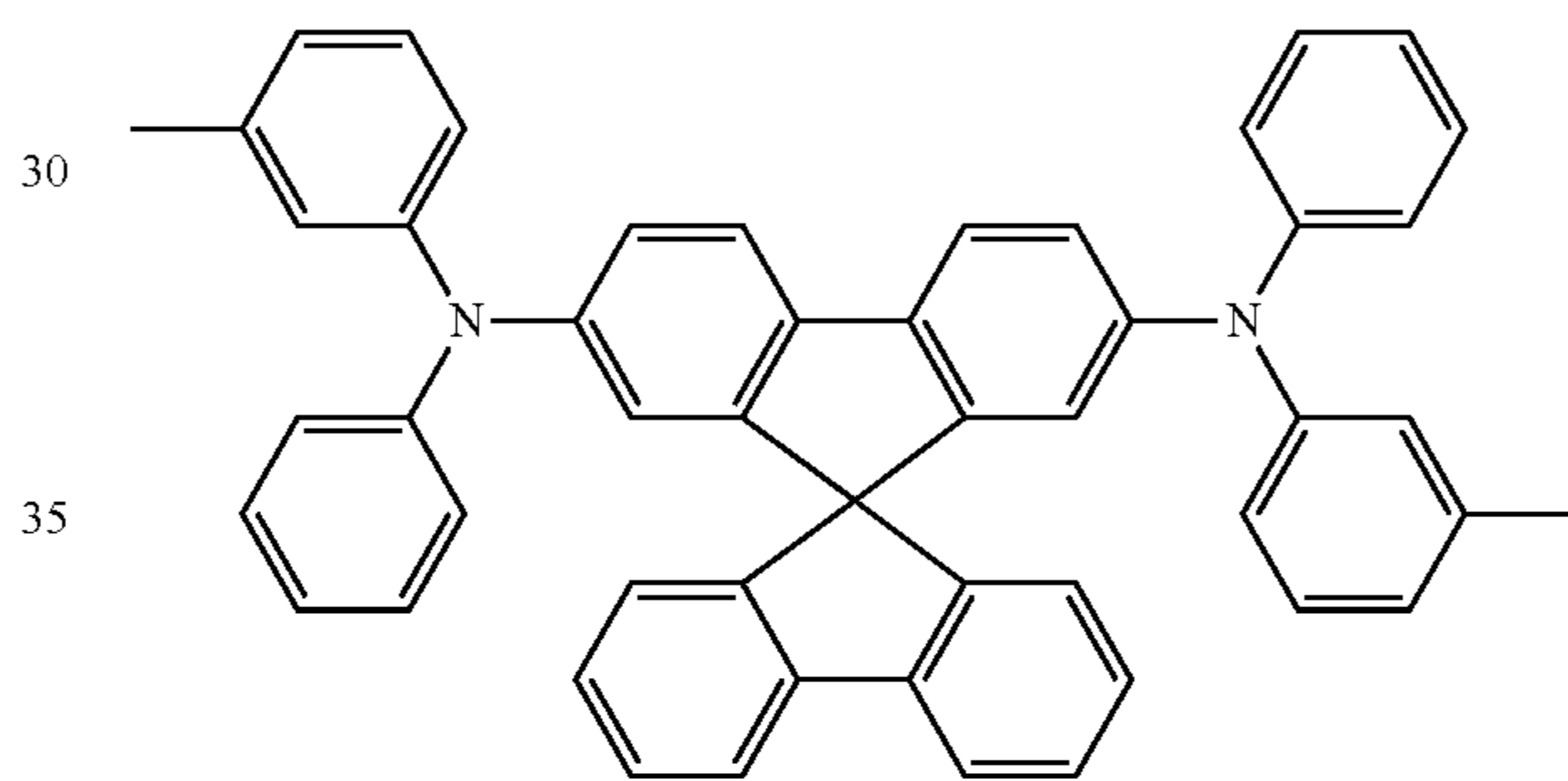
Spiro-TPD
