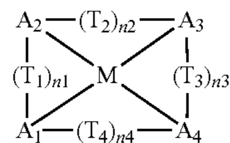
10 Formula A1-1
