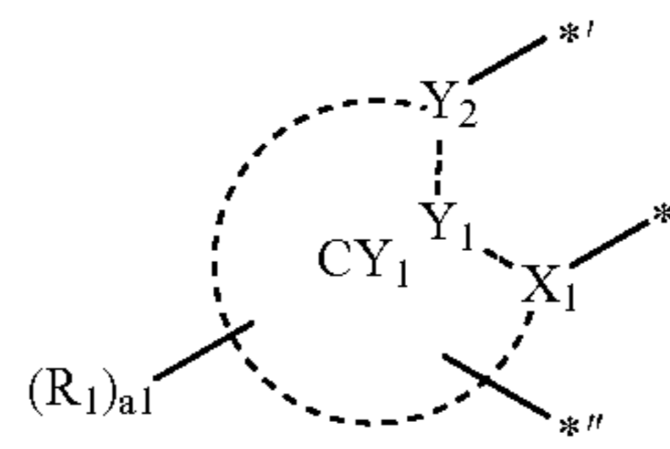
20 Formula A1-3
