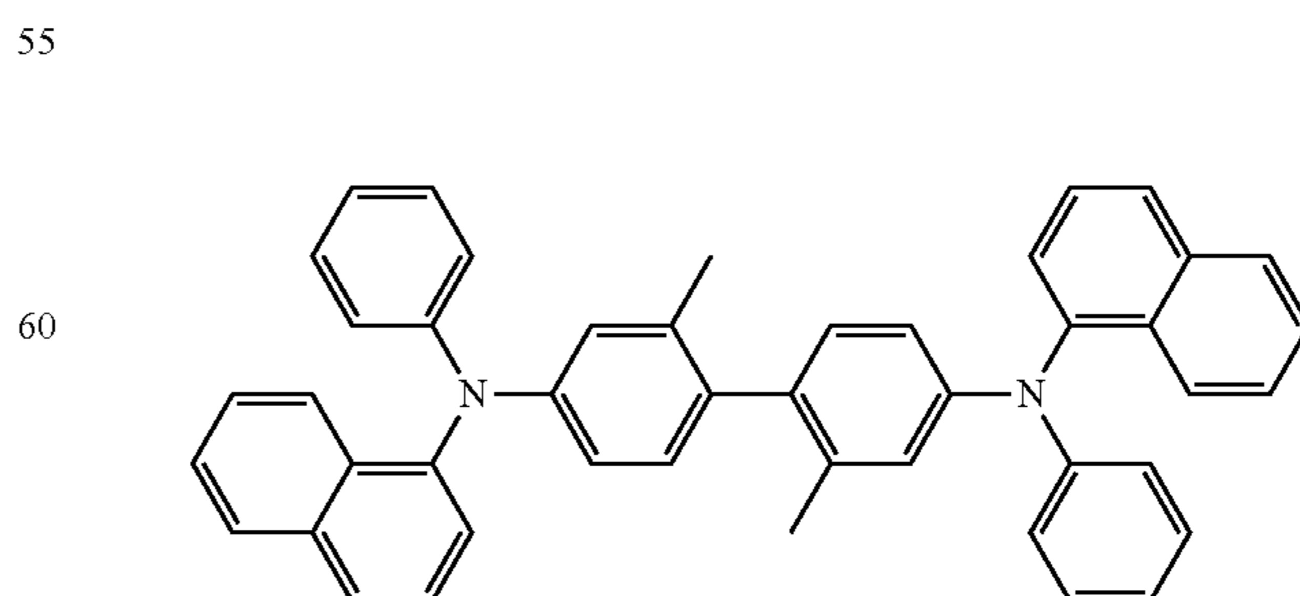
methylated NPB
