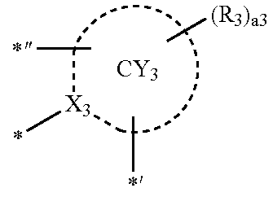
45 Formula A3-2
