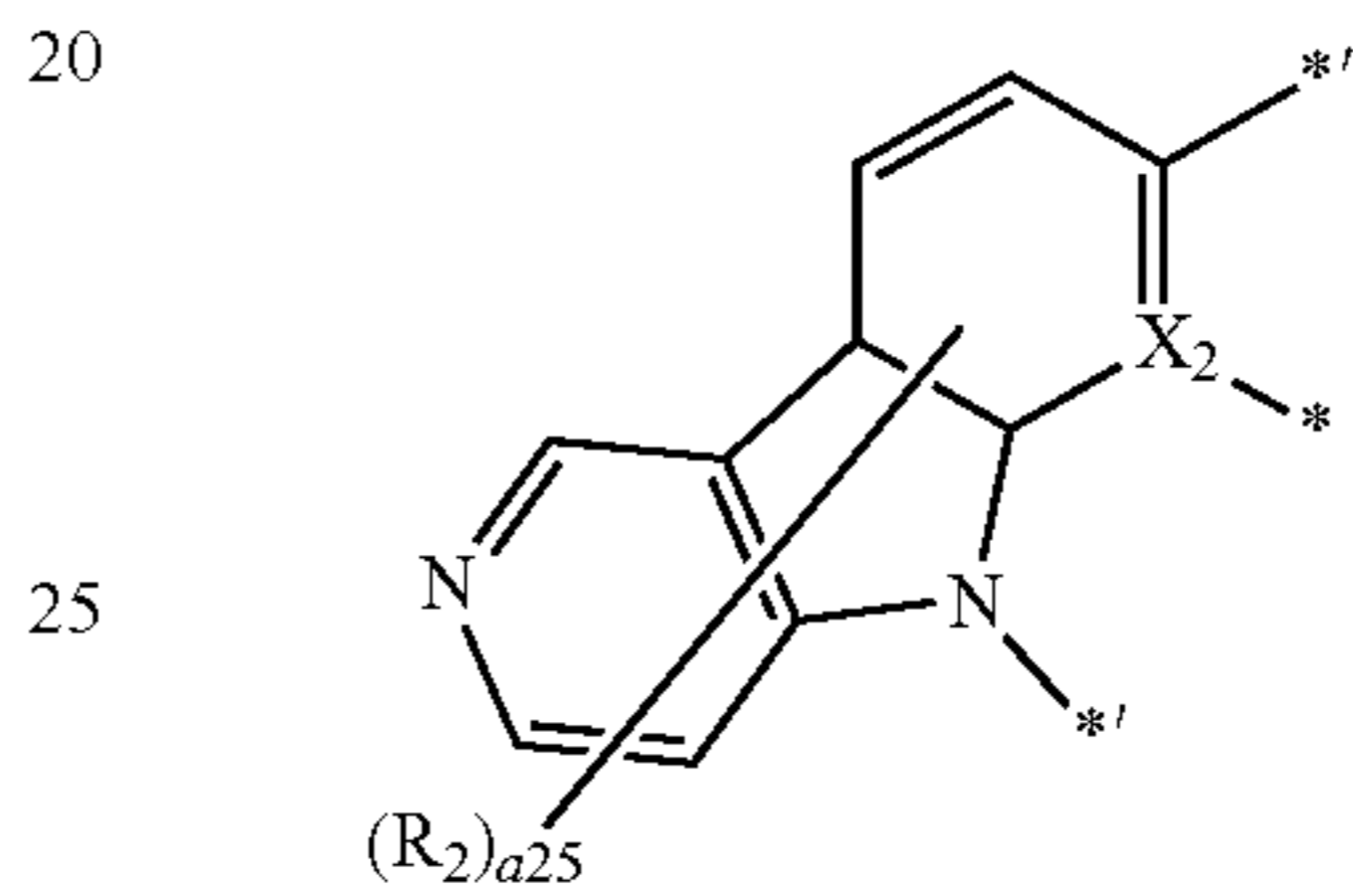
Formula A2-3(49)
