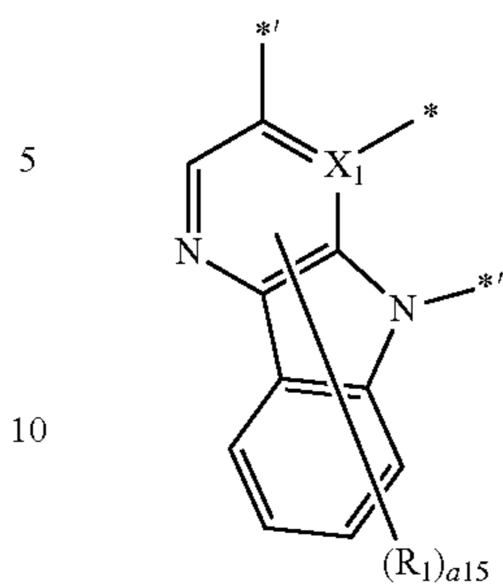
Formula A1-3(48)
