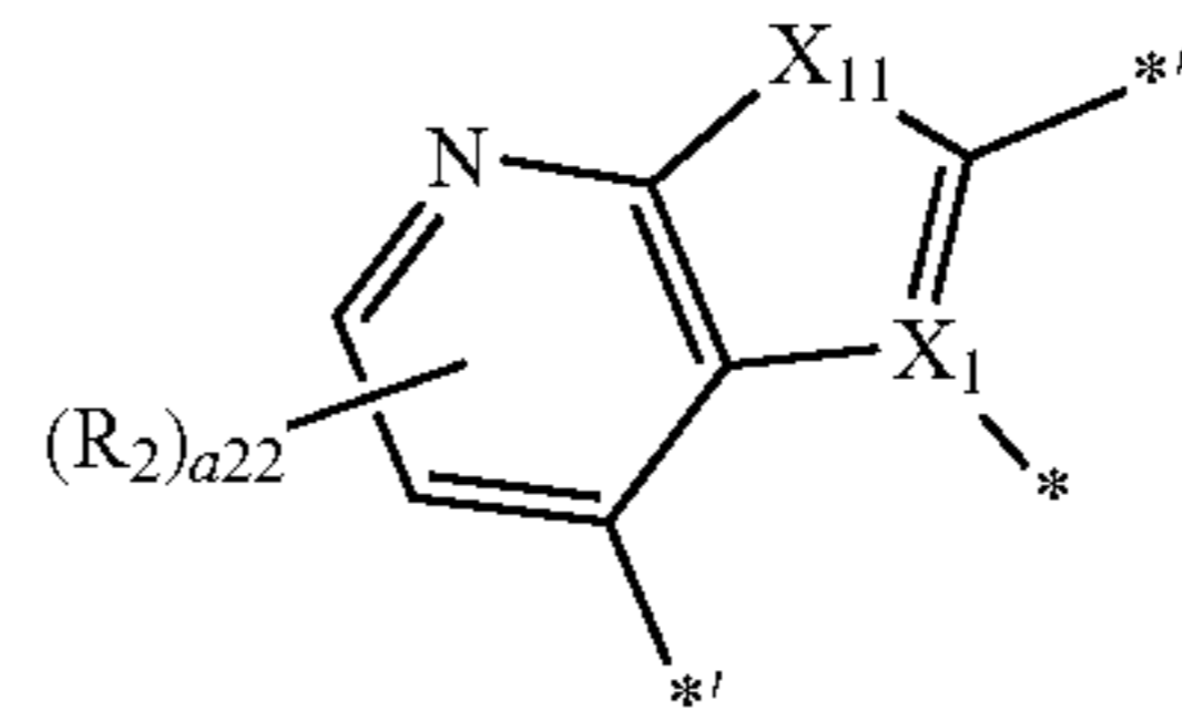
Formula A2-3(1)
