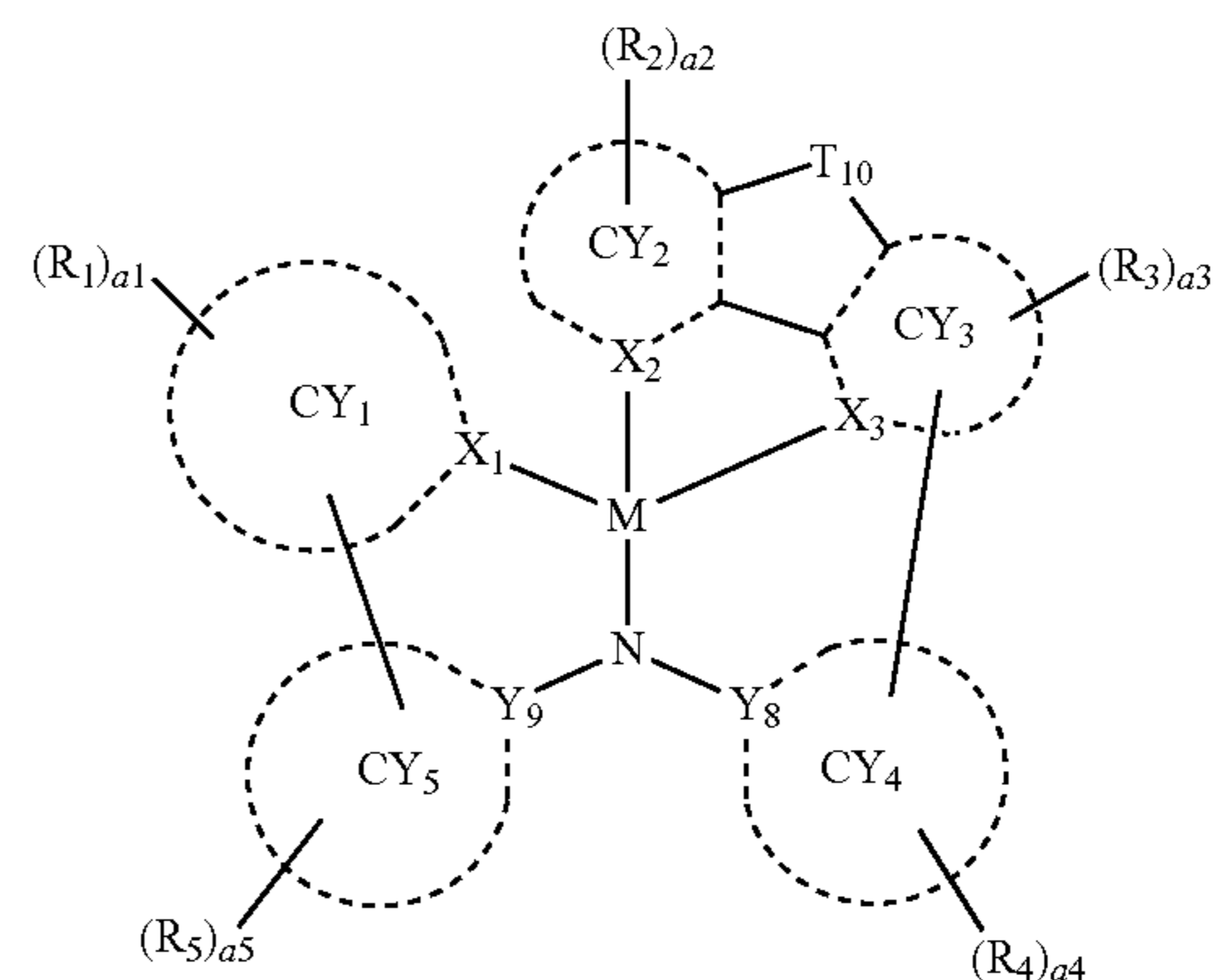
Formula 1-2
