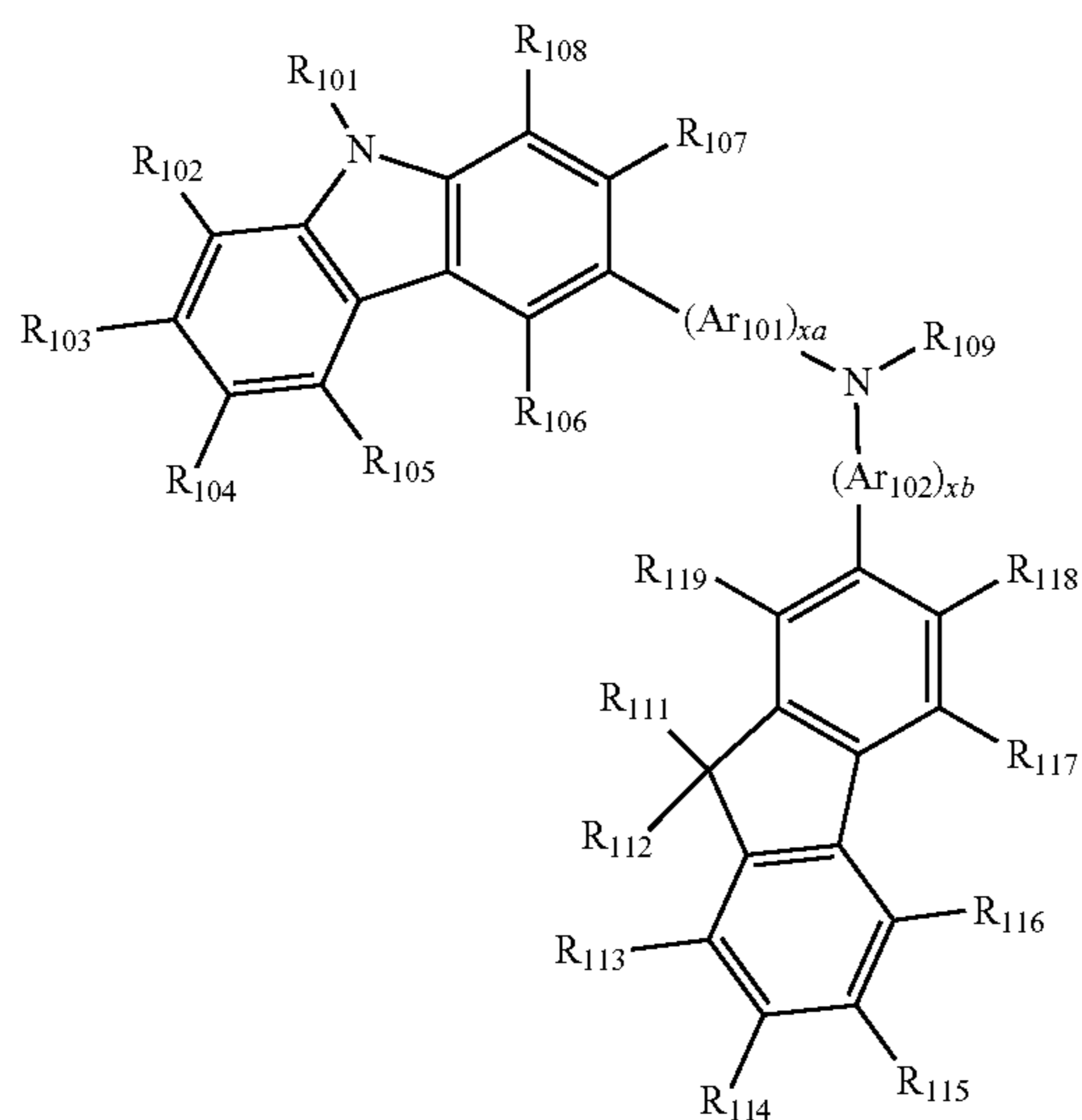
Formula 201
