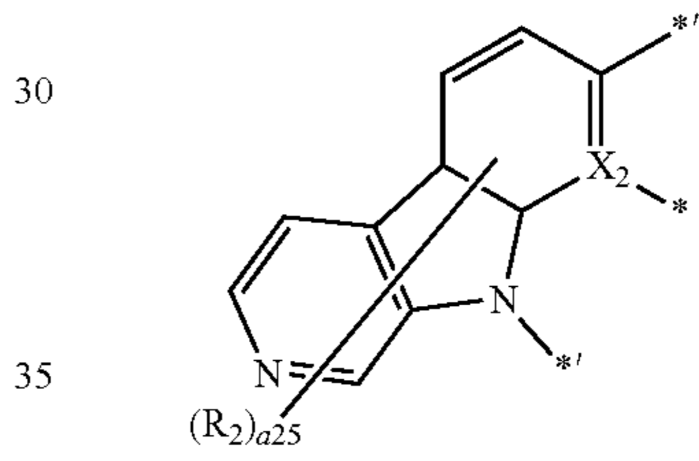
Formula A2-3(50)
