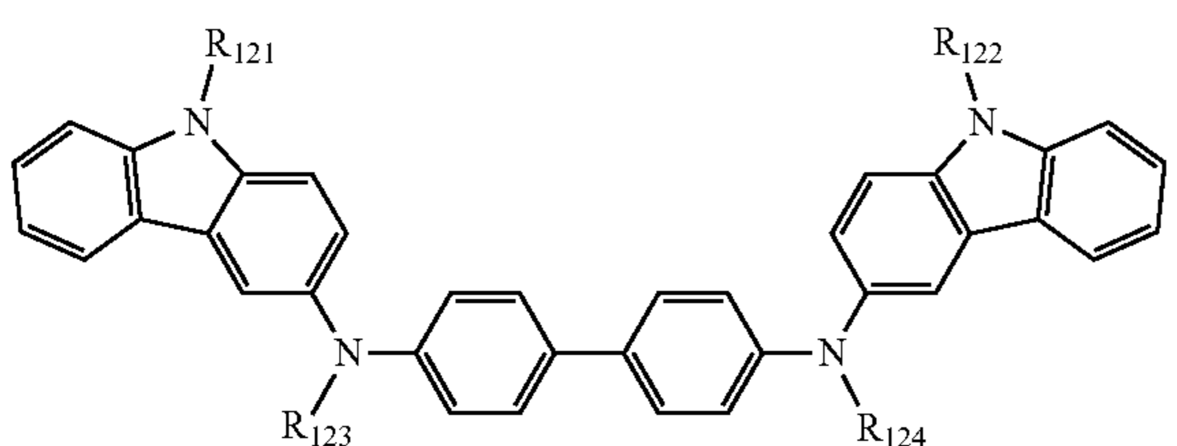
Formula 202
