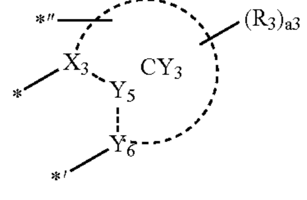
50 Formula A3-3
