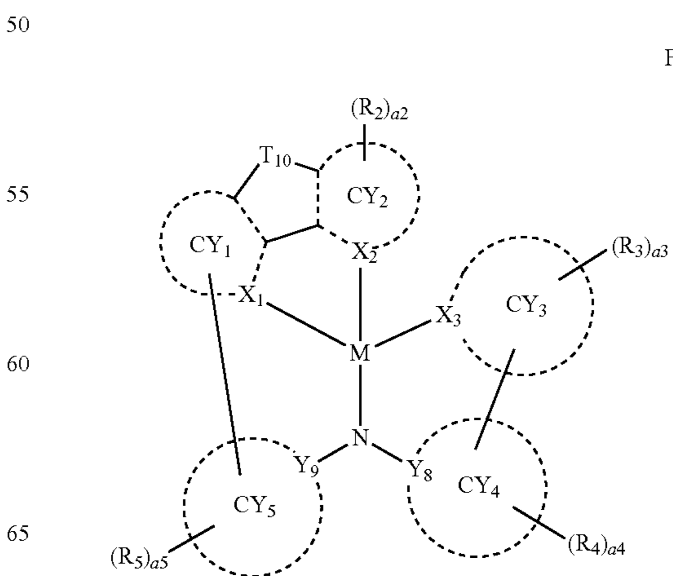
Formula CY4-25
