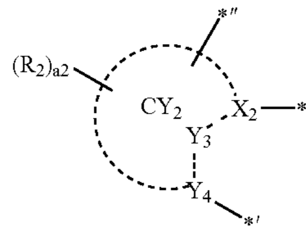
40 Formula A3-1
