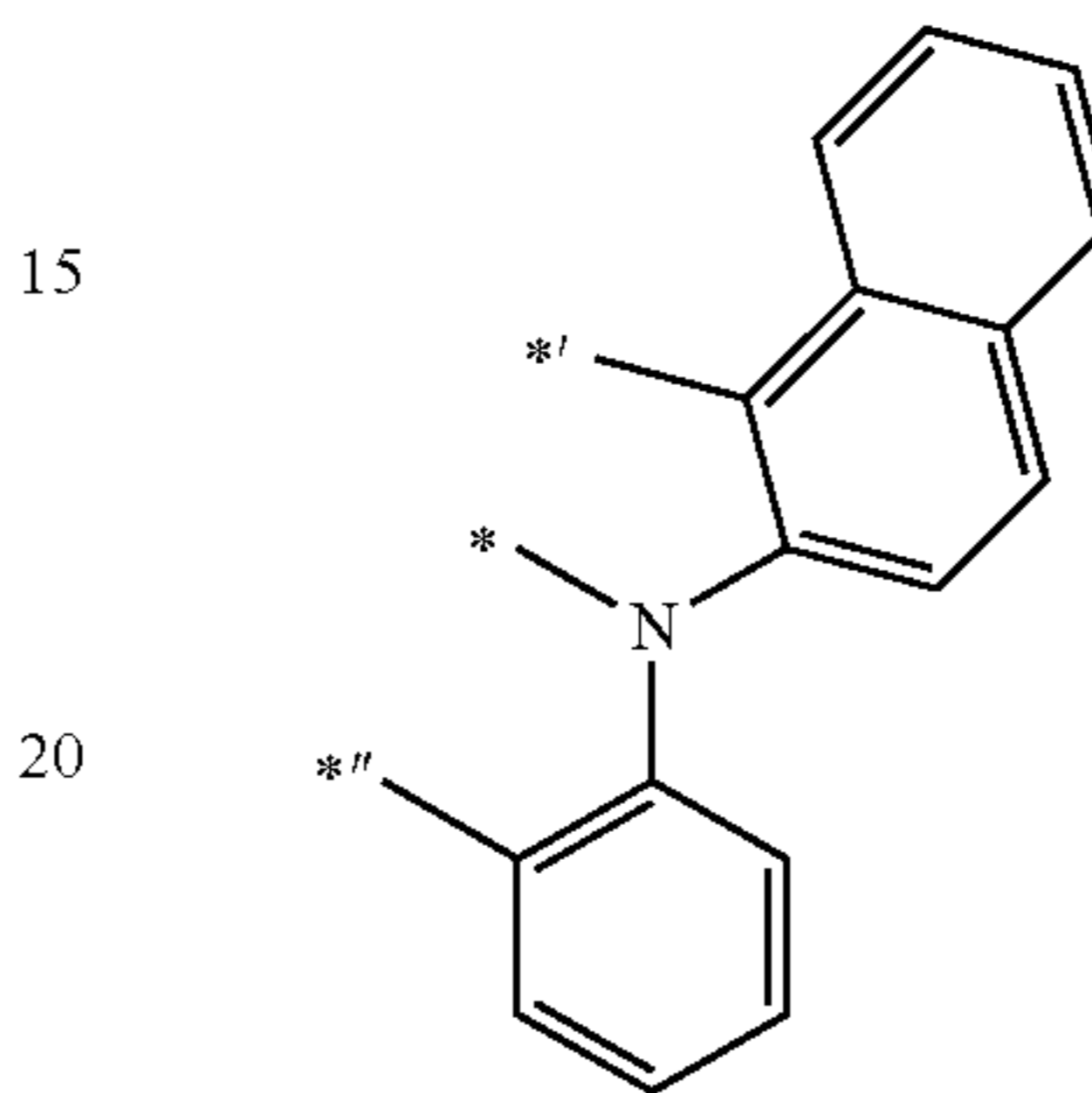
Formula CY4-22
