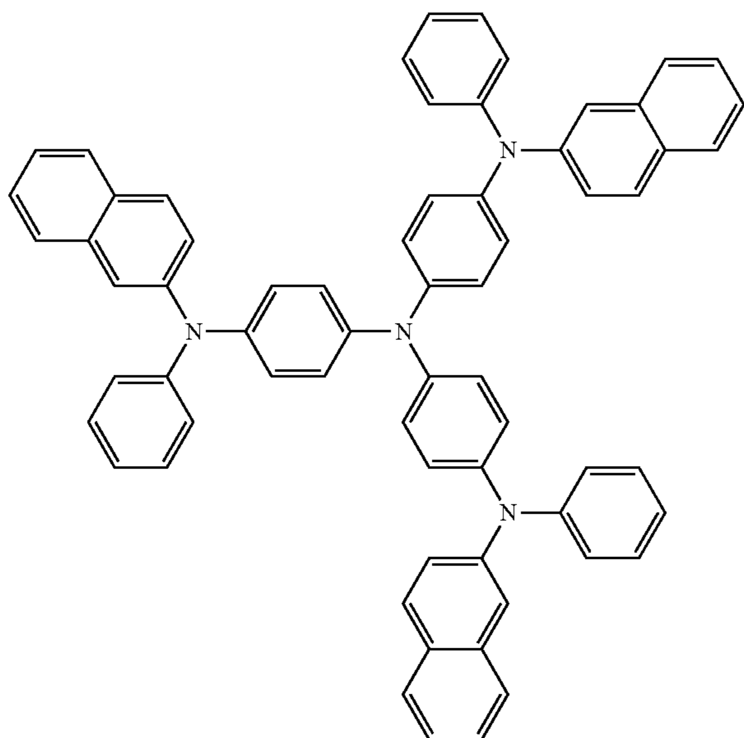
2-TNATA
