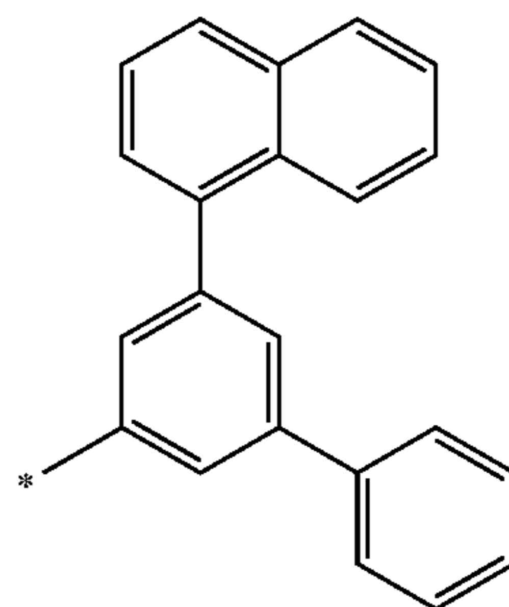
Formula 10-75
