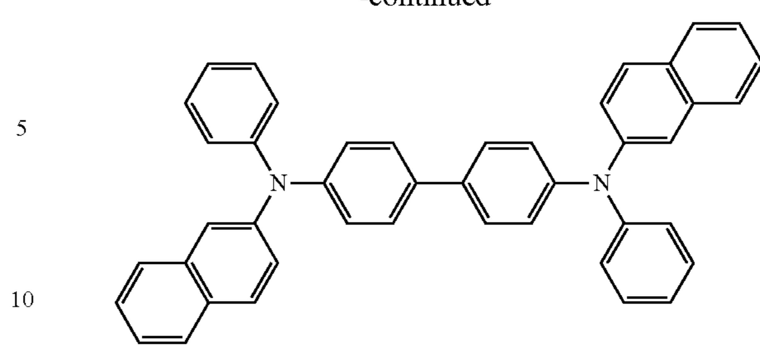
\beta -NPB
