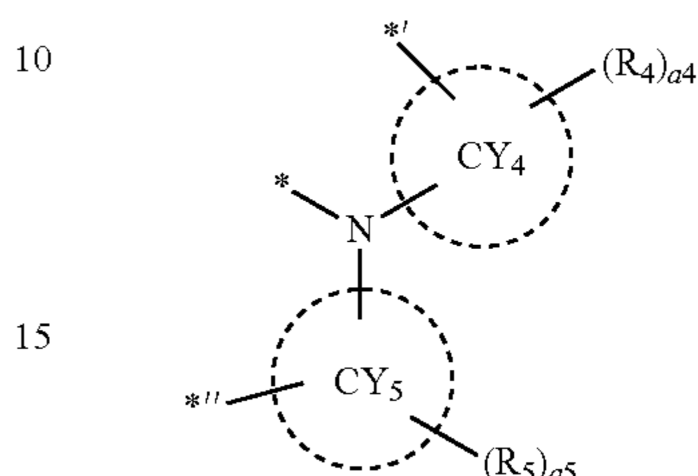
Formula A1-1
