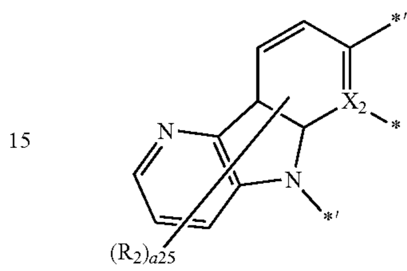
Formula A2-3(48)
