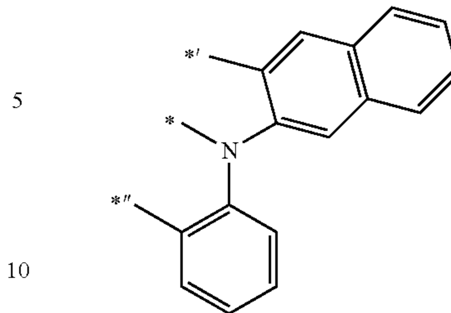
Formula CY4-21
