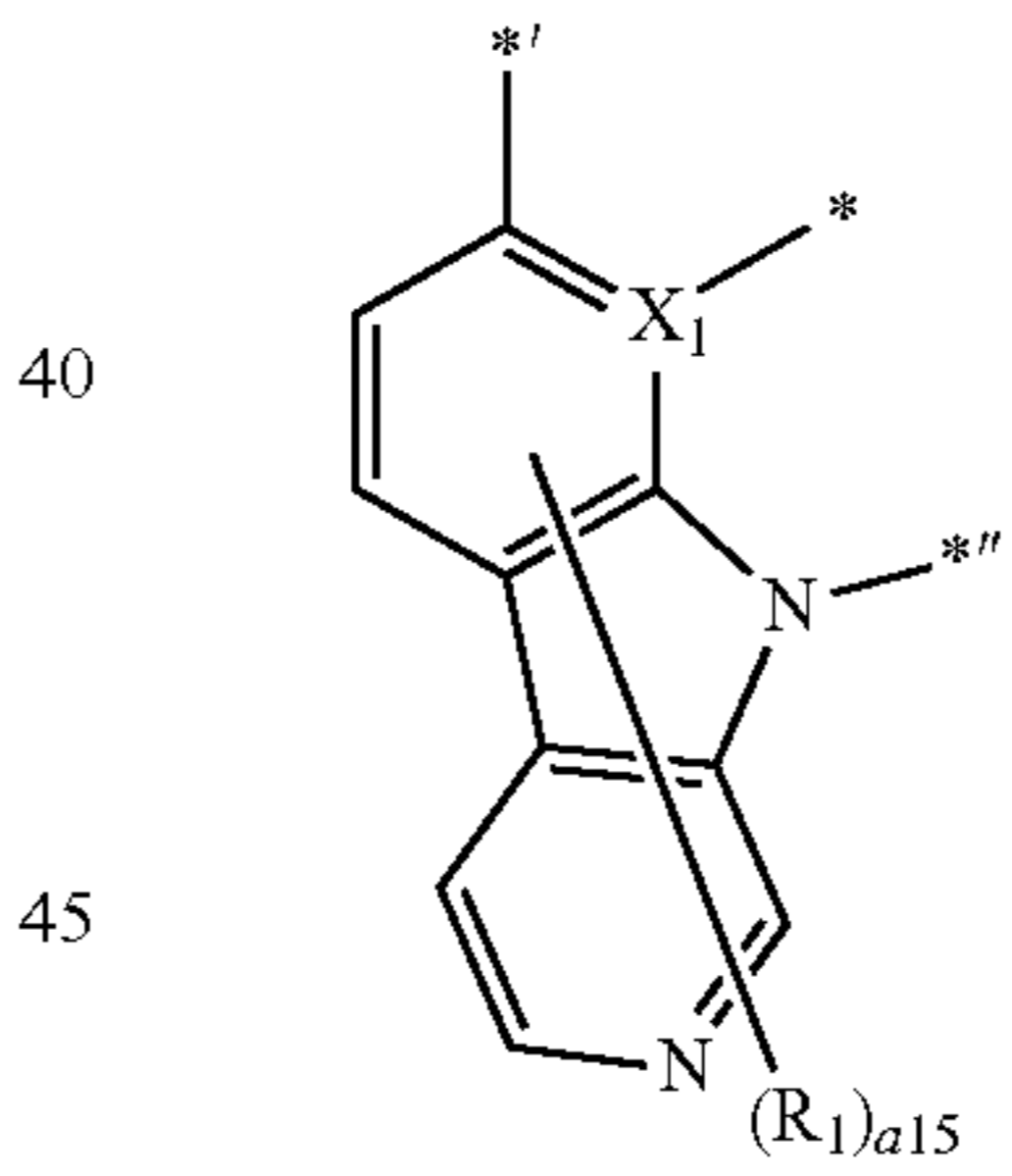
Formula A1-3(52)
