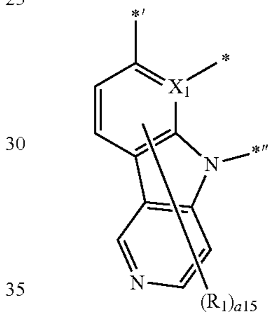
Formula A1-3(50)
