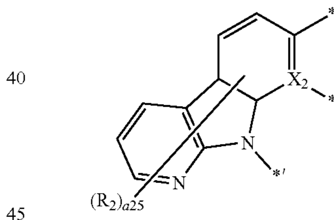
Formula A2-3(51)
