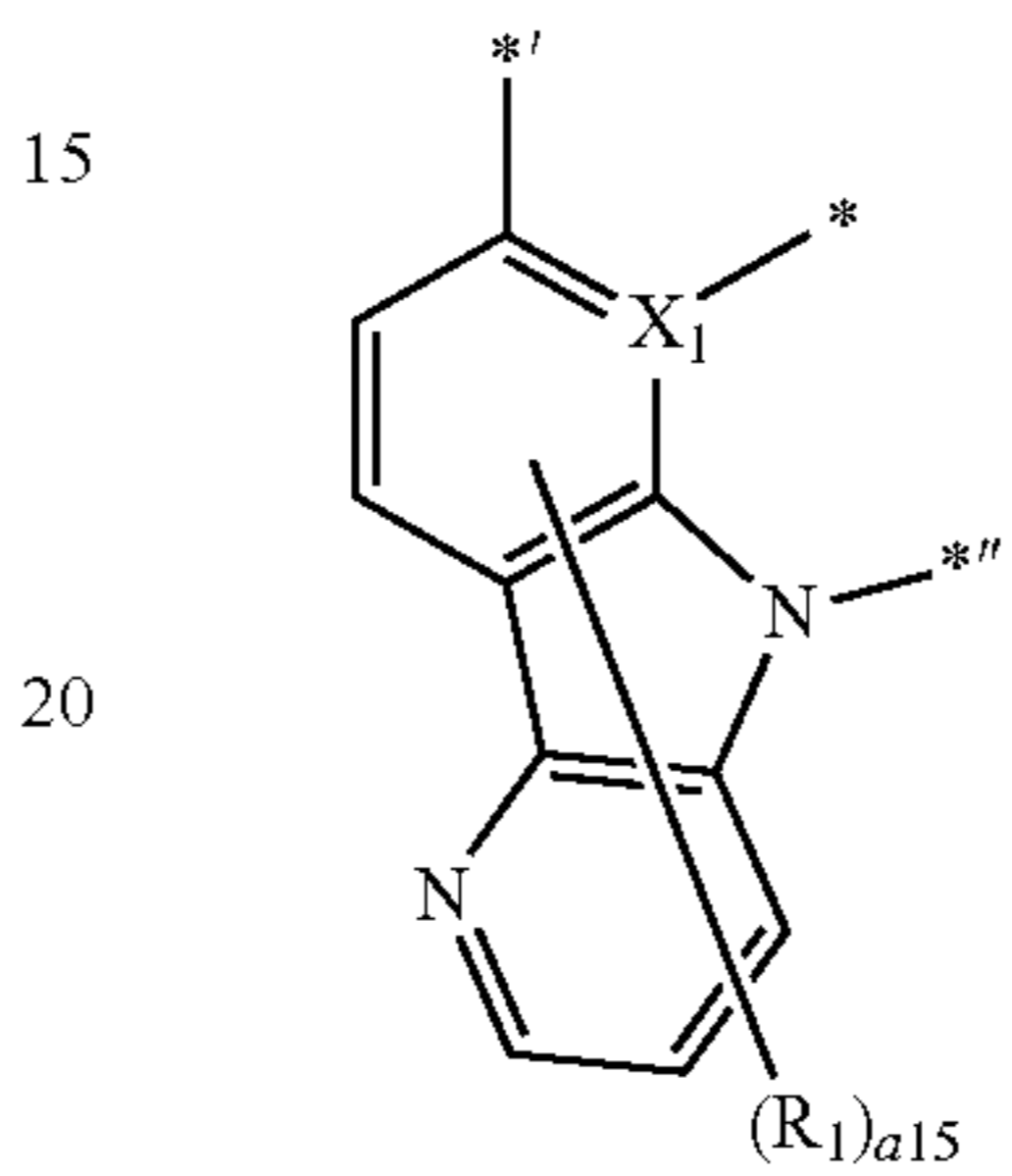
Formula A1-3(49)
