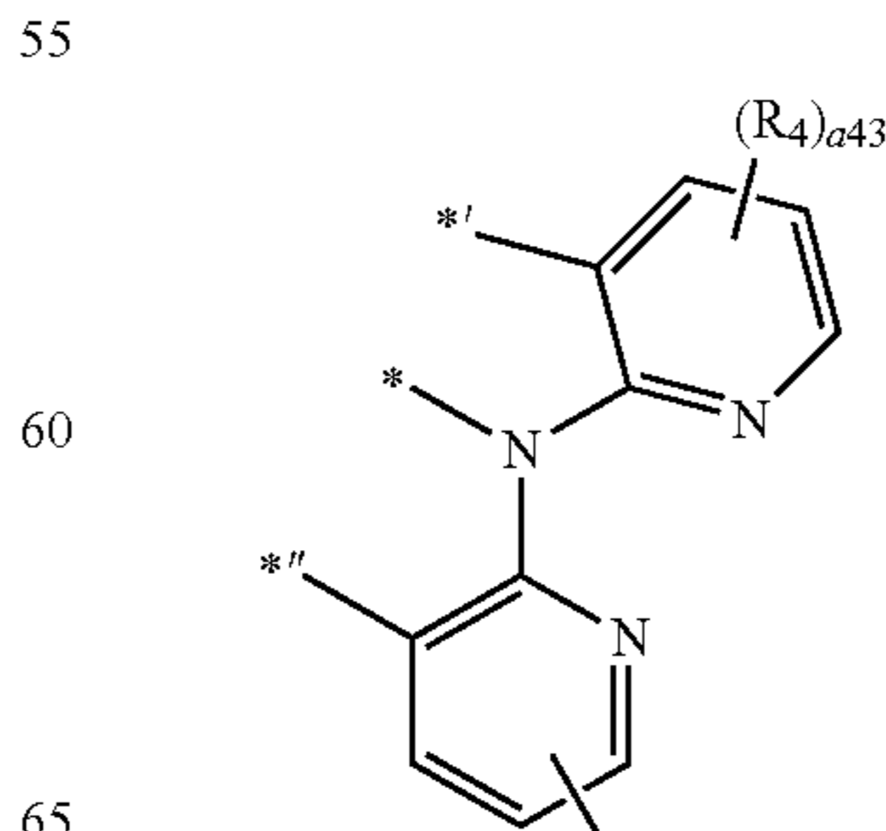
Formula A4-1(5)
