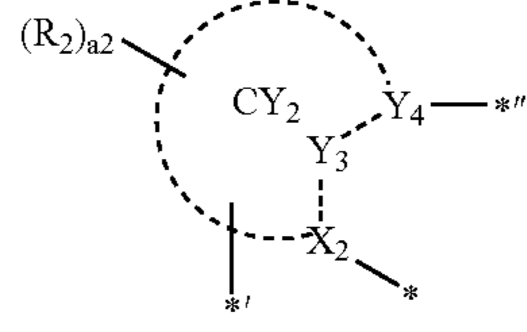
35 Formula A2-3
