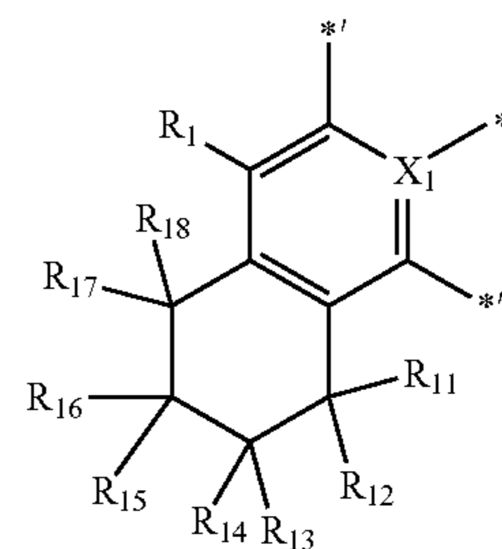
Formula A1-1(1)
