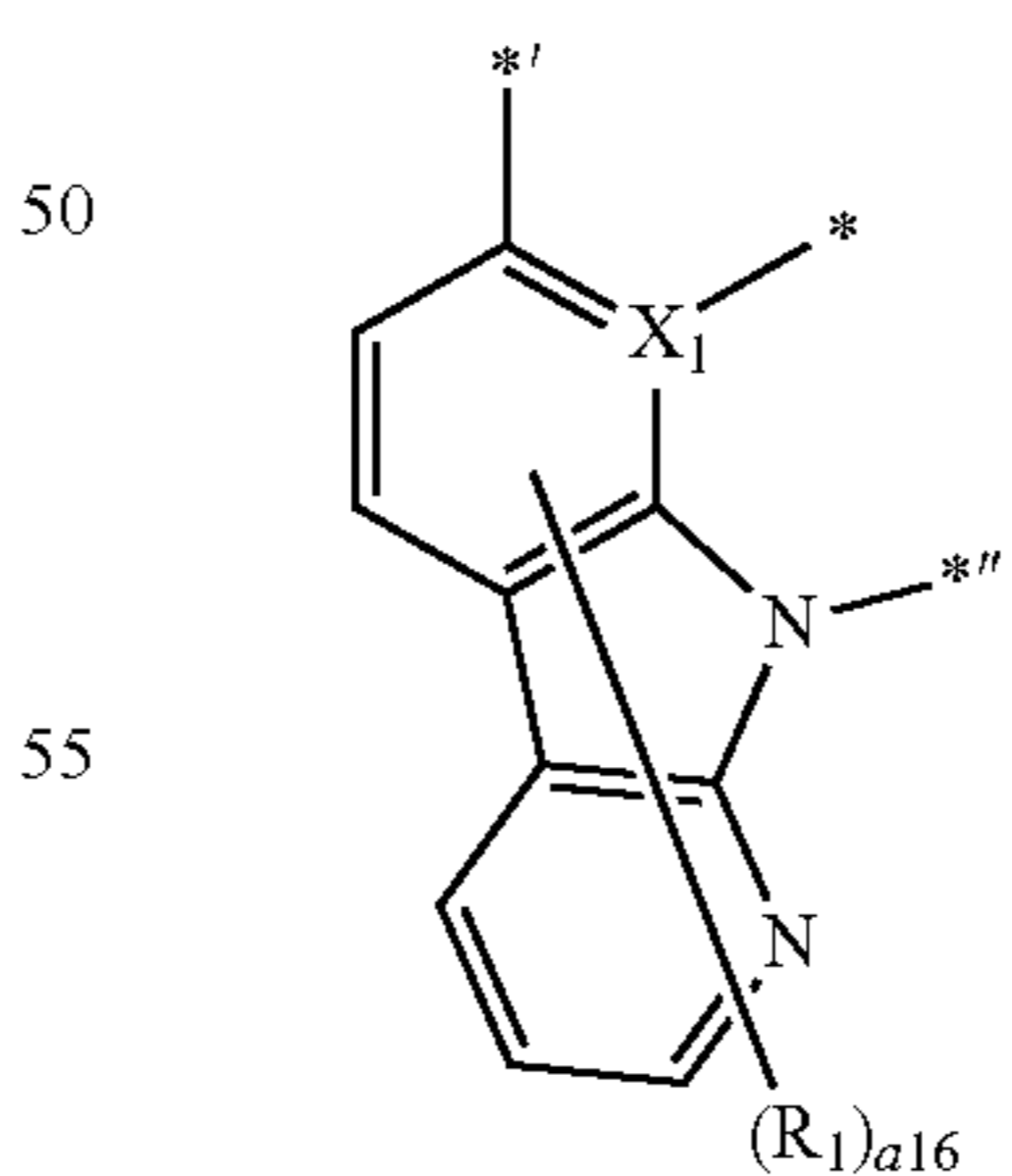
Formula A1-3(53)
