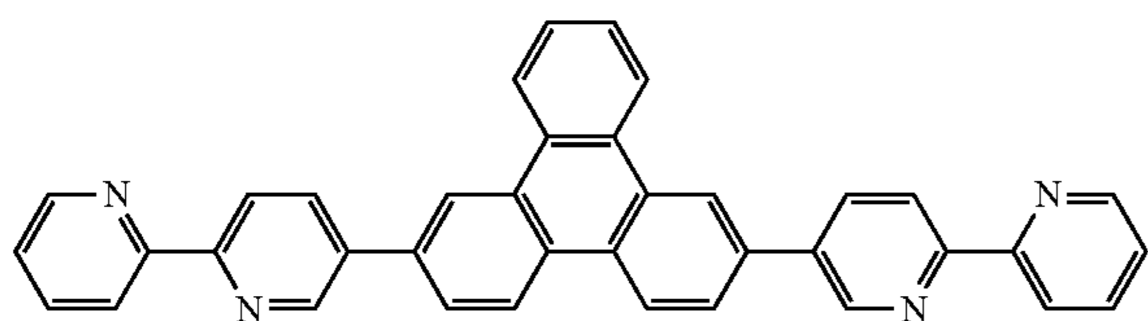
(Compound 3)
