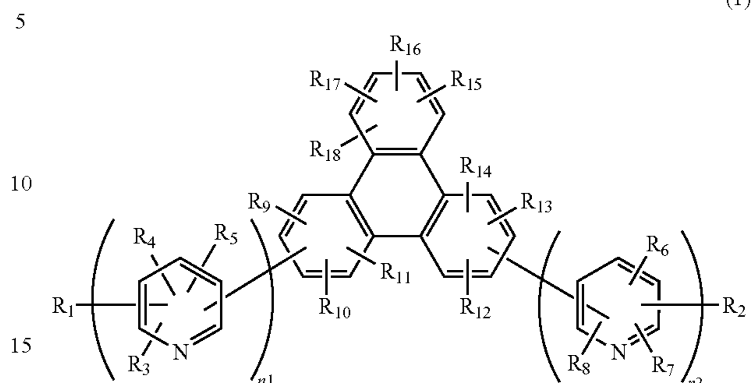
[Chemical Formula 1]
