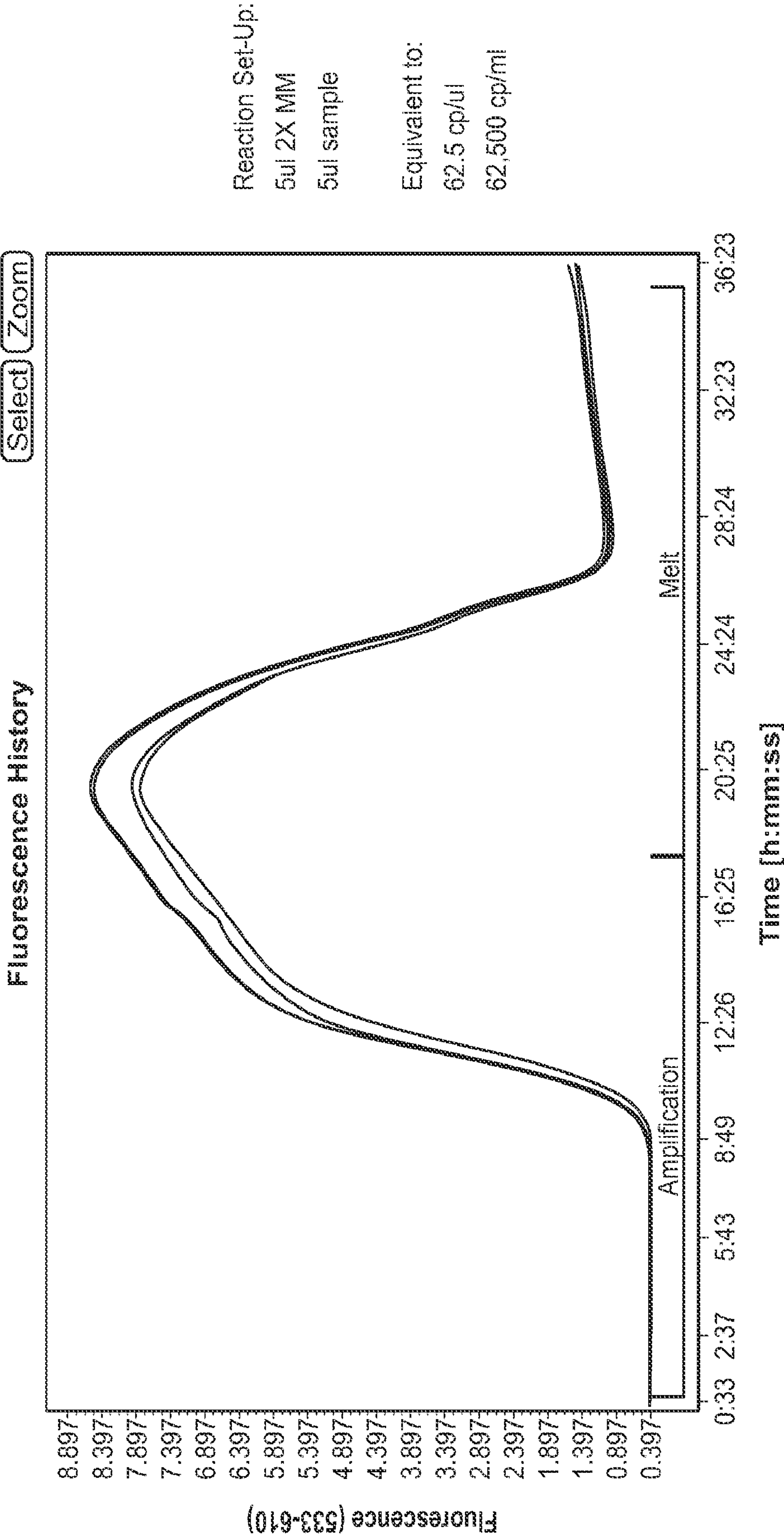
FIG. 3R 312 Copies gBlock in 18 ng Human cDNA Assay 2
