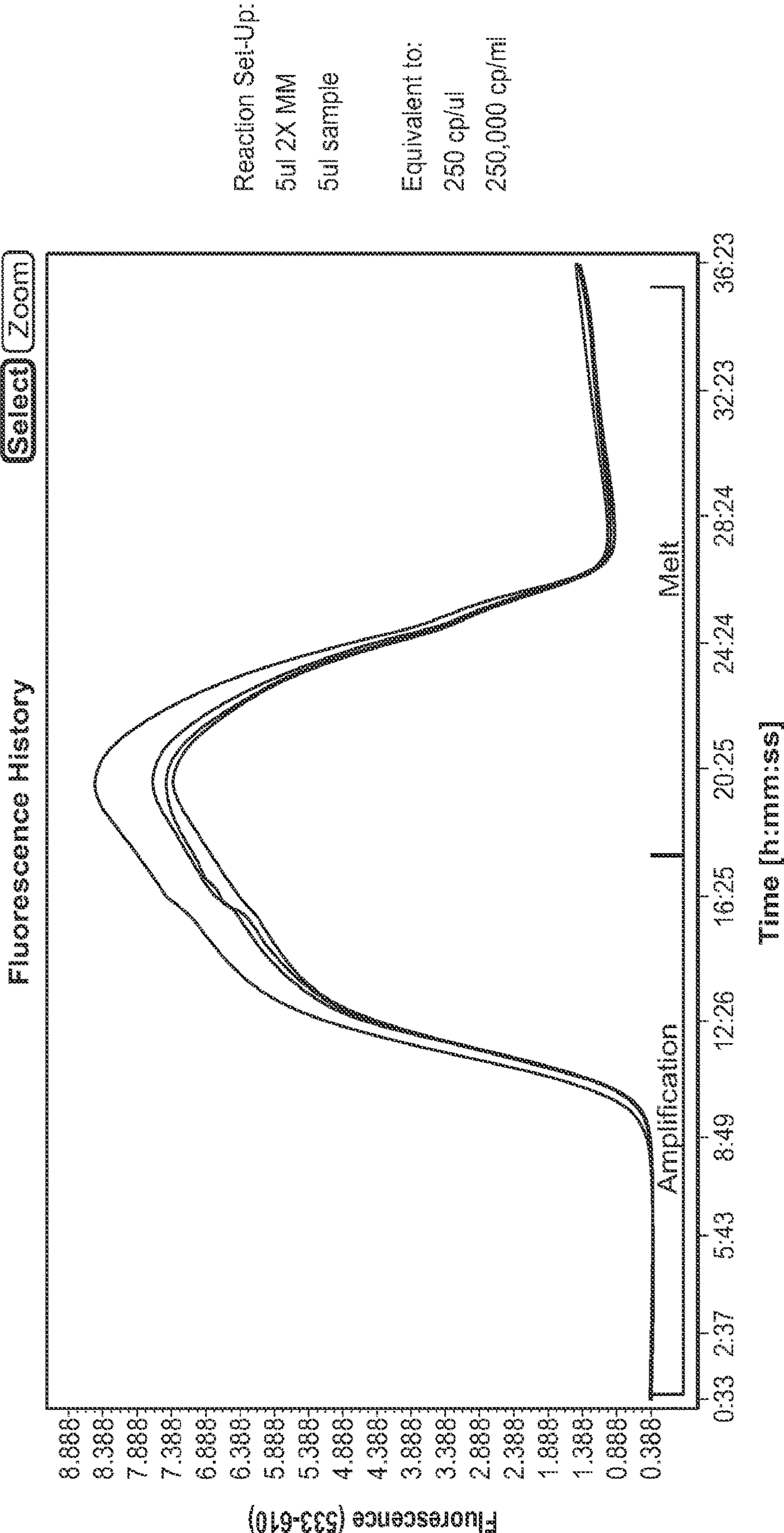
FIG. 3P 1.25K Copies gBlock in 18 ng Human cDNA Assay 2
