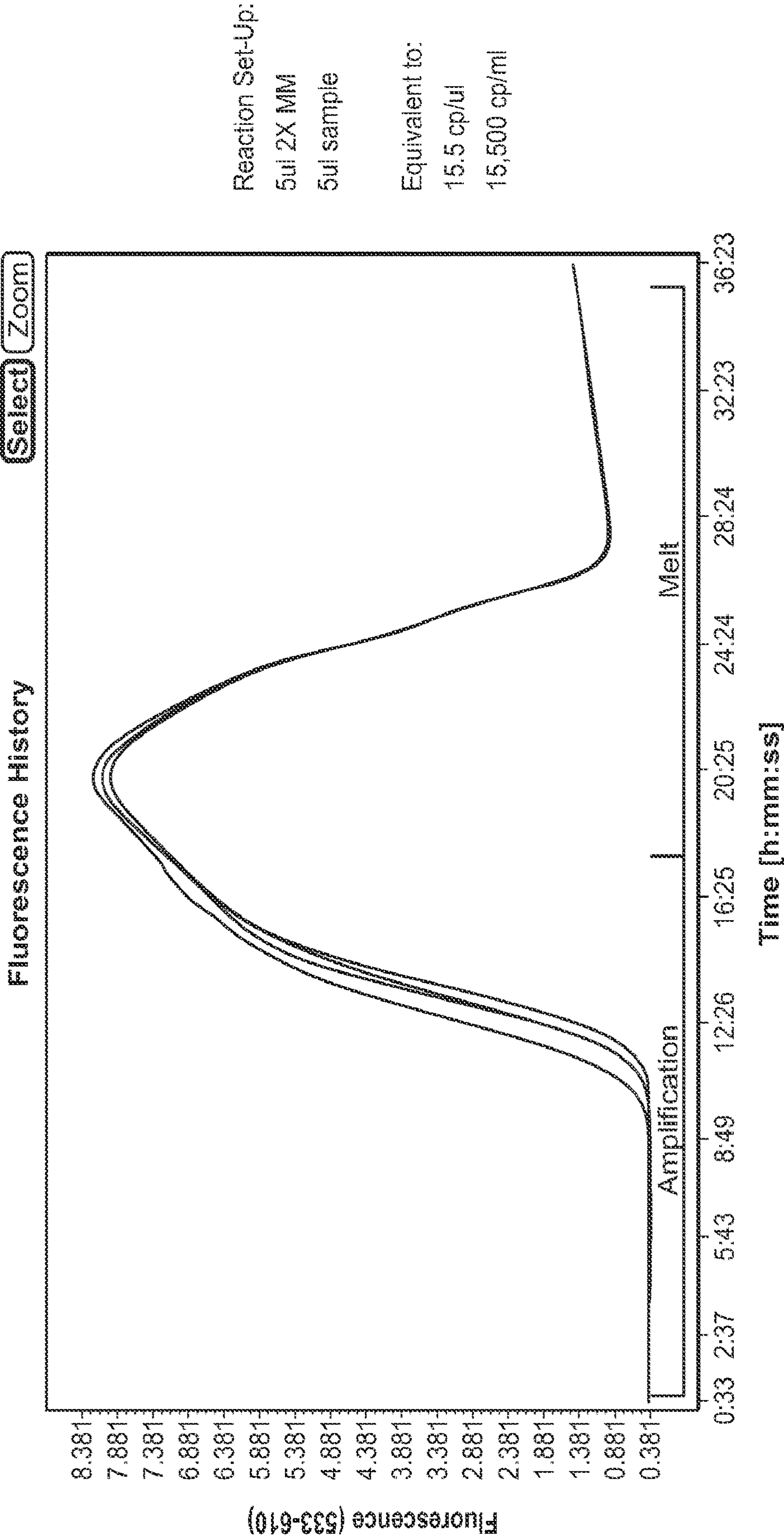
78 Copies gBlock in 18 ng Human cDNA Assay 2
