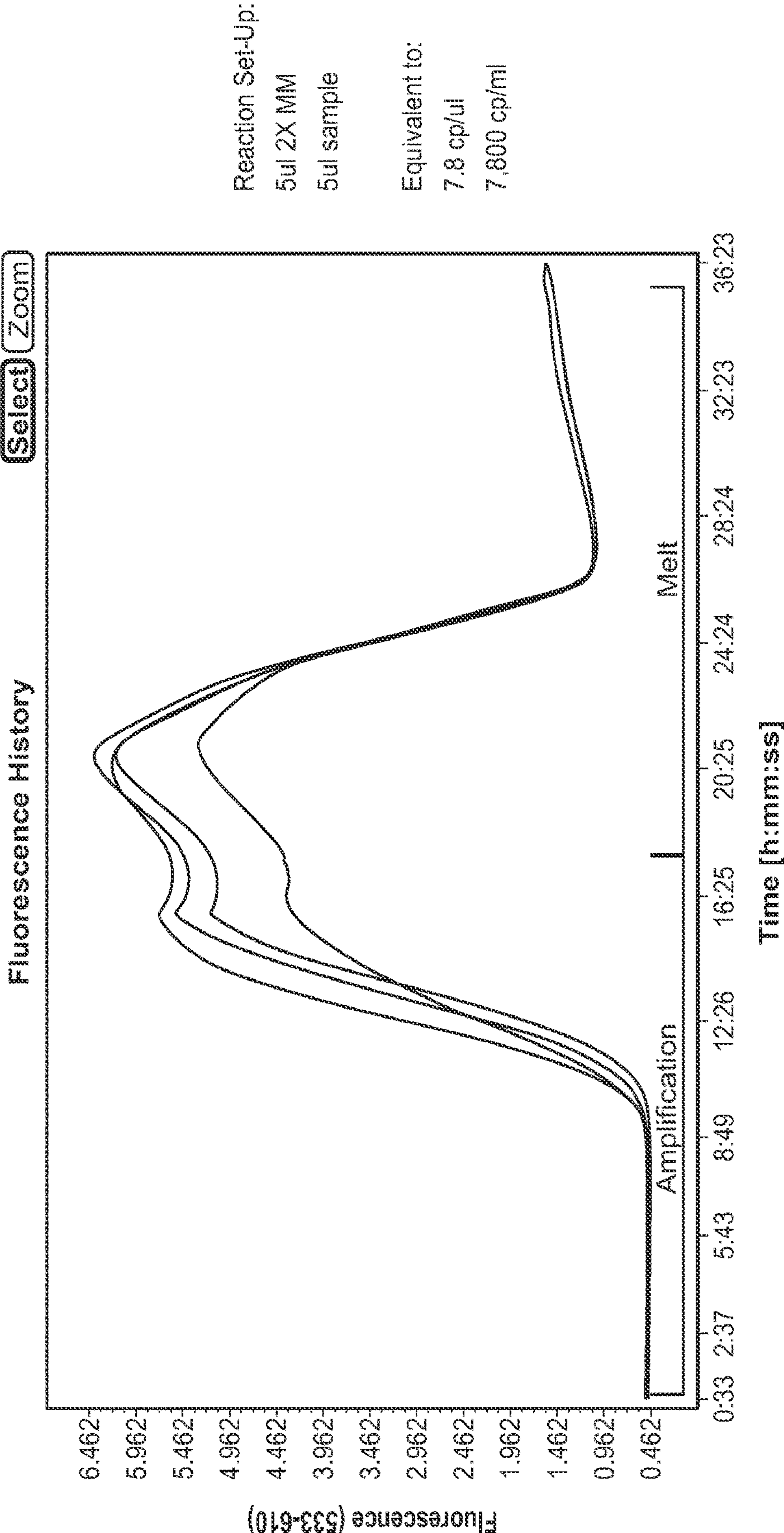
FIG. 3 39 Copies gBlock in 18 ng Human cDNA Assay 1
