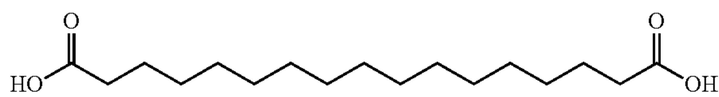
Heptadecanedioic acid
