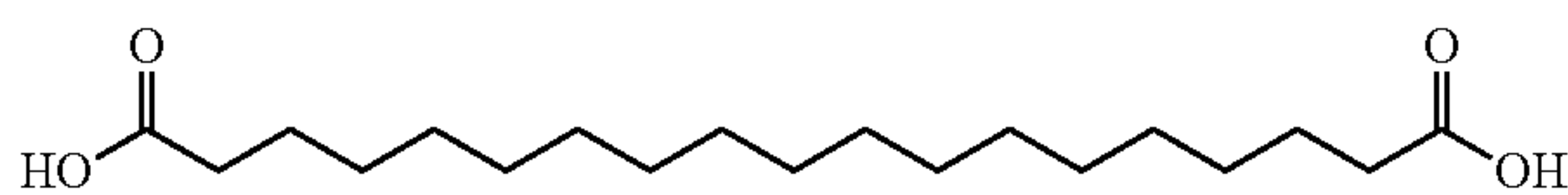
Nonadecanedioic acid
