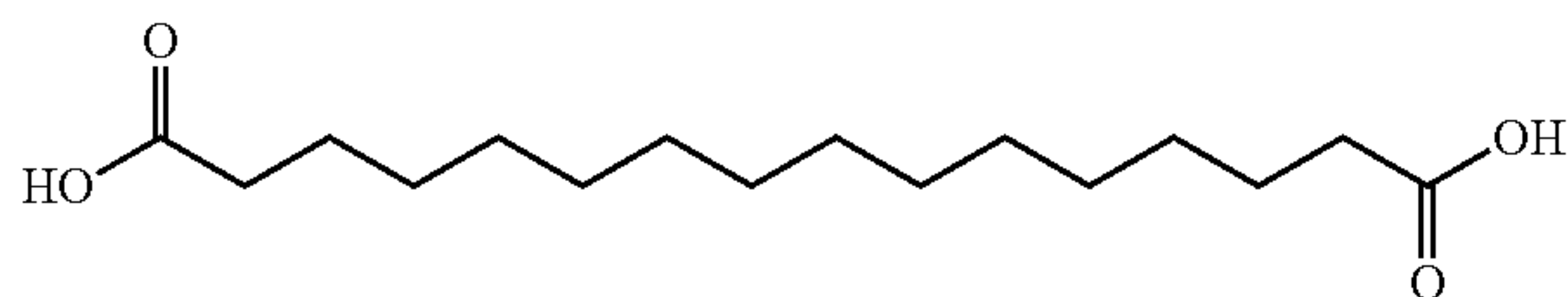
Hexadecanedioic acid
