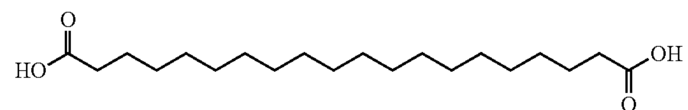
Eicosanedioic acid
