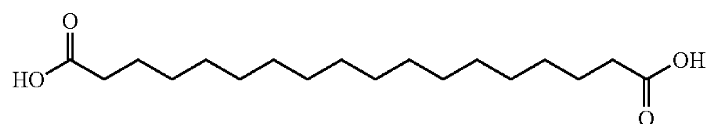
Octadecanedioic acid
