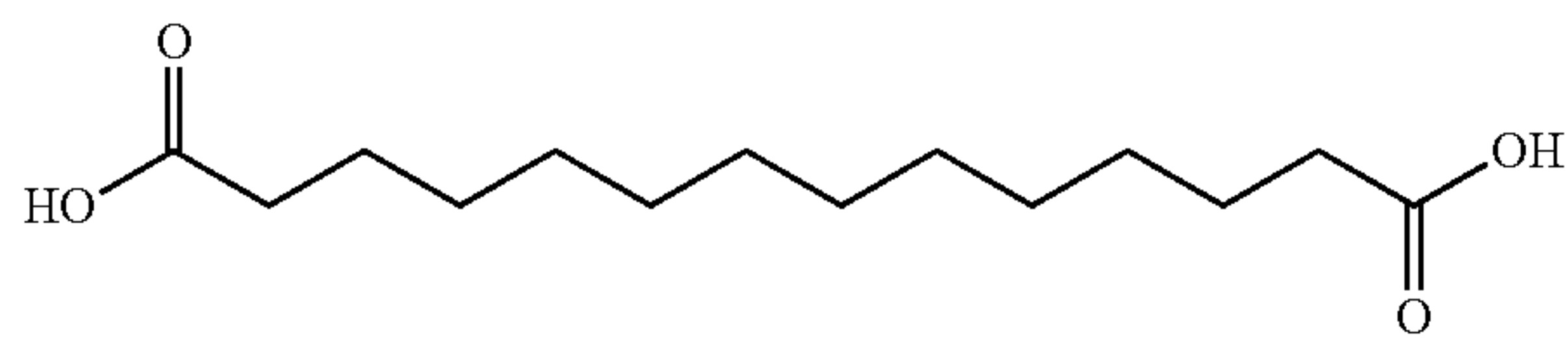
Tetradecanedioic acid
