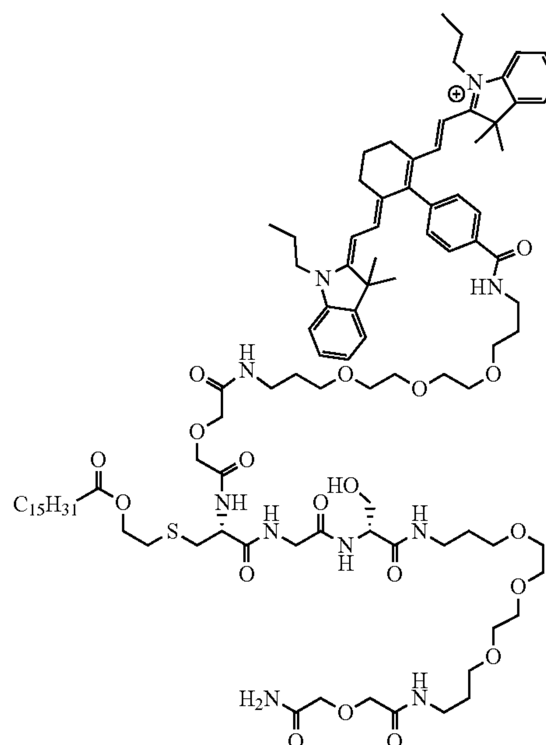
Compound 16 (which contains an IR780 dye moiety)
