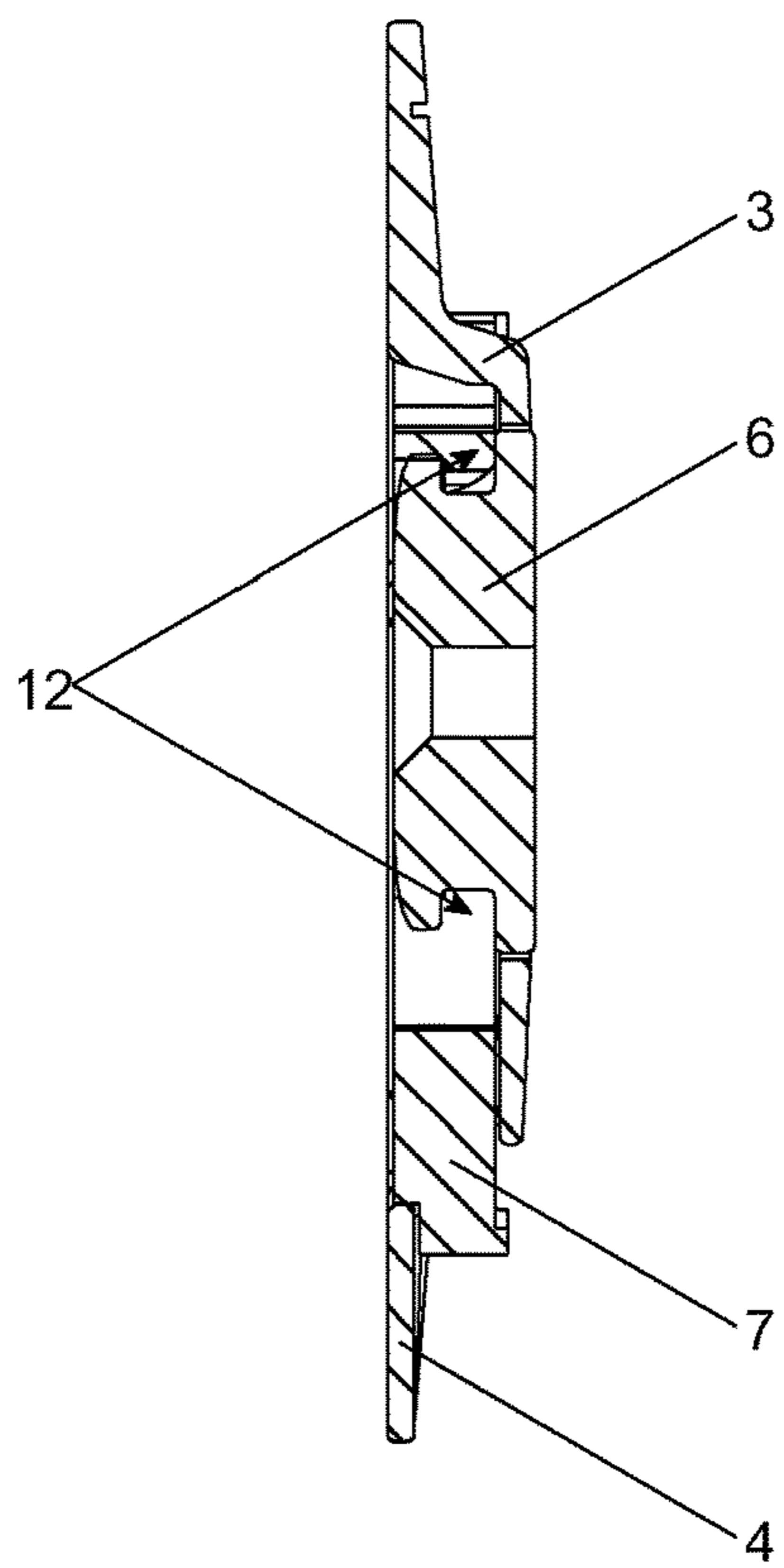
SECTION B-B
