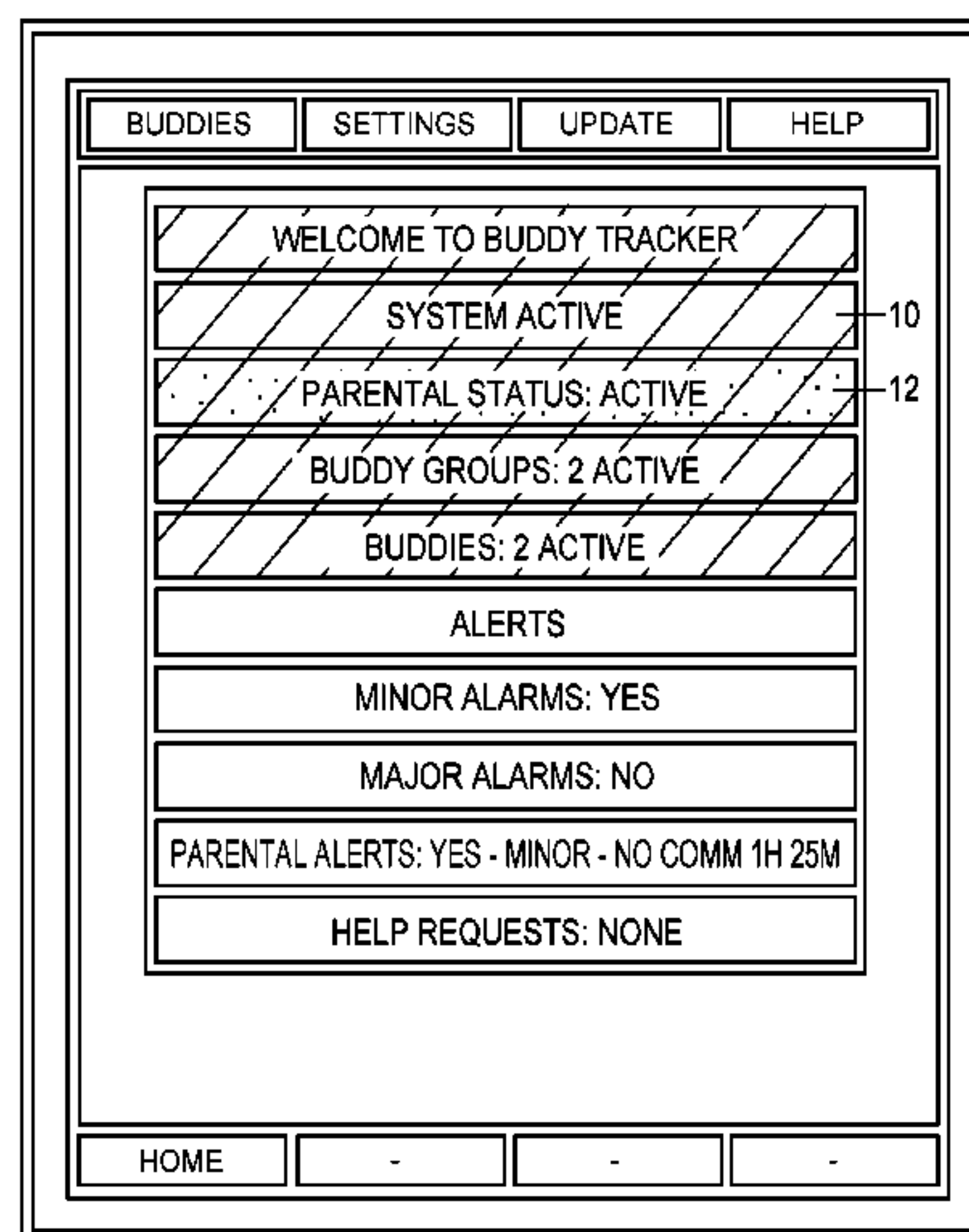
OPENING SCREEN
