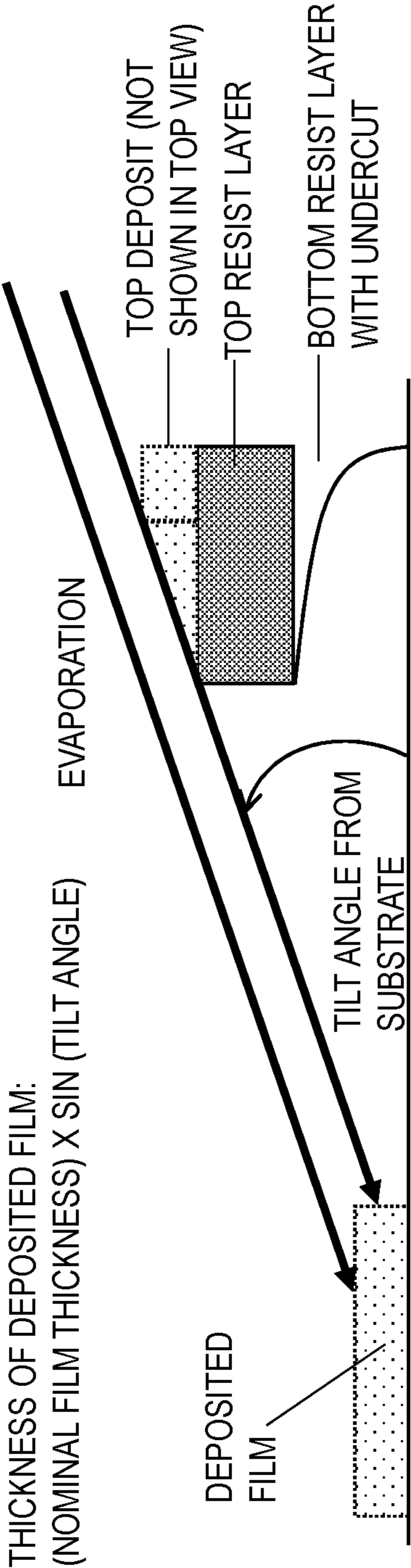
FIG. 31 CROSS-SECTION A
