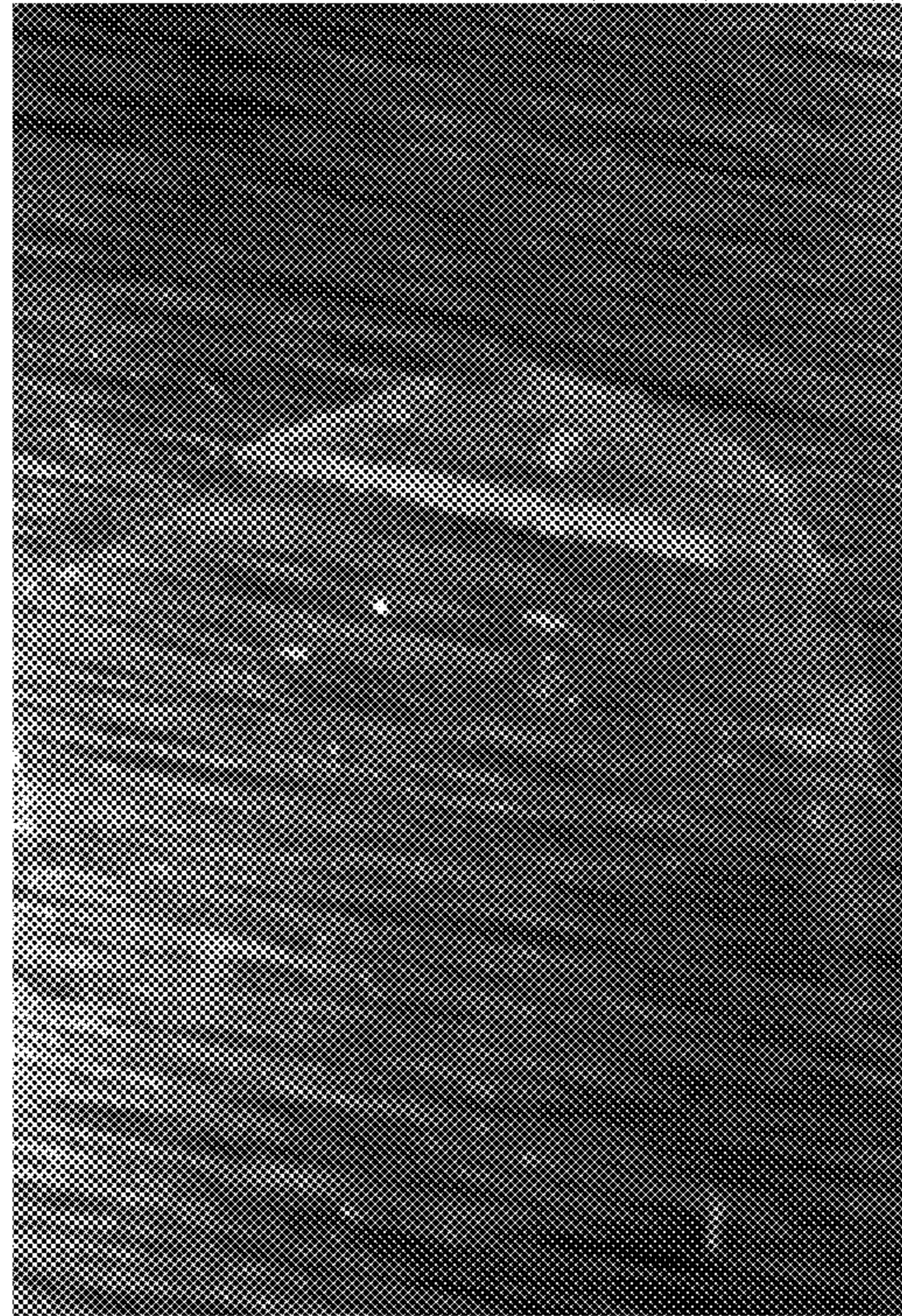
Non-reactive surfactant
