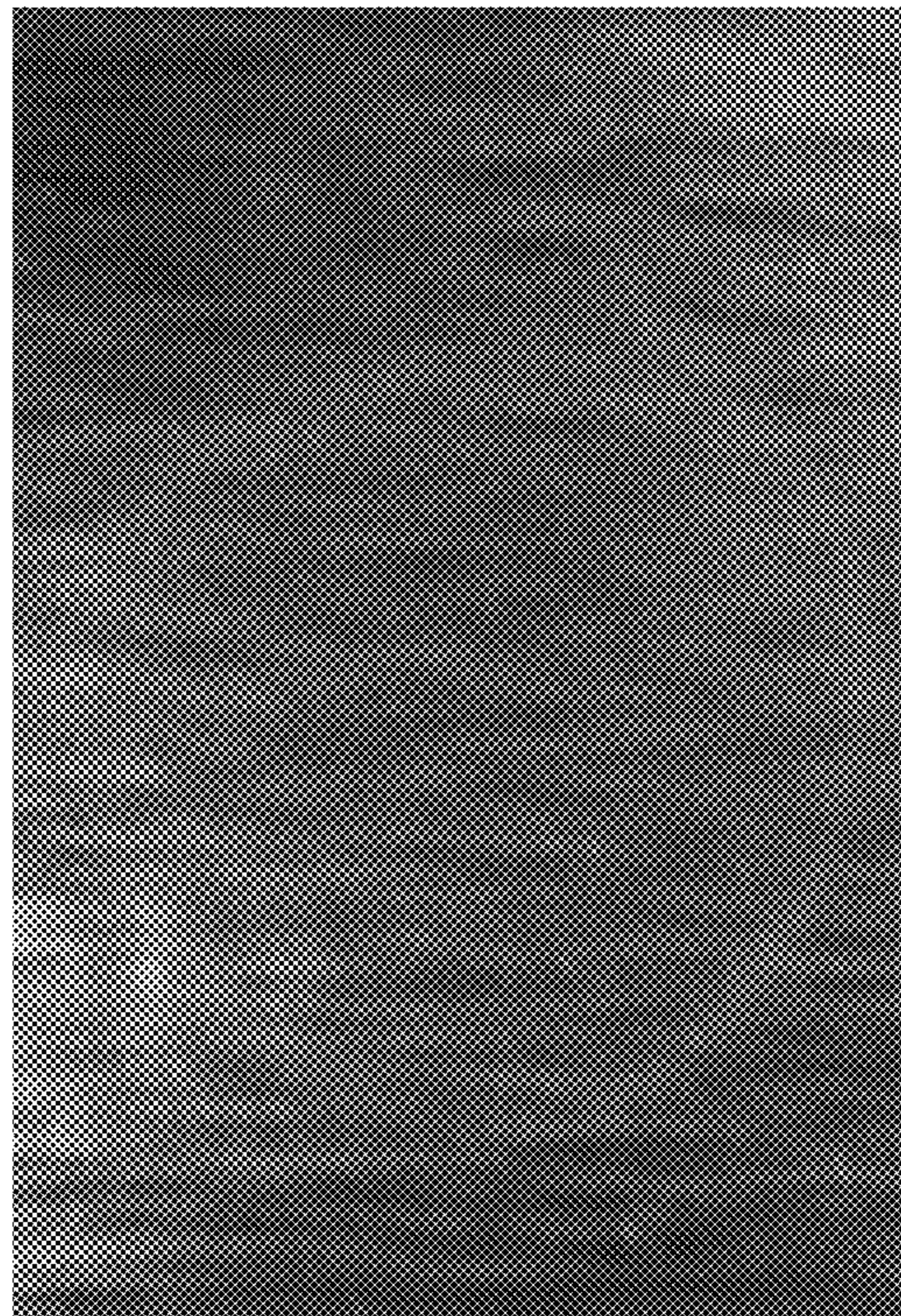
Reactive surfactant
