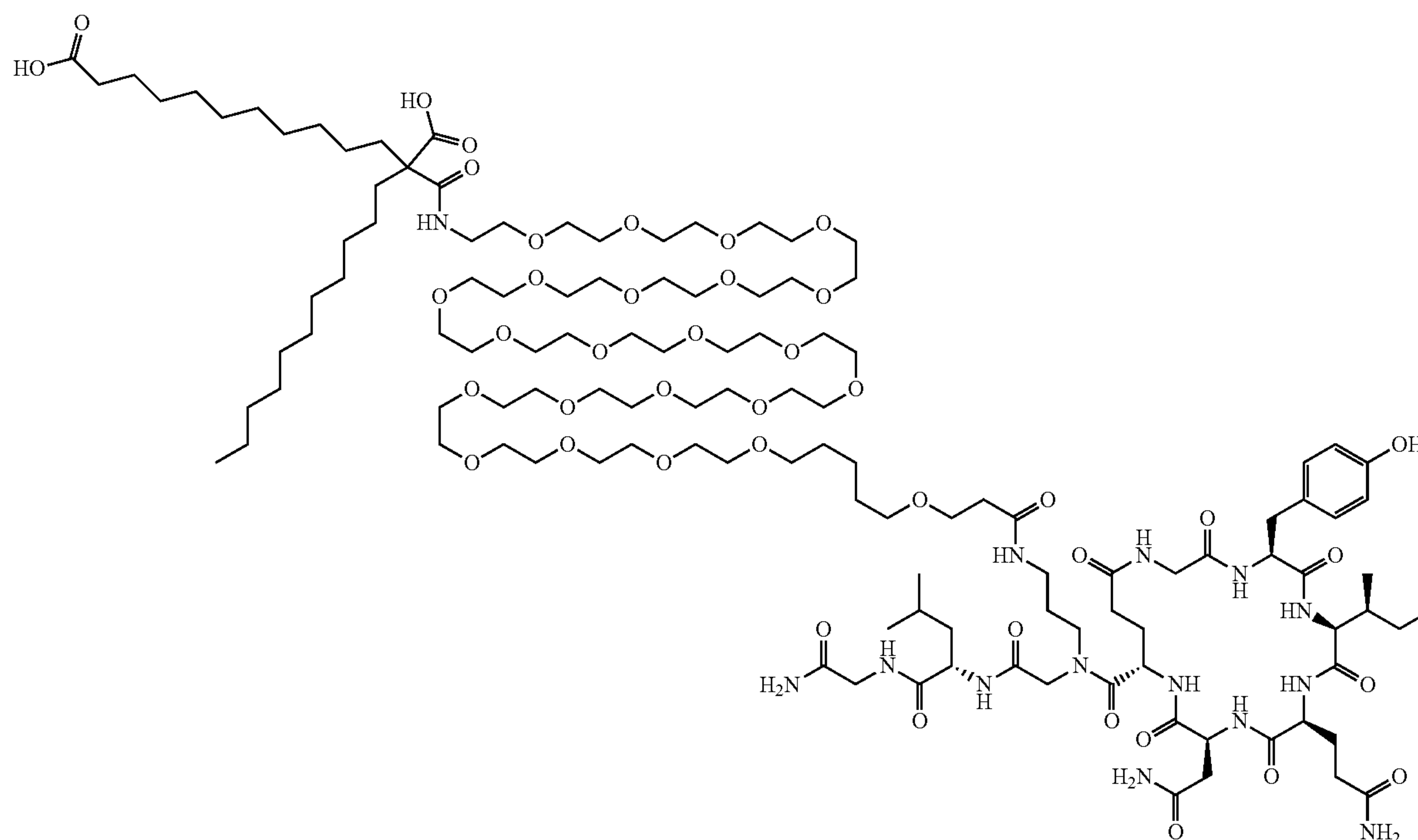
Oxytocin FA Conjugate
