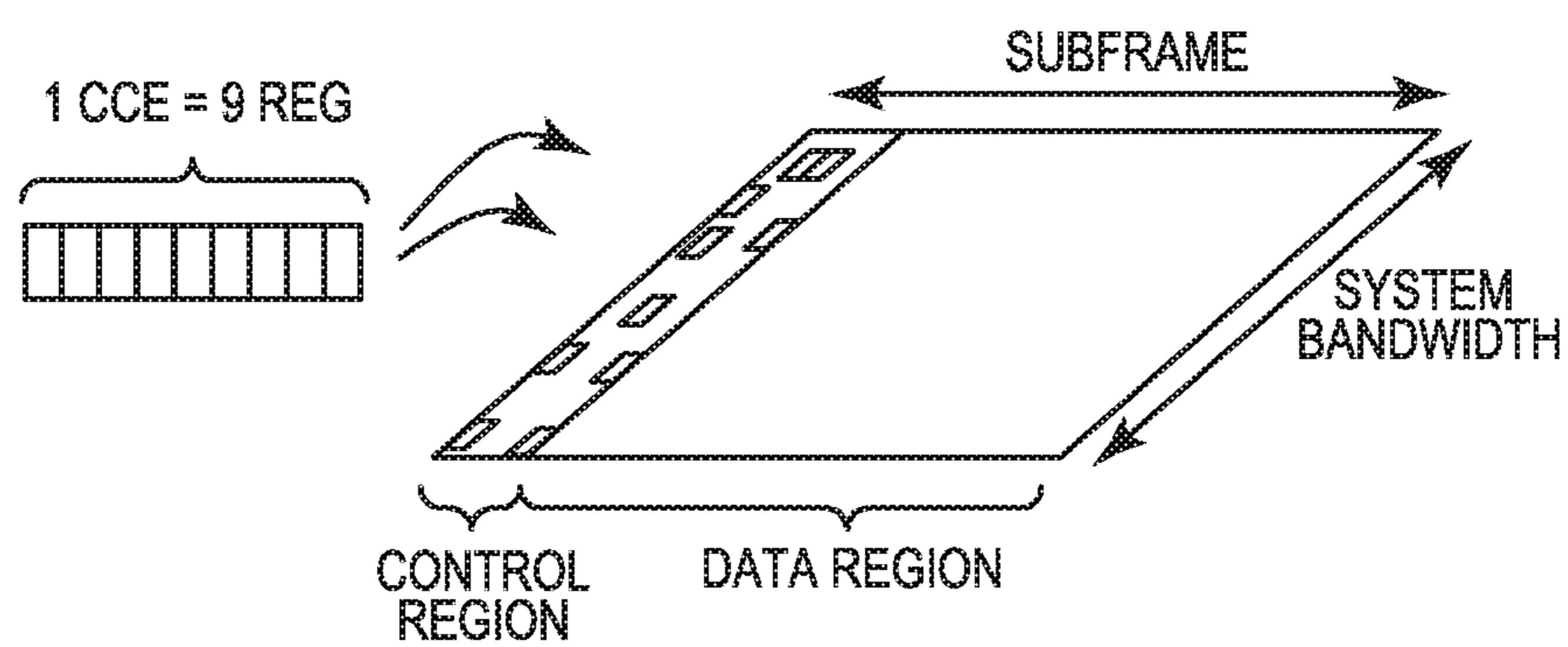
FIG. 4 (PRIOR ART)
