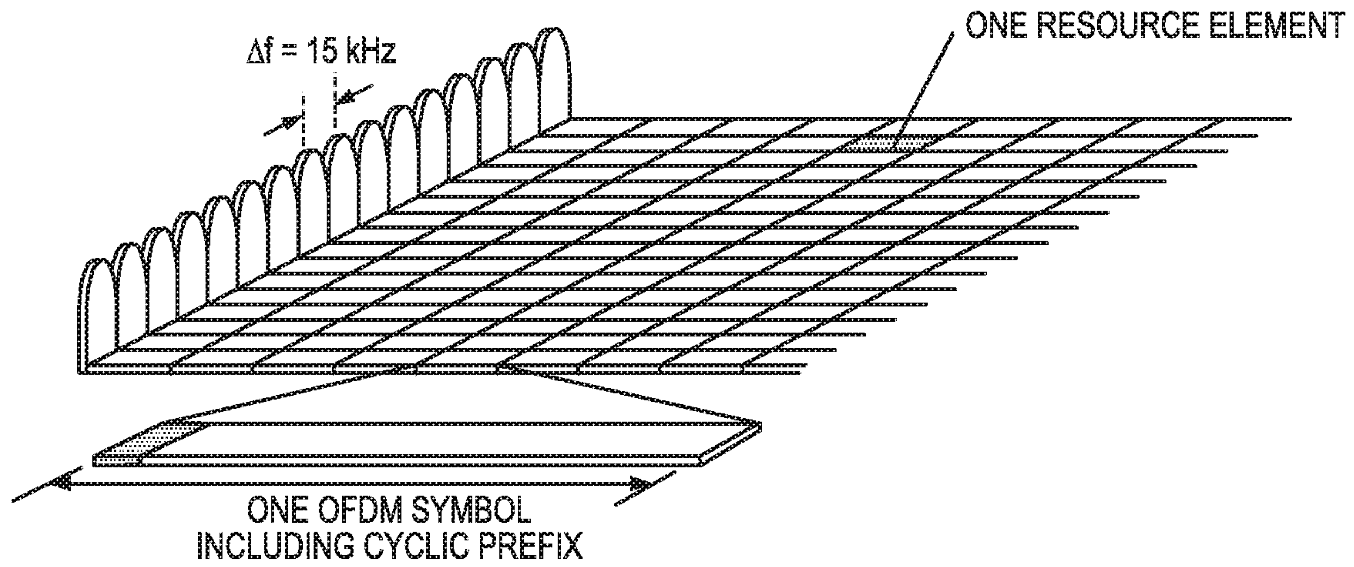
FIG. 1 (PRIOR ART)
