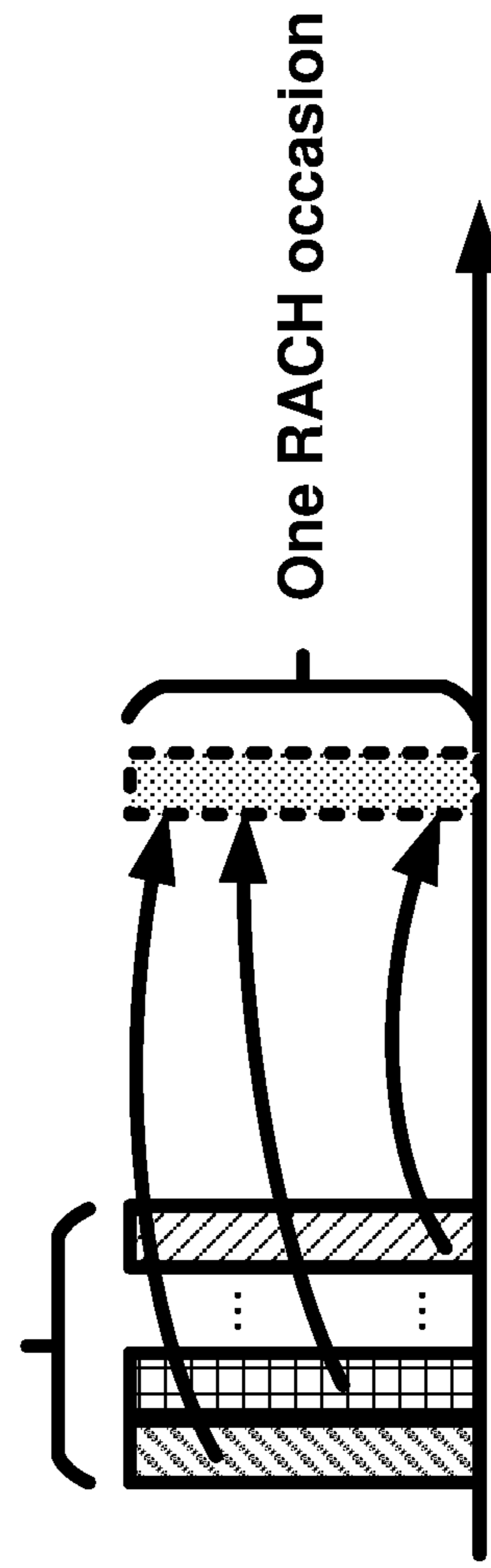
FIG. 20C multi-to-one mapping
