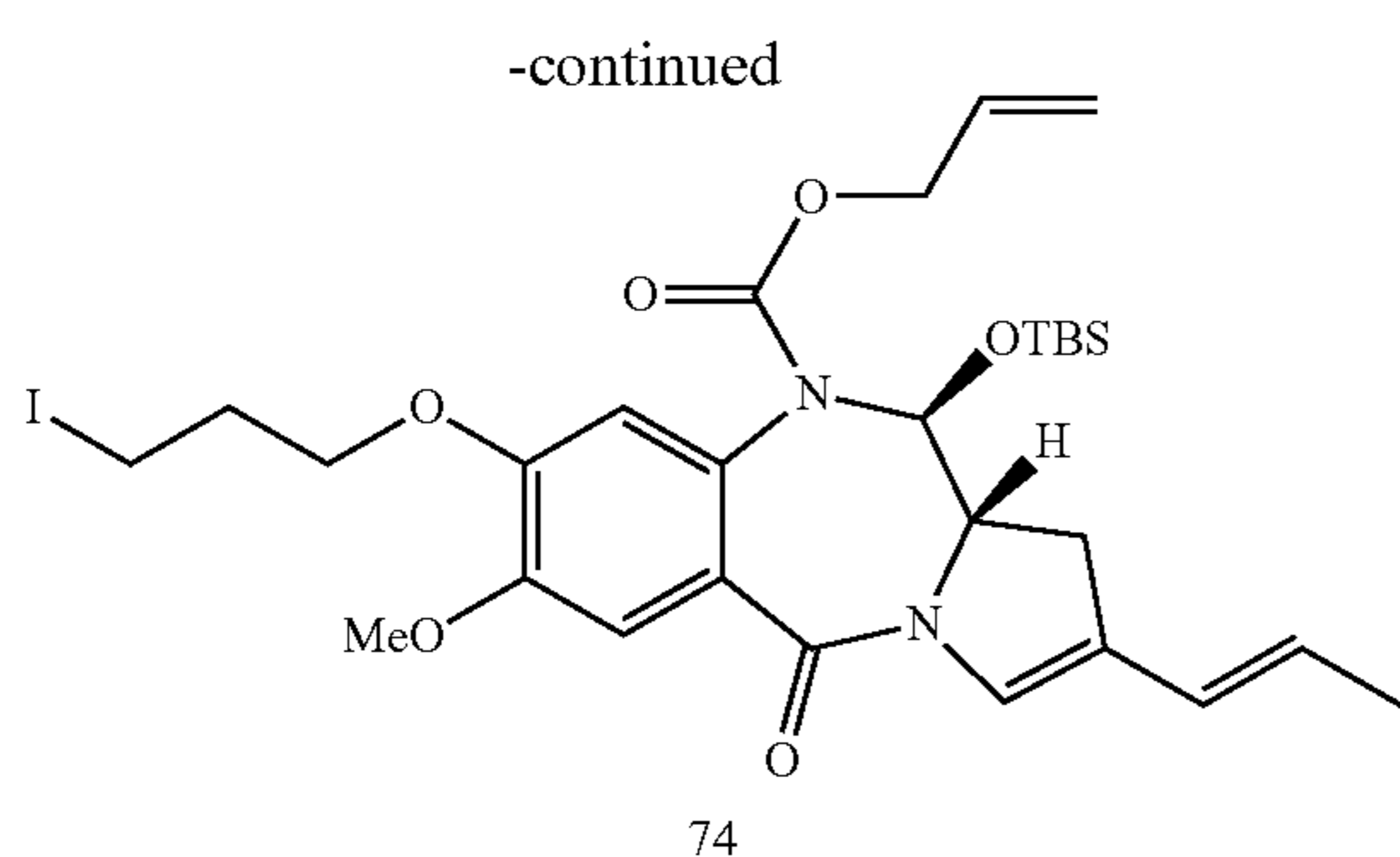
(a) (S)-5-((tert-butyldimethylsilyloxy)methyl)-1-(5-methoxy-2-nitro-4-(triisopropylsilyloxy)benzoyl)-4,5-dihydro-1H-pyrrol-3-yl trifluoromethanesulfonate (47)
