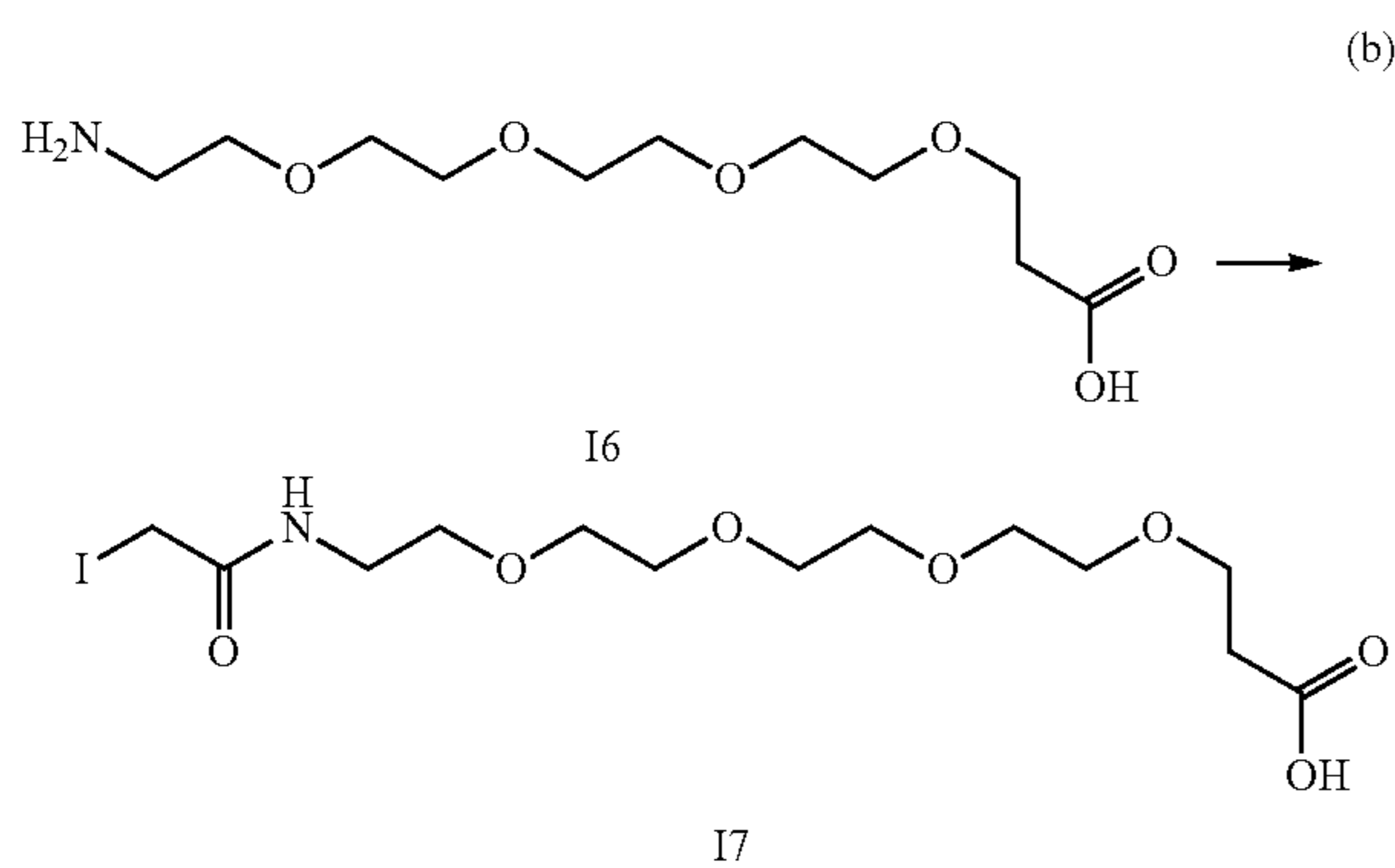
1-iodo-2-oxo-6,9,12,15-tetraoxa-3-azaoctadecan-18-oic acid (17)
