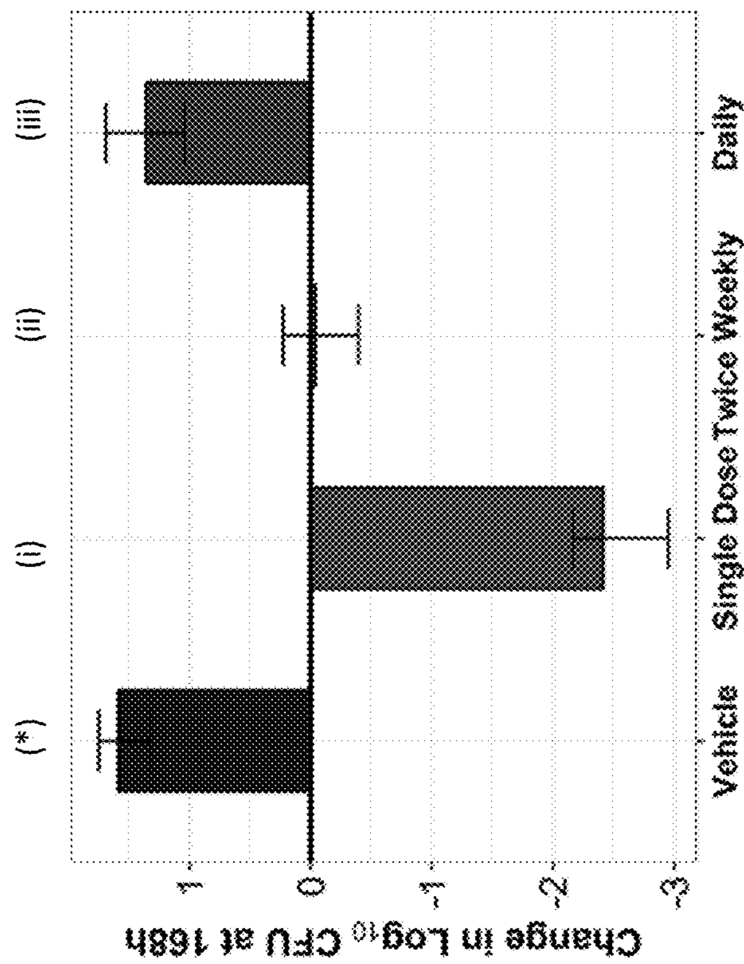
FIG. 6 Mean (bar) and range (error bars) change in \log_{10} CFU from baseline allowing administration of Compound 1 2 mg/kg grouped by fractionation schedule
