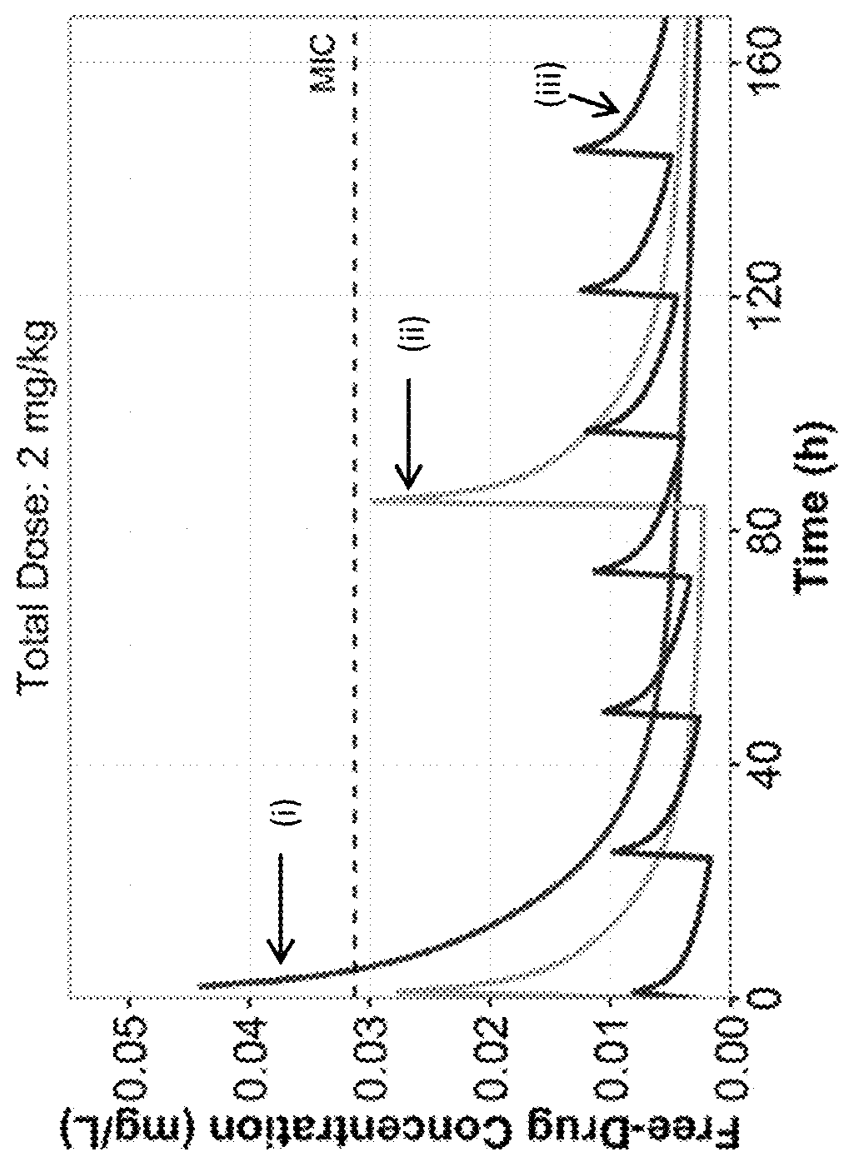
FIG. 7 Simulated free-drug concentration time profiles relative to the MIC for the fractionated Compound 1 2 mg/kg regimen
