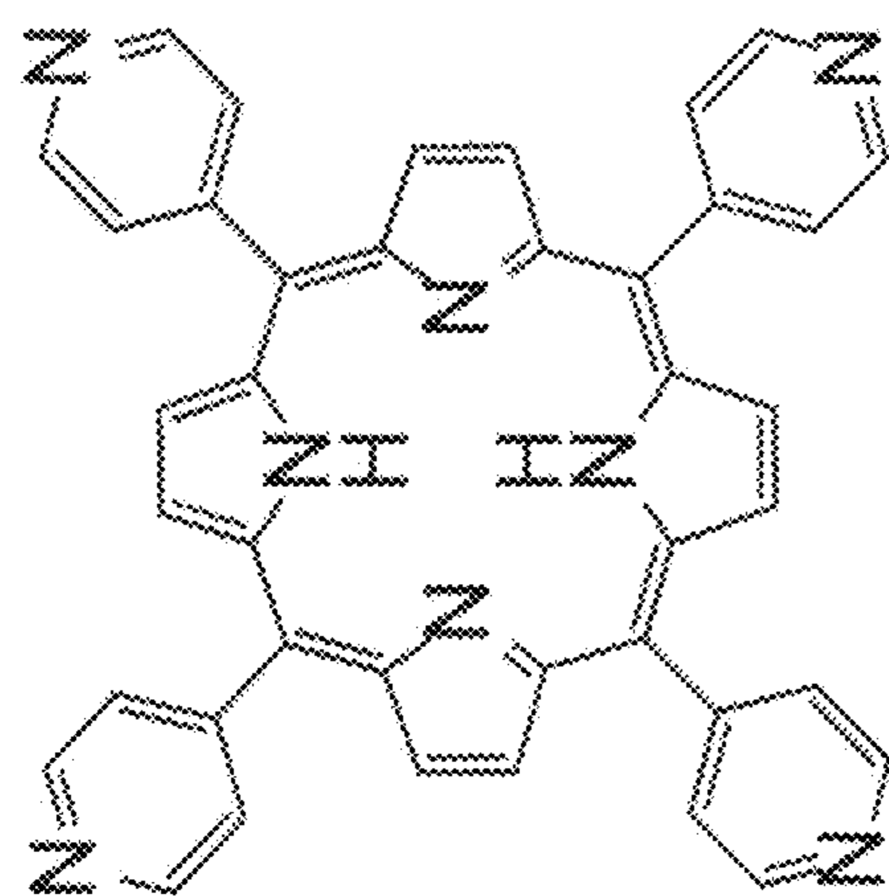
5,10,15,20-tetra(p-pyridyl)porphyrin
