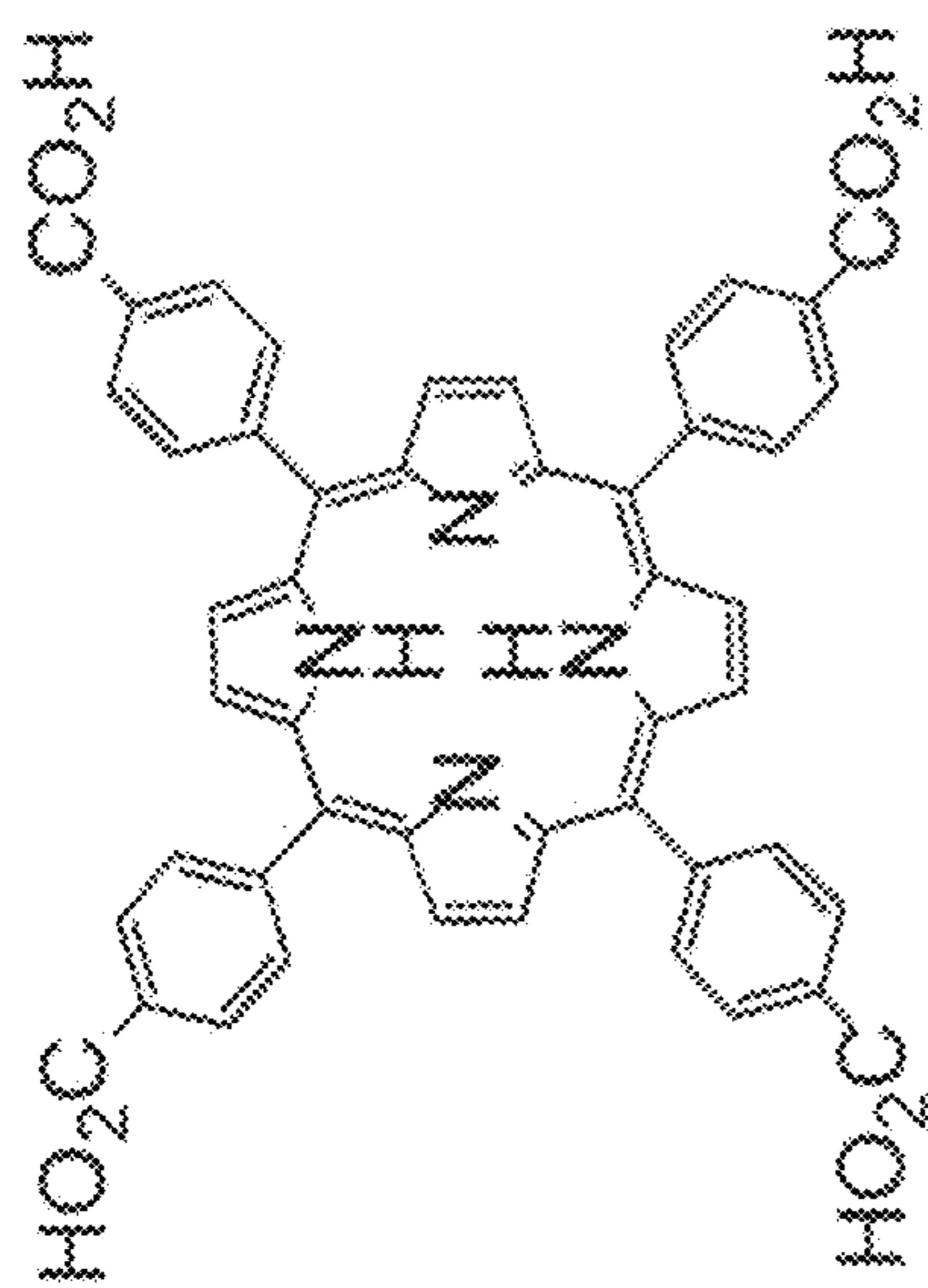
5,10,15,20-tetra(p-carboxyphenyl)porphyrin
