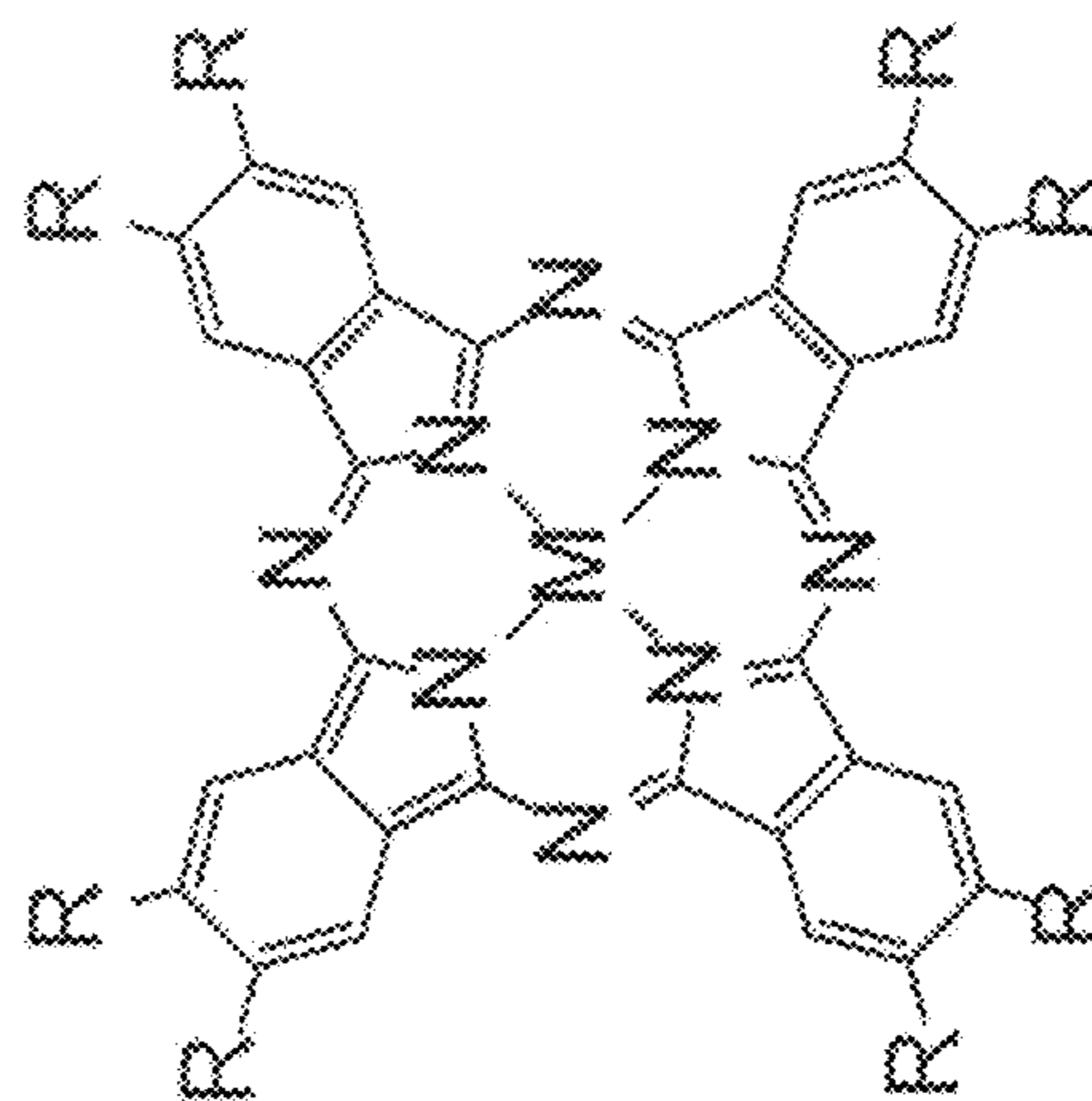
5,10,15,20-tetra(p-pyridyl)porphyrin
