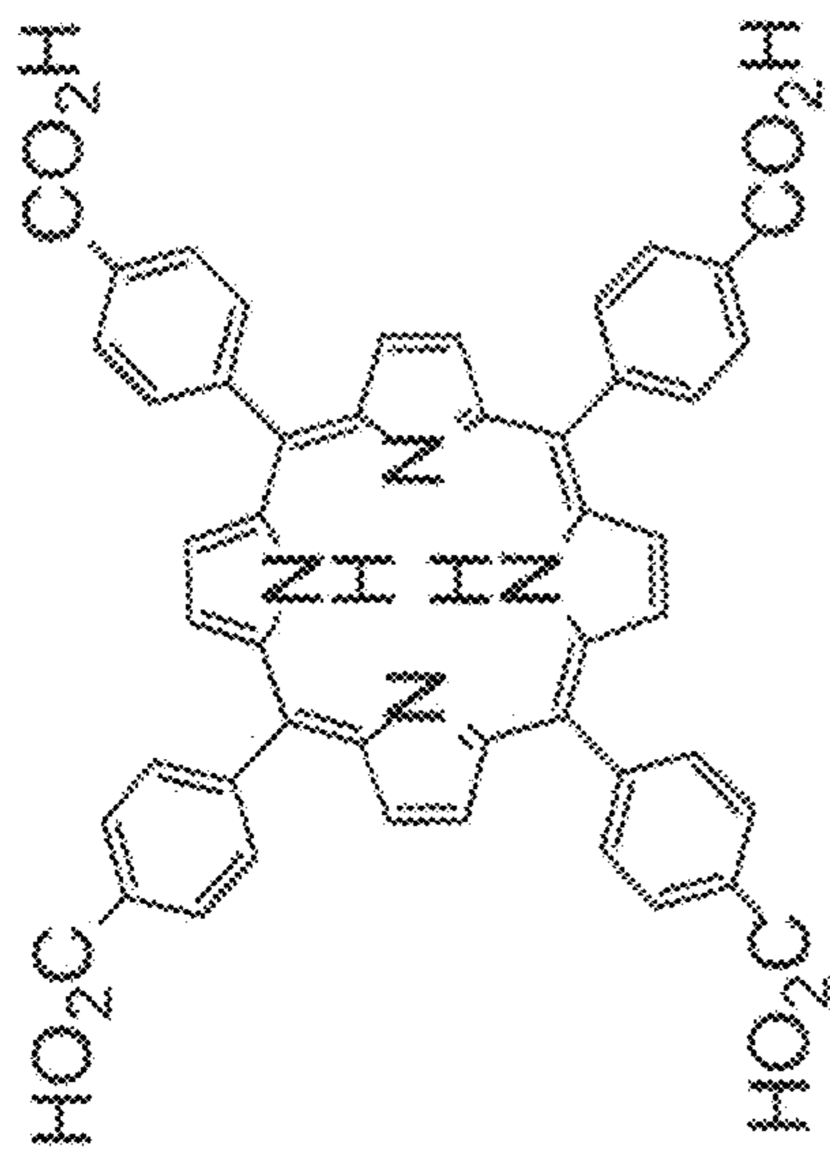
5,10,15,20-tetra(p-carboxyphenyl)porphyrin
