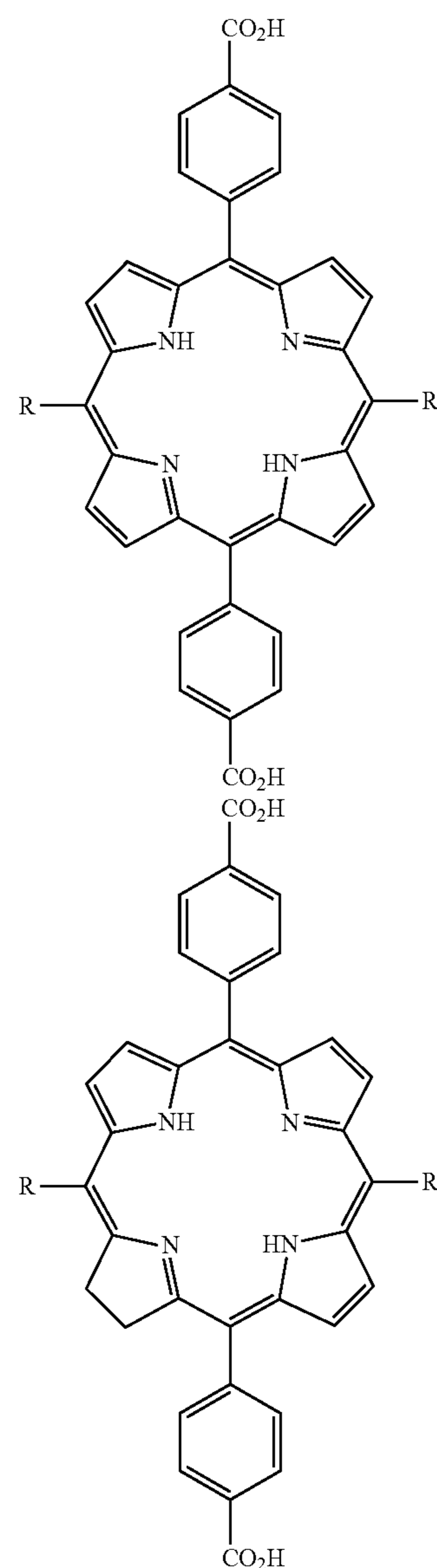
Scheme 1. Exemplary DBP, DBC, and DBBC ligands.
