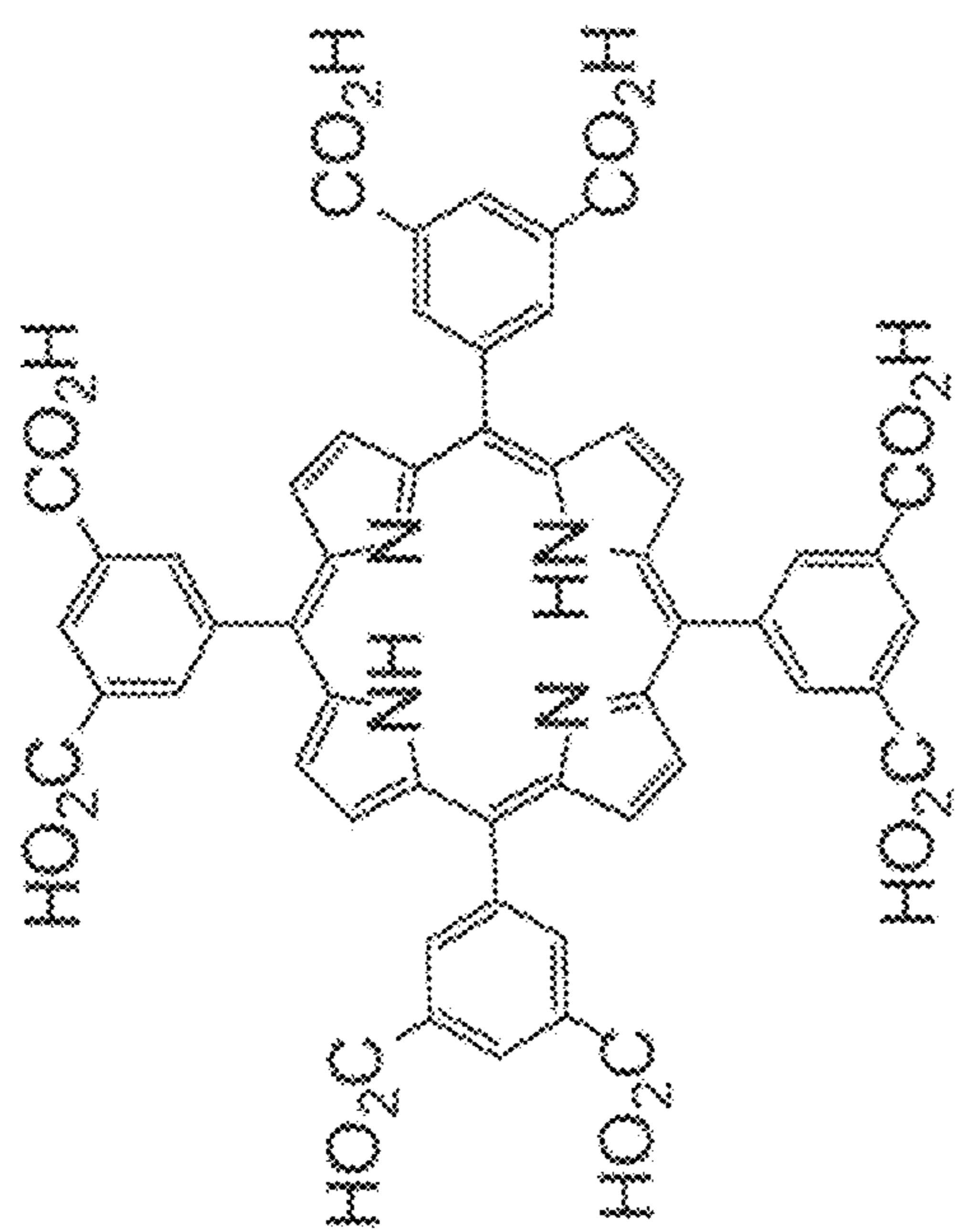
5,10,15,20-tetra(3',5'-dicarboxylphenyl)porphyrin
