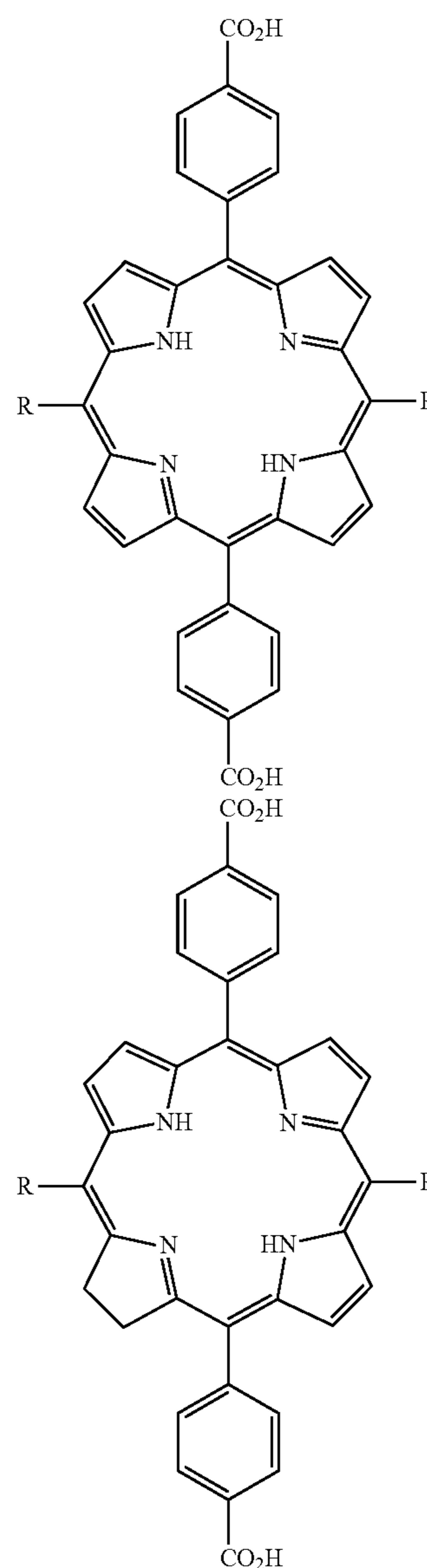
Scheme 1. Exemplary DBP, DBC, and DBBC ligands.
