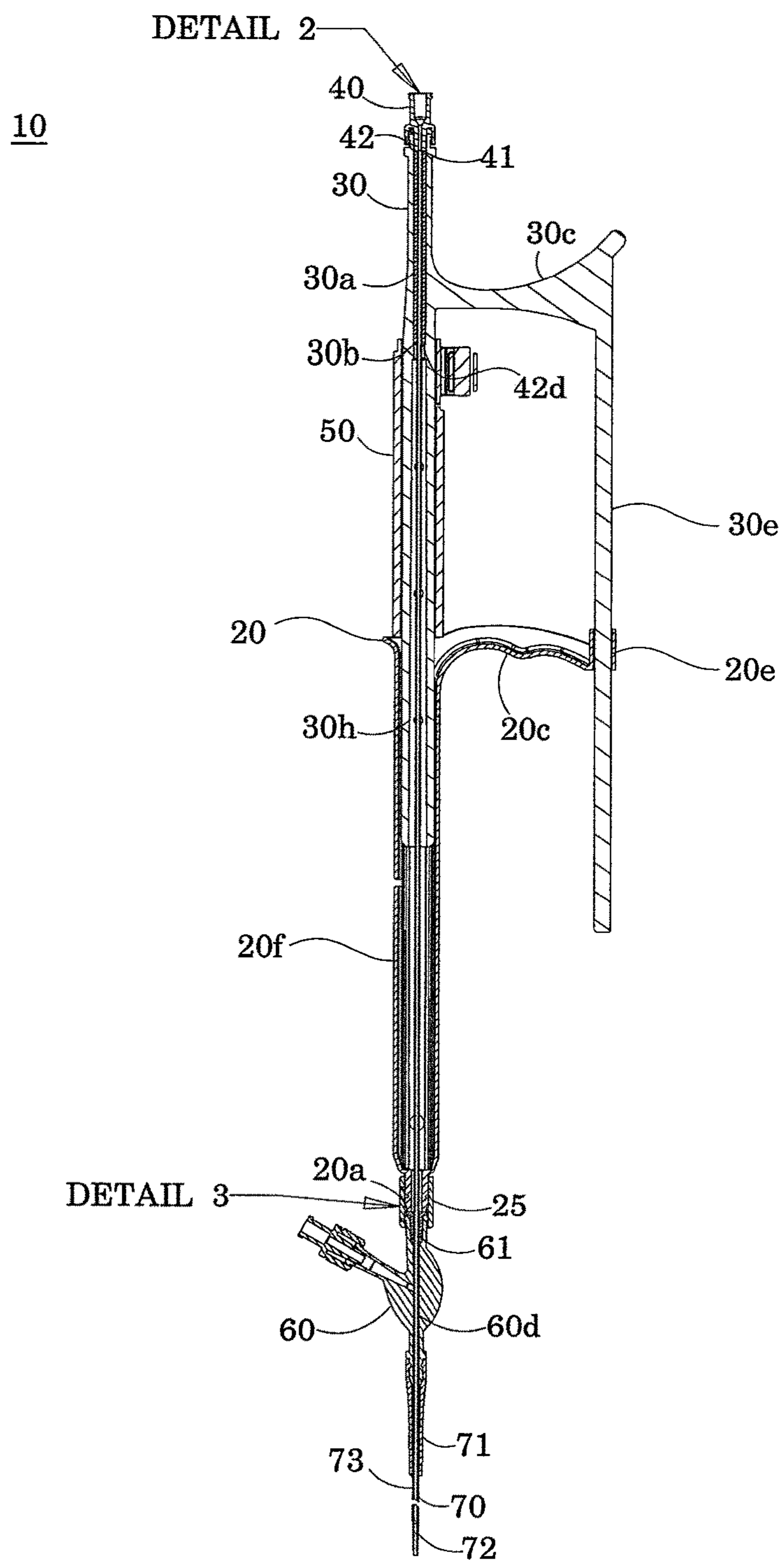
SECTION 1-1 FIG. 2B
