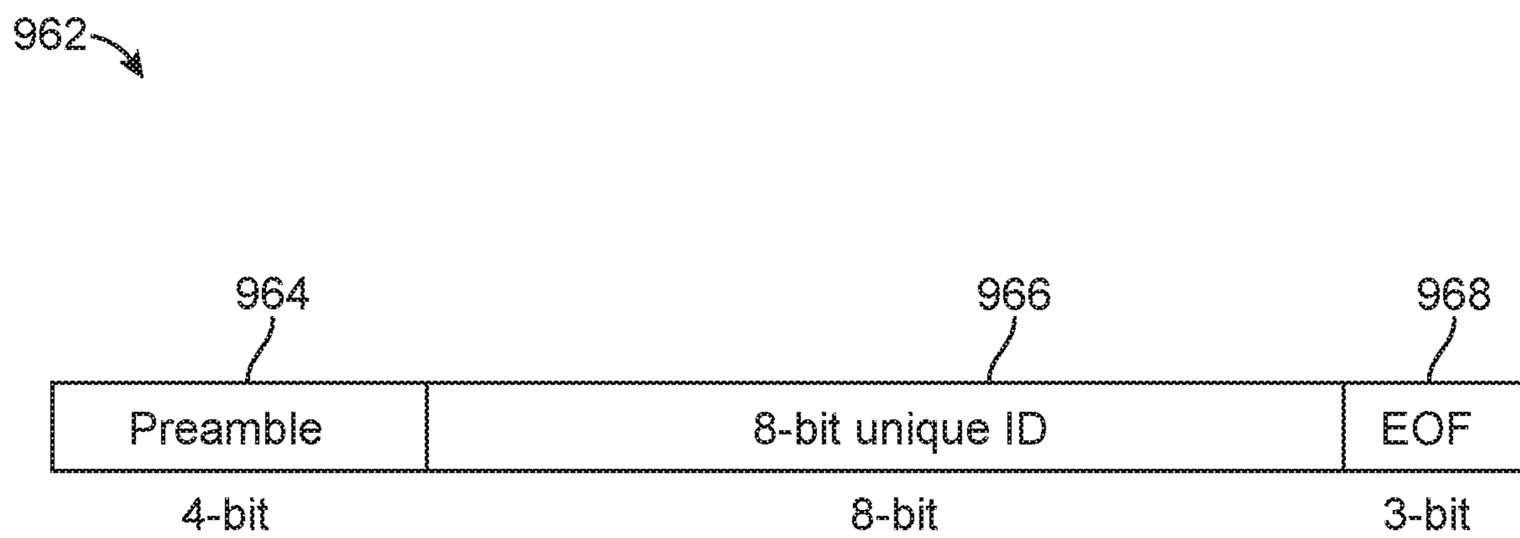
Packet structure
