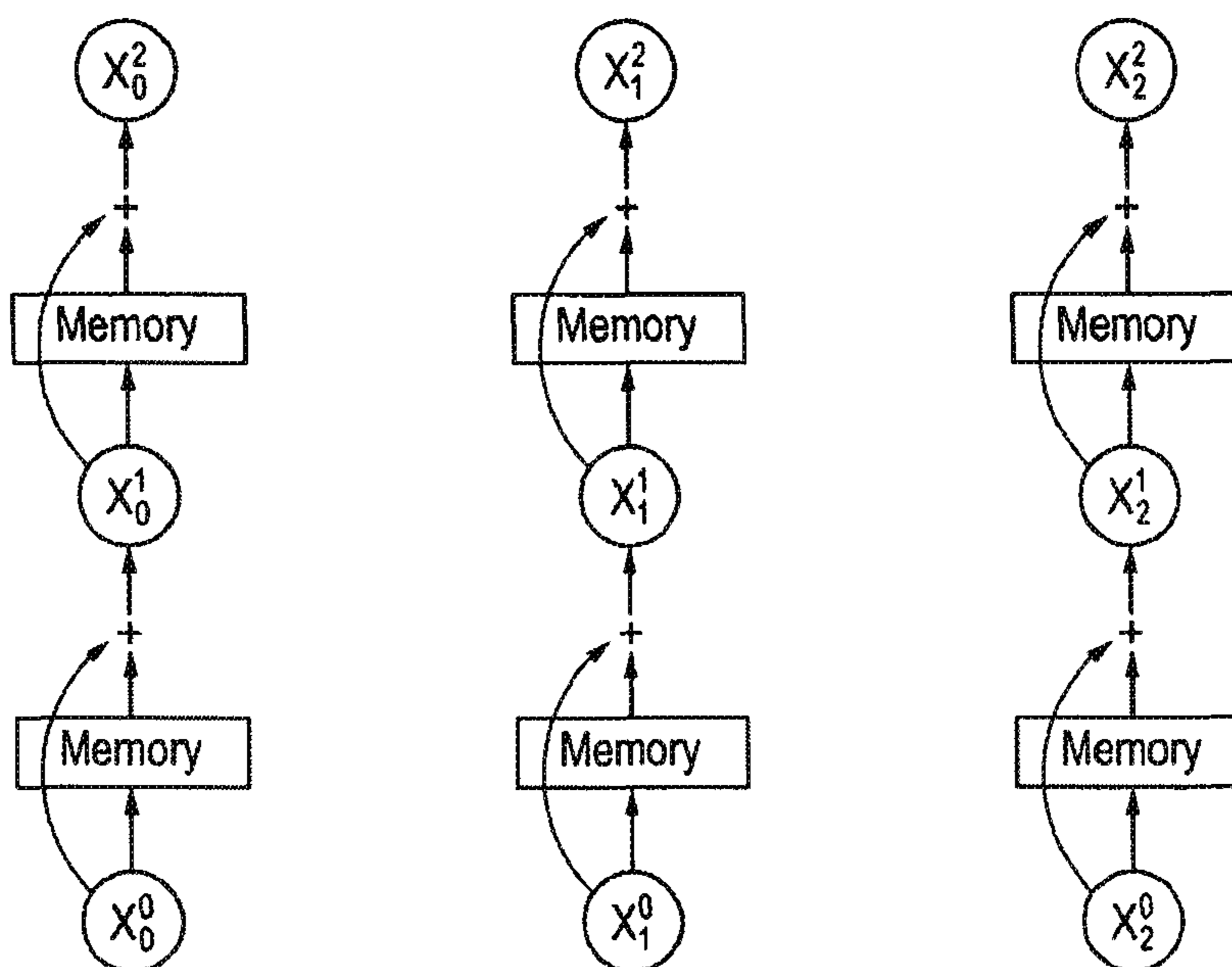
Neural Network
