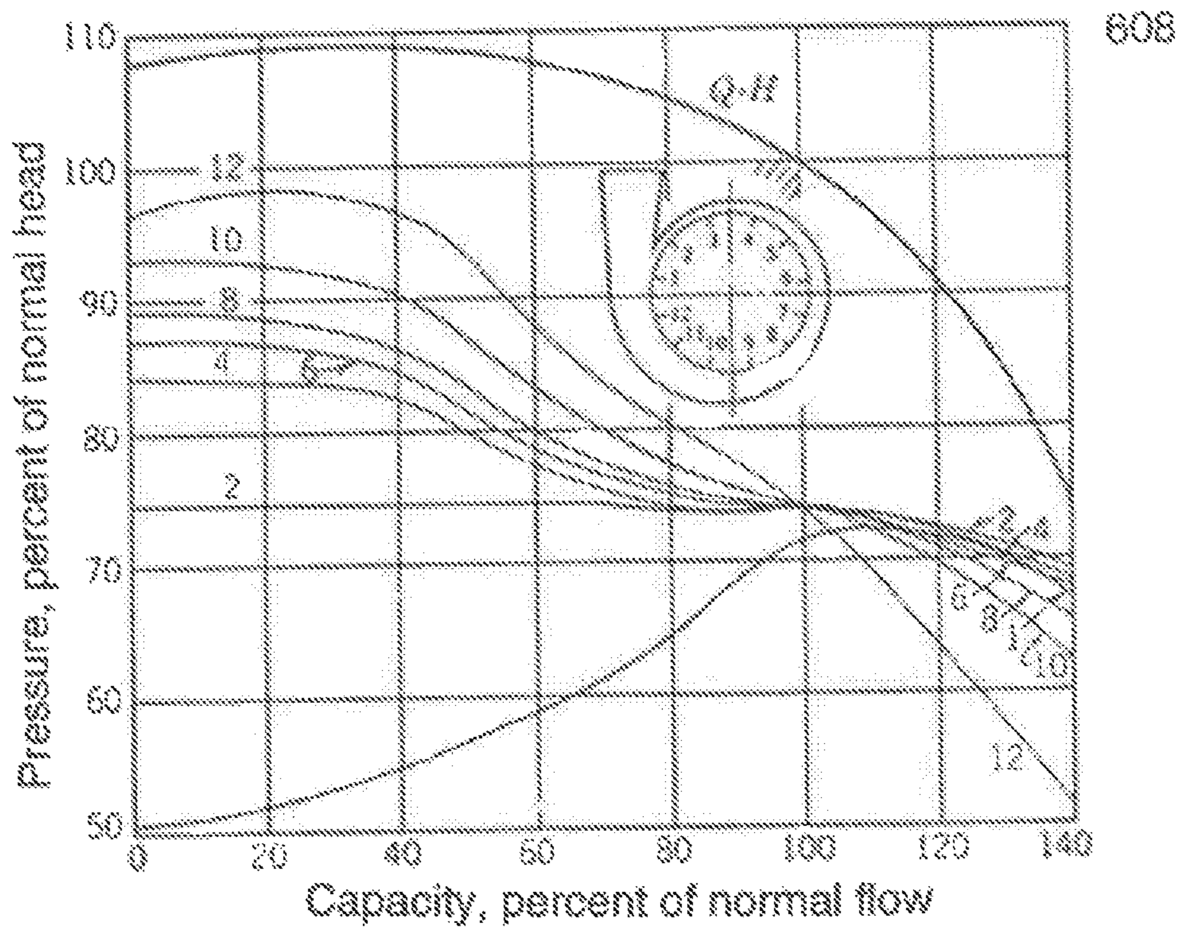
FIG. 7 (Prior Art)
