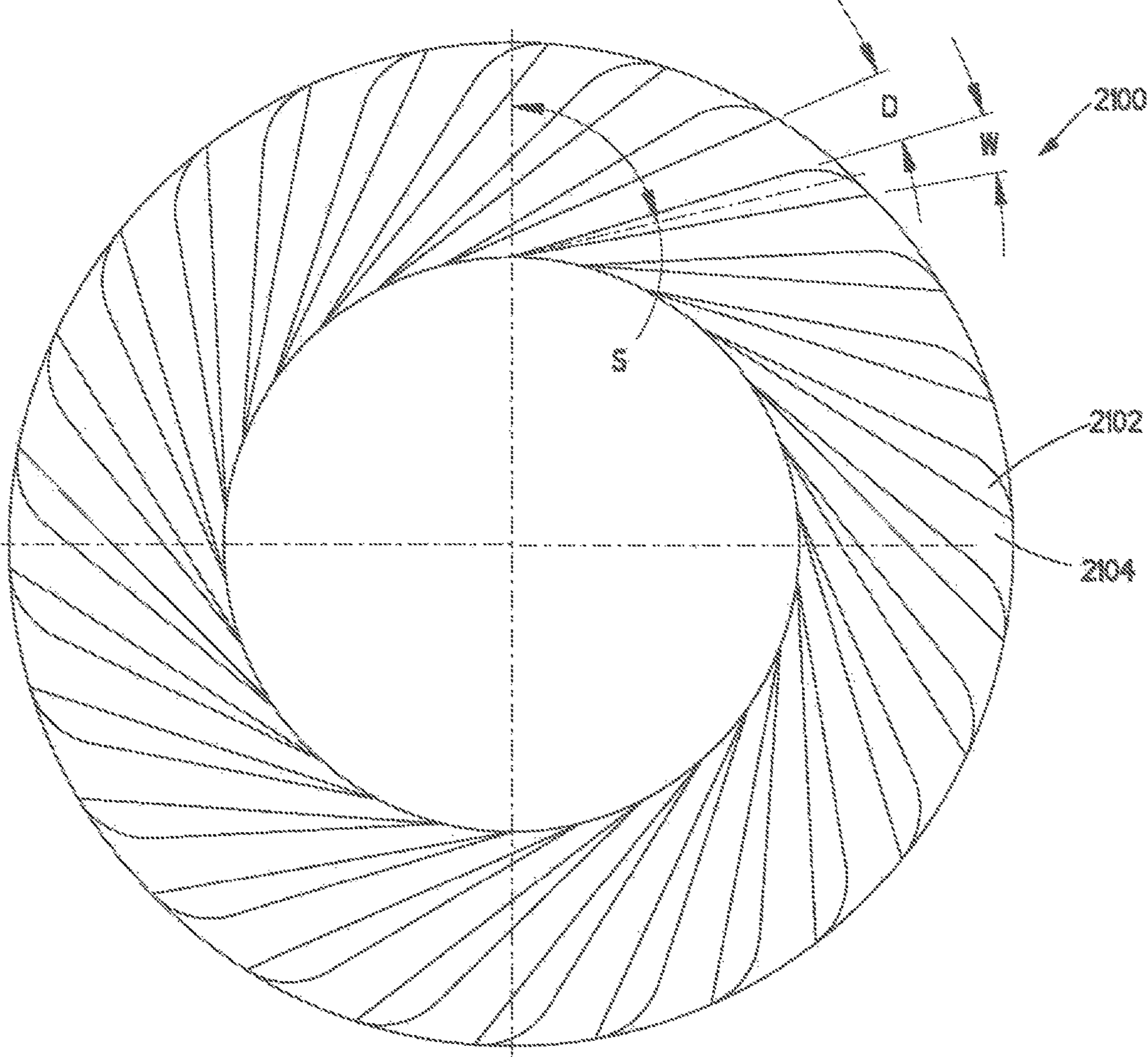
FIG. 21 (Prior Art)
