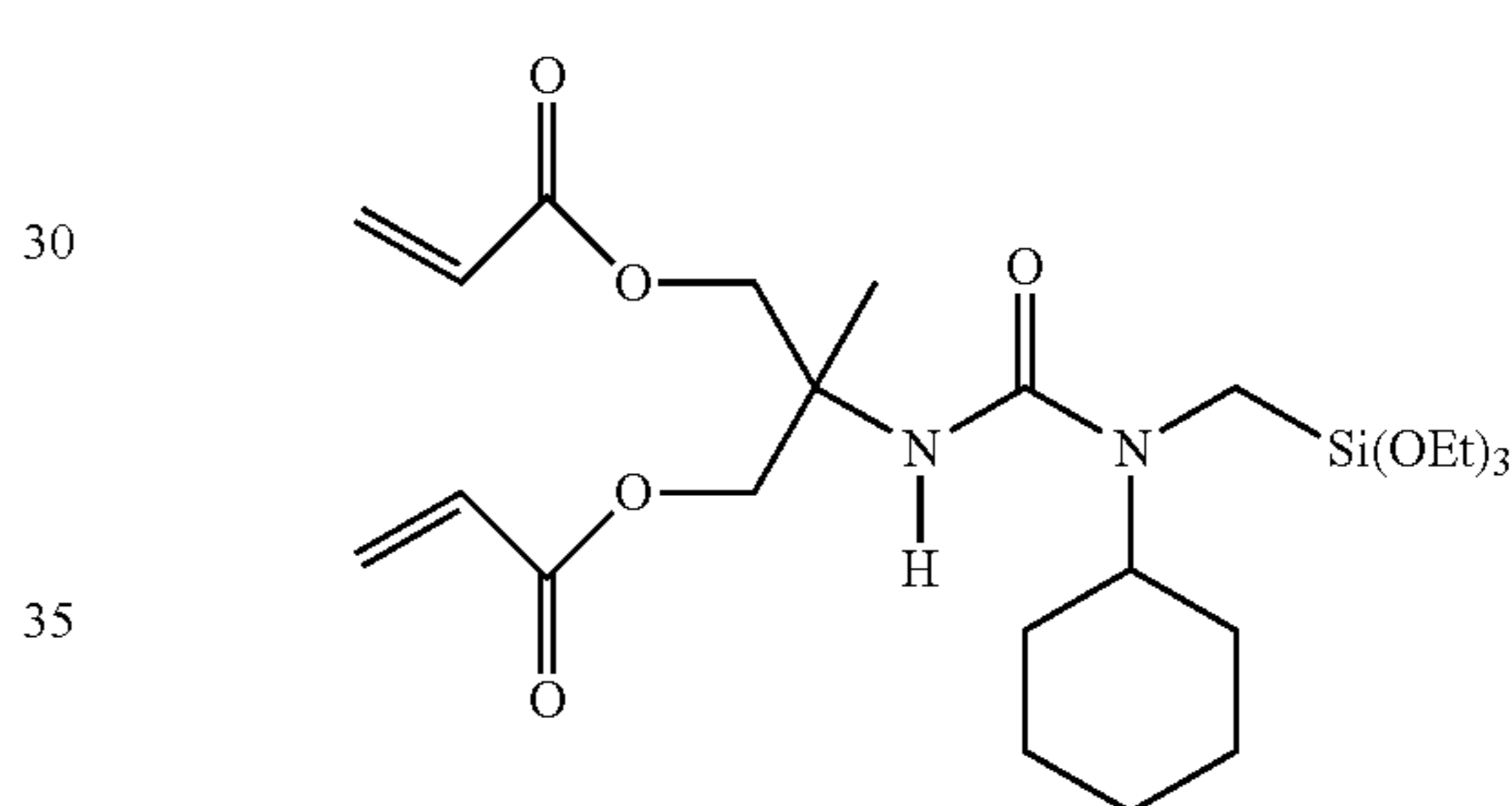
Preparatory Example 8
