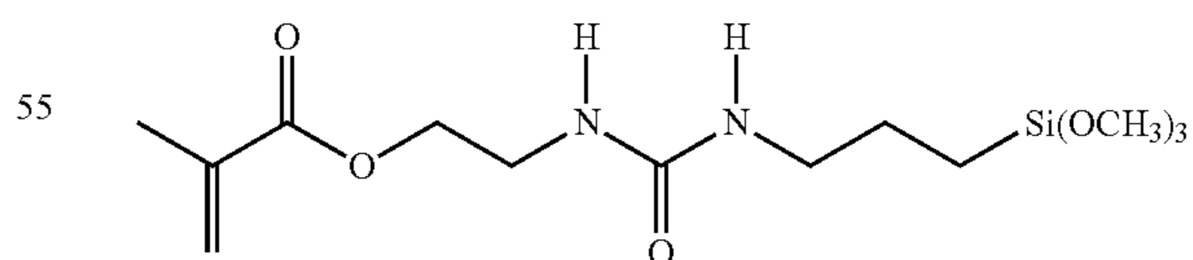
Preparatory Example 9
