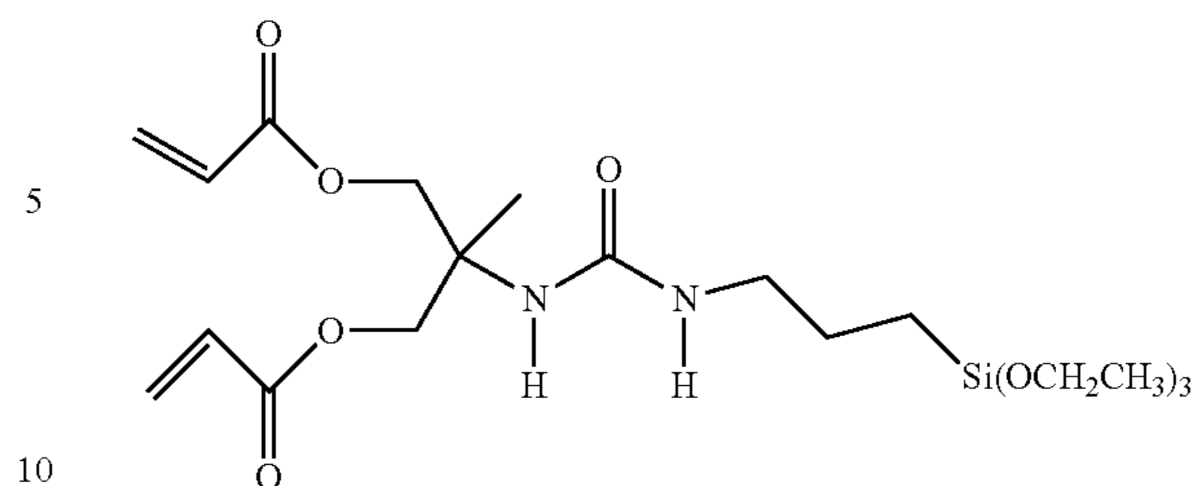
Preparatory Example 7
