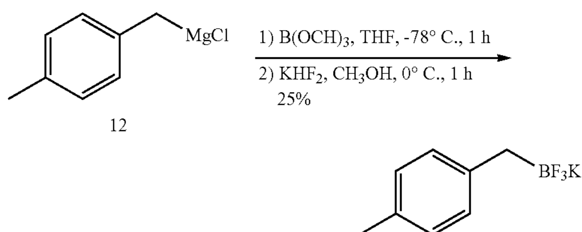
Scheme 2D
