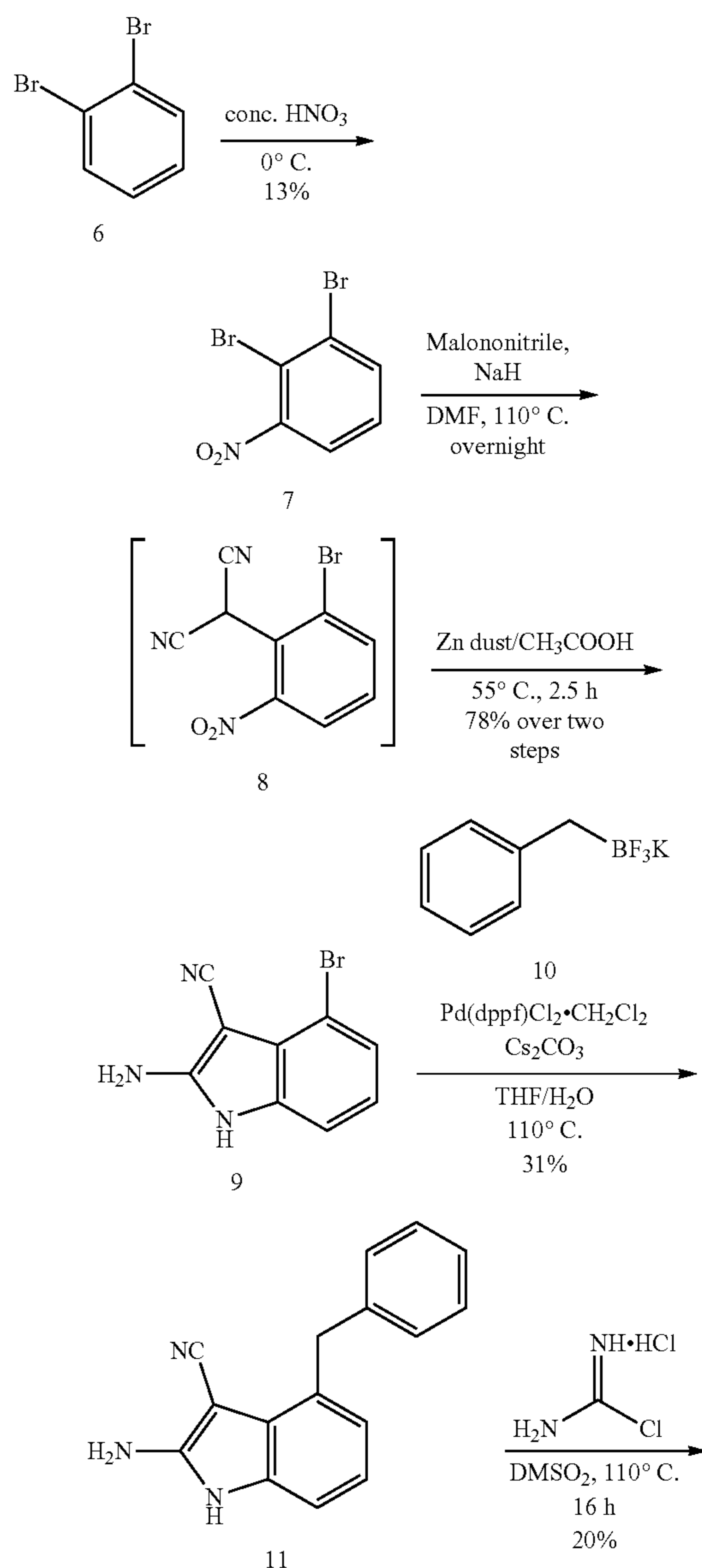
Scheme 1D
