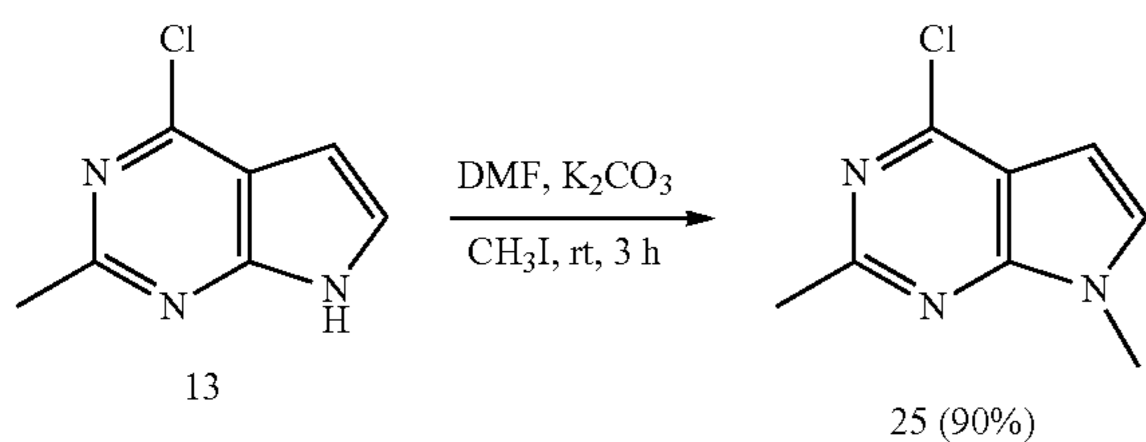
Scheme 3C
