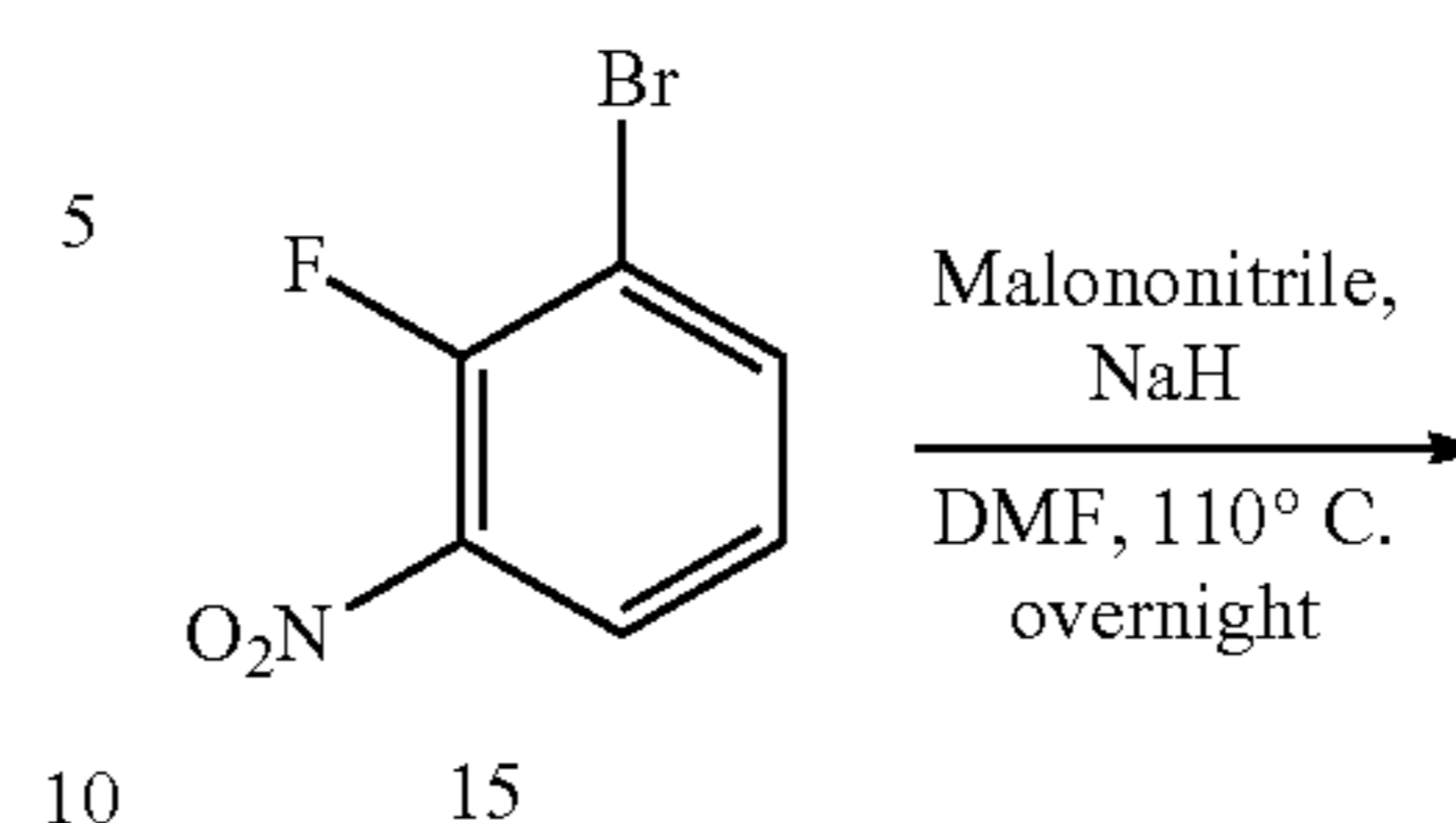
Scheme 3D
