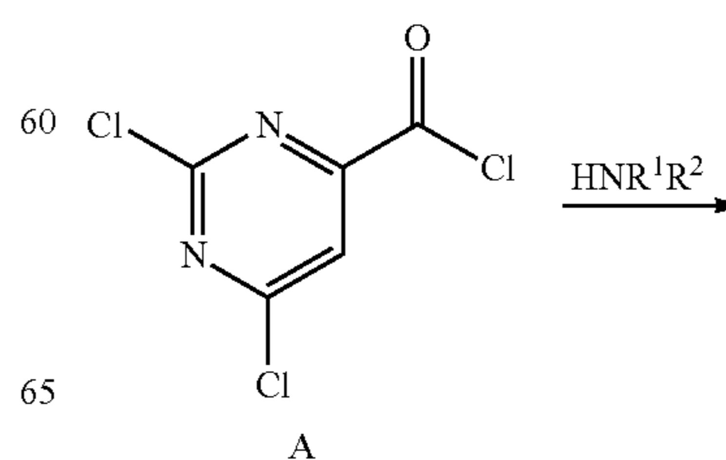
General Scheme 1
