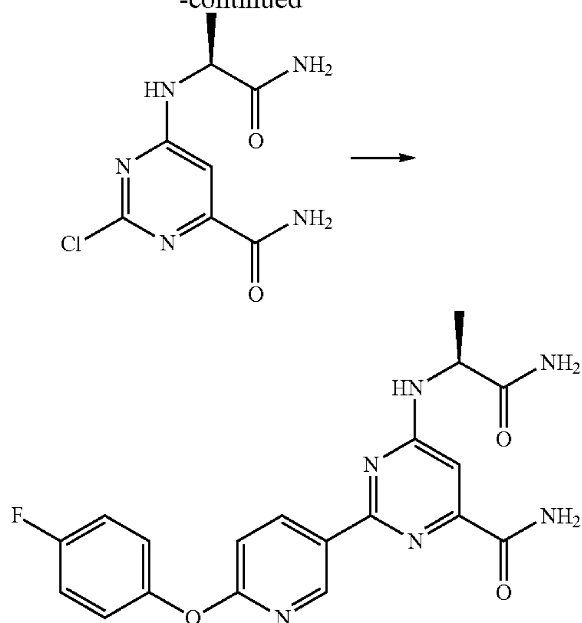
(S)-6-((1-amino-1-oxopropan-2-yl)amino)-2-(6-(4-fluorophenoxy)pyridin-3-yl)pyrimidine-4-carboxamide
