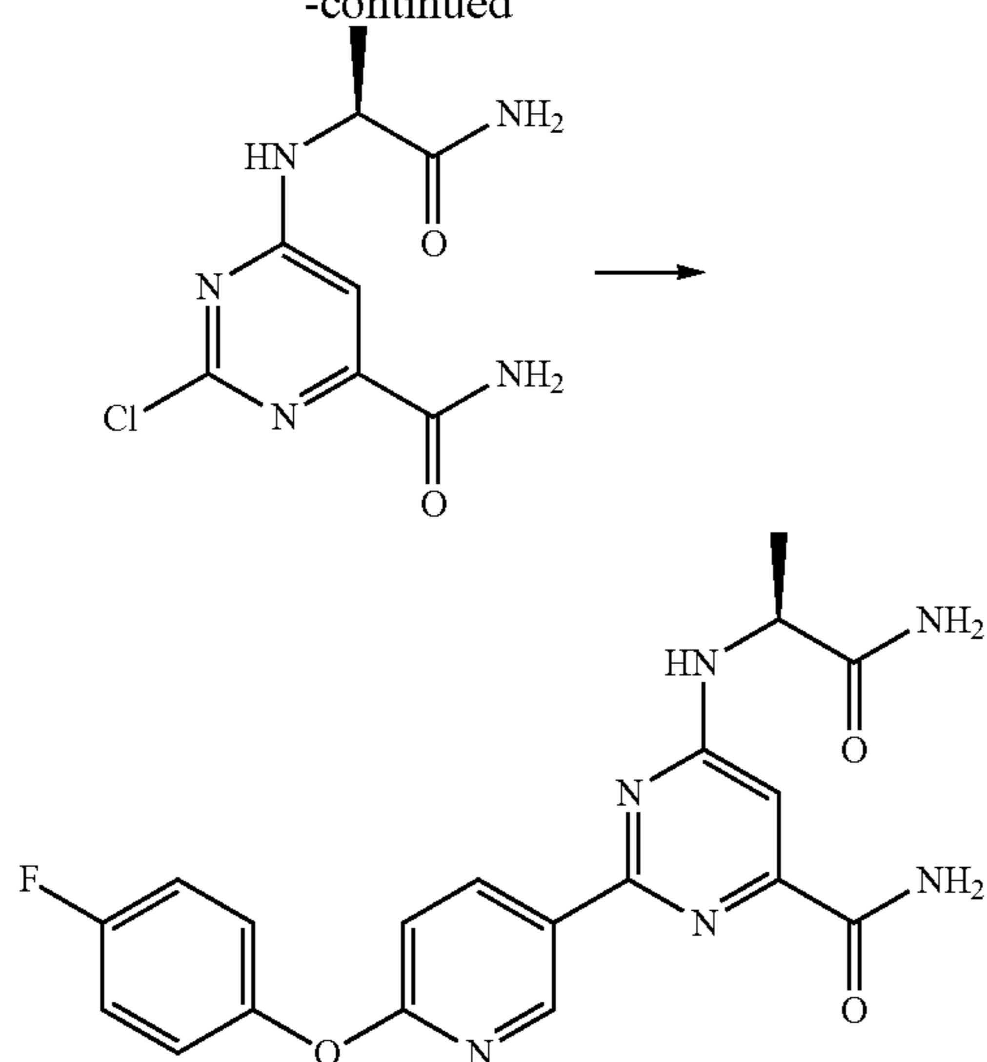
(S)-6-((1-amino-1-oxopropan-2-yl)amino)-2-(6-(4-fluorophenoxy)pyridin-3-yl)pyrimidine-4-carboxamide
