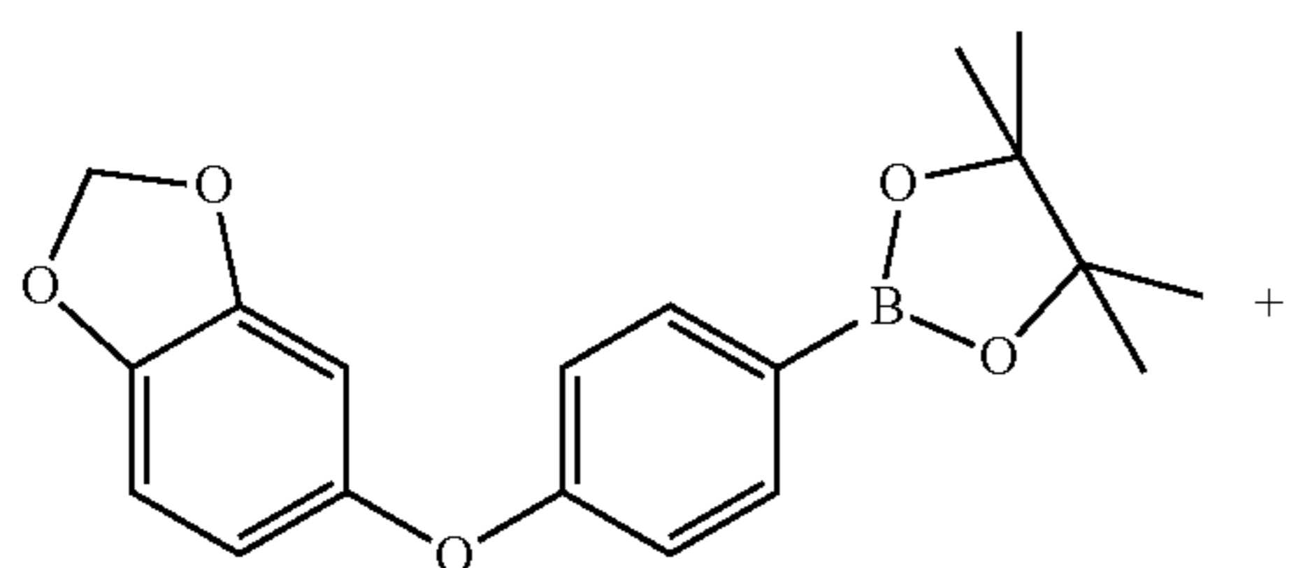
Scheme 72
