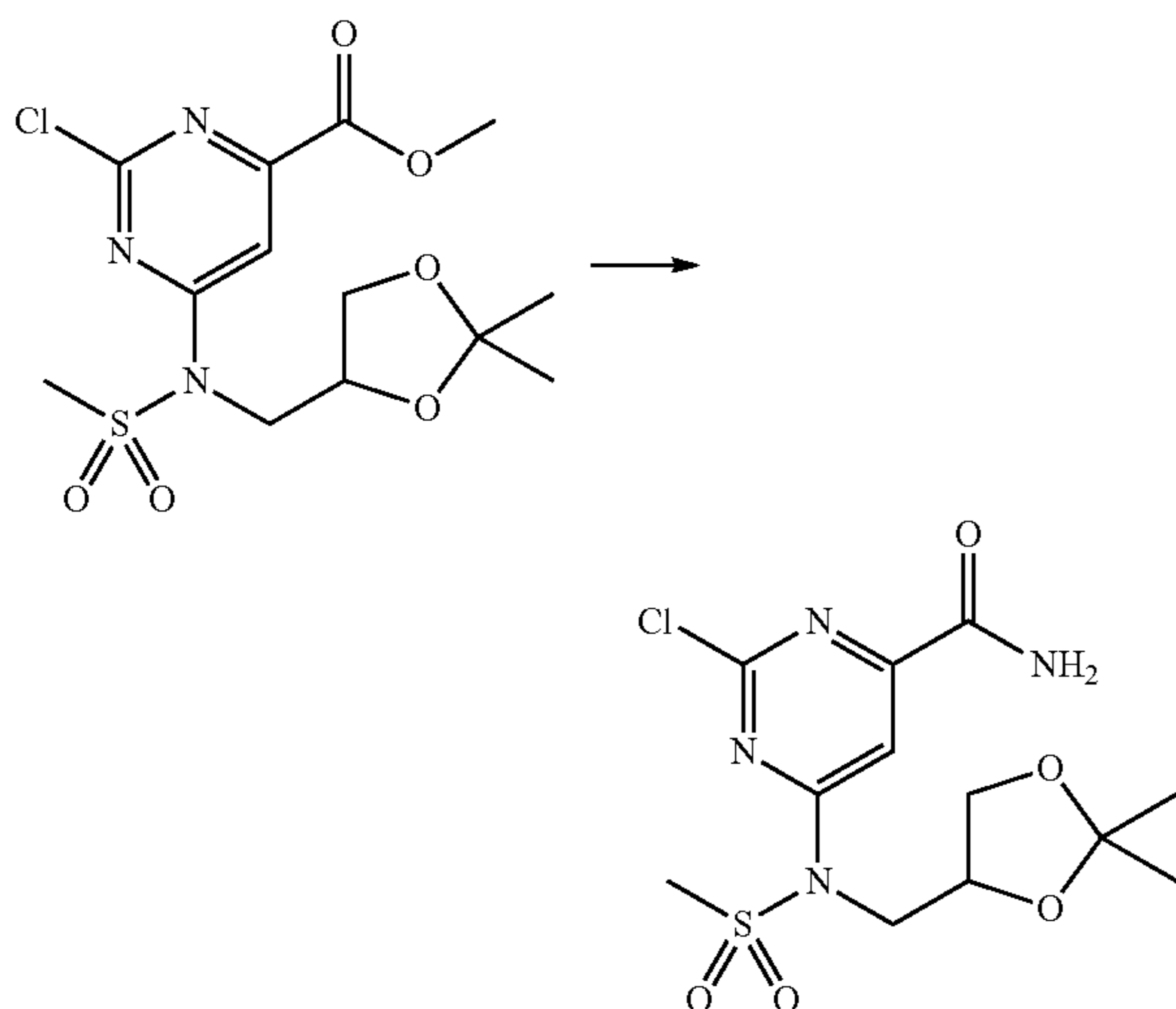
Scheme 34
