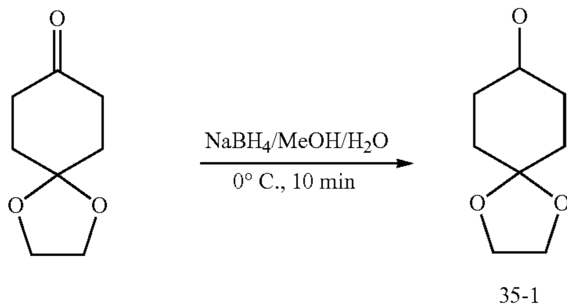
Scheme 77
