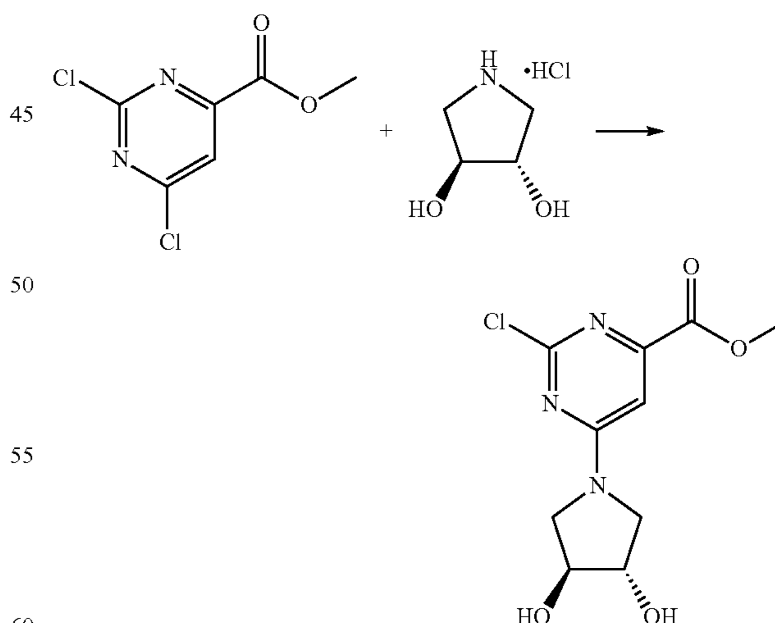
Scheme 58
