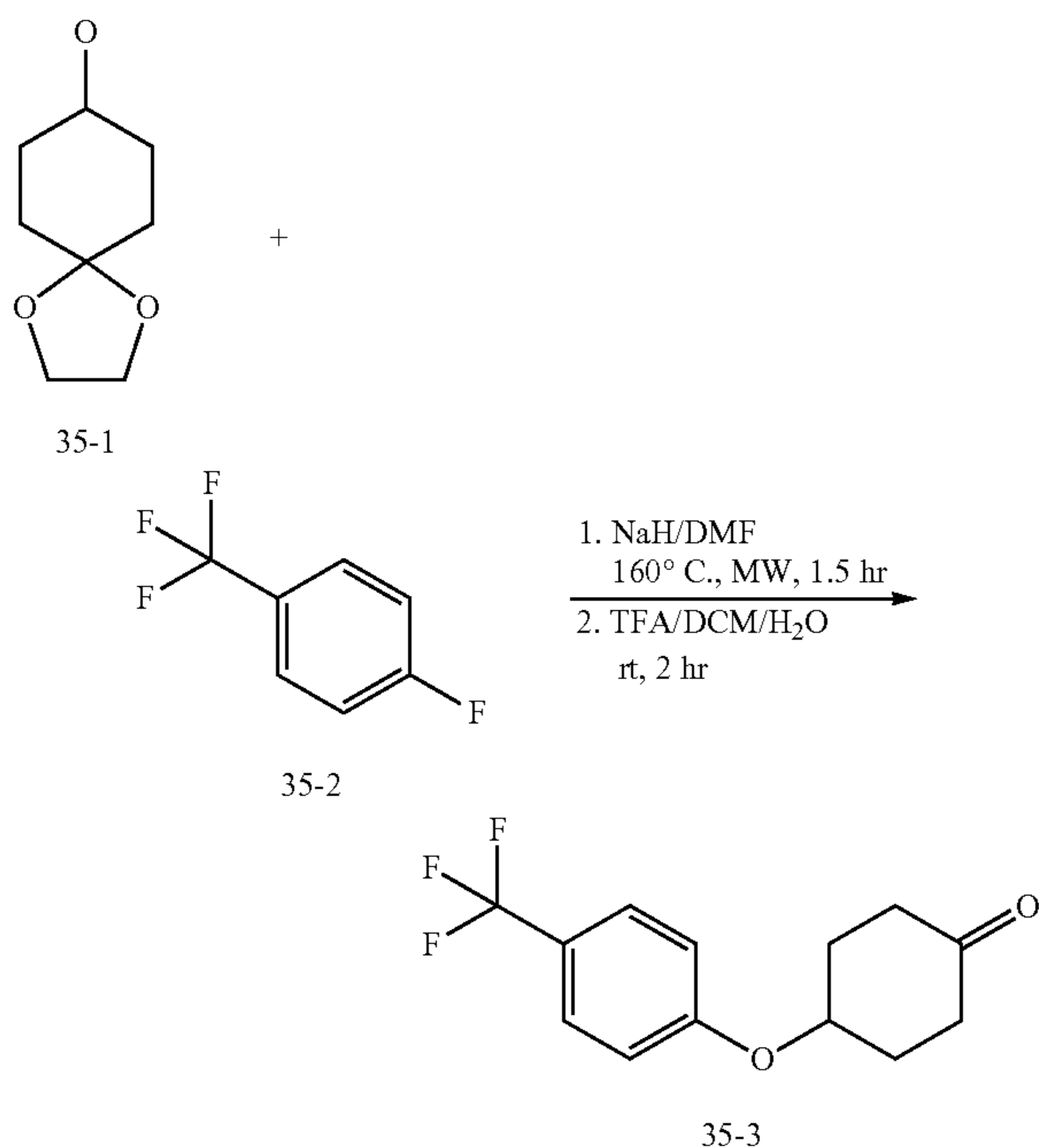
Scheme 78
