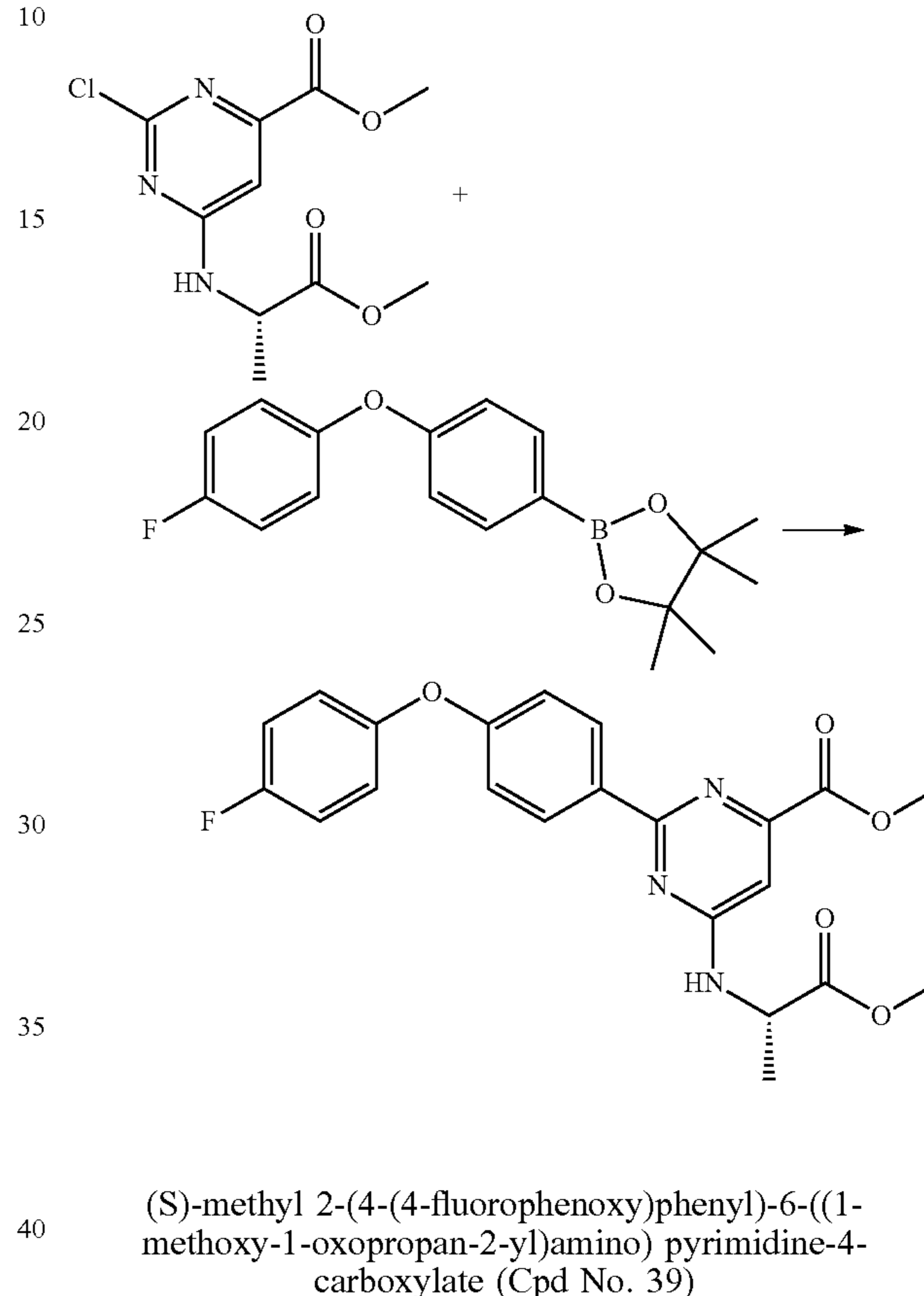
Scheme 20
