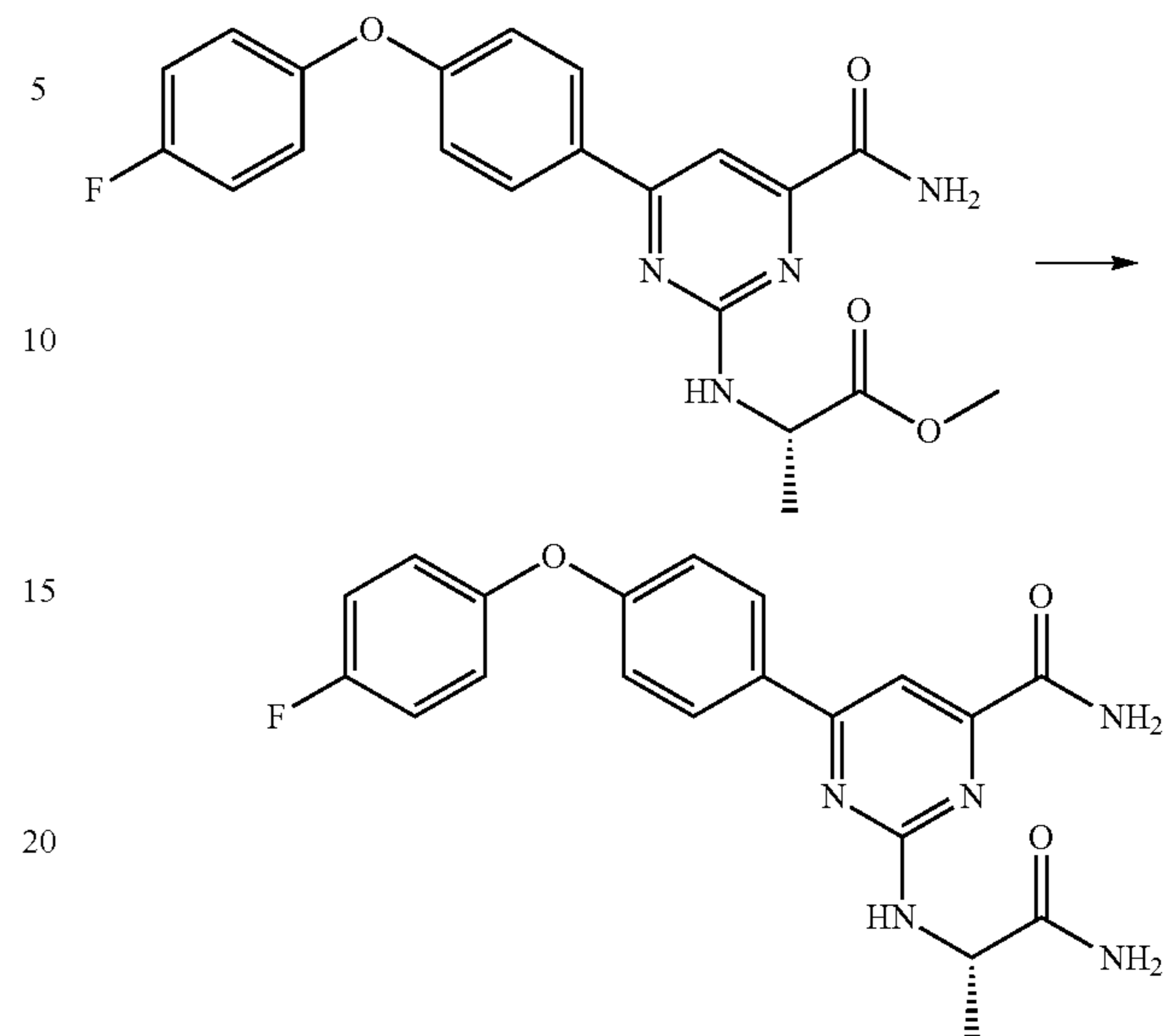
Scheme 38
