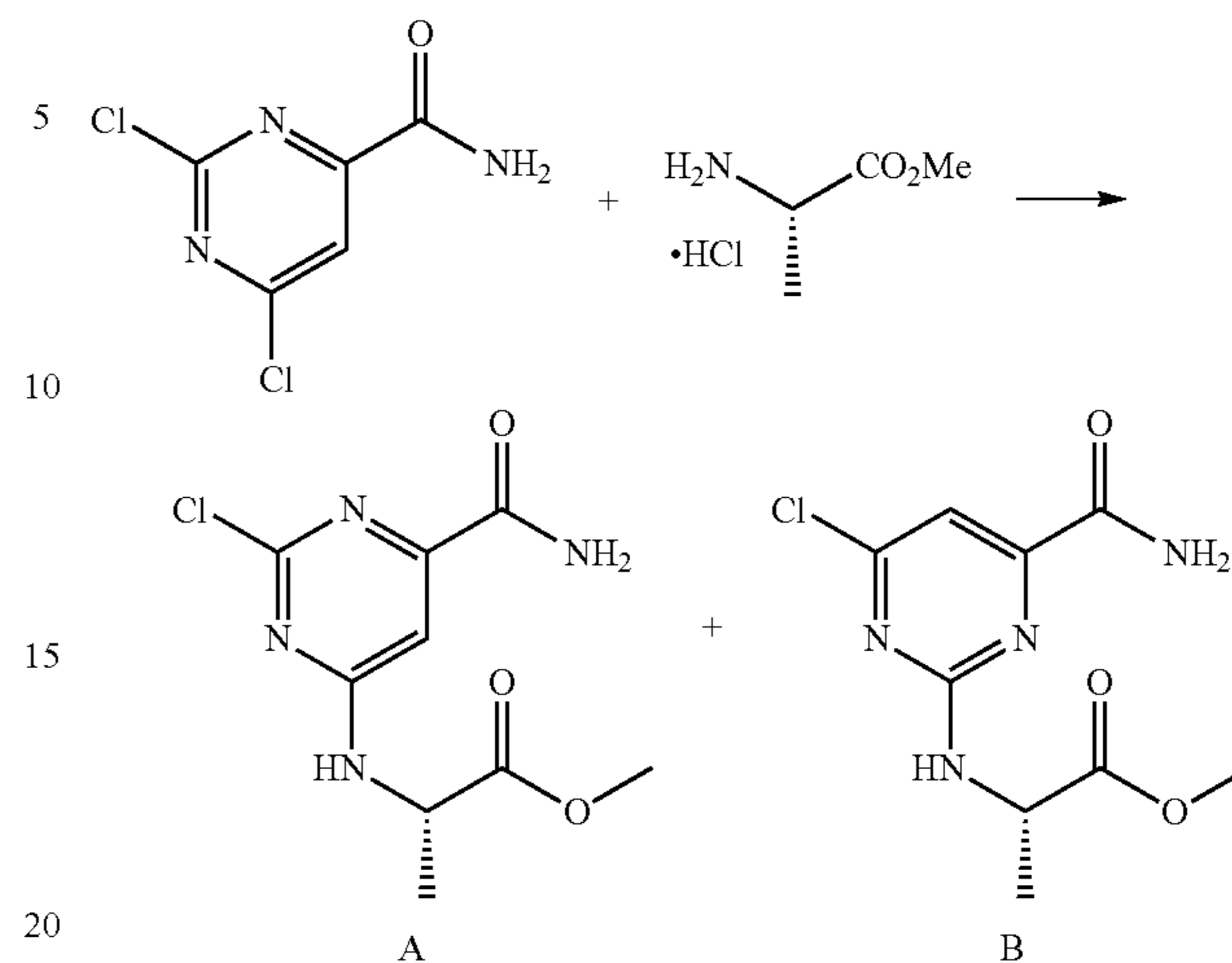
Scheme 4
