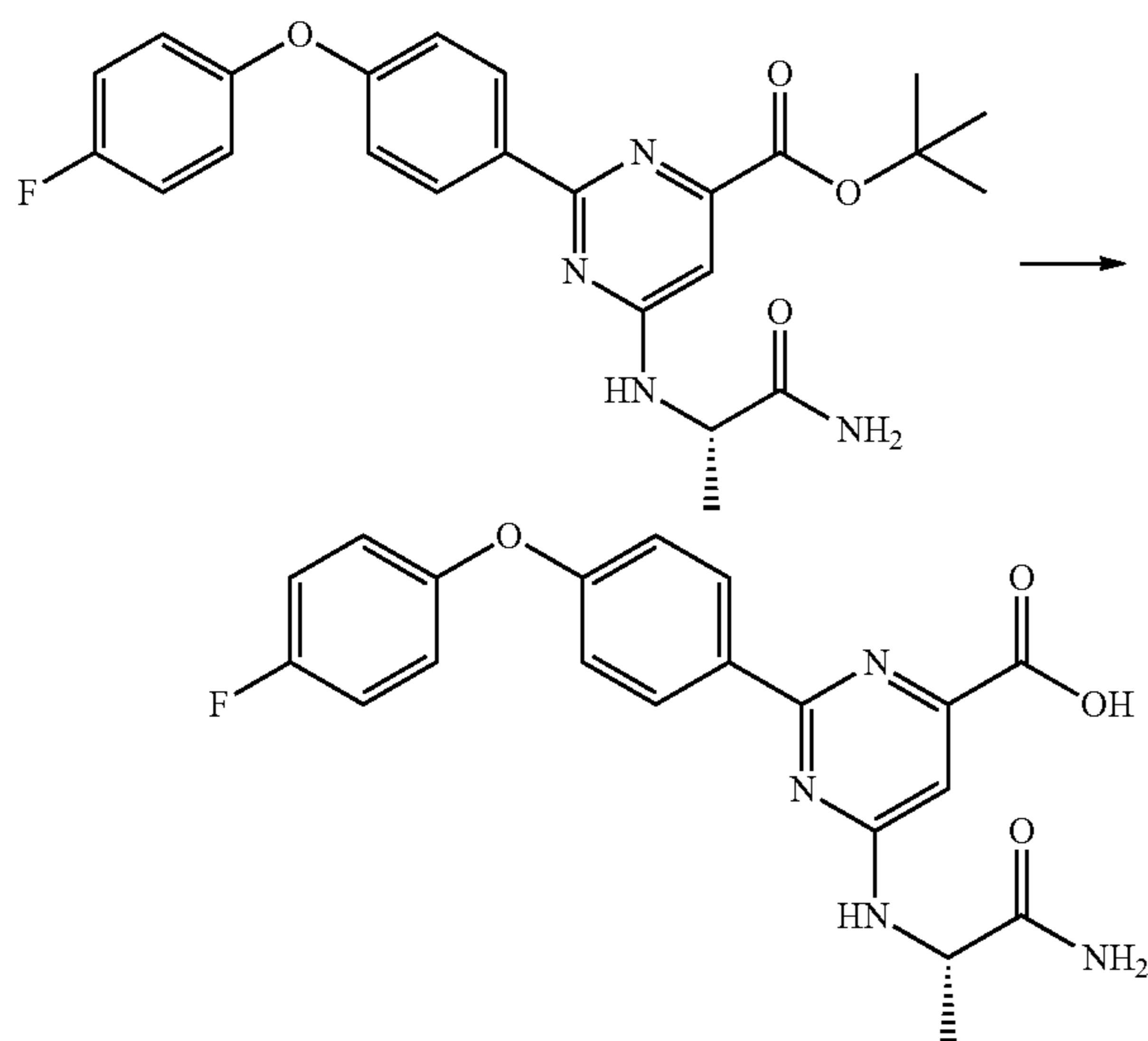
Scheme 16
