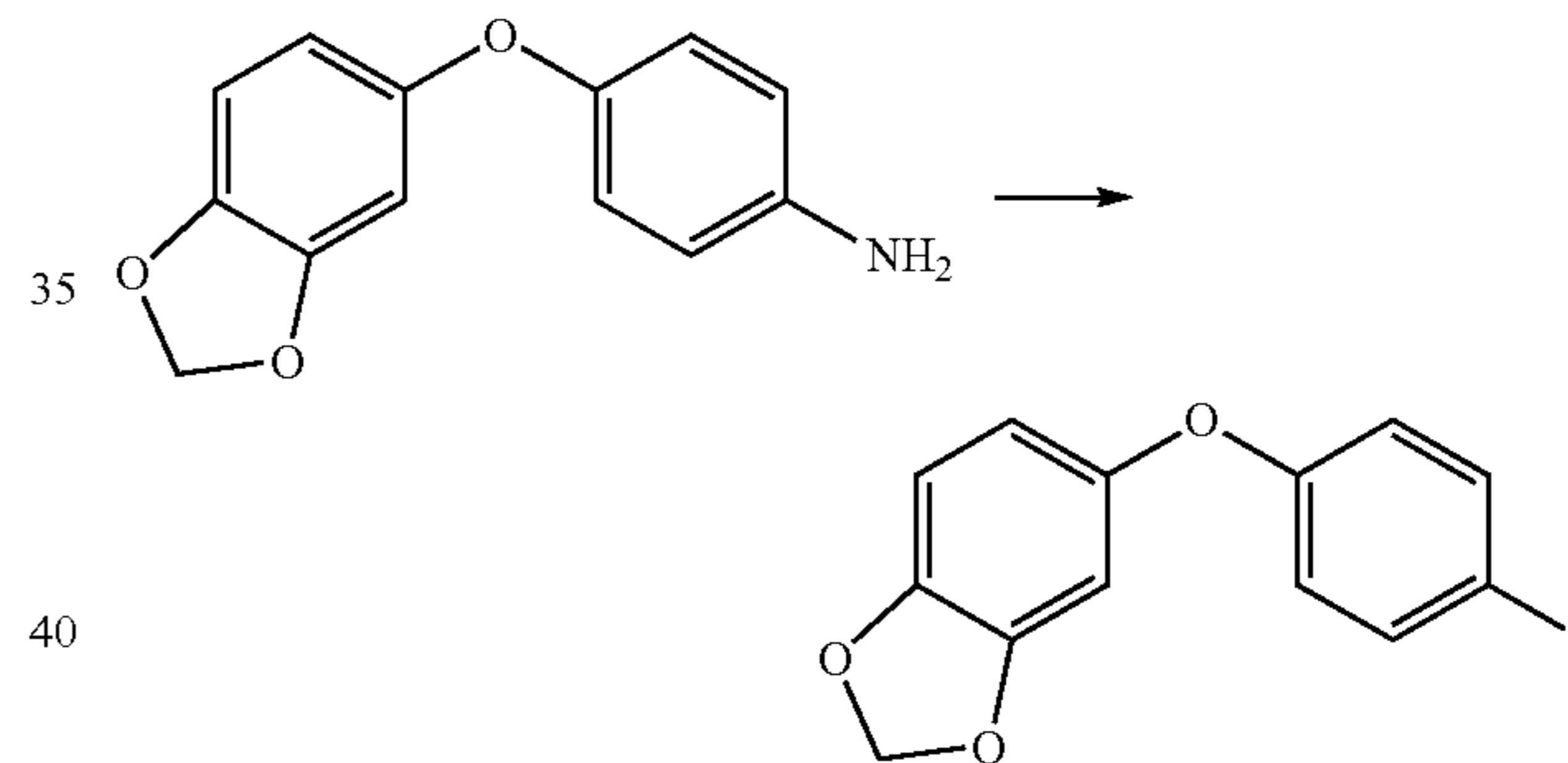
Scheme 70
