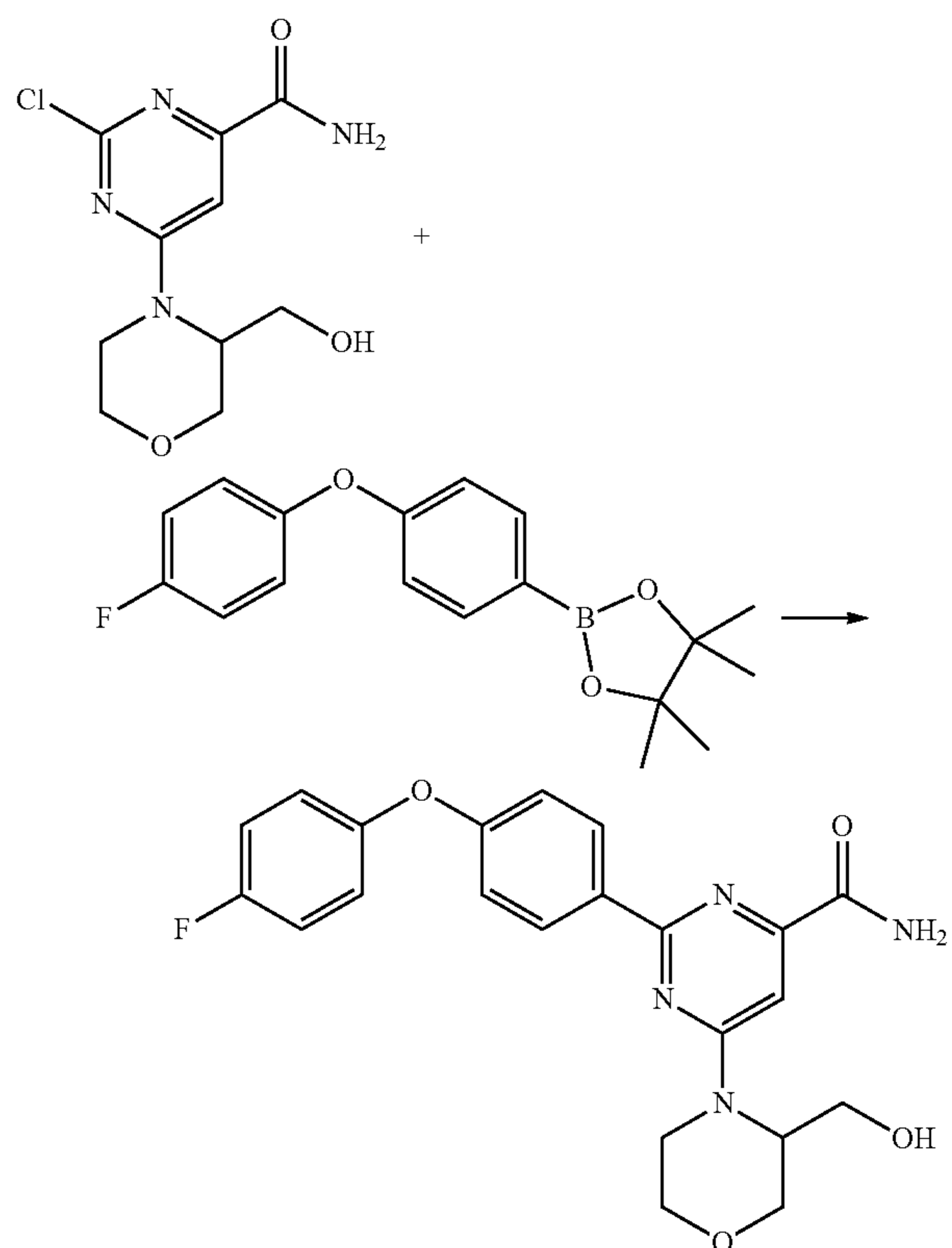
Scheme 23
