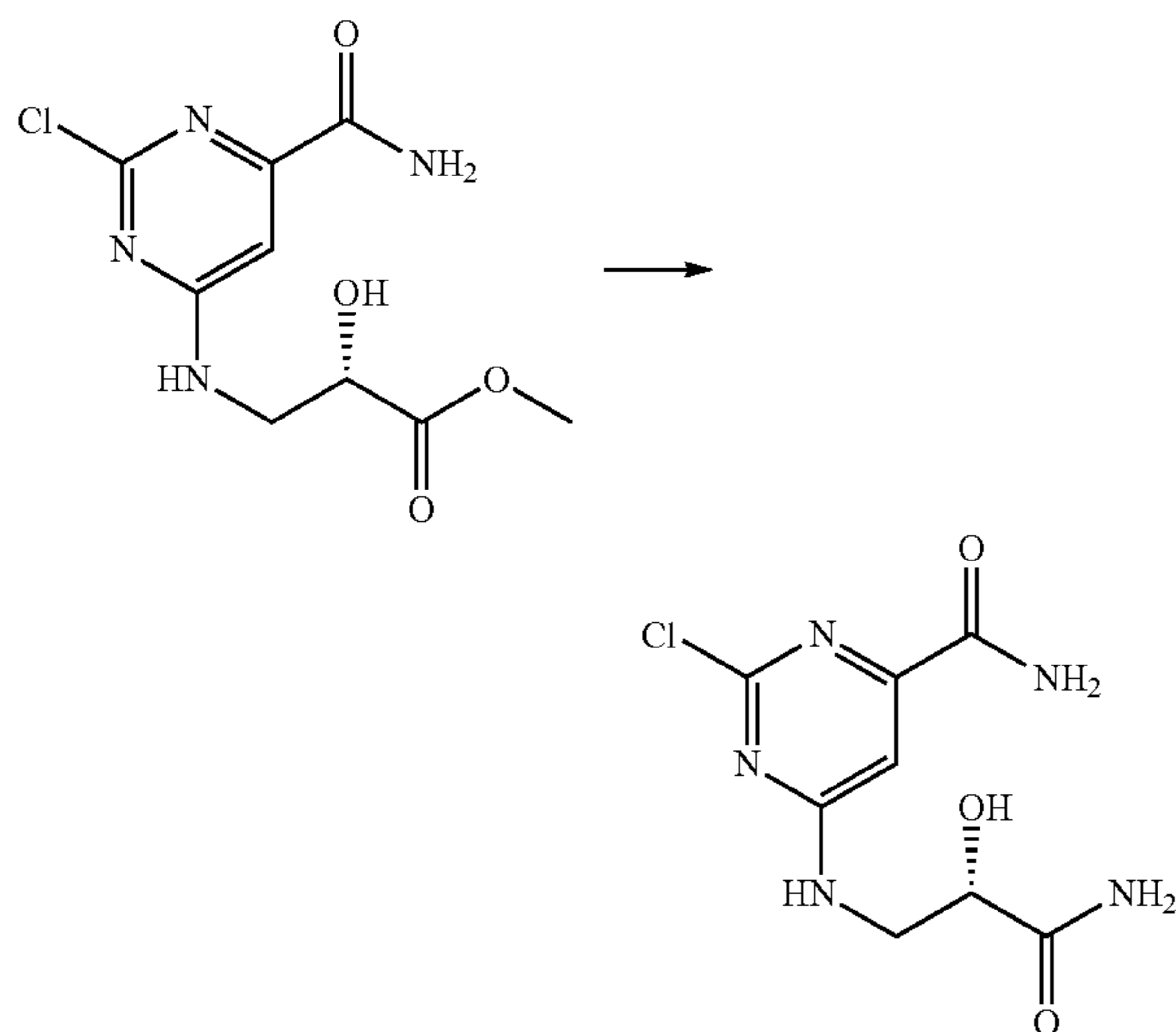
Scheme 29
