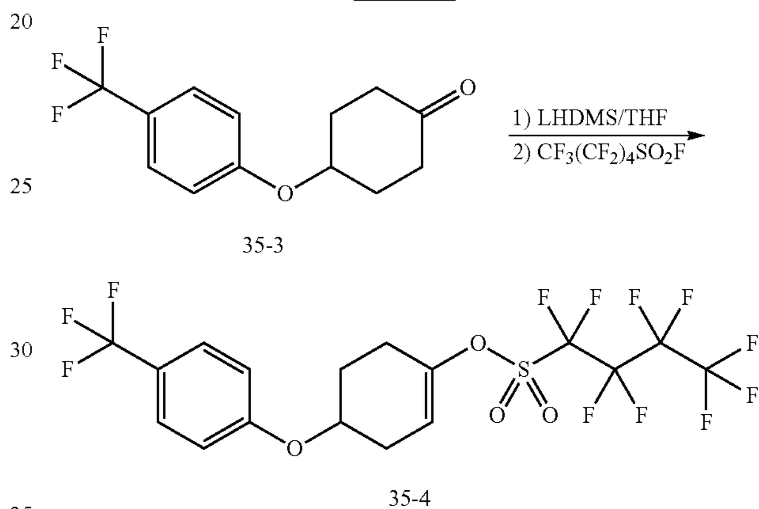
Scheme 79
