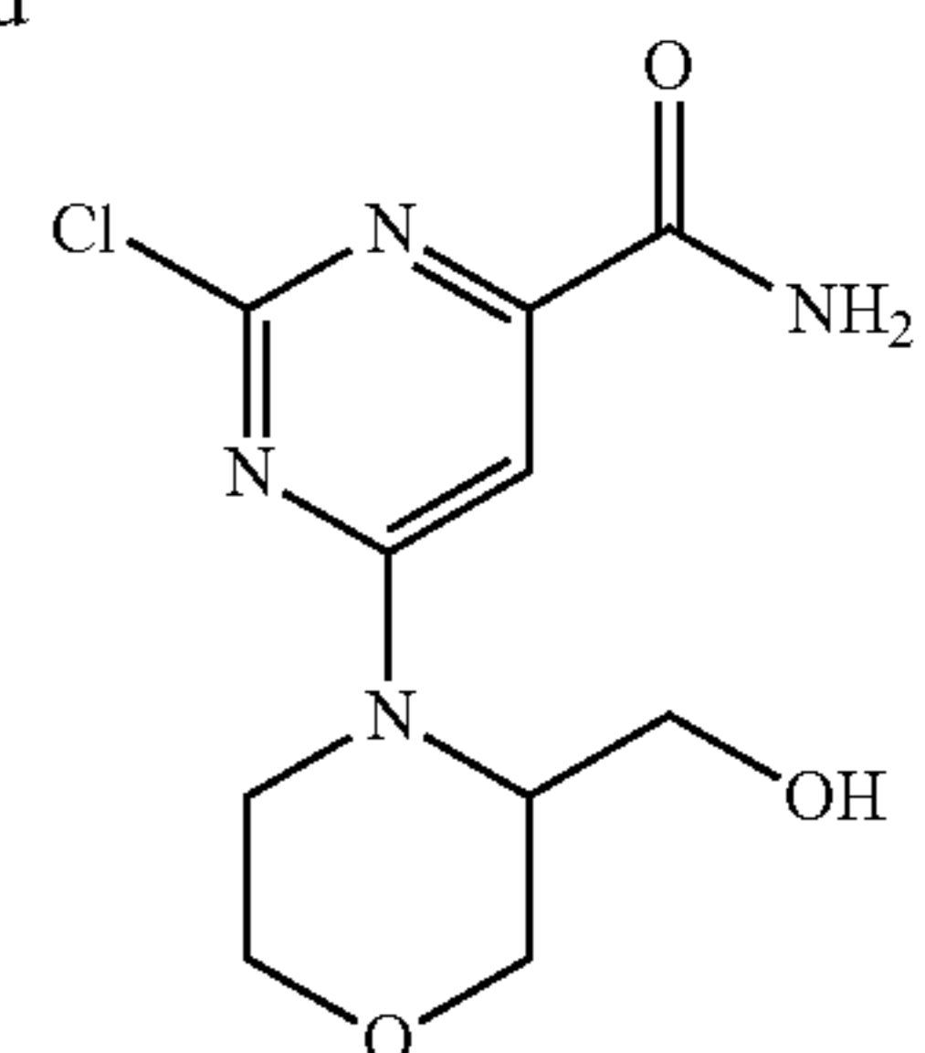
2-chloro-6-(3-(hydroxymethyl)morpholino)pyrimidine-4-carboxamide
