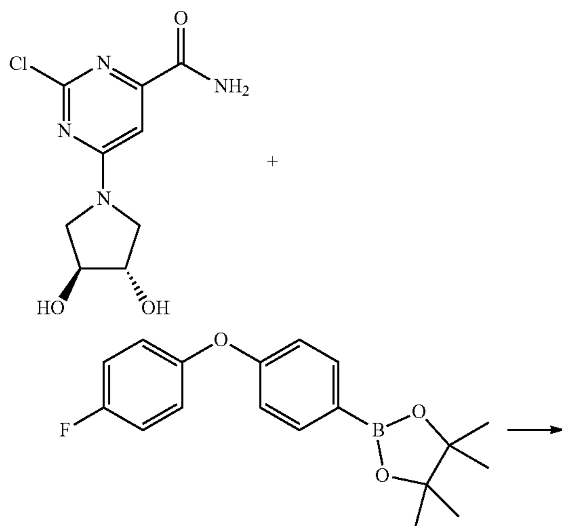
Scheme 60
