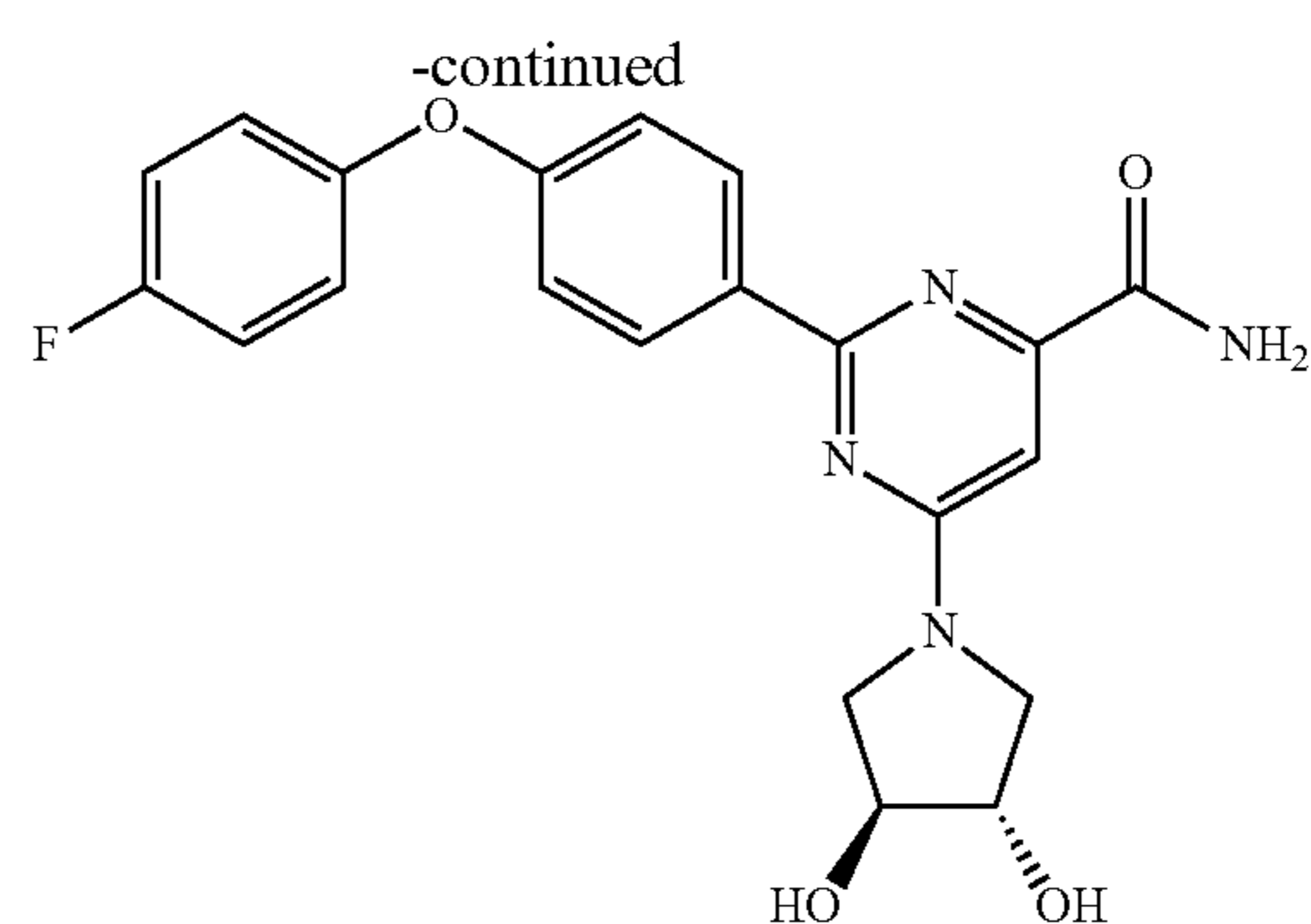
6-((3S,4S)-3,4-dihydroxypyrrolidin-1-yl)-2-(4-(4-fluorophenoxy)phenyl)pyrimidine-4-carboxamide
