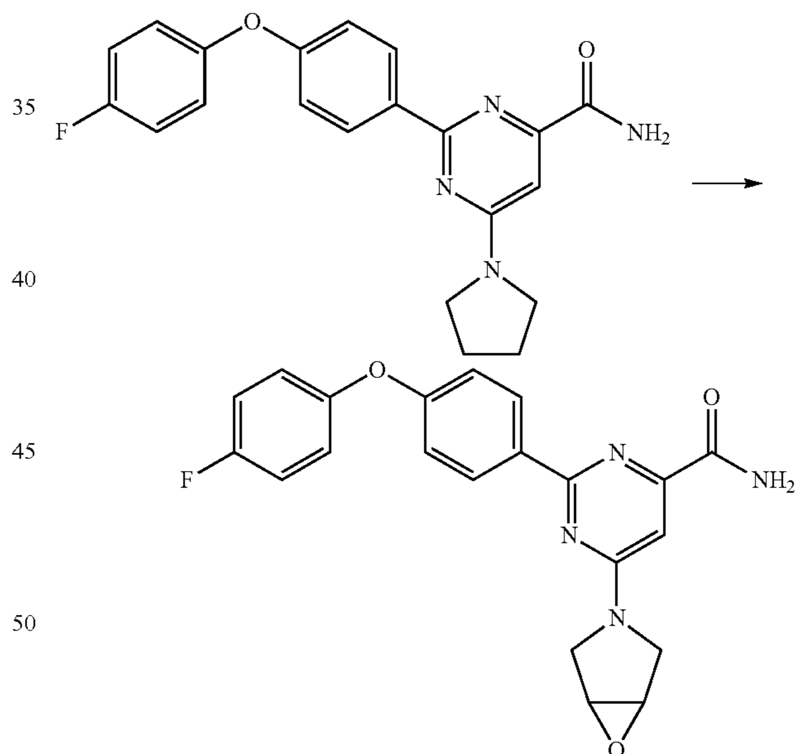
Scheme 25
