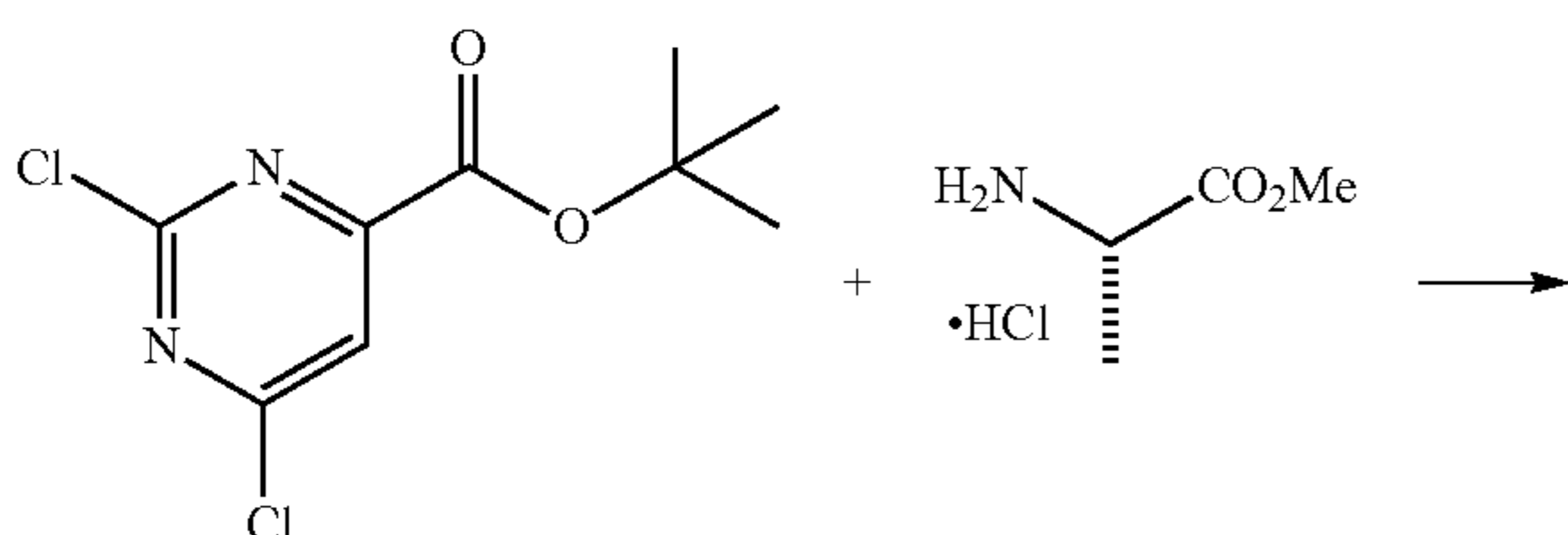
Scheme 11
