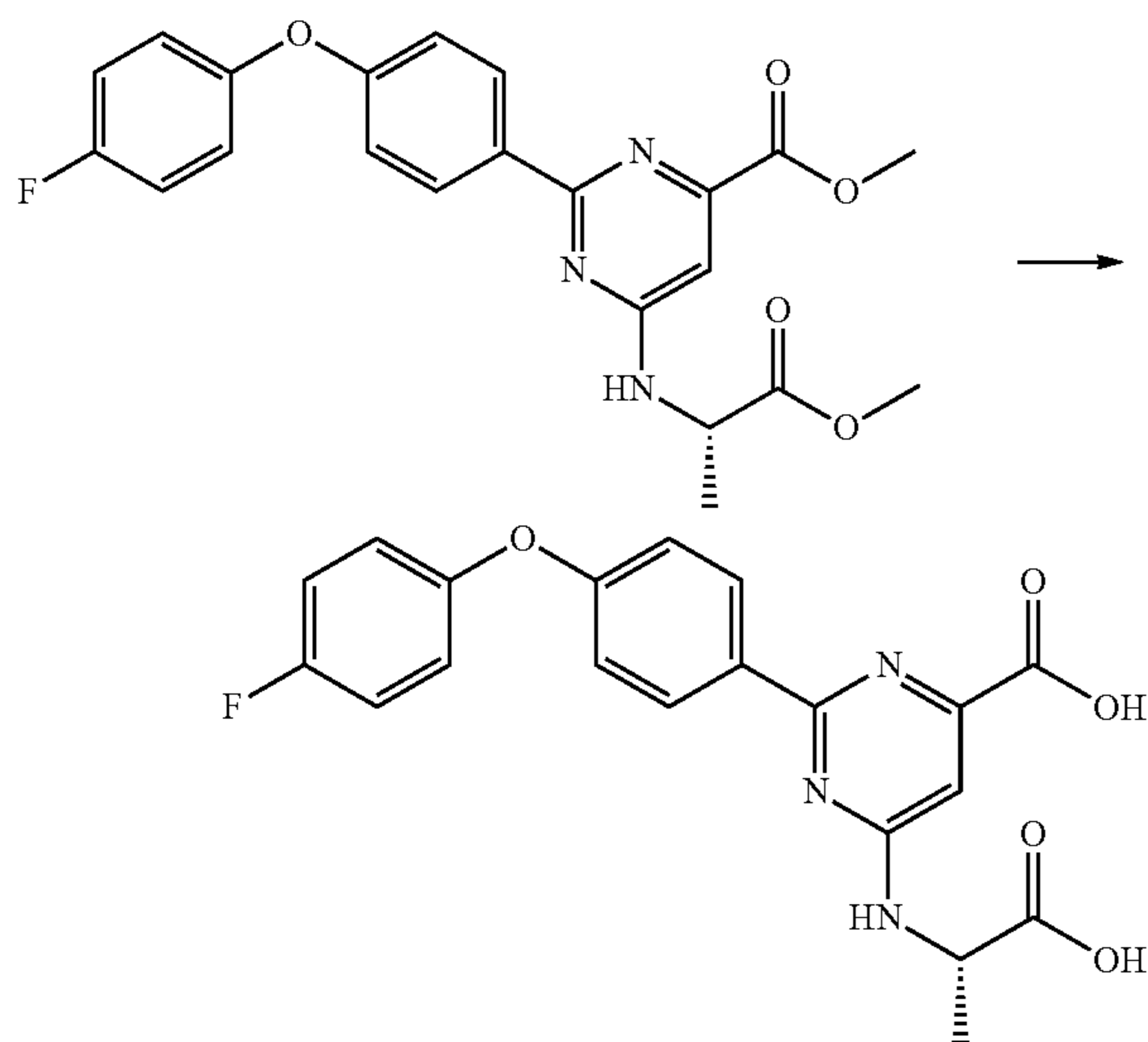
Scheme 21
