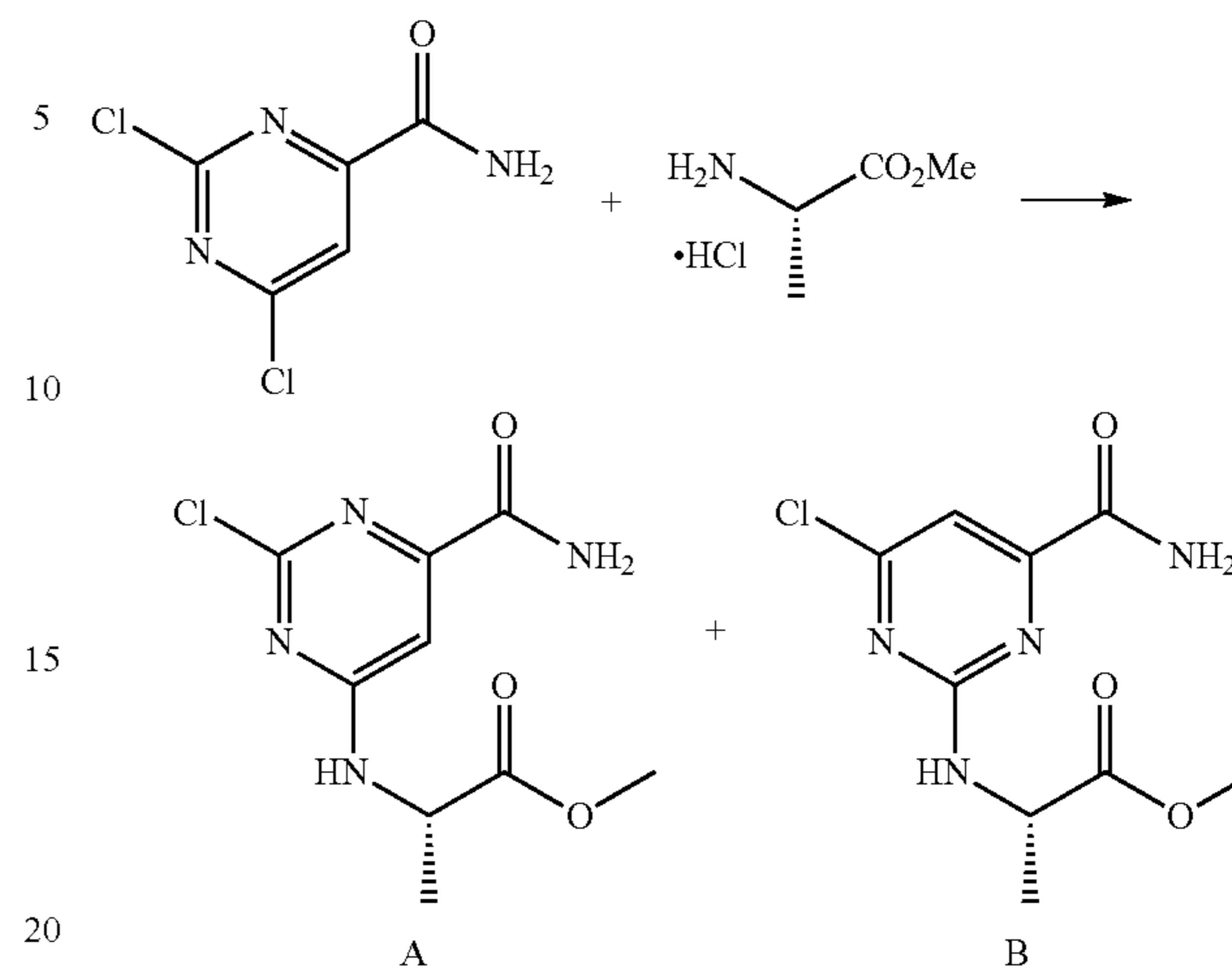
Scheme 4
