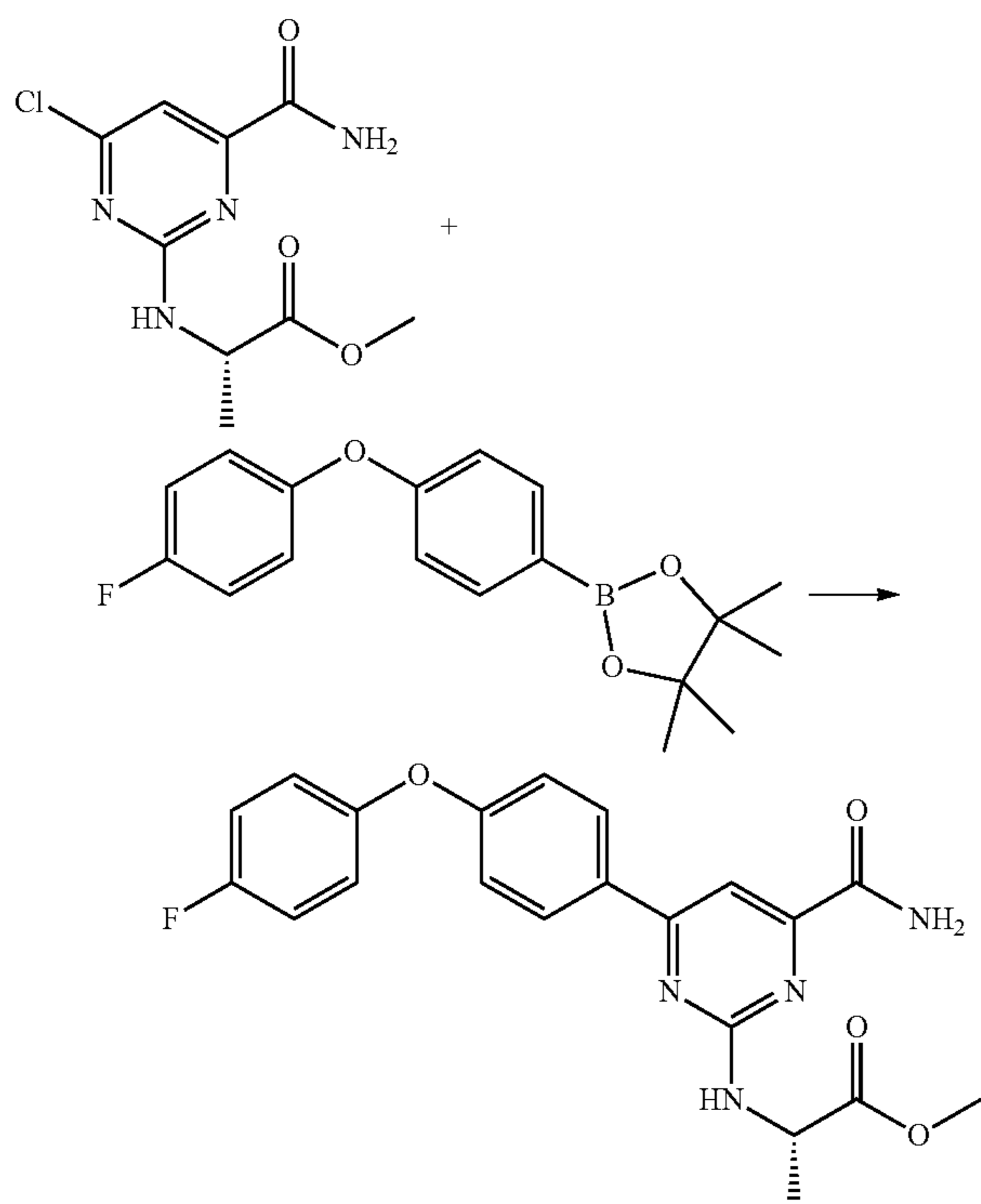
Scheme 30
