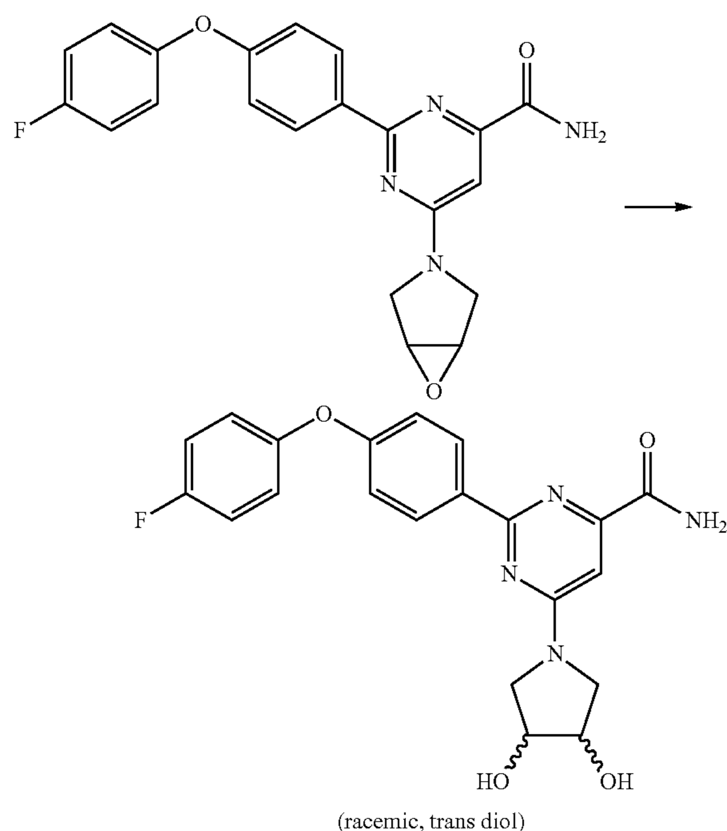
Scheme 26
