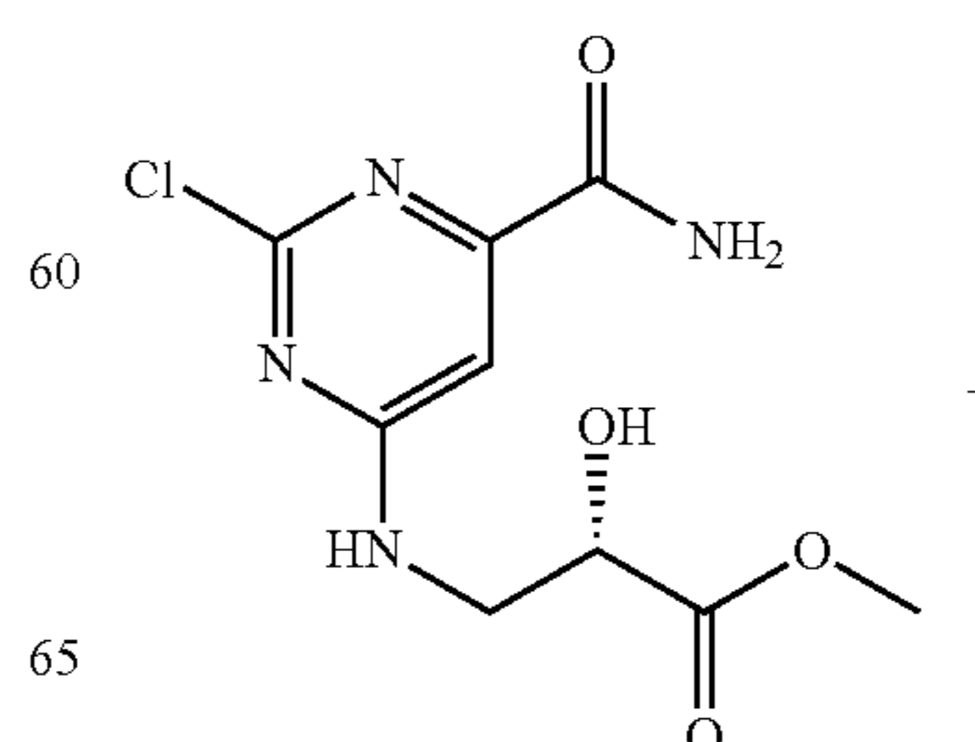
Scheme 31
