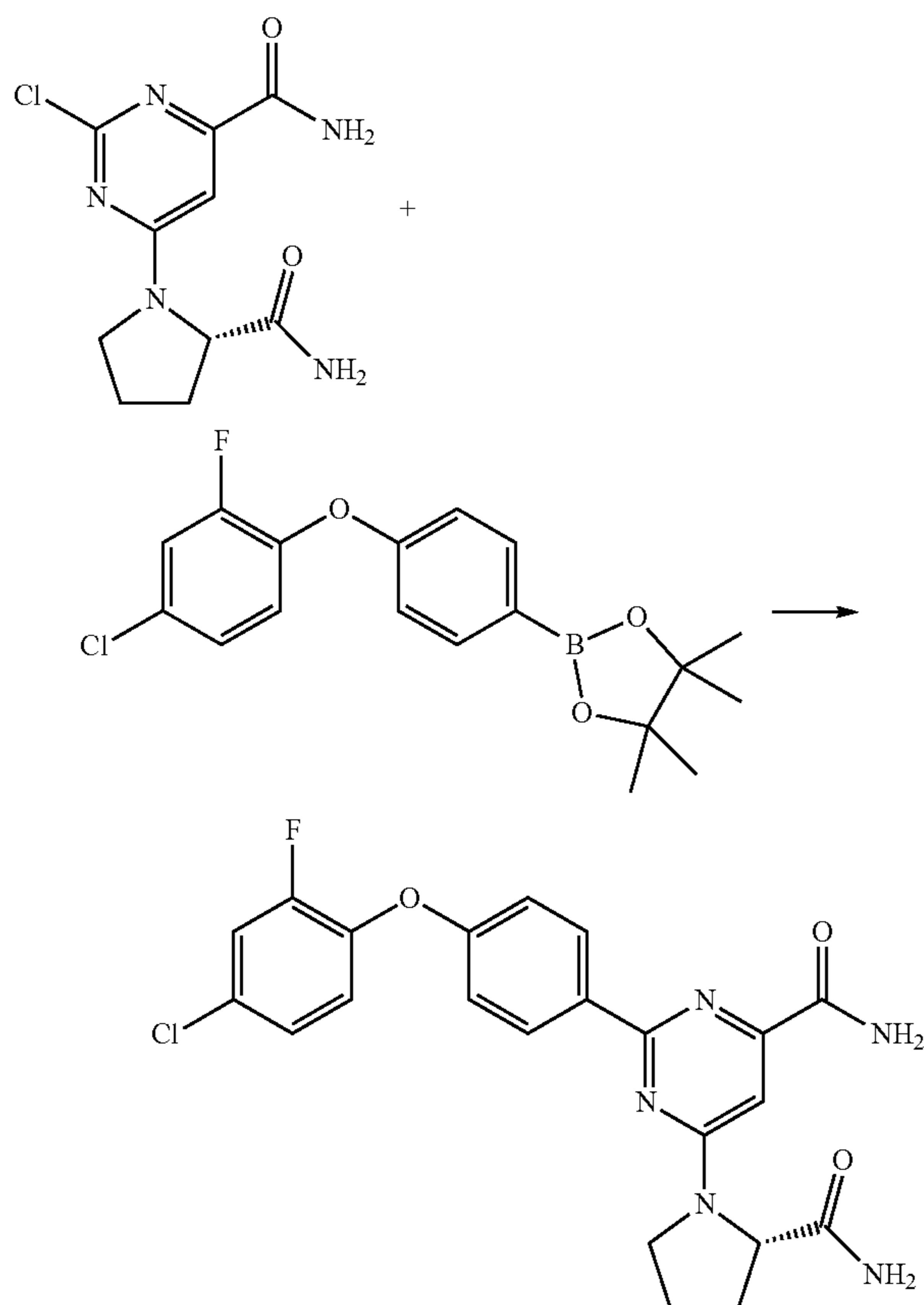
Scheme 57
