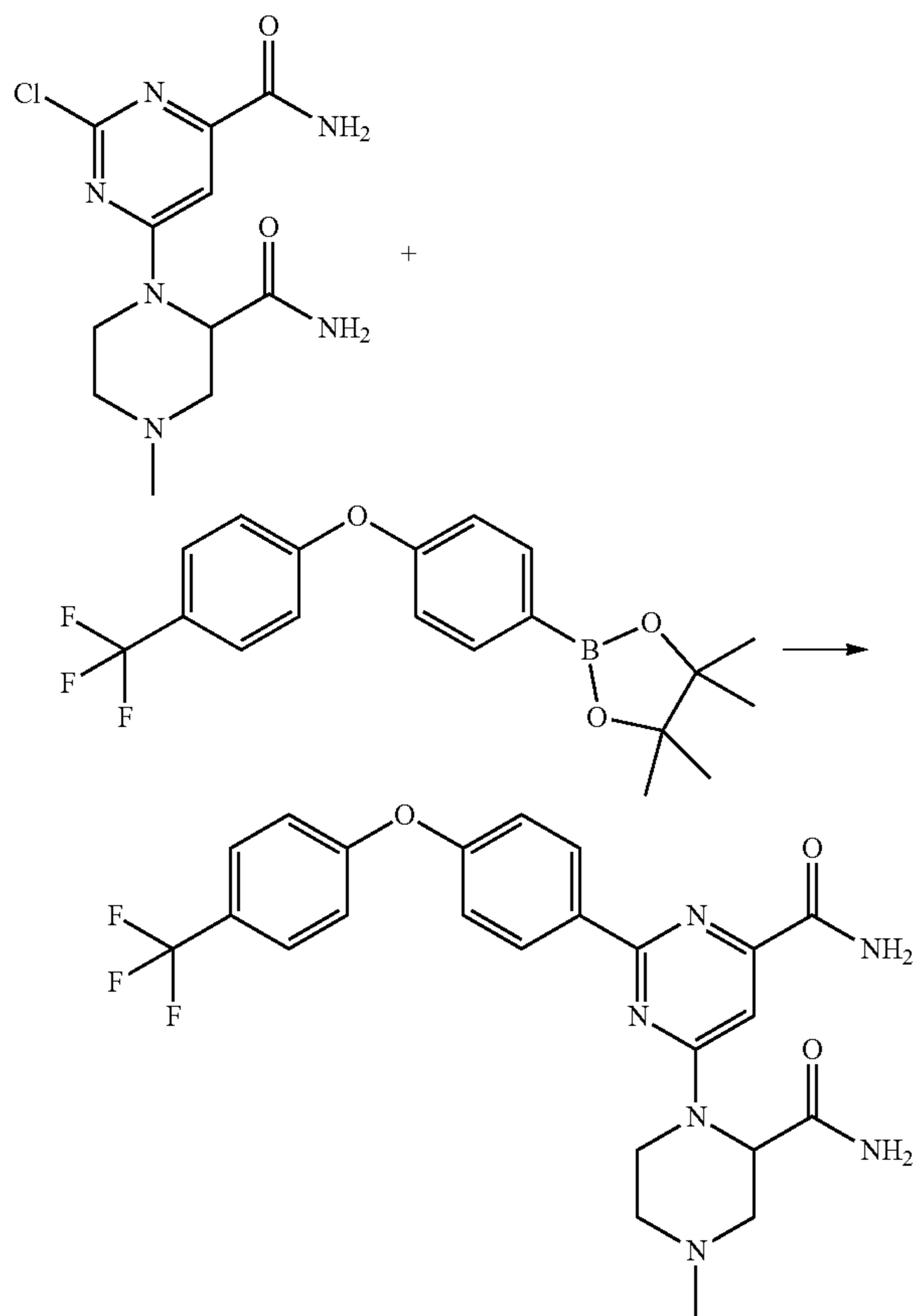
Scheme 64
