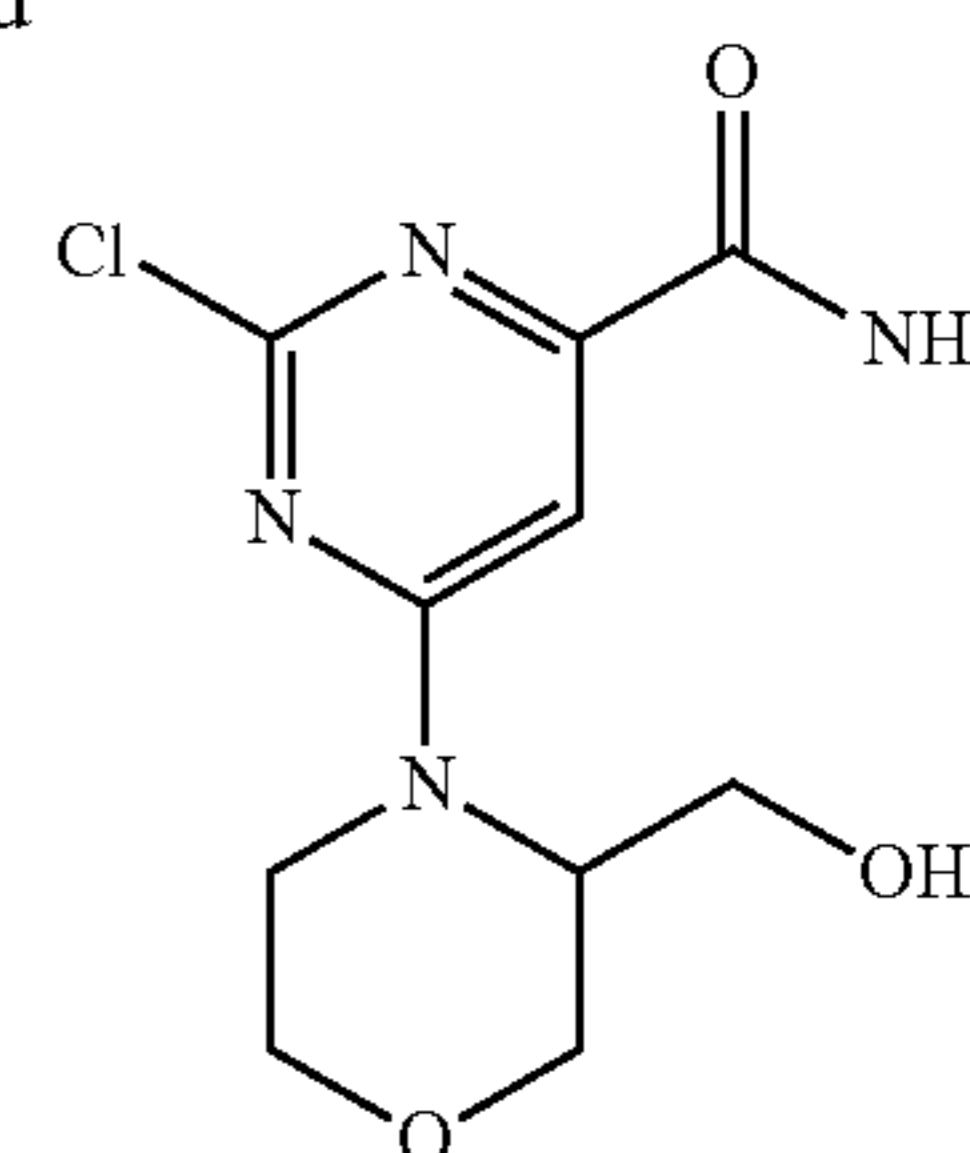
2-chloro-6-(3-(hydroxymethyl)morpholino)pyrimidine-4-carboxamide
