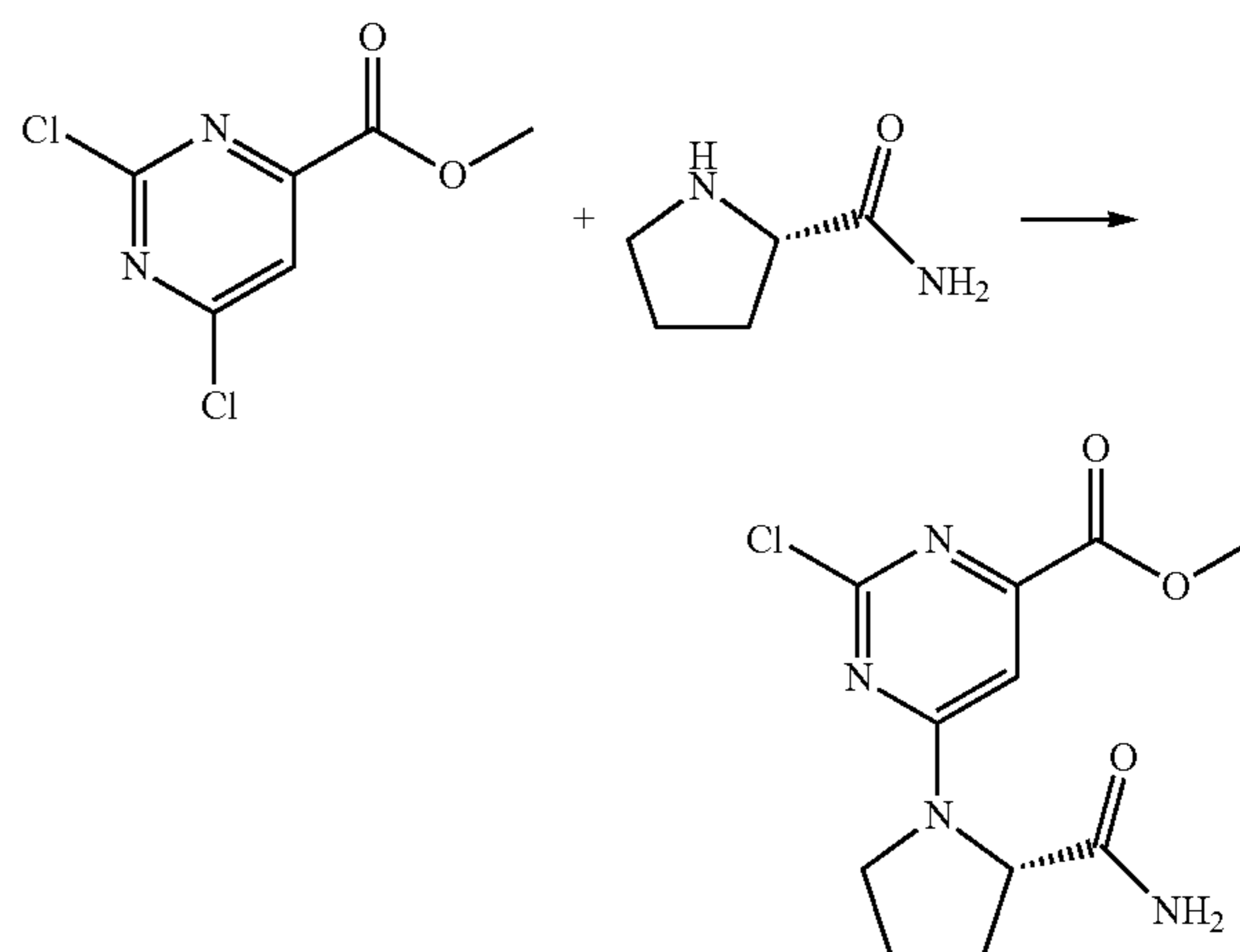
Scheme 55
