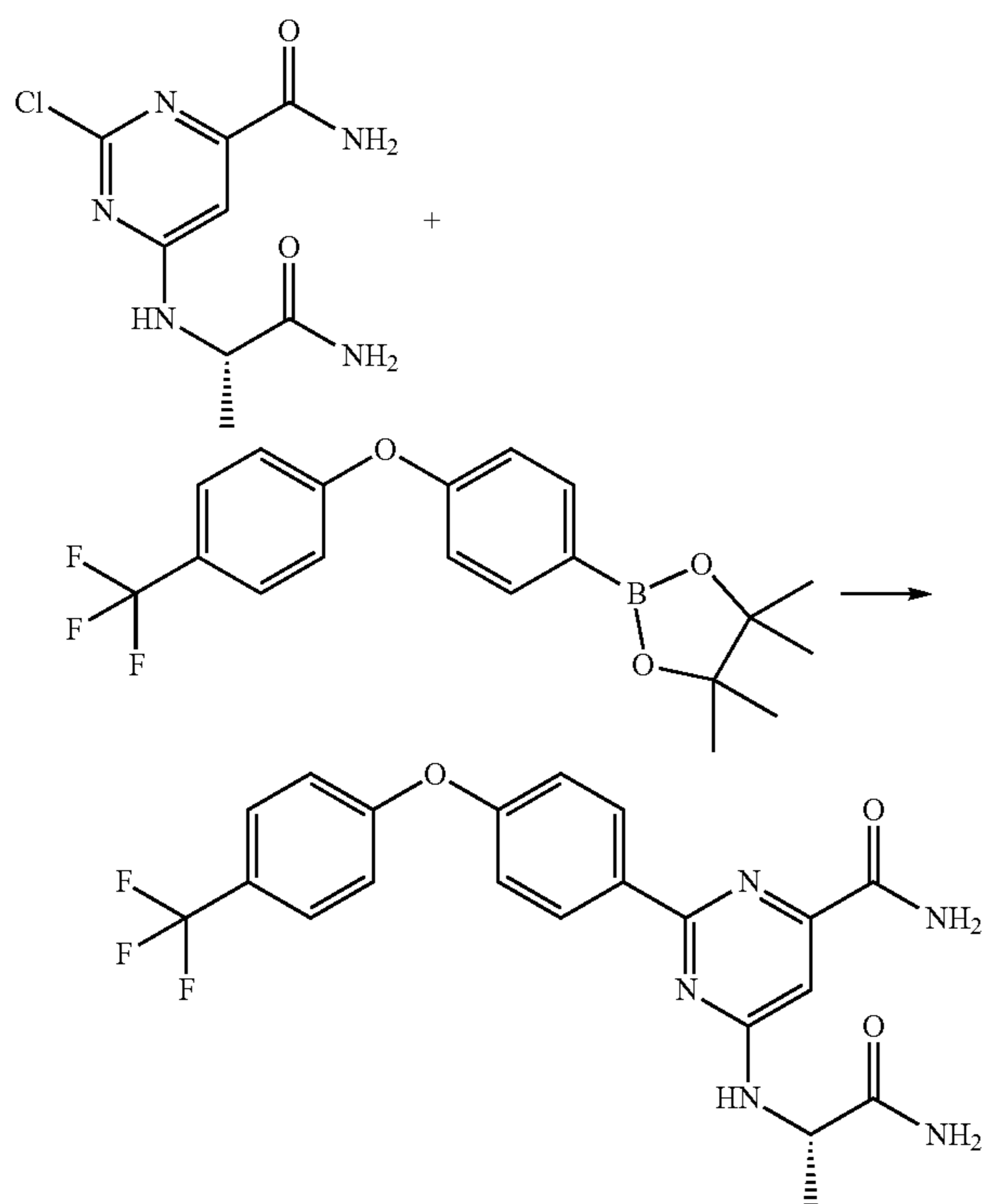
Scheme 19
