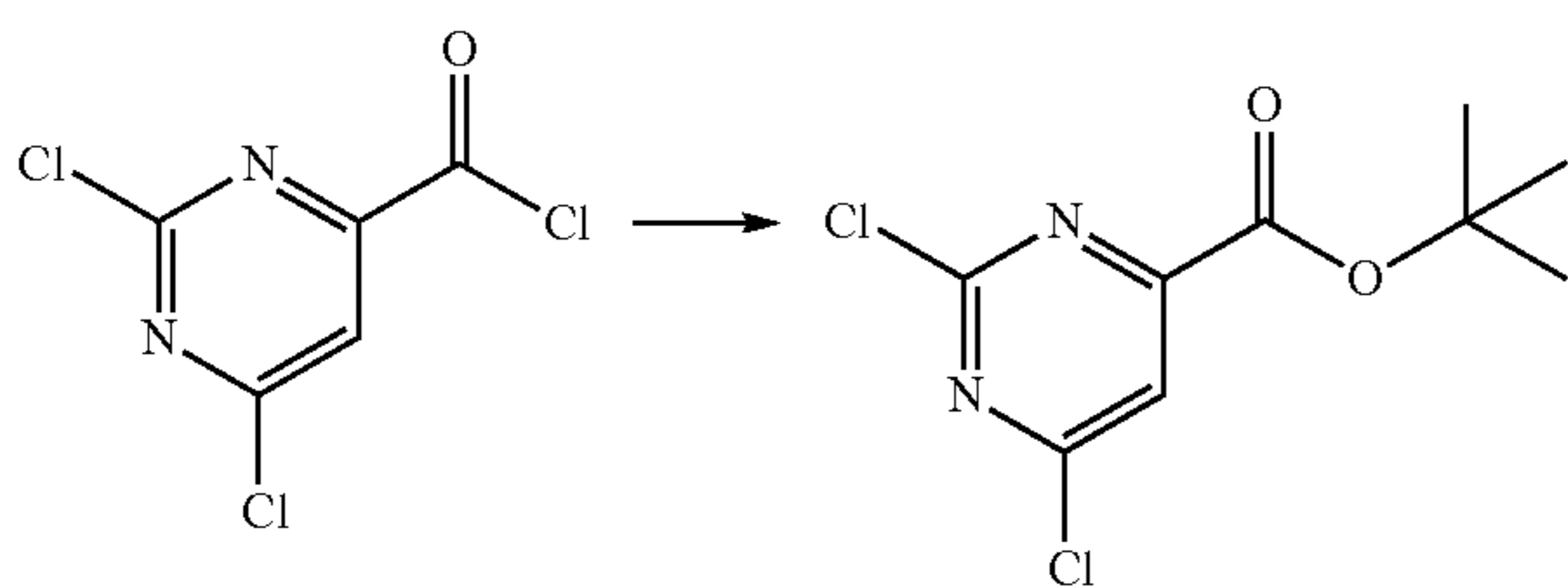
Scheme 10
