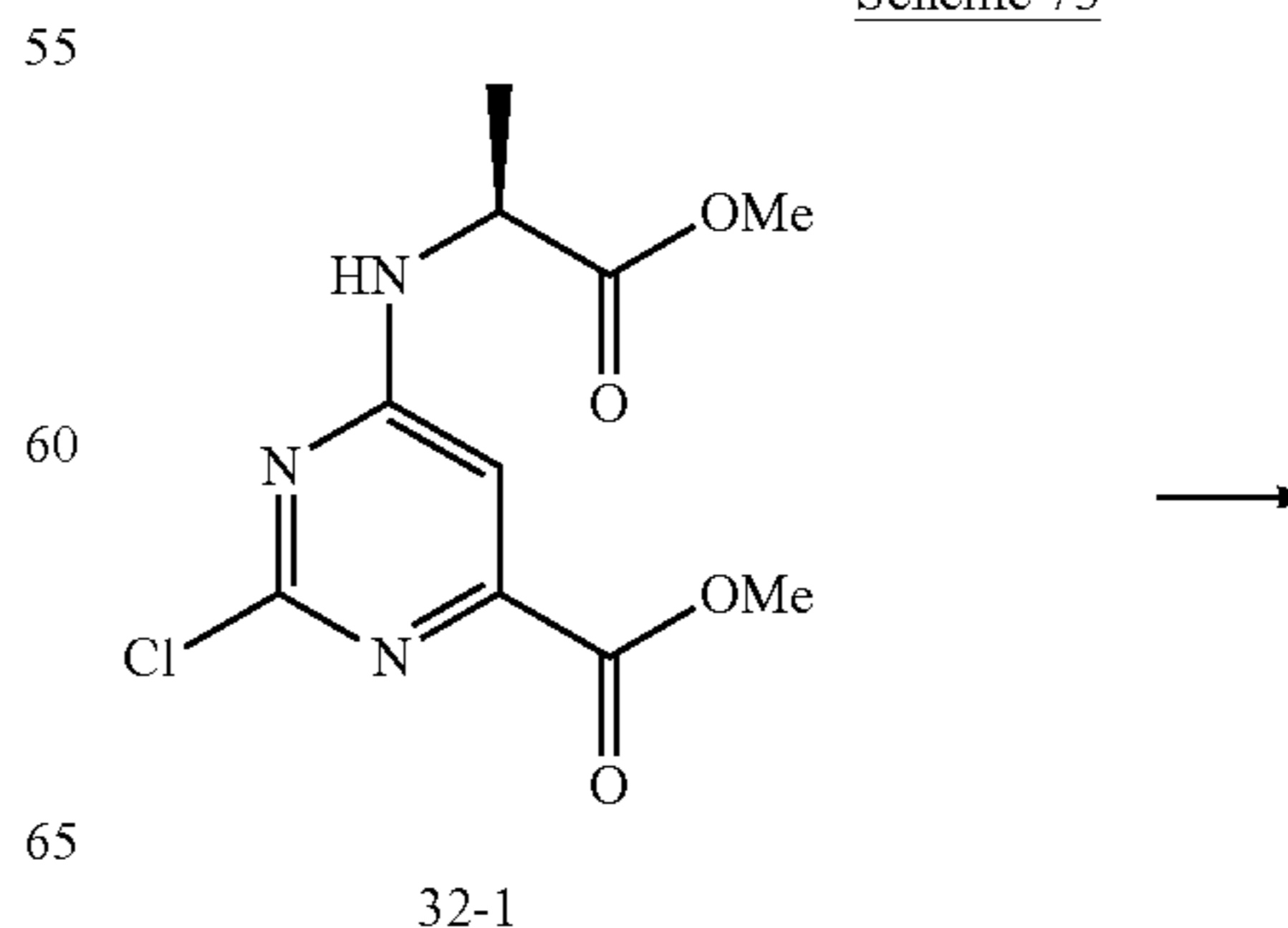
Scheme 73
