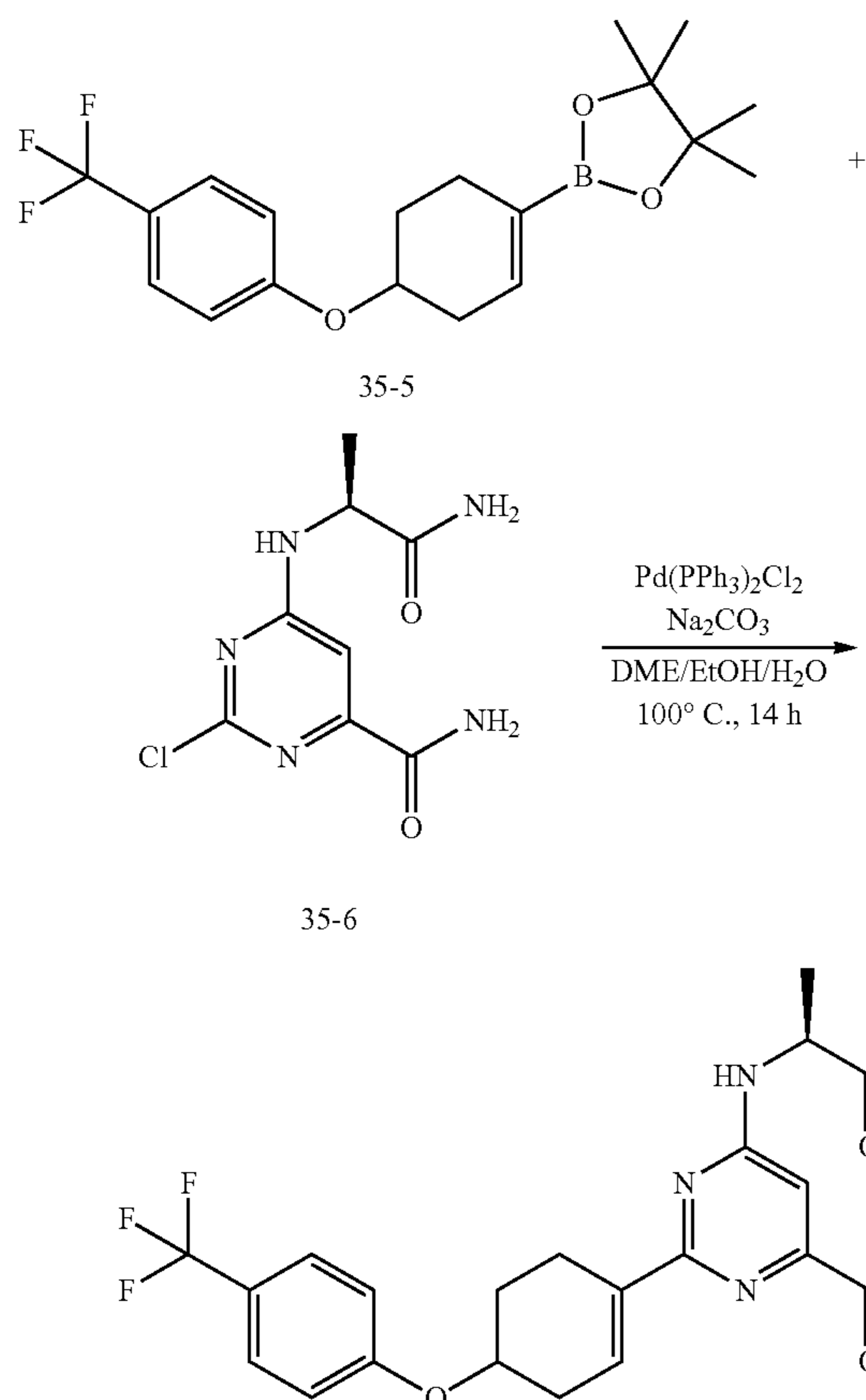
Scheme 81
