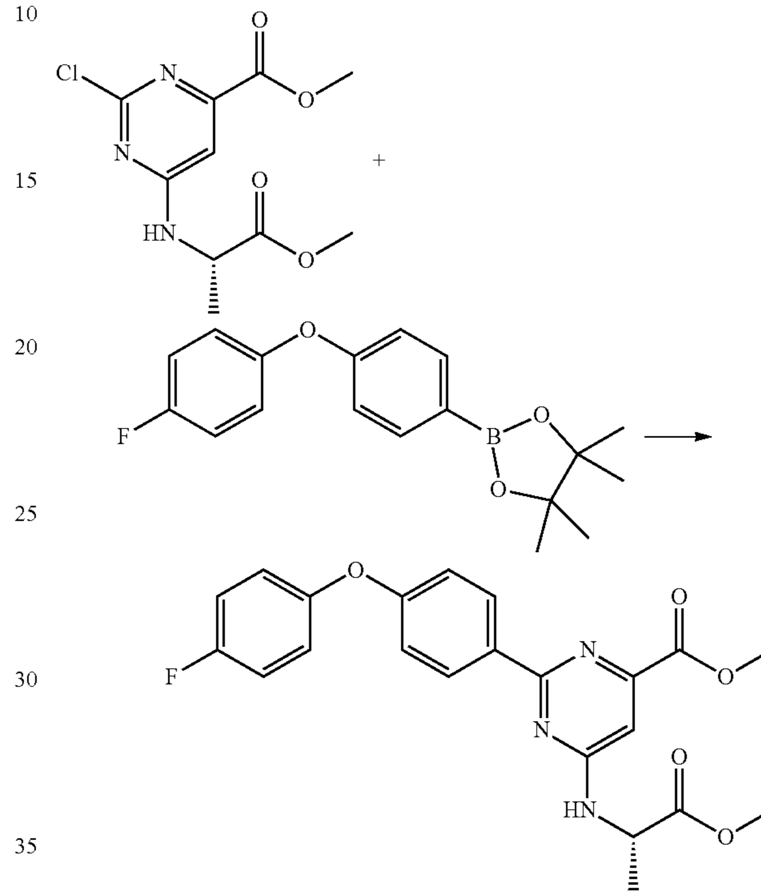
Scheme 20
