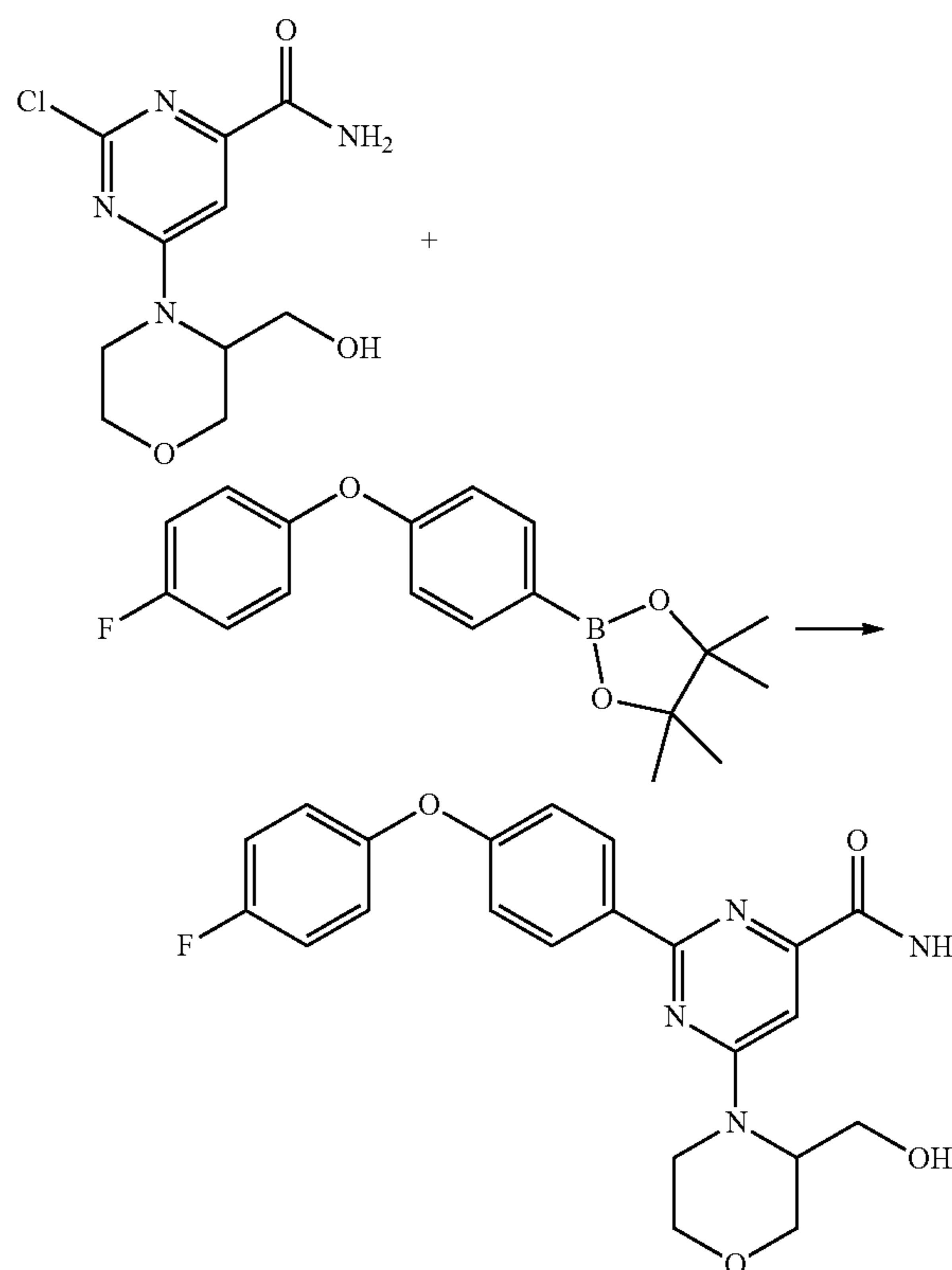
Scheme 23
