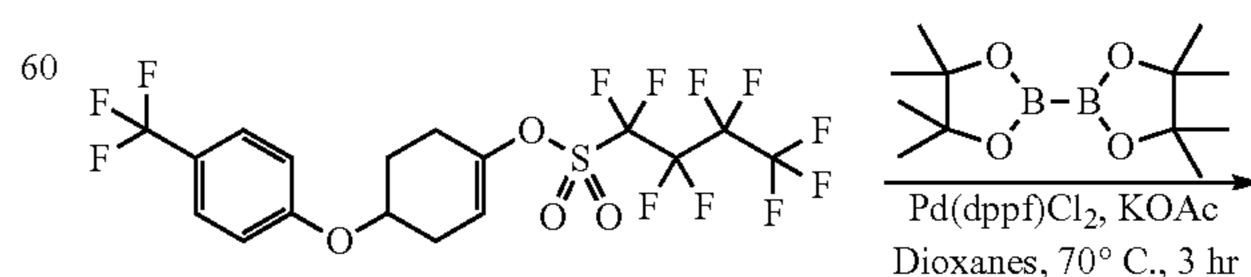
Scheme 80
