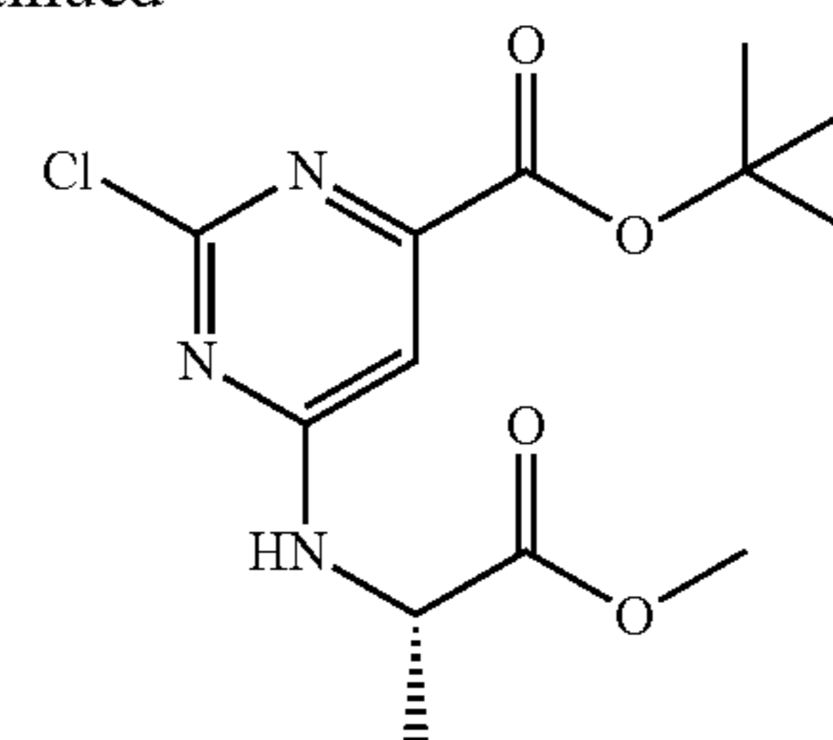
(S)-tert-butyl 2-chloro-6-((1-methoxy-1-oxopropan-2-yl)amino)pyrimidine-4-carboxylate
