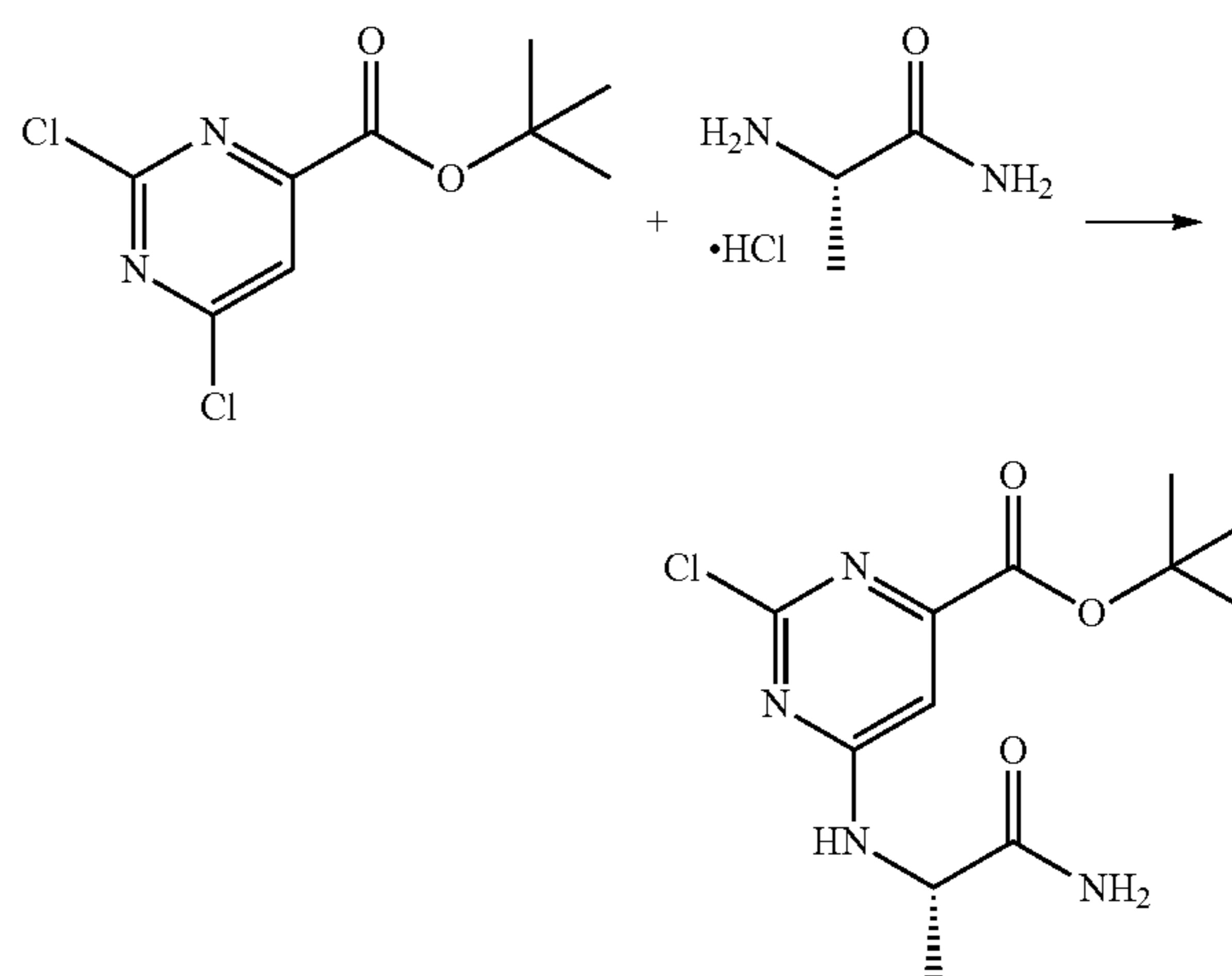
Scheme 14
