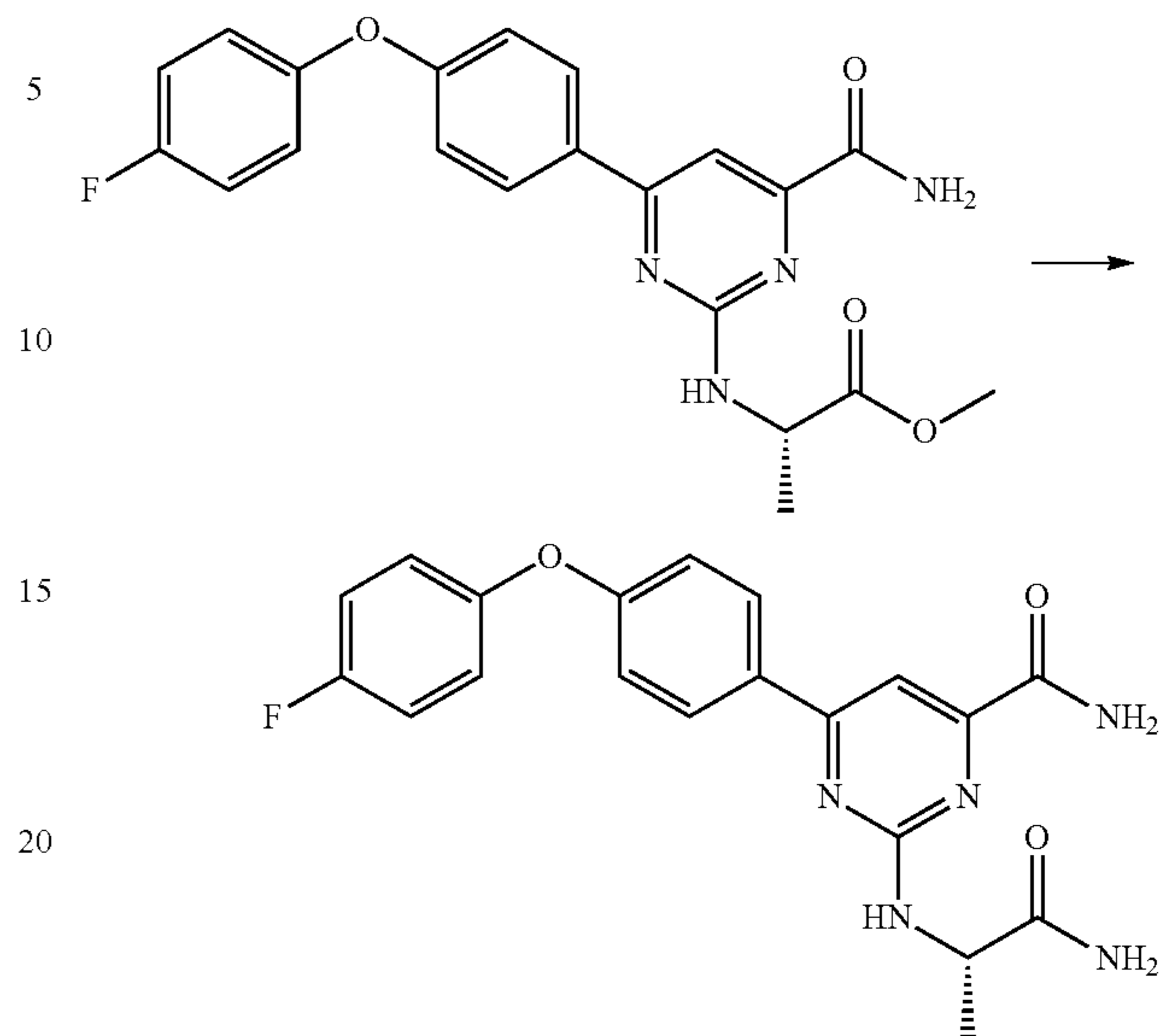
Scheme 38
