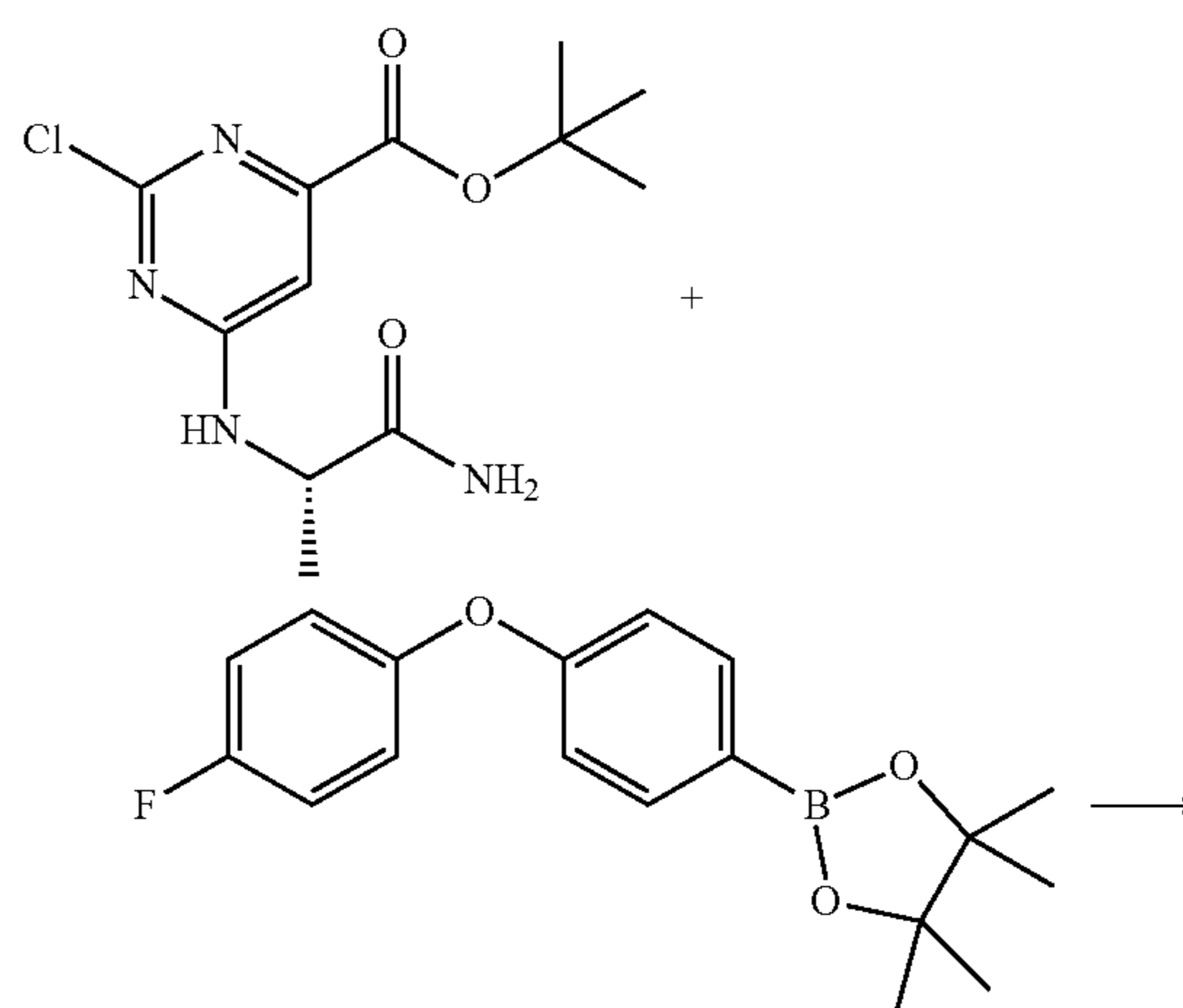
Scheme 15
