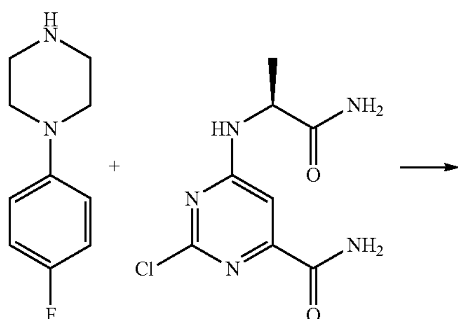
Scheme 54
