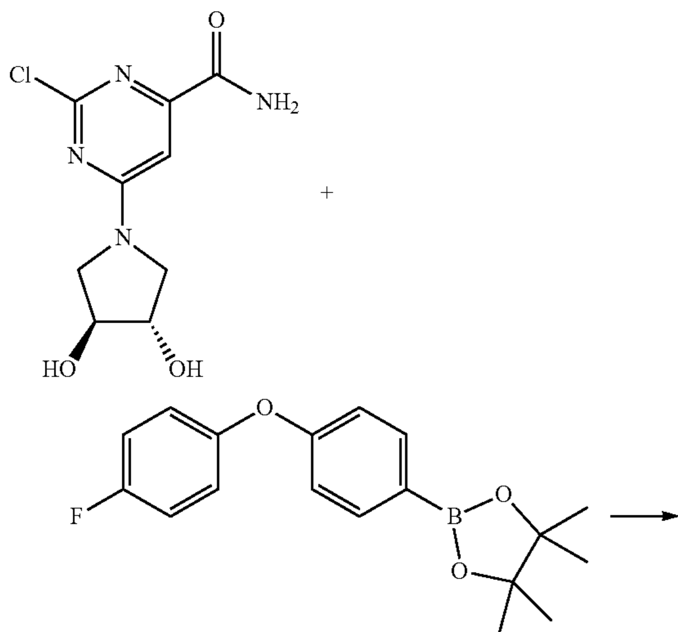
Scheme 60
