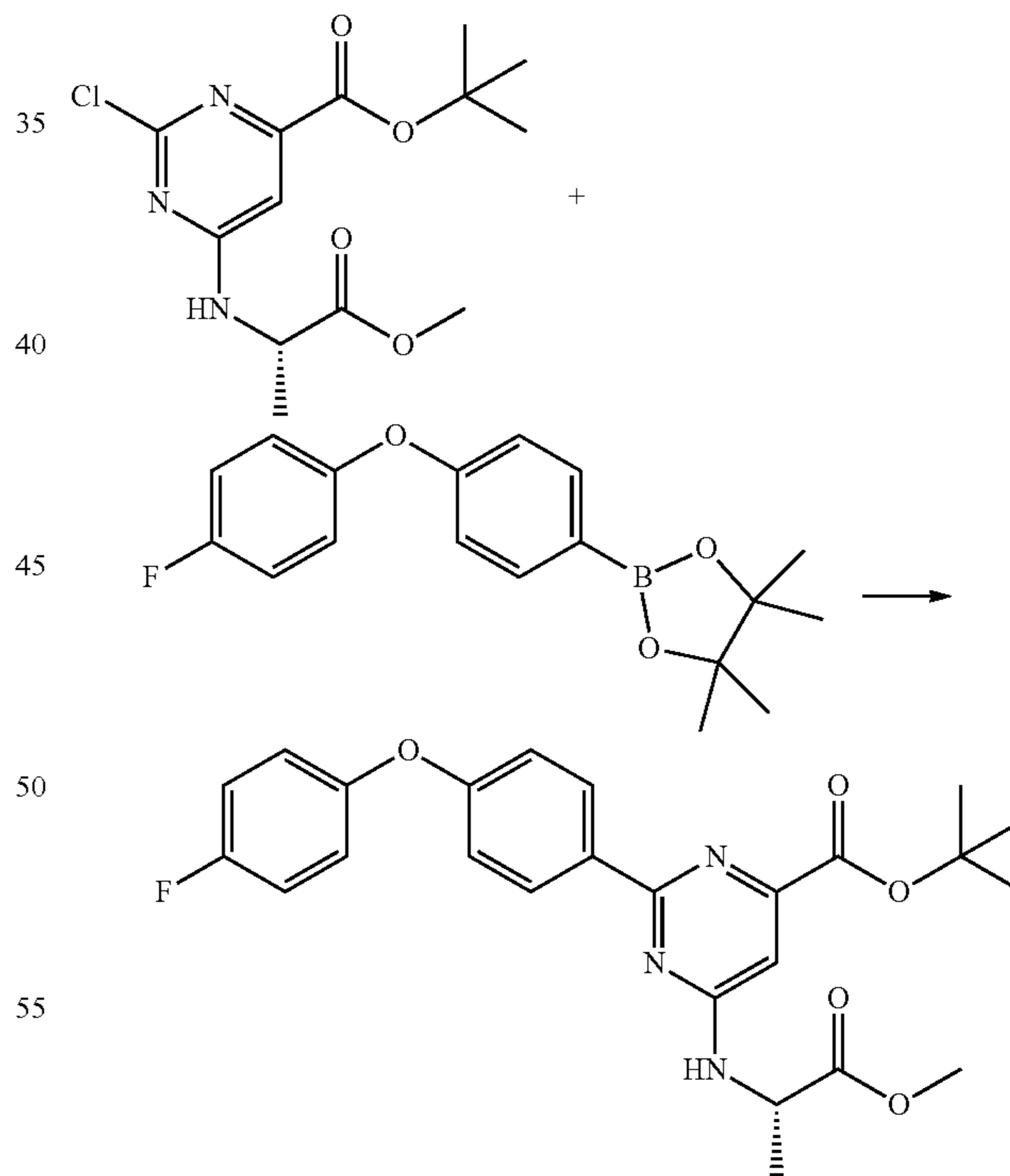
Scheme 12
