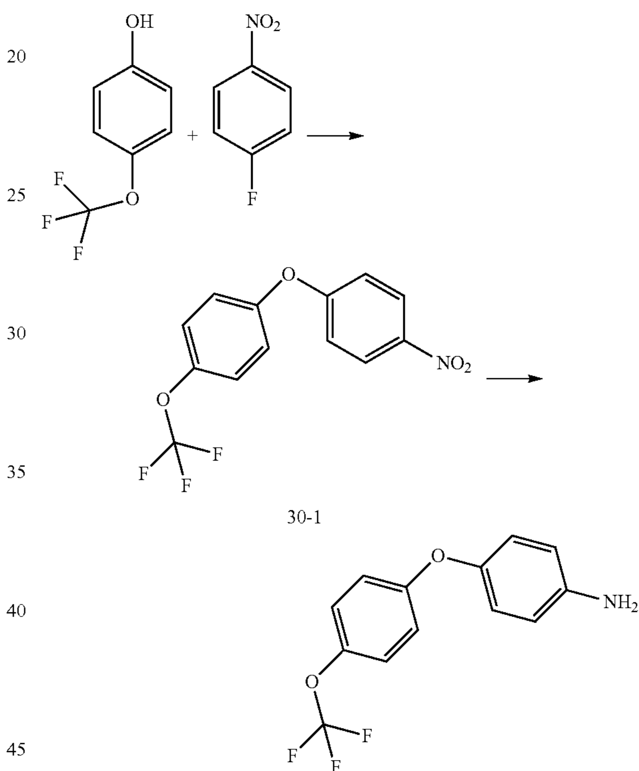
Scheme 65
