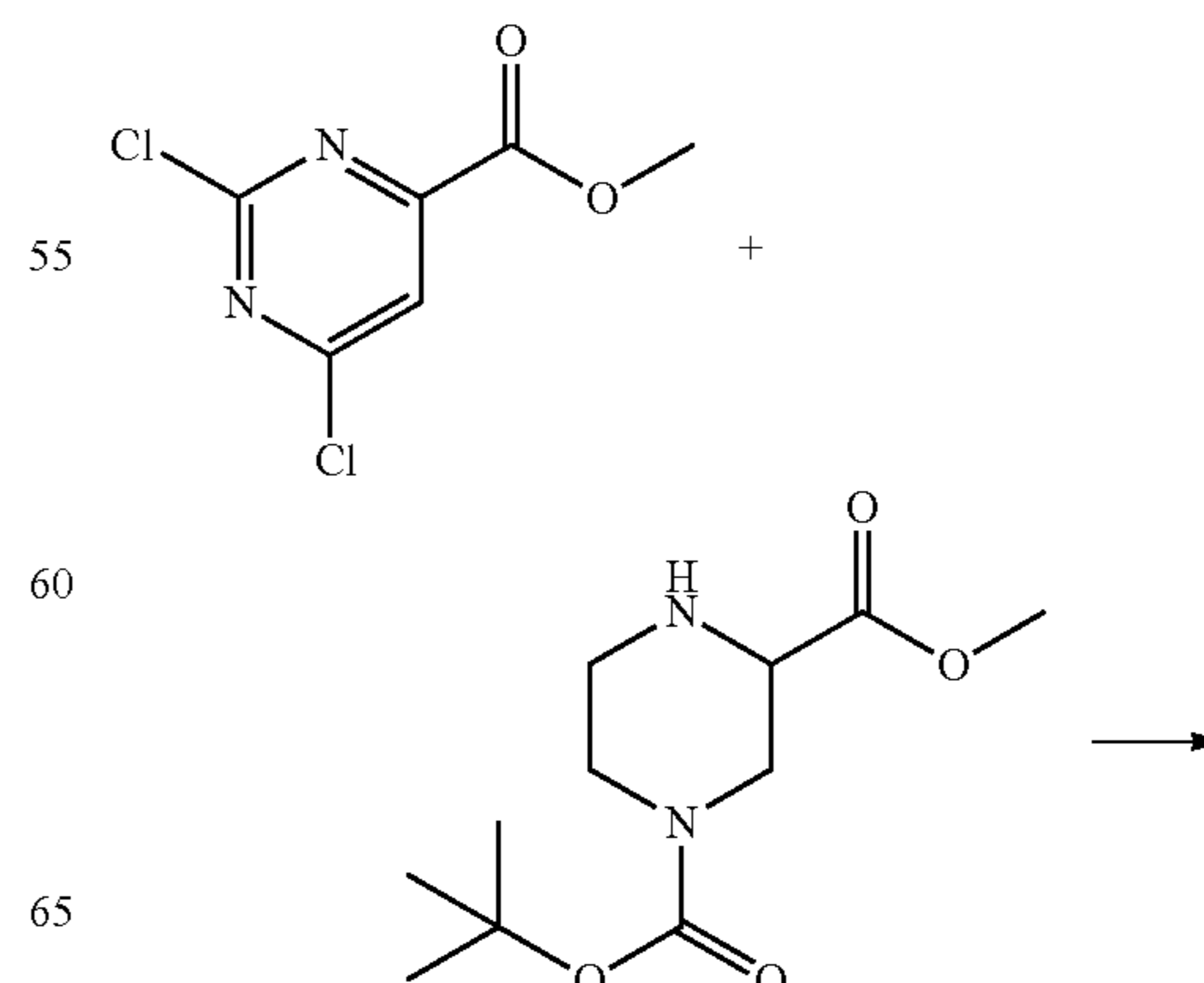
Scheme 61
