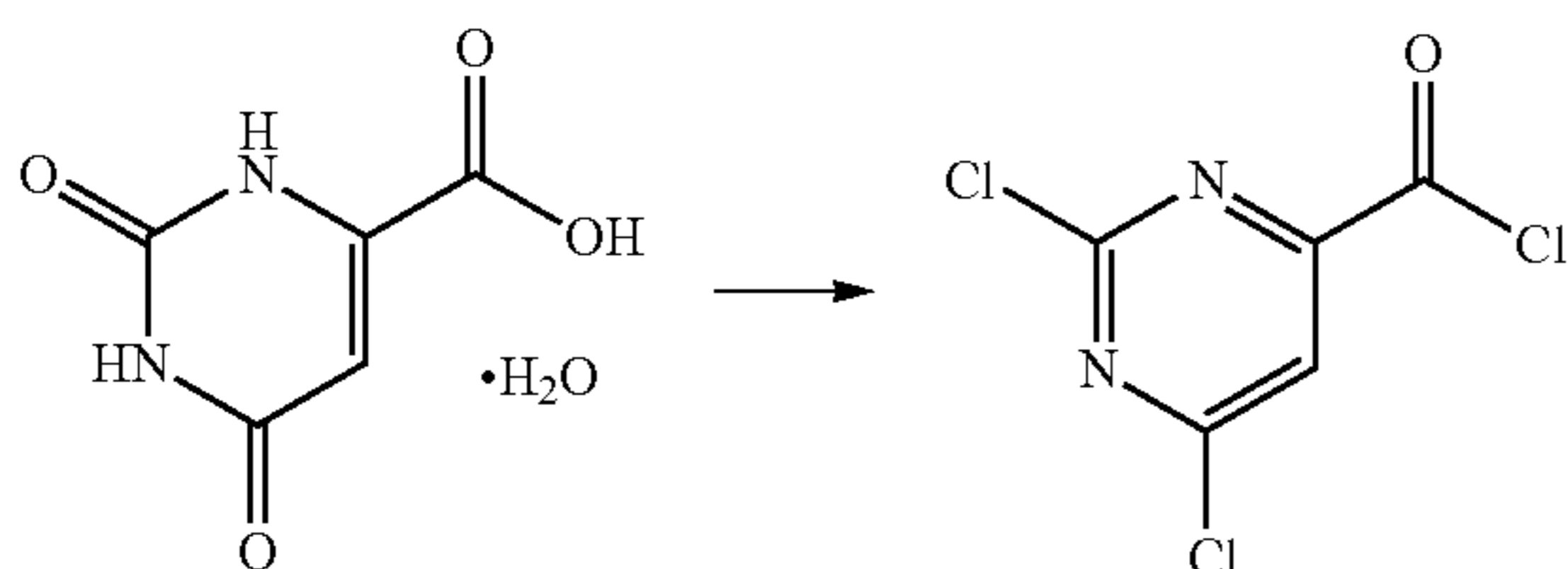
Scheme 2
