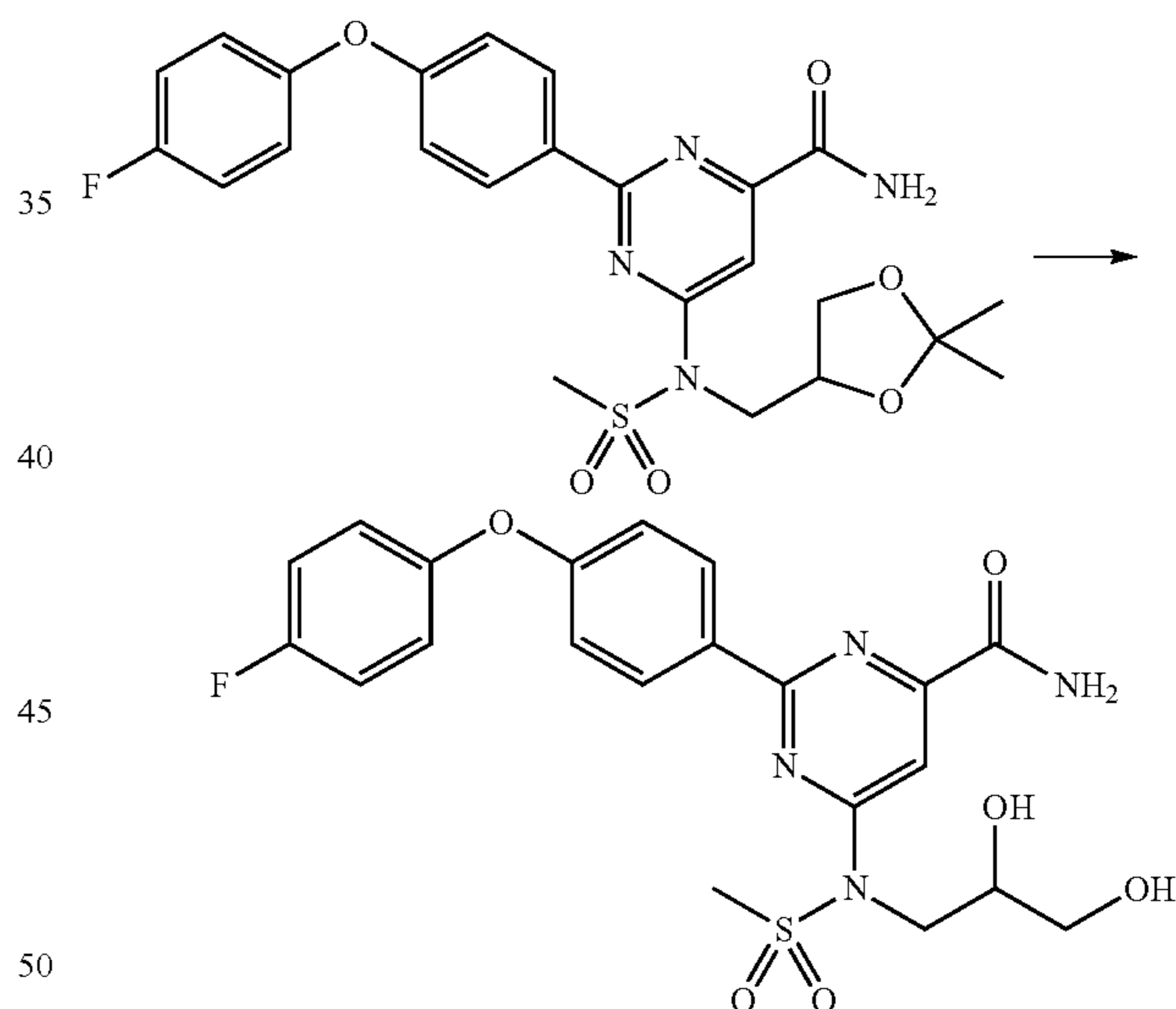
Scheme 36
