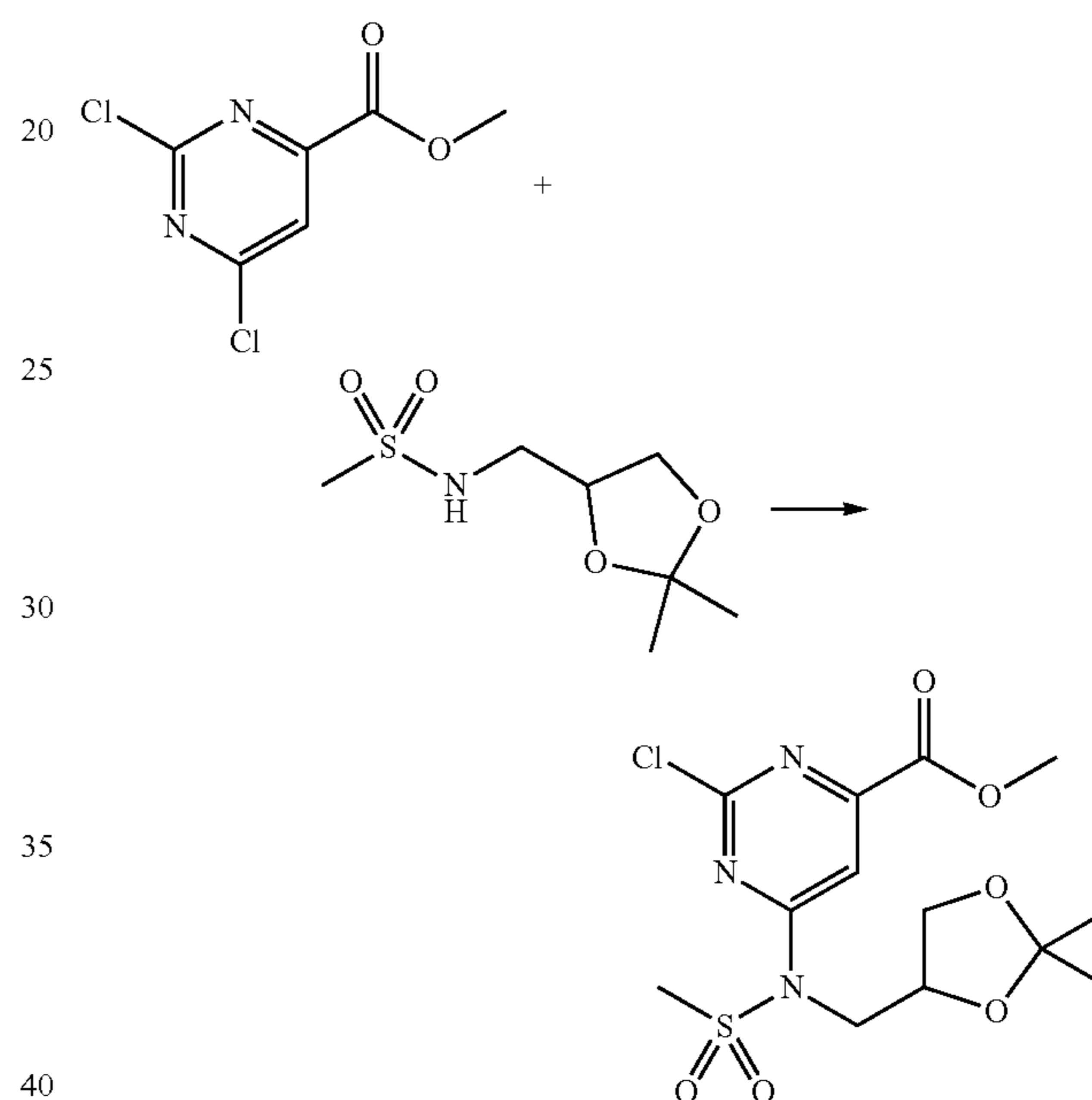
Scheme 33
