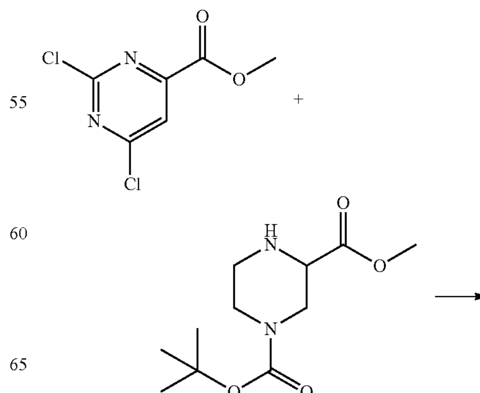
Scheme 61
