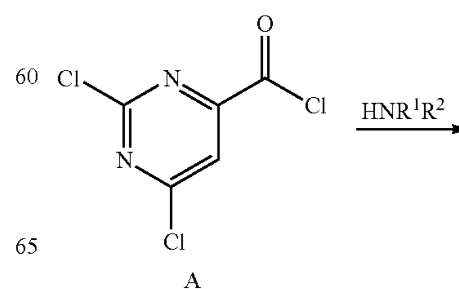
General Scheme 1
