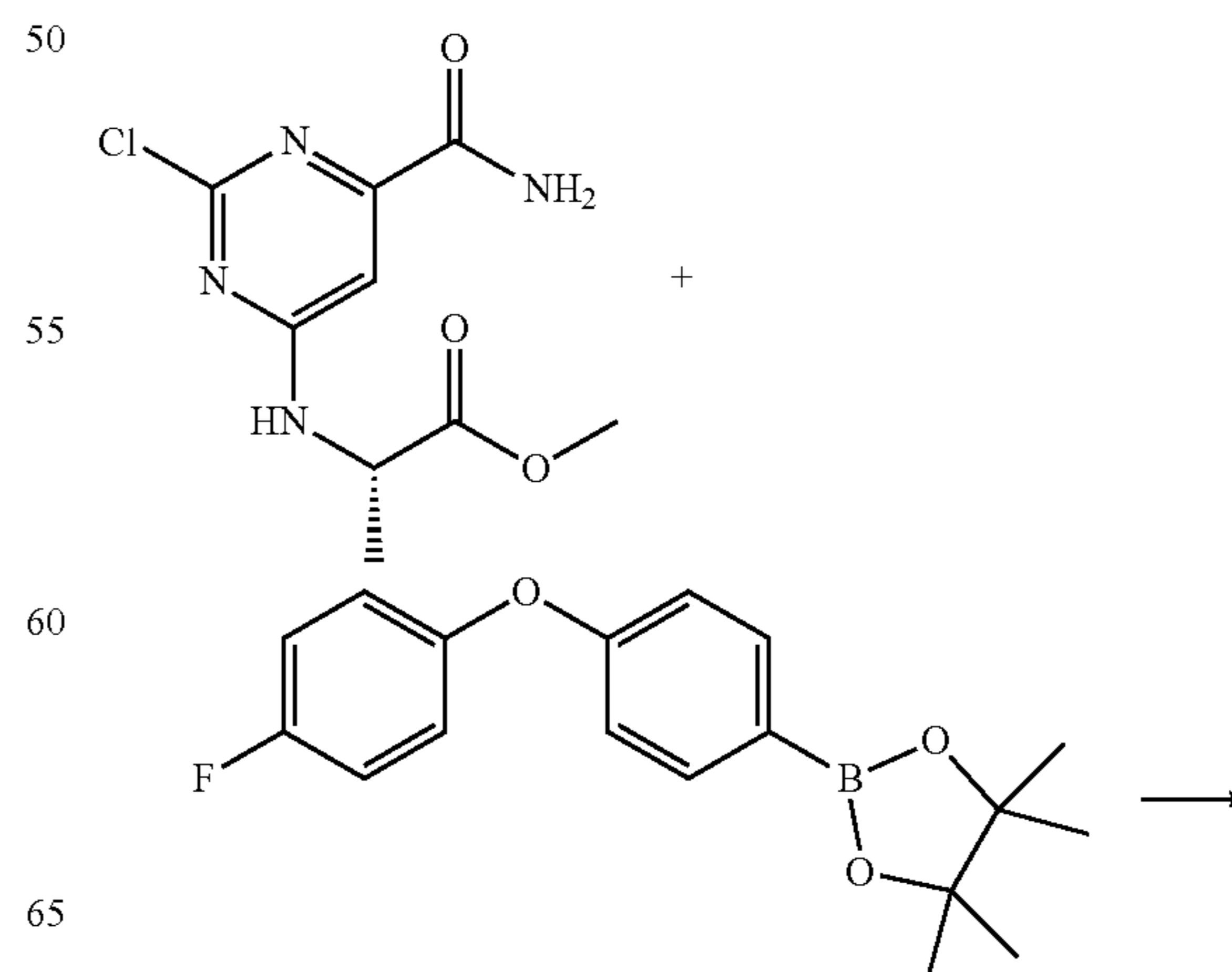
Scheme 5
