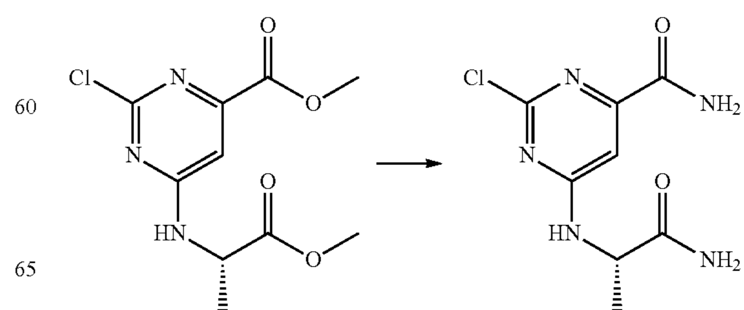
Scheme 18
