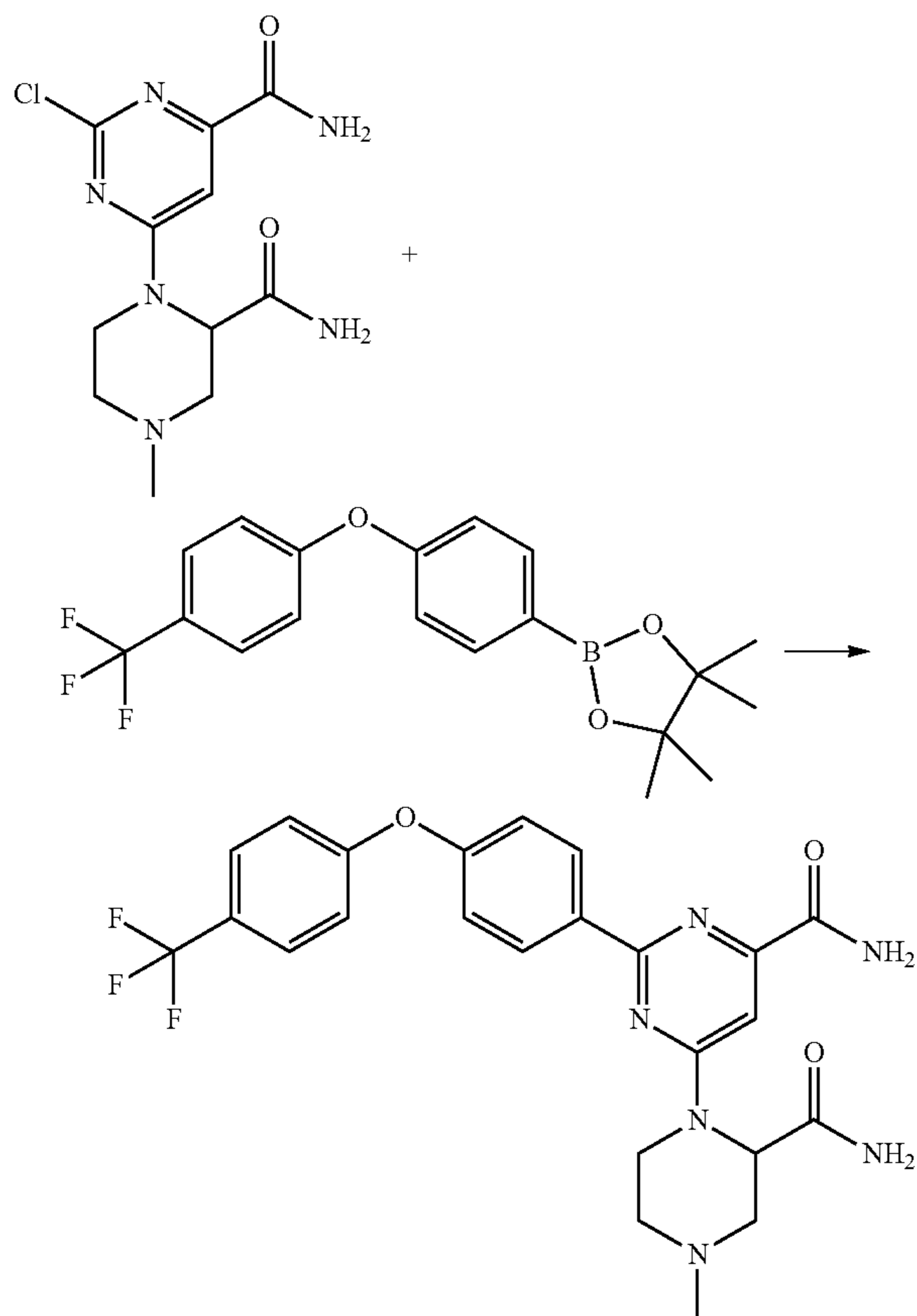
Scheme 64
