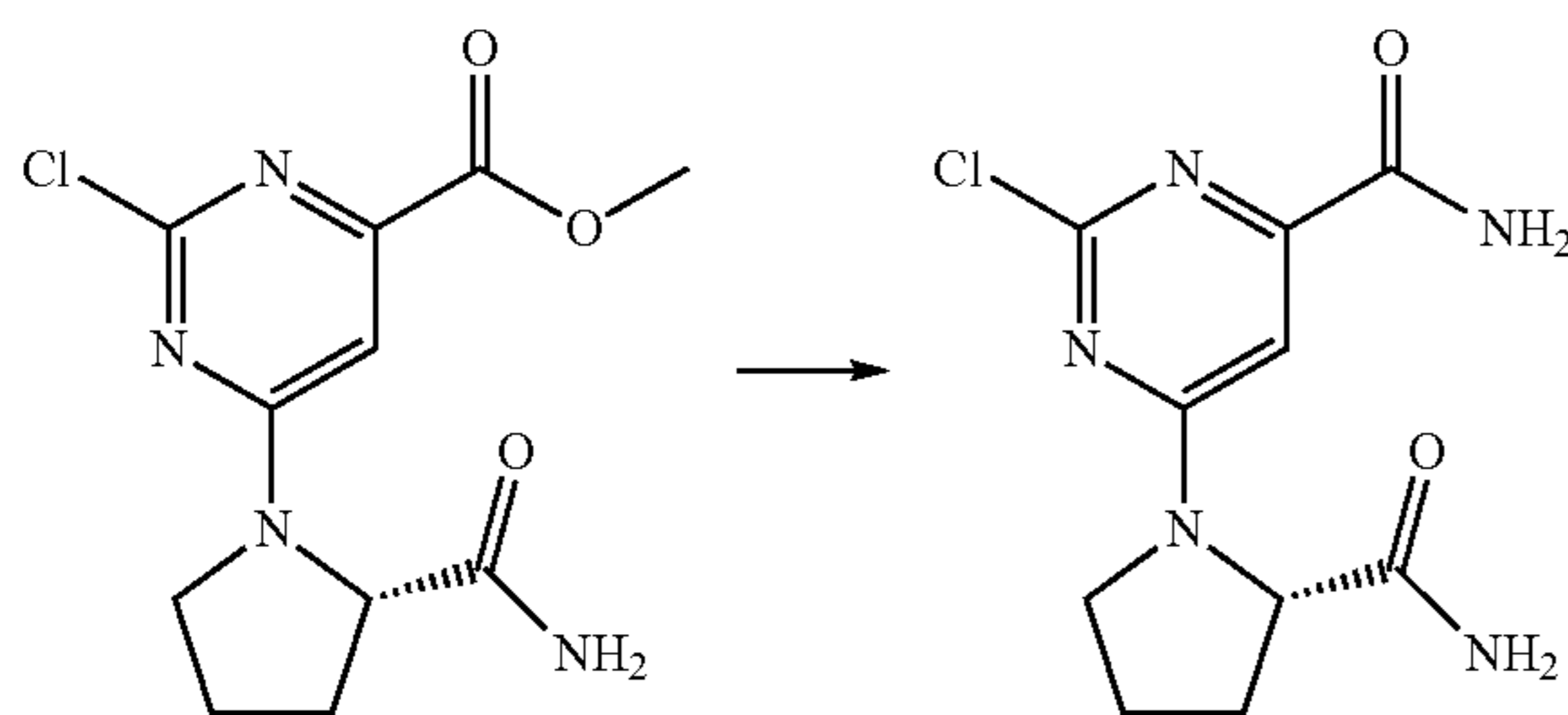
Scheme 56
