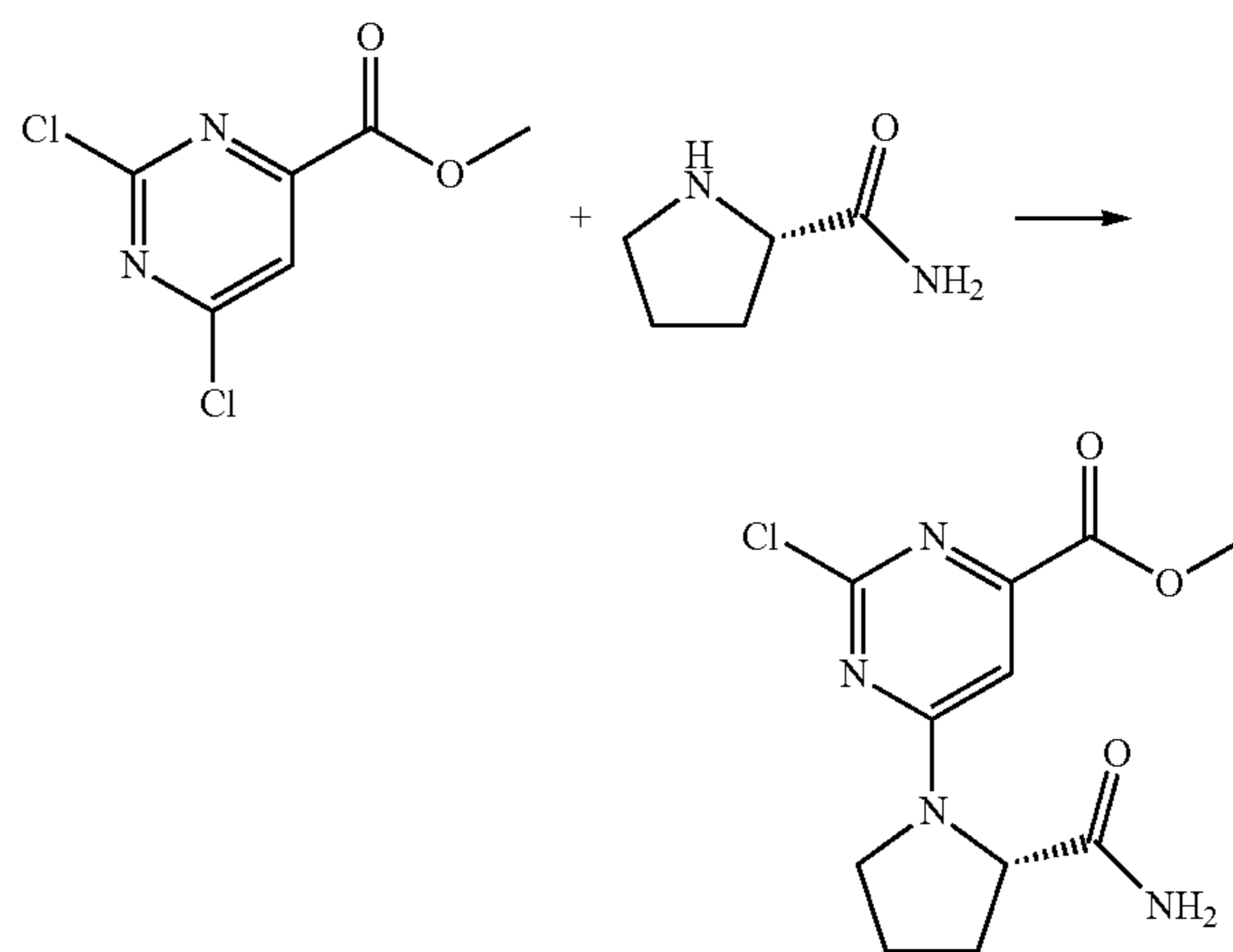
Scheme 55
