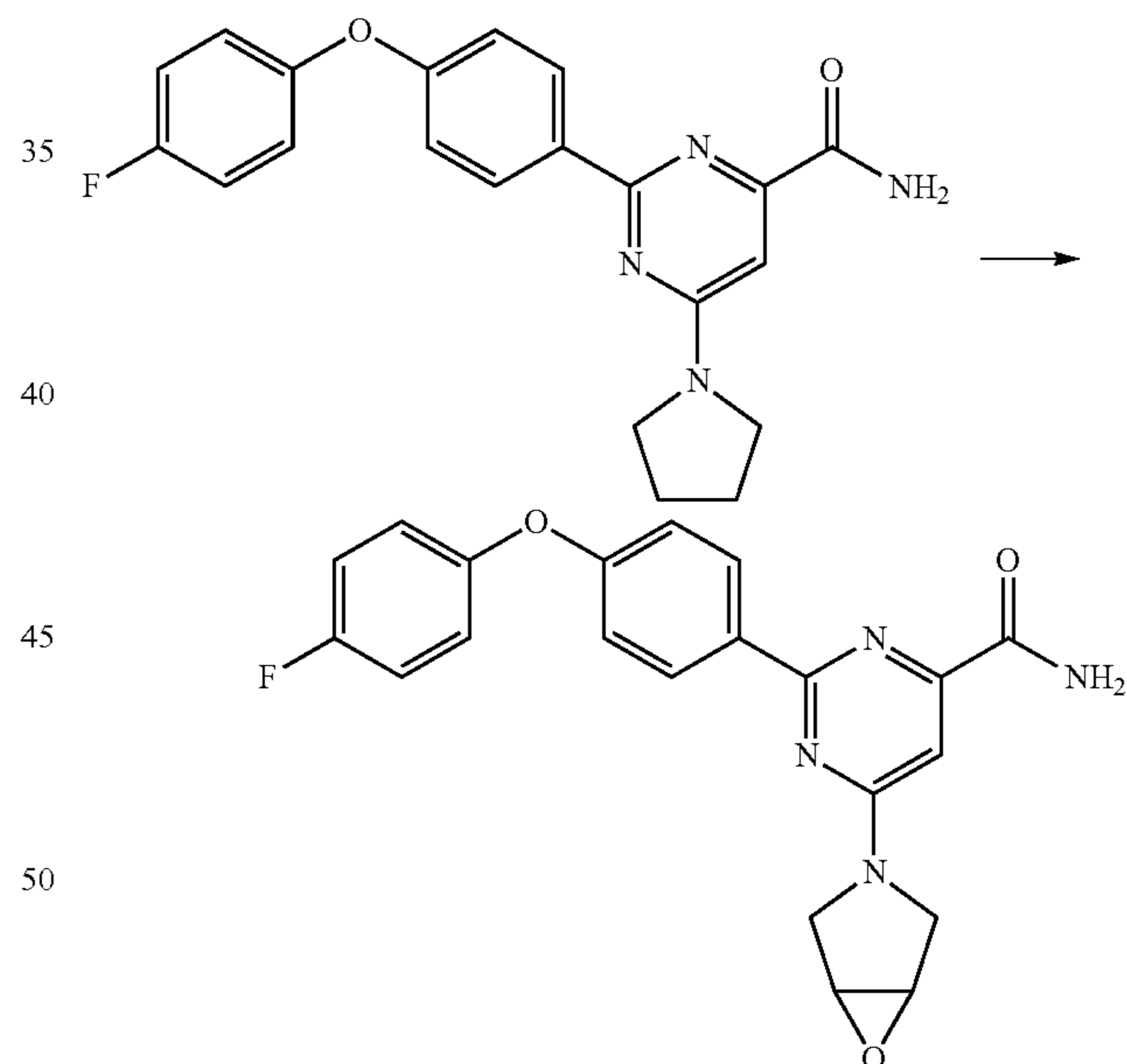
Scheme 25
