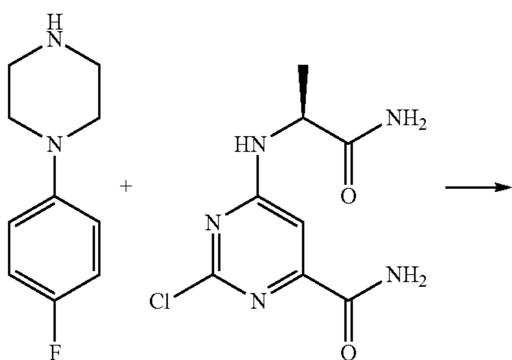
Scheme 54
