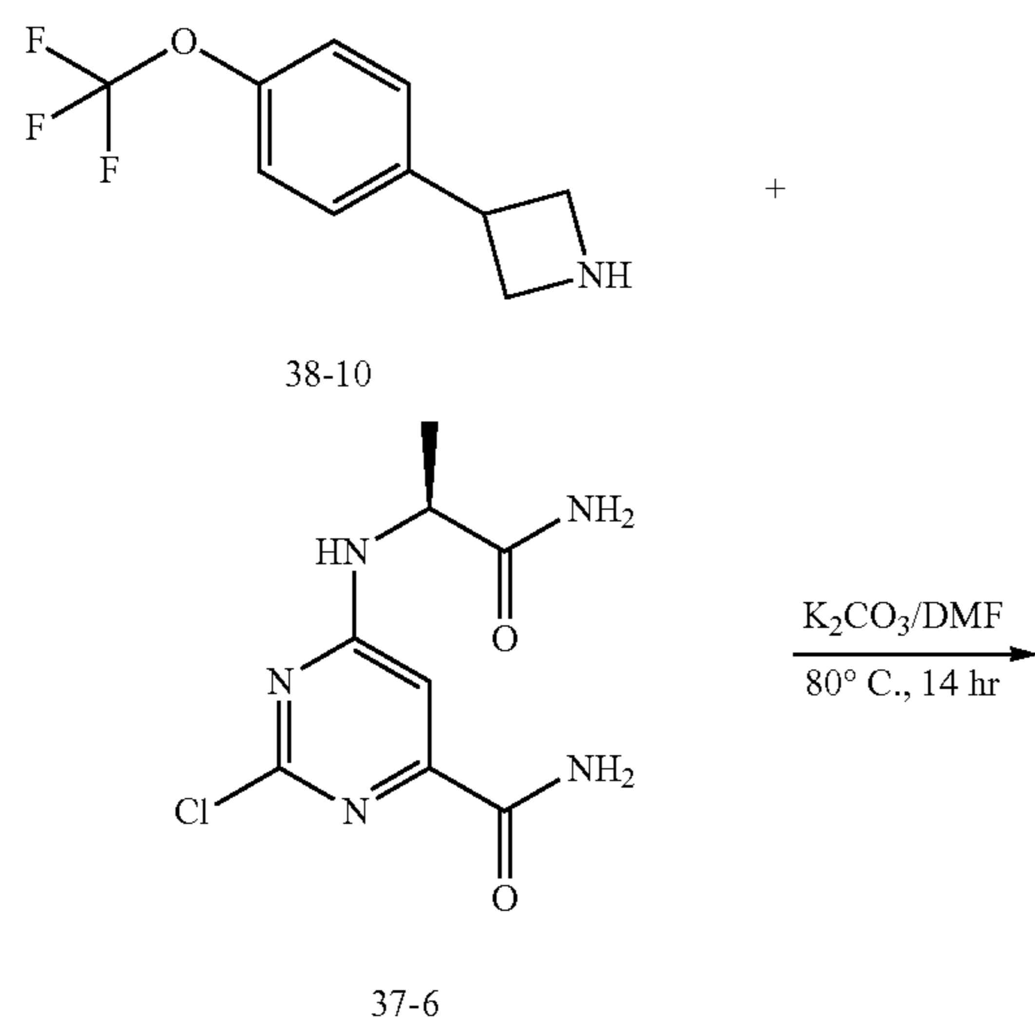
Scheme 86
