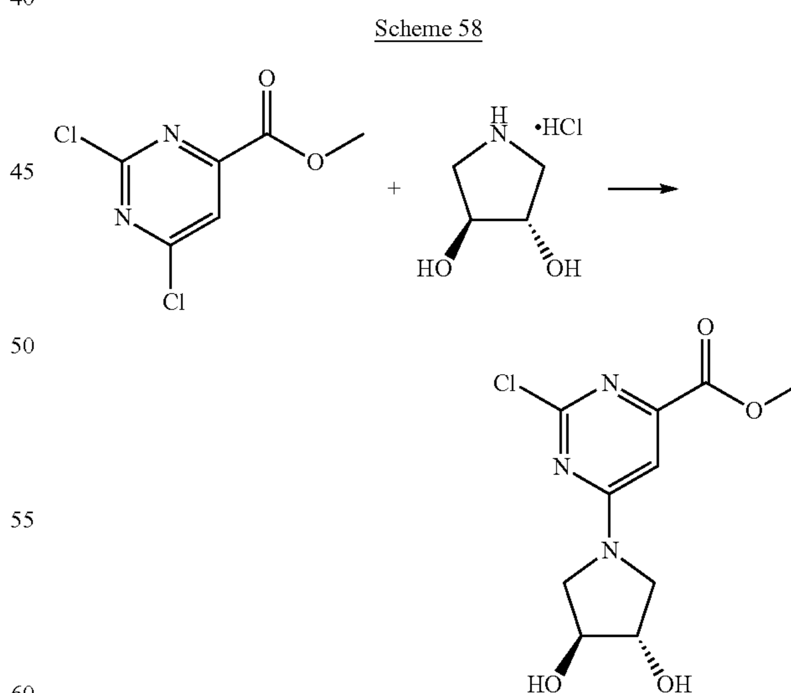
Methyl 2-chloro-6-((3S,4S)-3,4-dihydroxypyrrolidin-1-yl)pyrimidine-4-carboxylate
