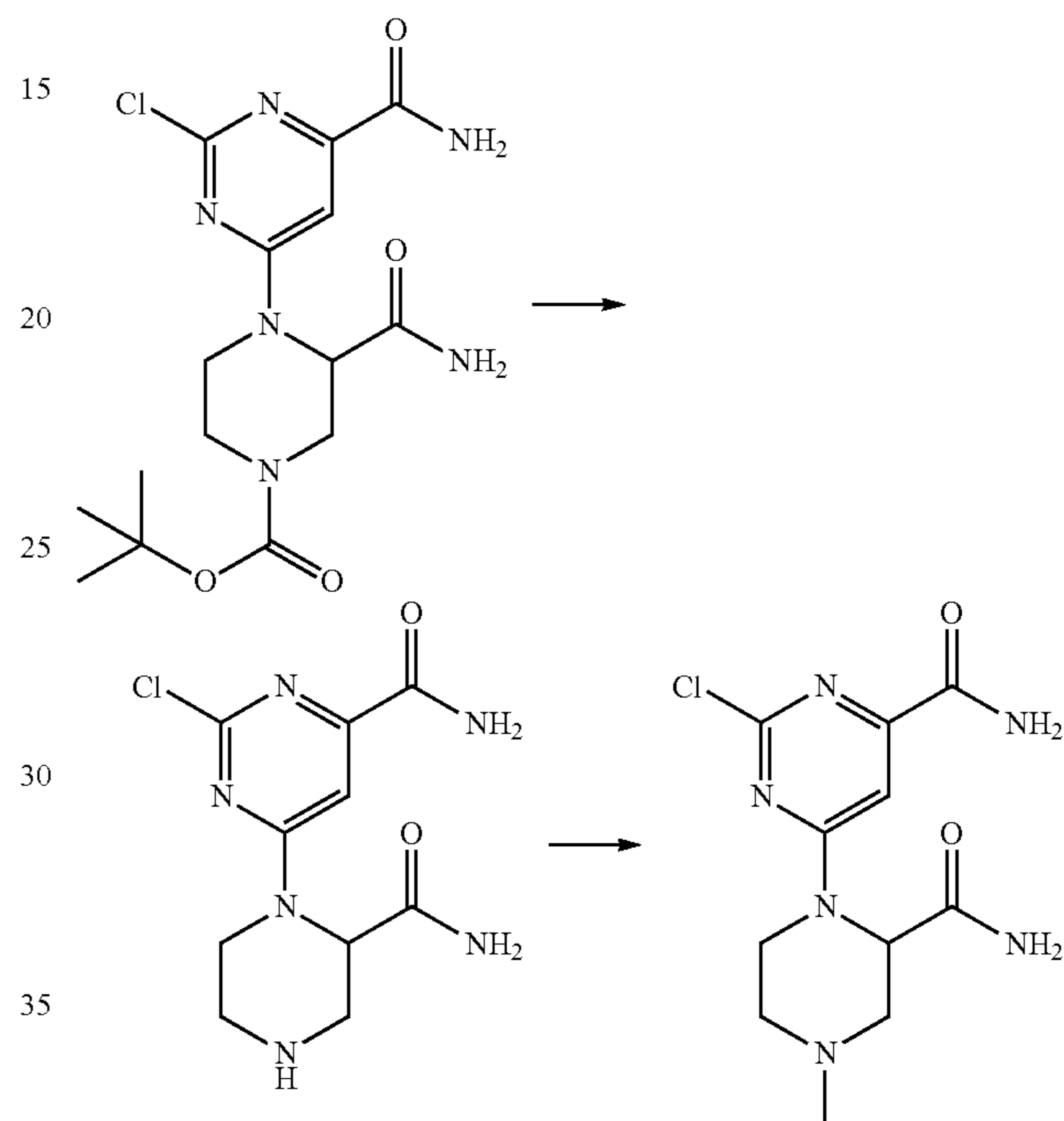
Scheme 63
