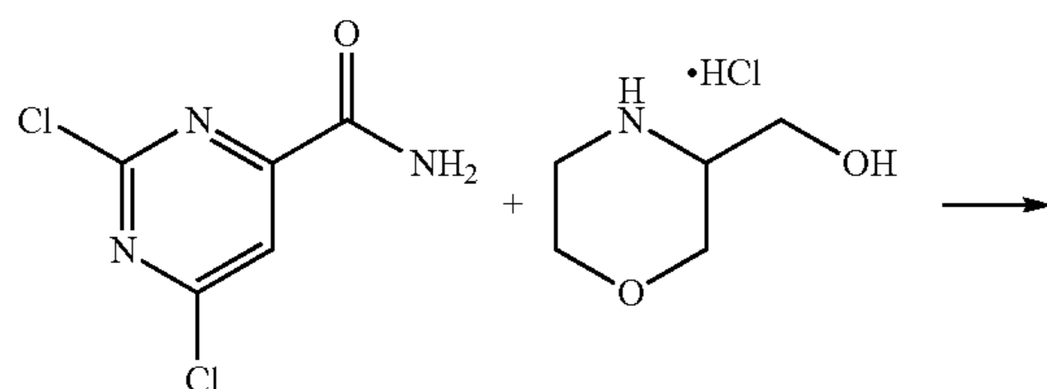
Scheme 22
