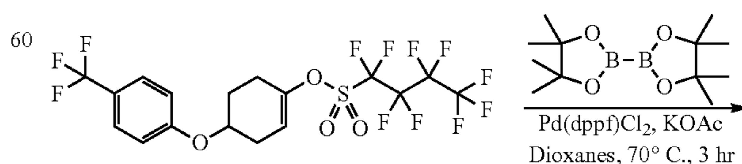
Scheme 80
