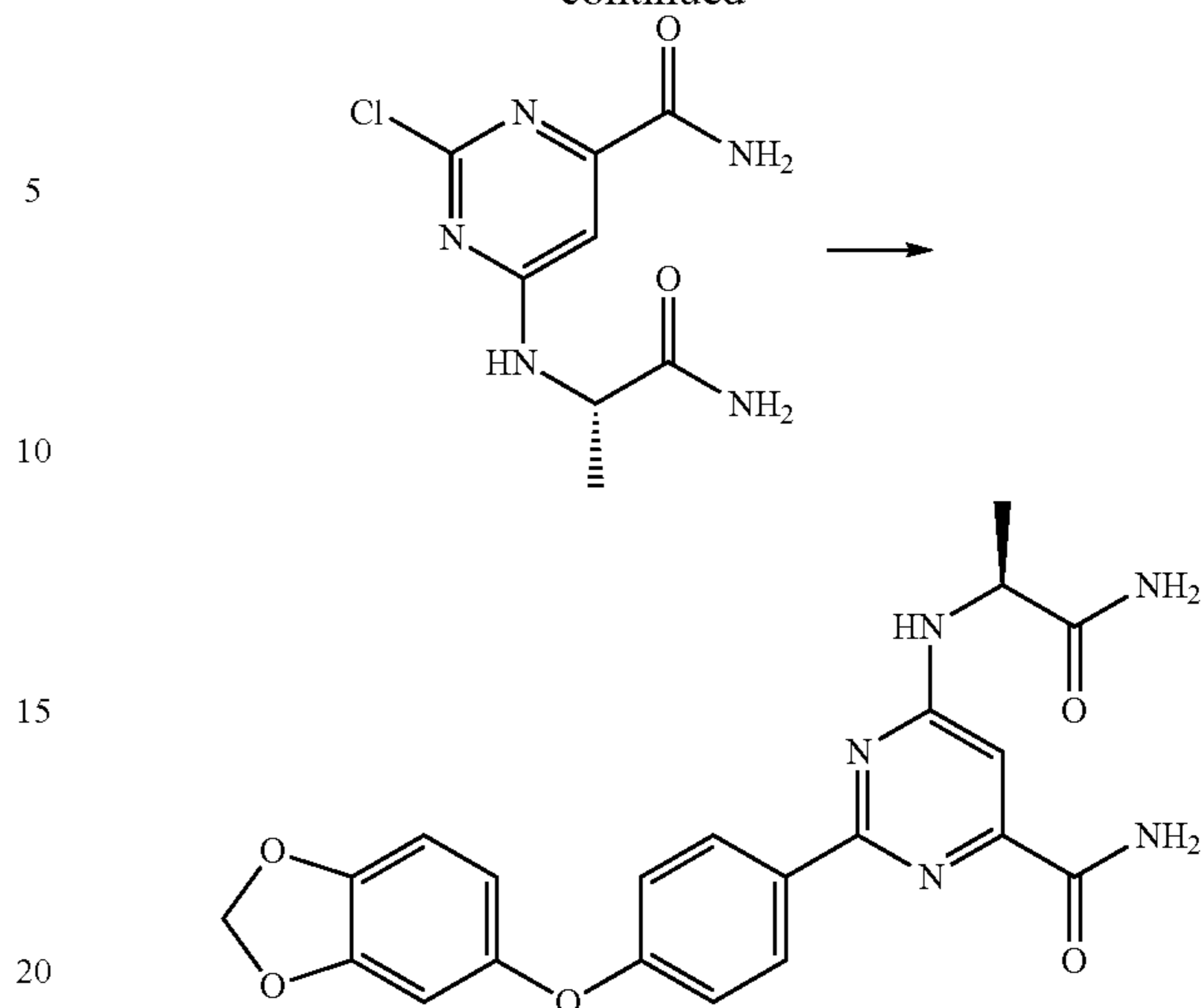
(S)-6-((1-amino-1-oxopropan-2-yl)amino)-2-(4-(benzo[d][1,3]dioxol-5-yloxy)phenyl)pyrimidine-4-carboxamide
