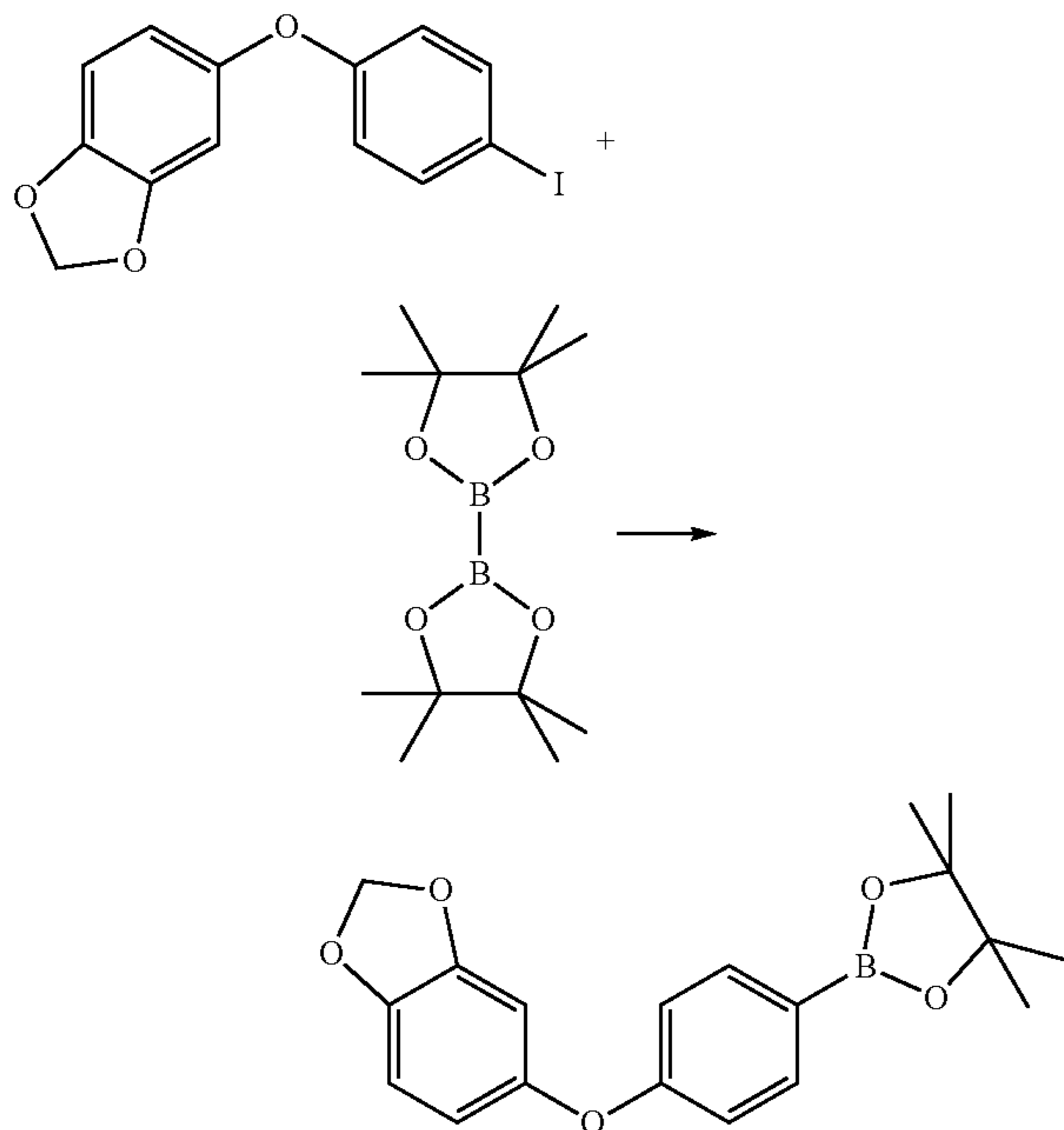
Scheme 71
