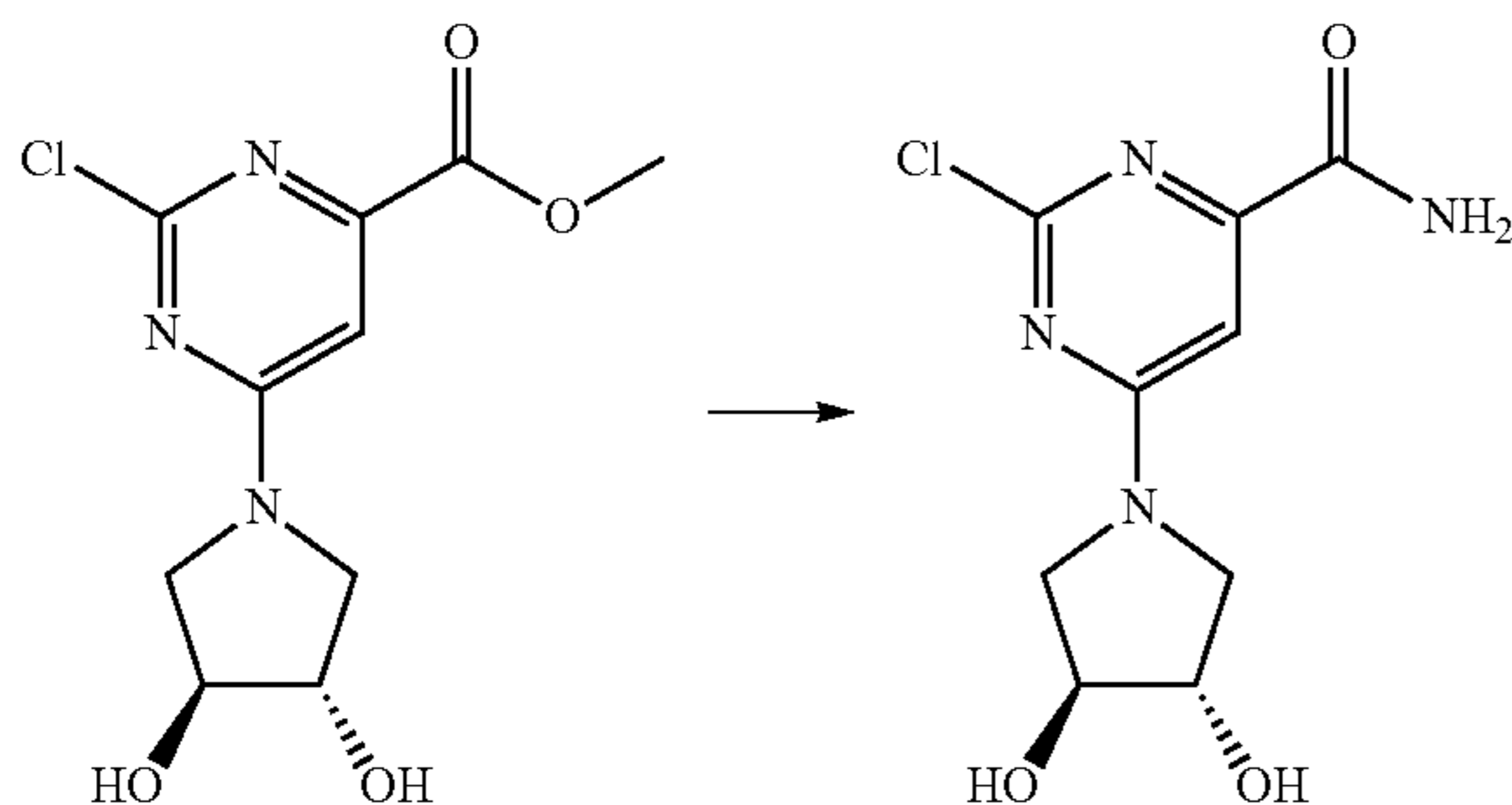
Scheme 59
