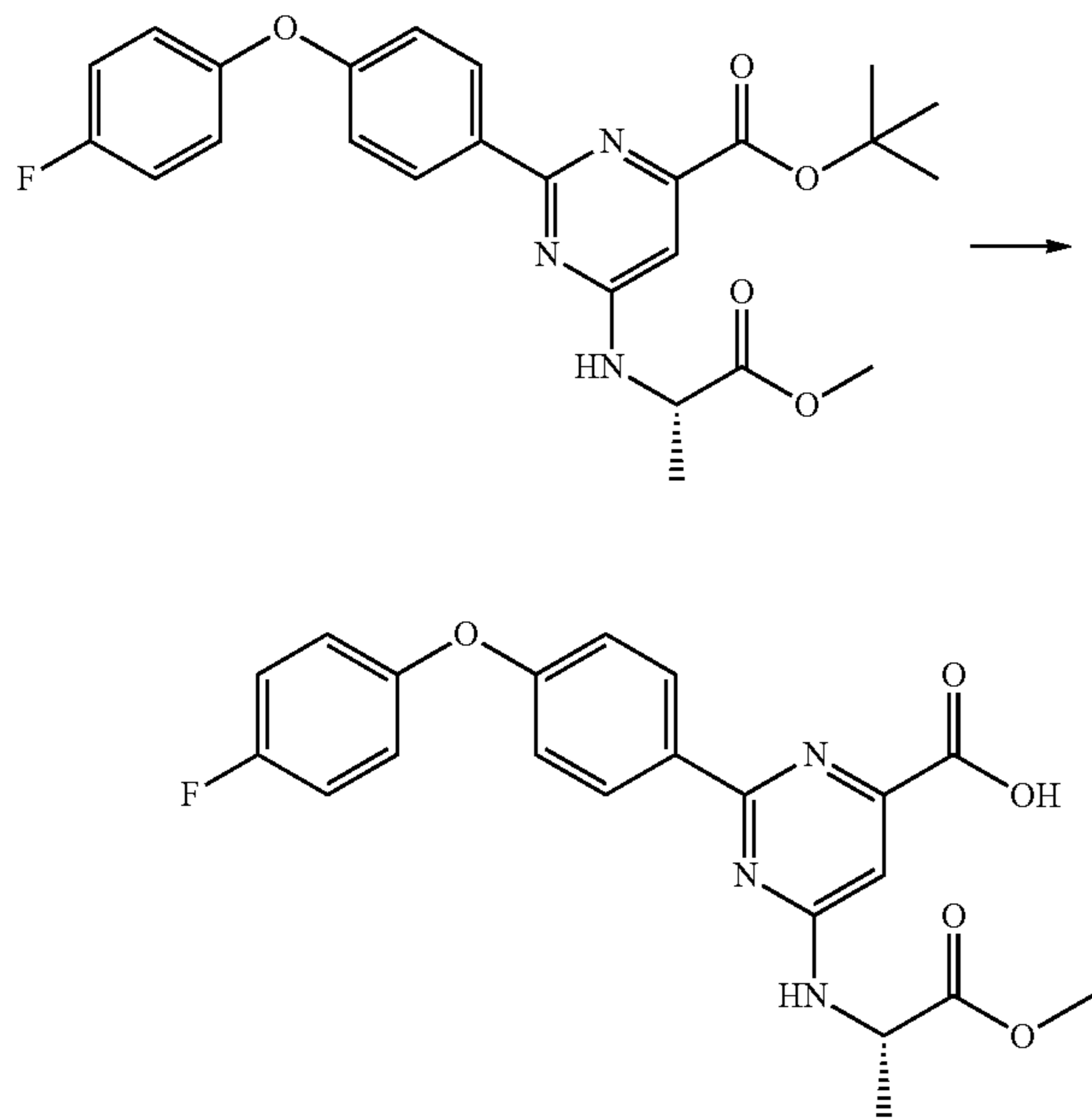
Scheme 13
