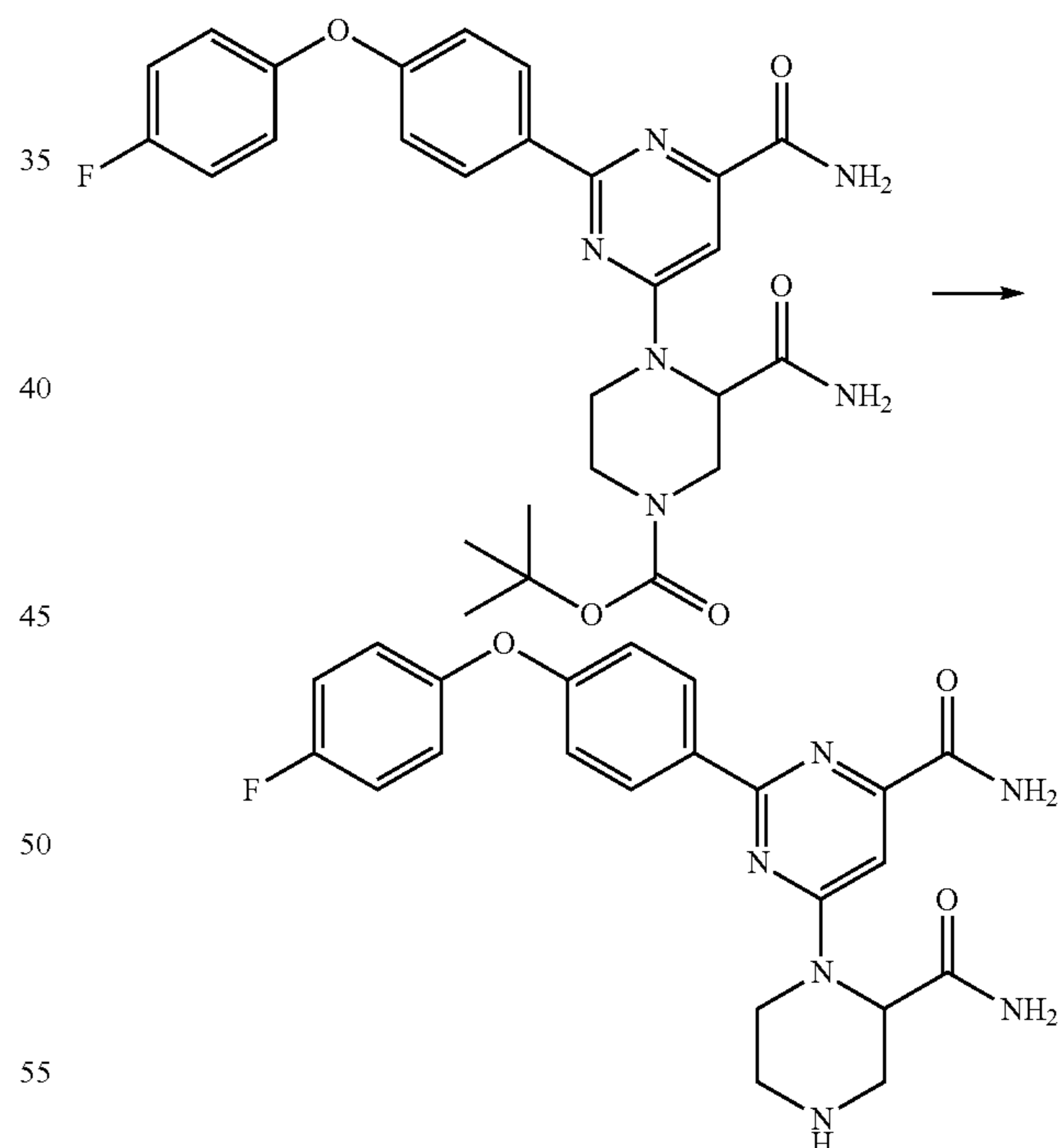
Scheme 7
