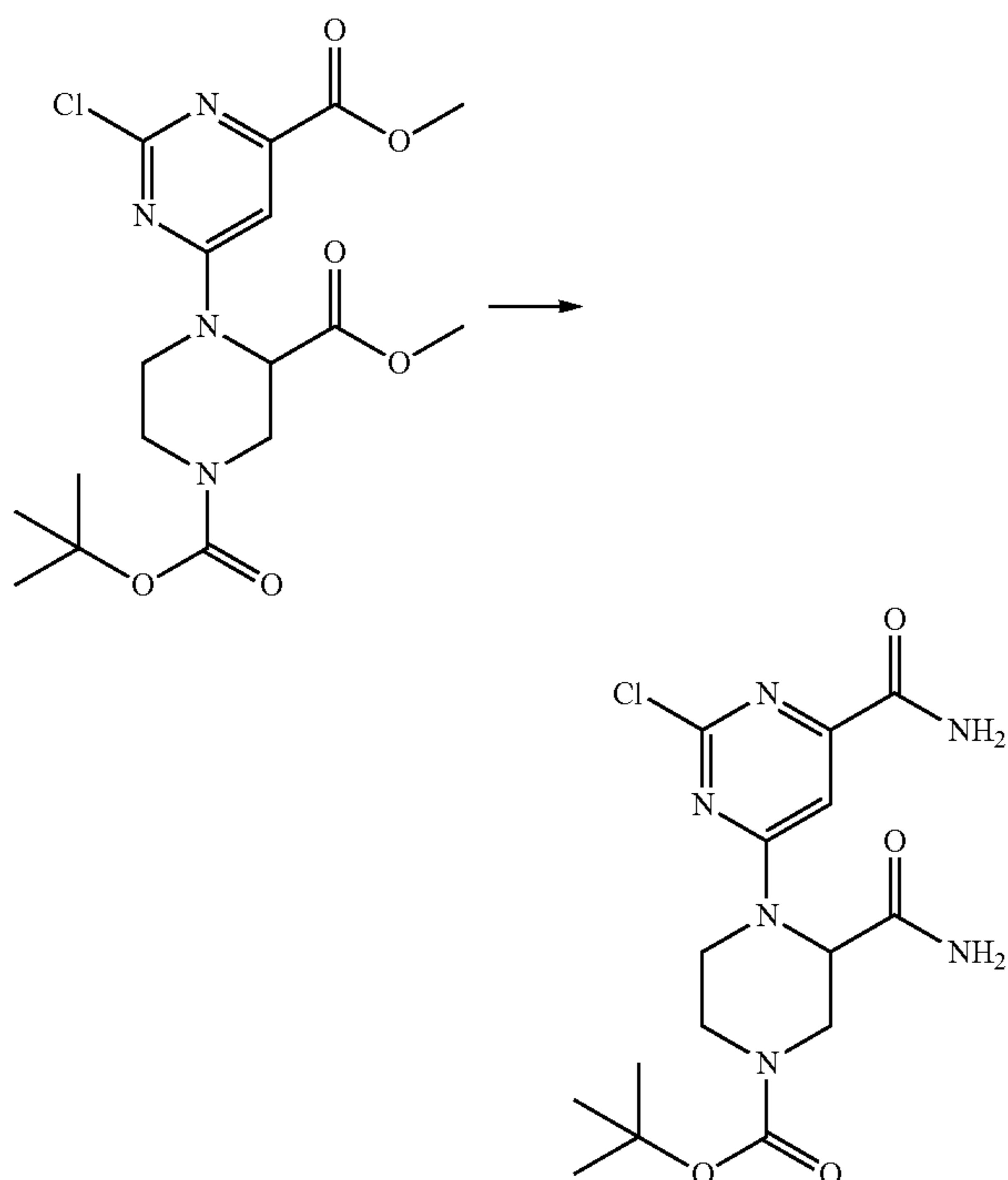
Scheme 62
