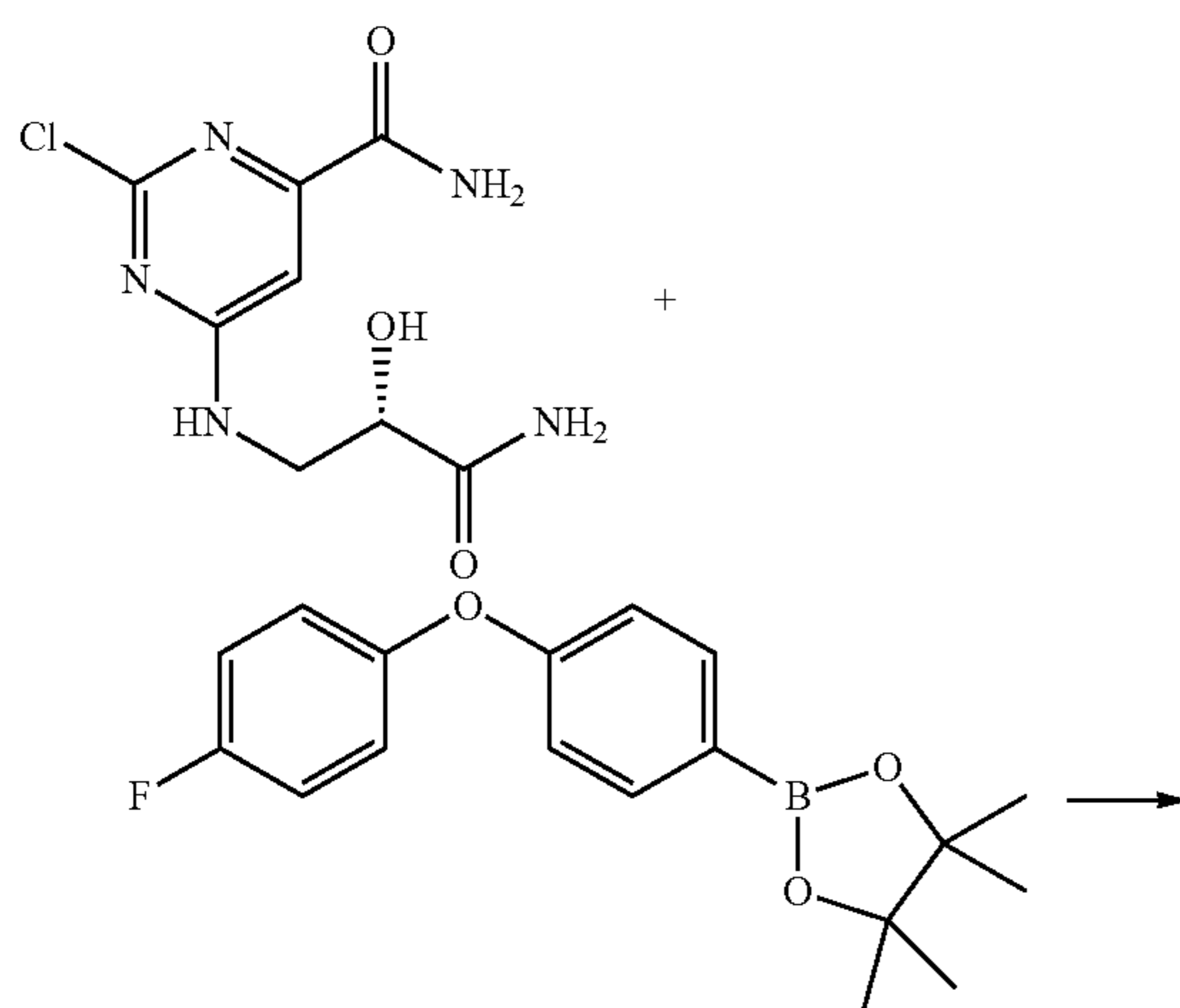
Scheme 30
