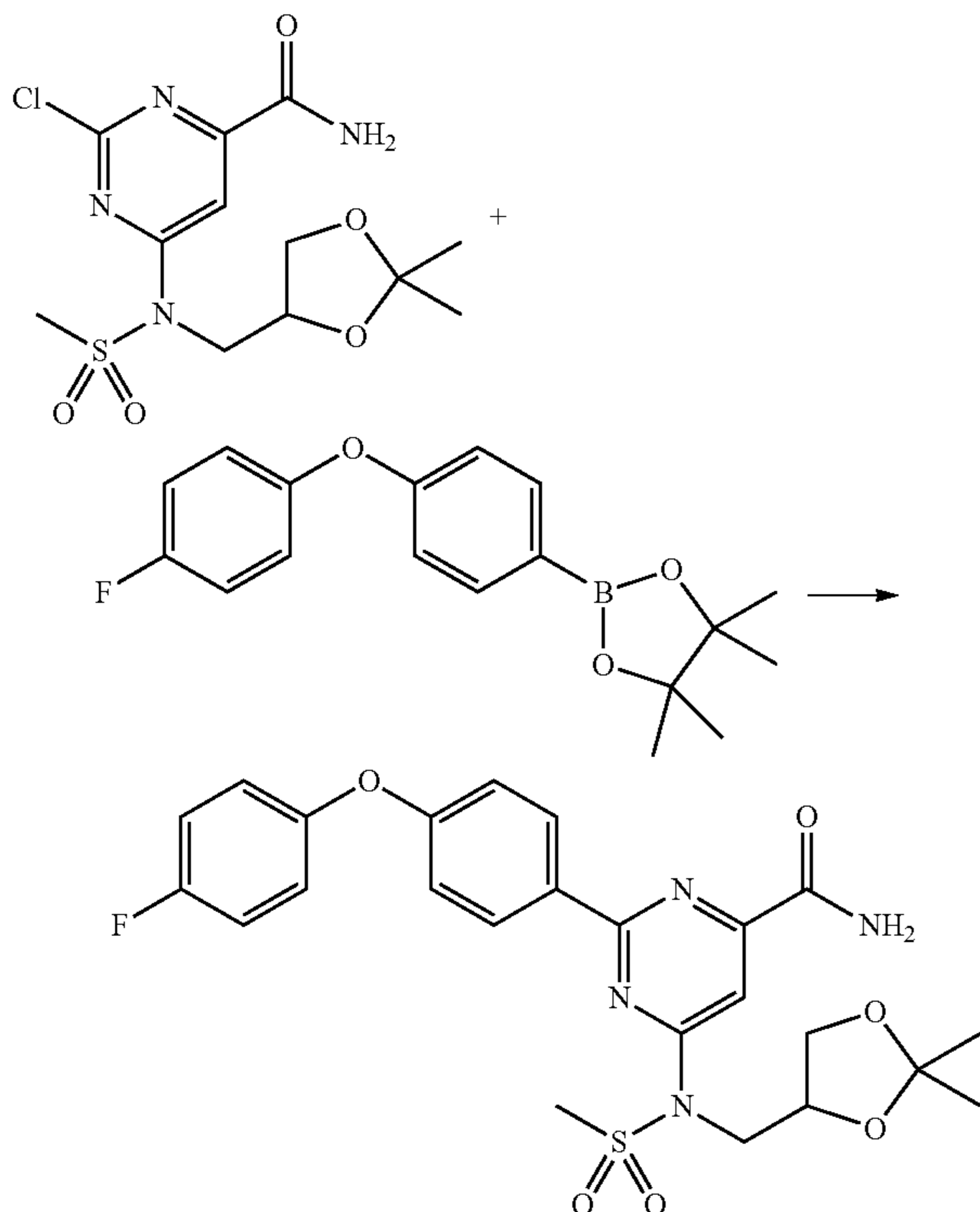
Scheme 35
