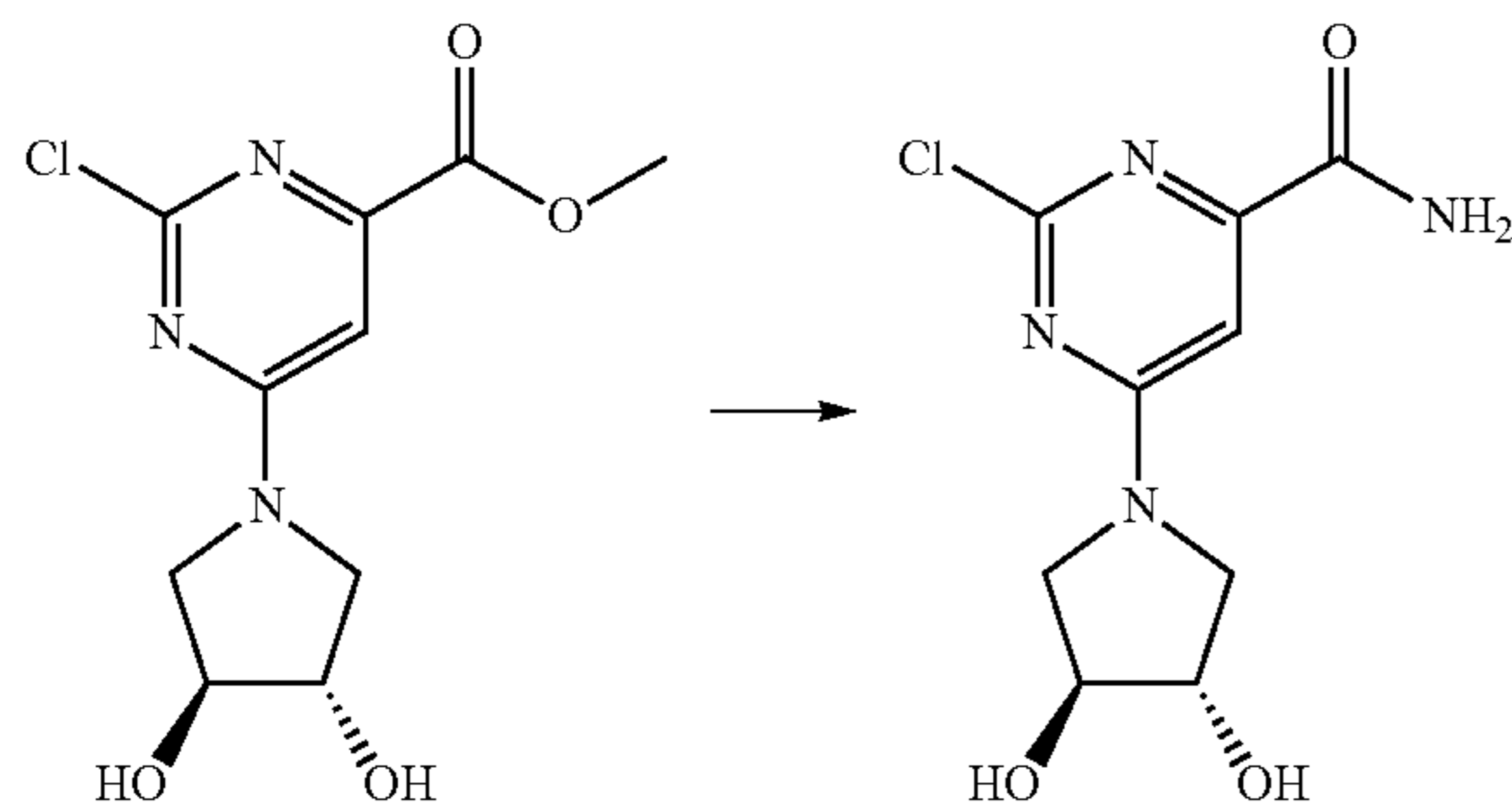
Scheme 59
