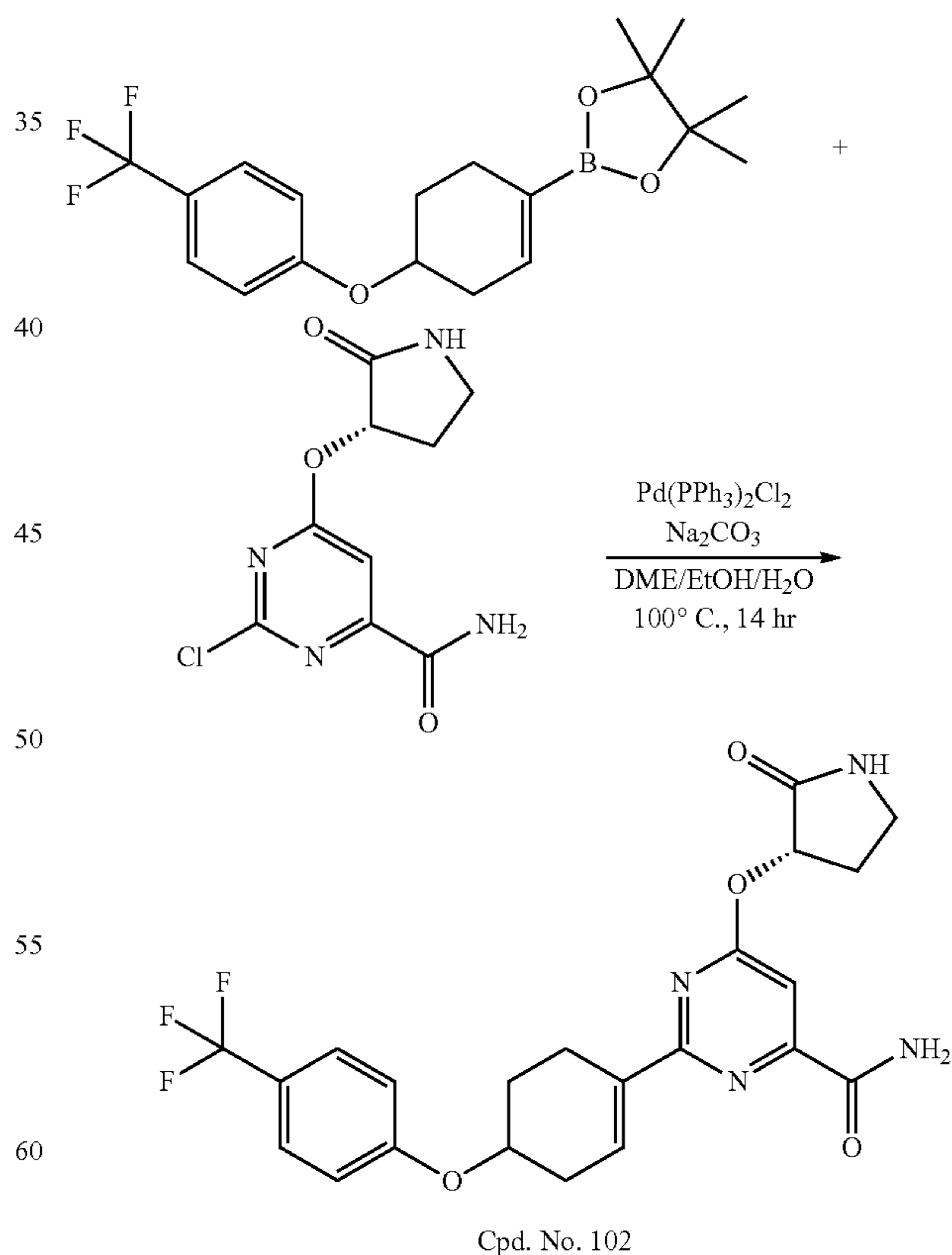
Scheme 82
