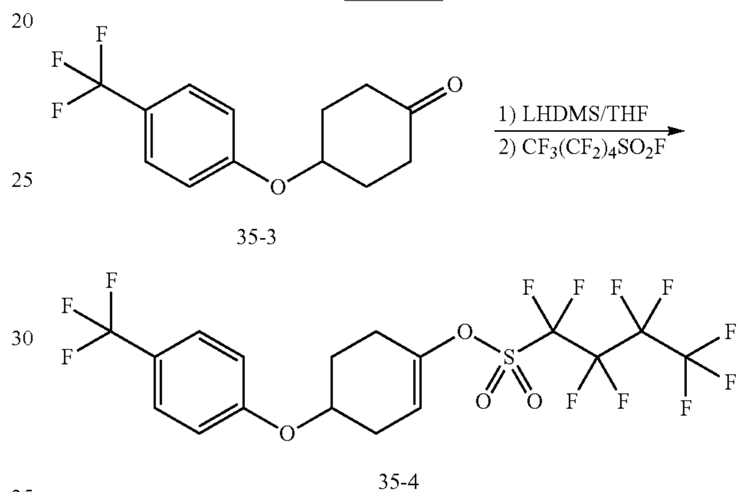
Scheme 79
