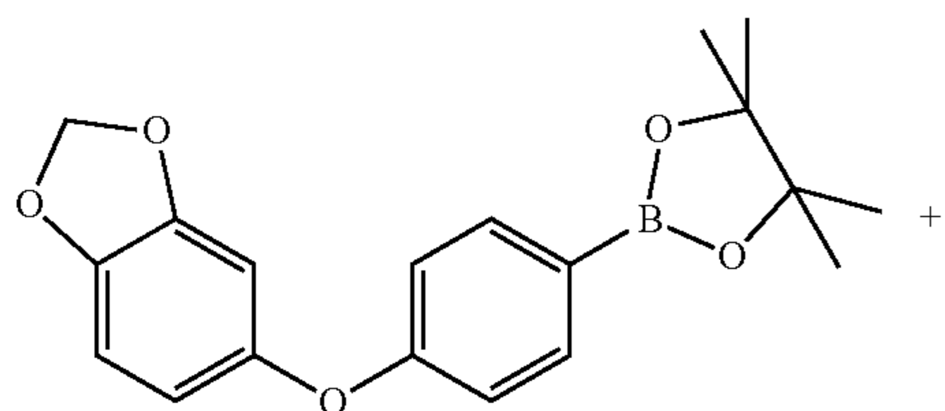
Scheme 72
