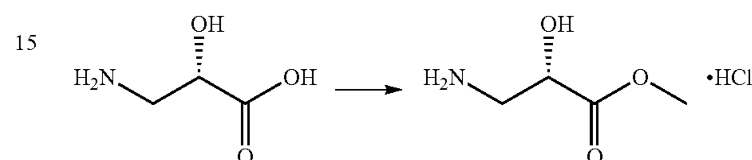
Scheme 27
