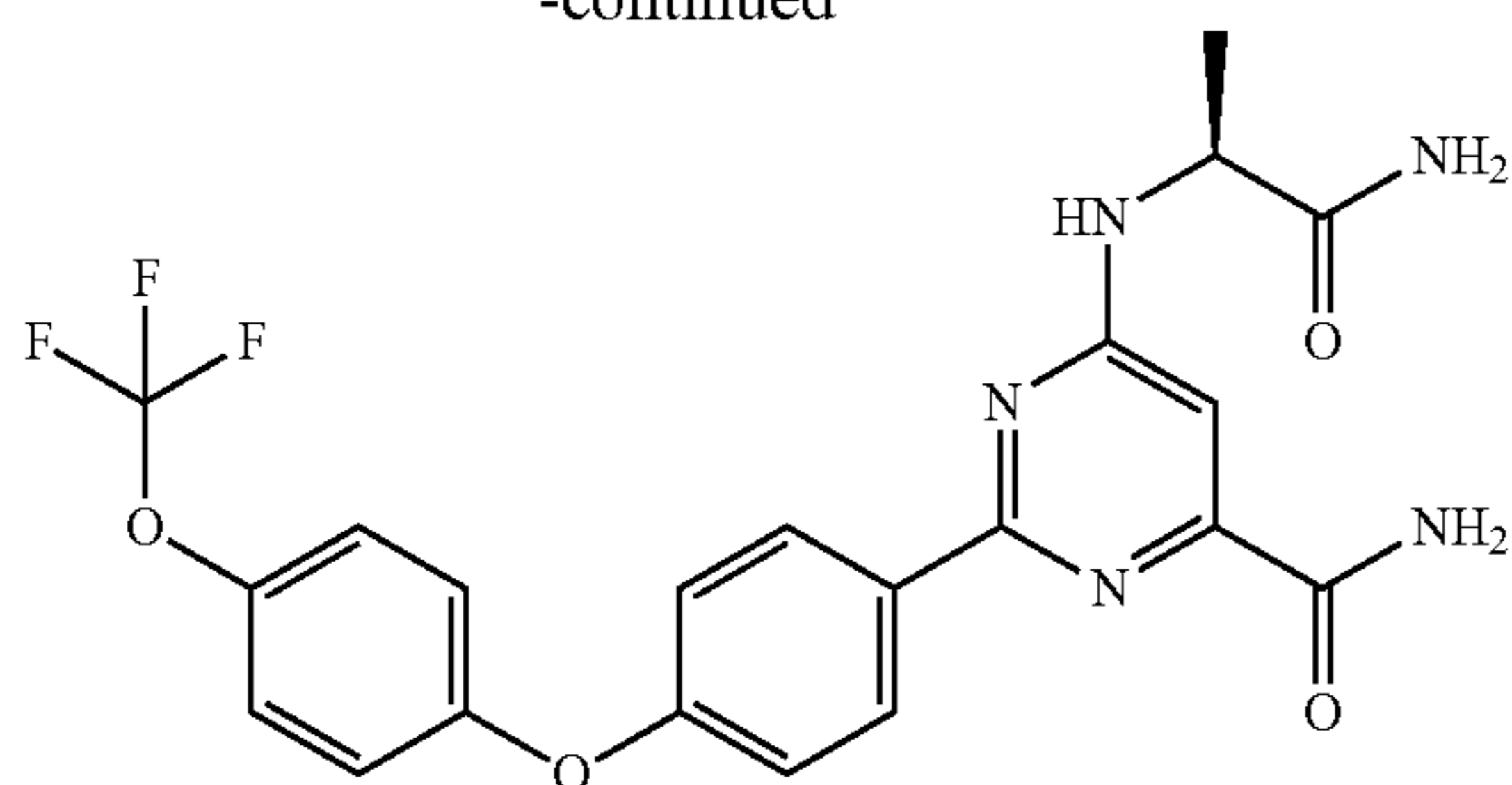
(S)-6-((1-amino-1-oxopropan-2-yl)amino)-2-(4-(4-(trifluoromethoxy)phenoxy)phenyl) pyrimidine-4-carboxamide
