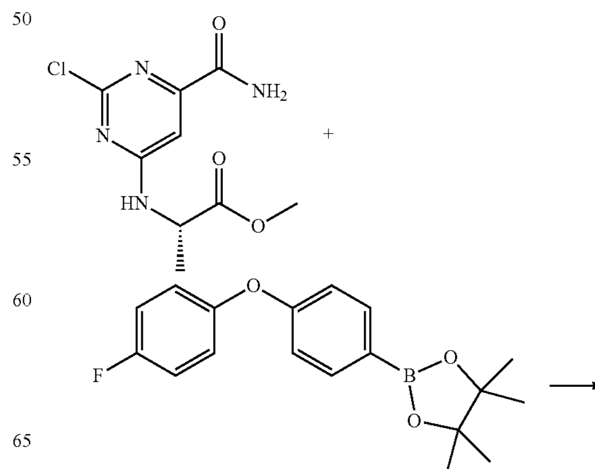
Scheme 5
