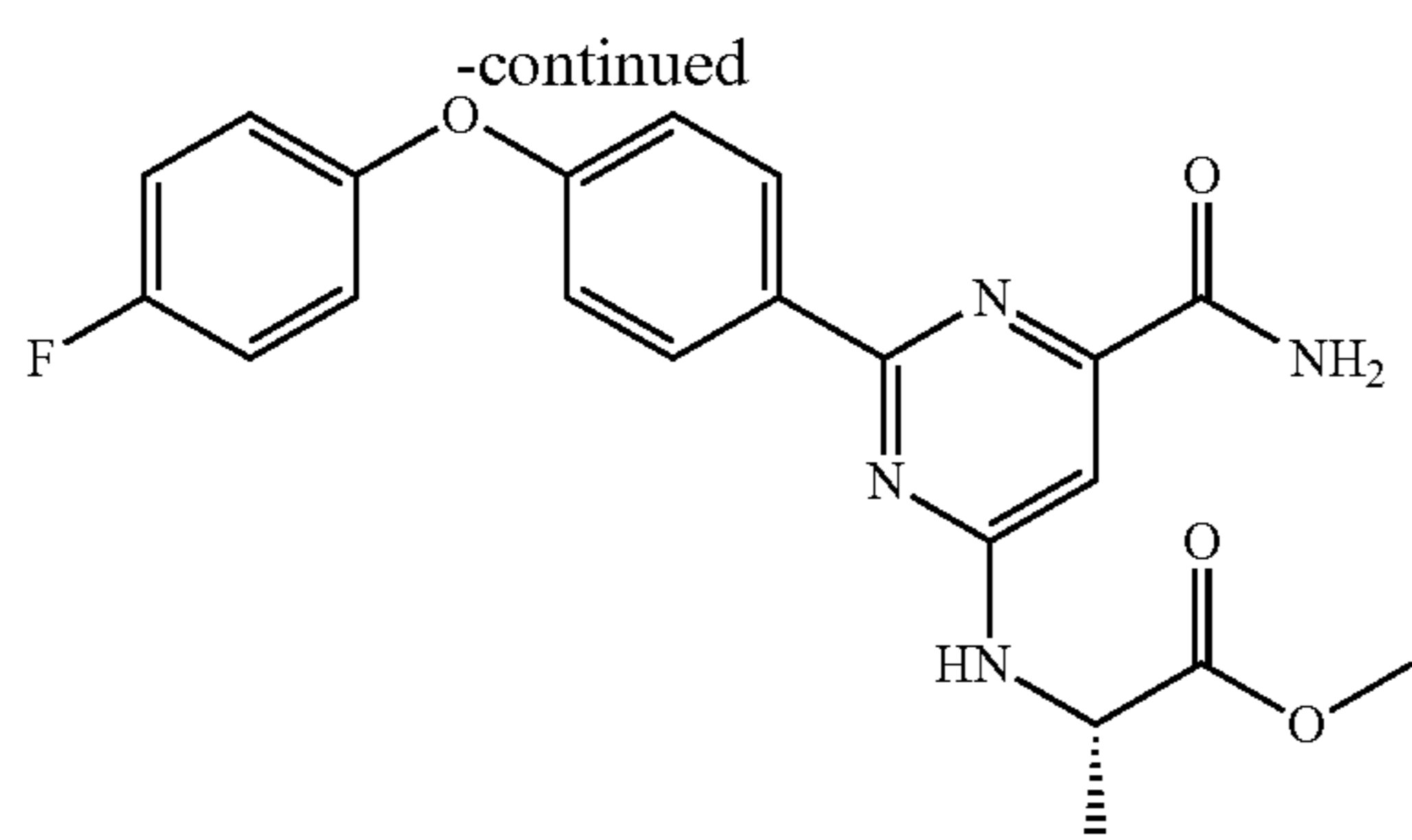
(S)-methyl 2-((6-carbamoyl-2-(4-(4-fluorophenoxy)phenyl)pyrimidin-4-yl)amino)propanoate
