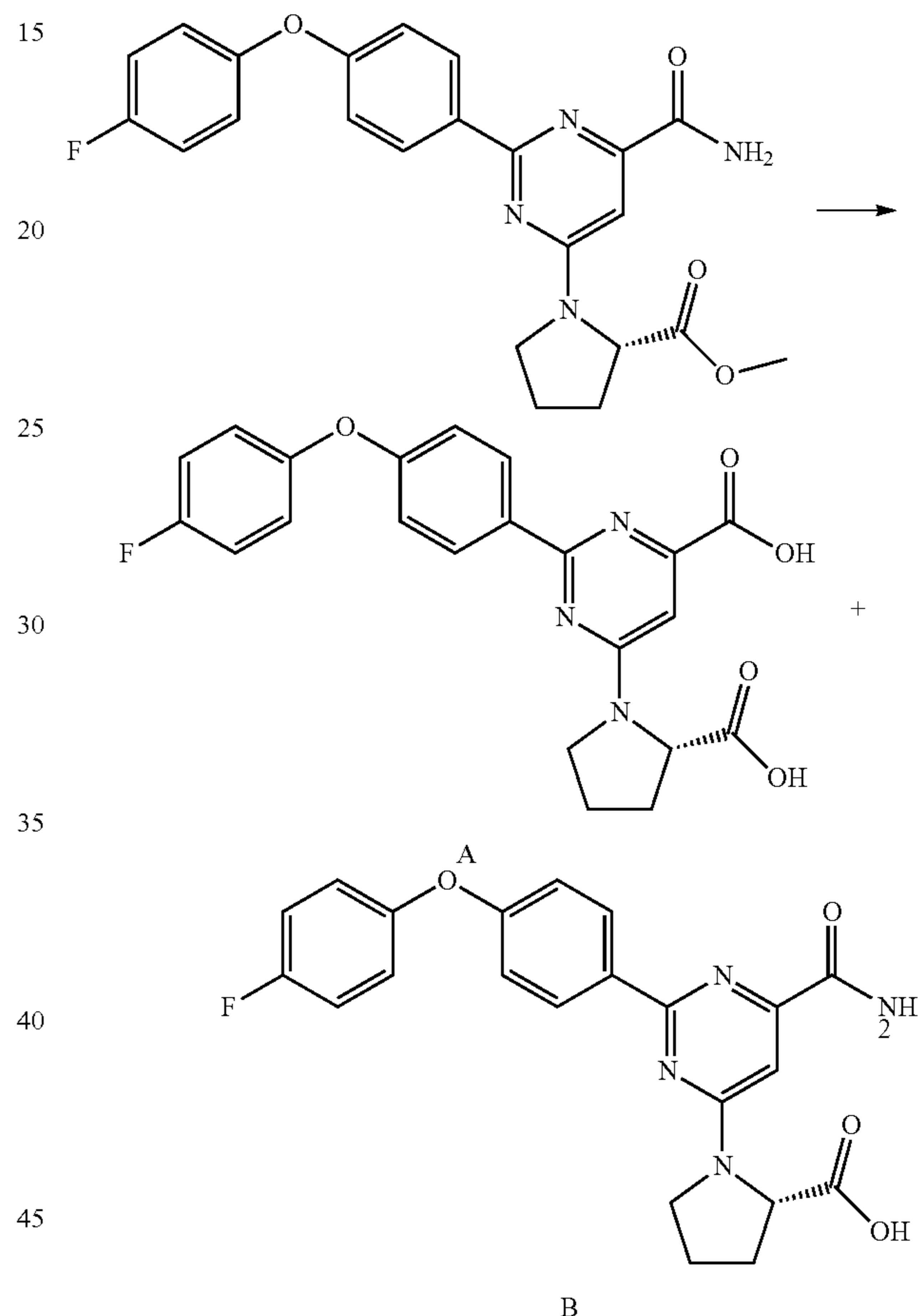
Scheme 9
