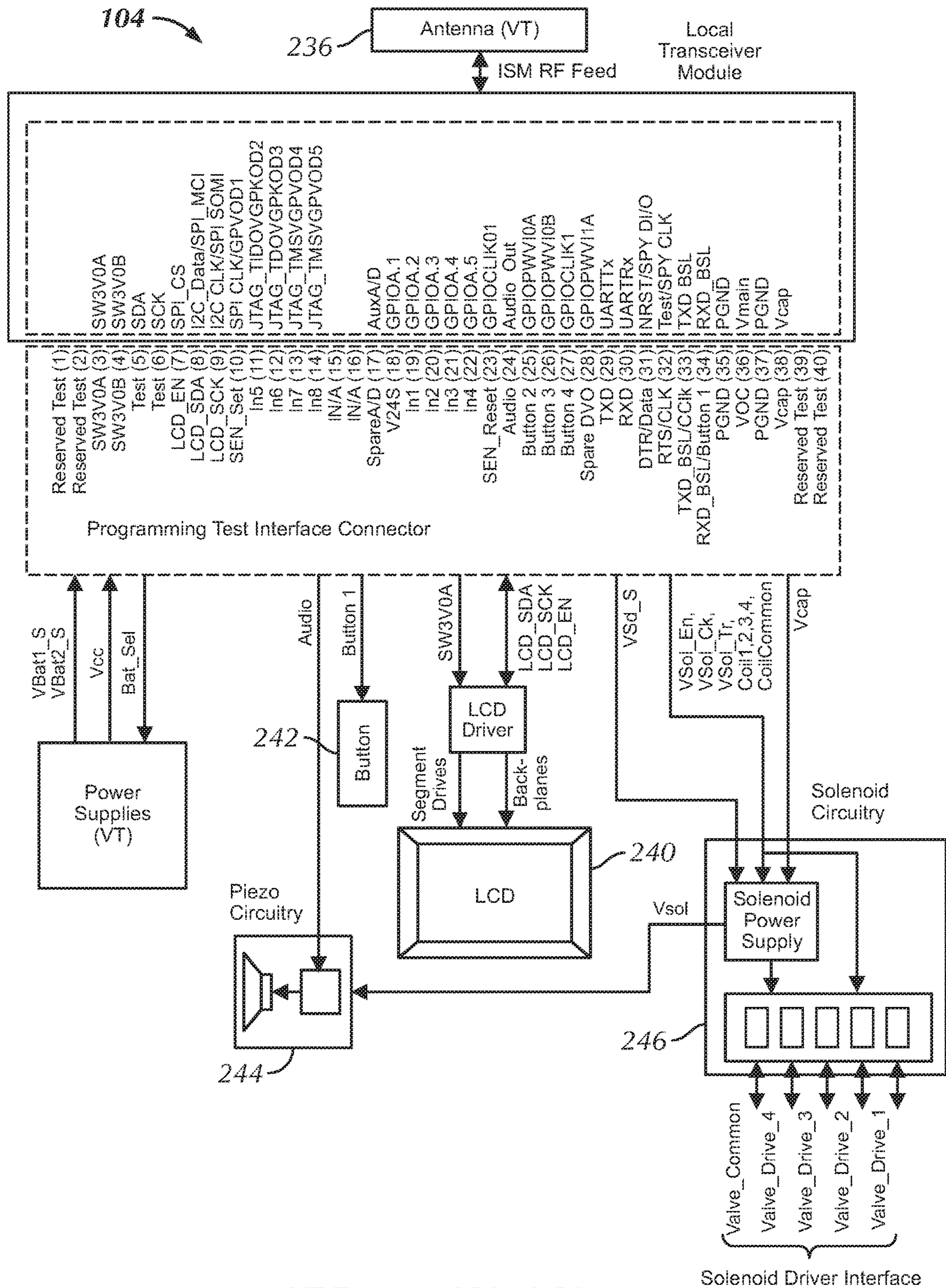
VT Top Level Block Diagram
