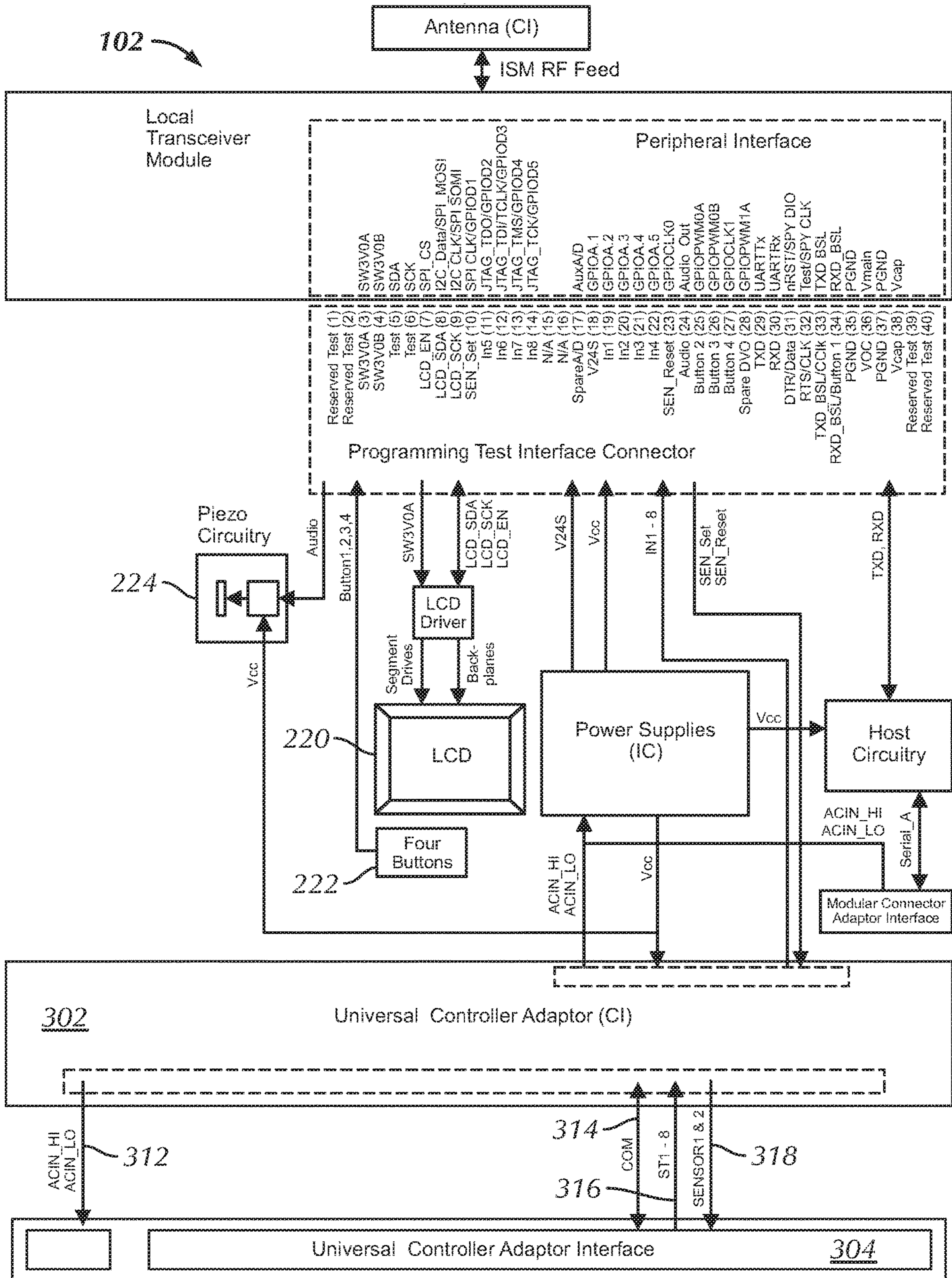
CI Top Level Block Diagram
