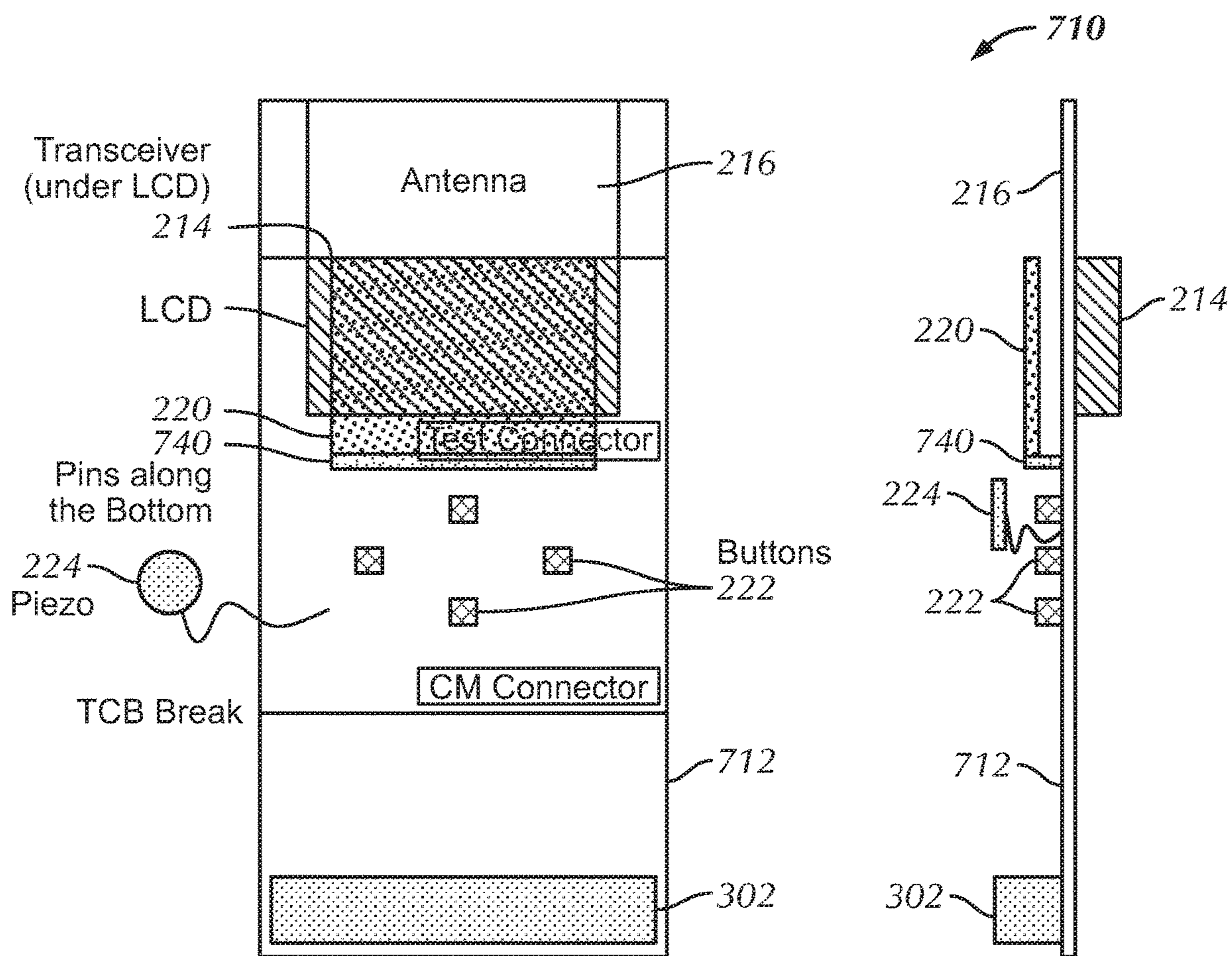
CI board
