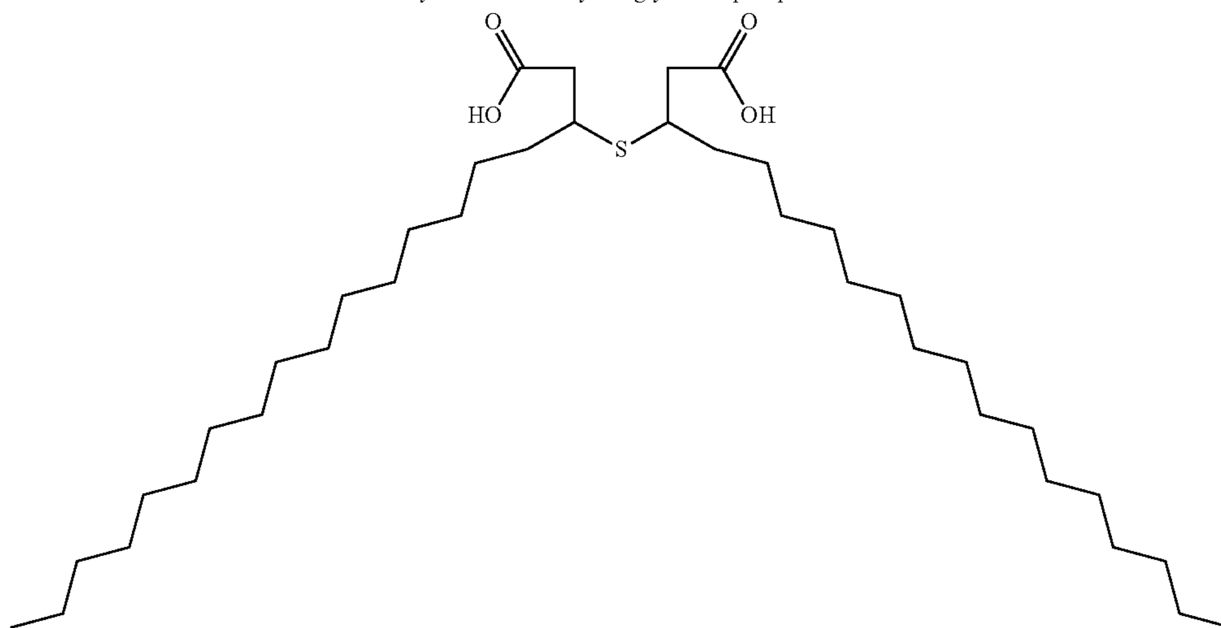
3,3'-Thiodinonadecanoic acid
