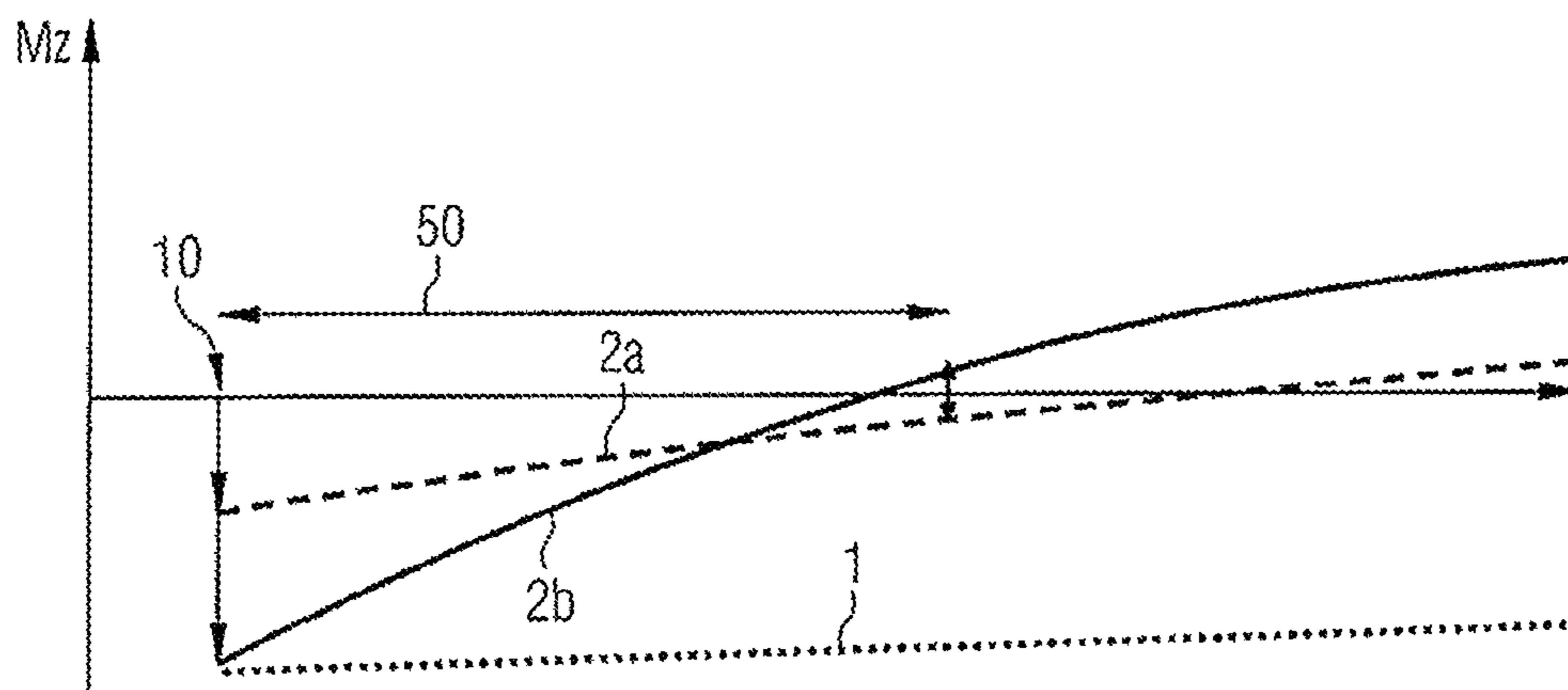
FIG 5 Prior art
