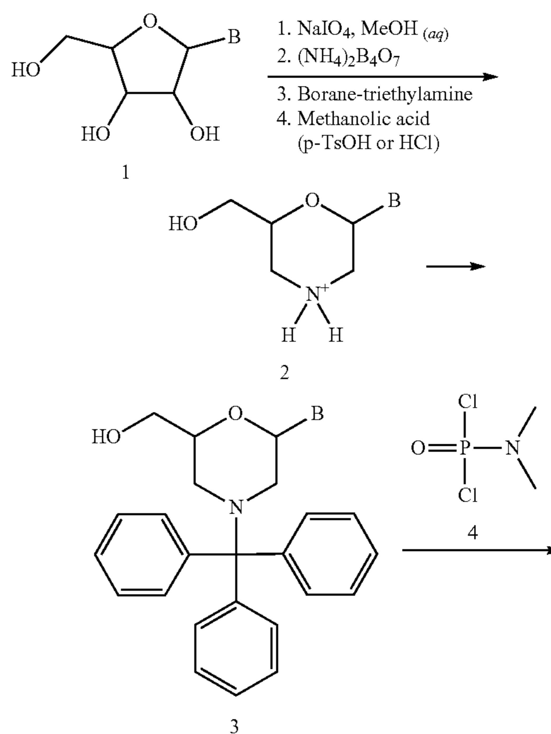
Scheme 1: General synthetic route to PMO Subunits
