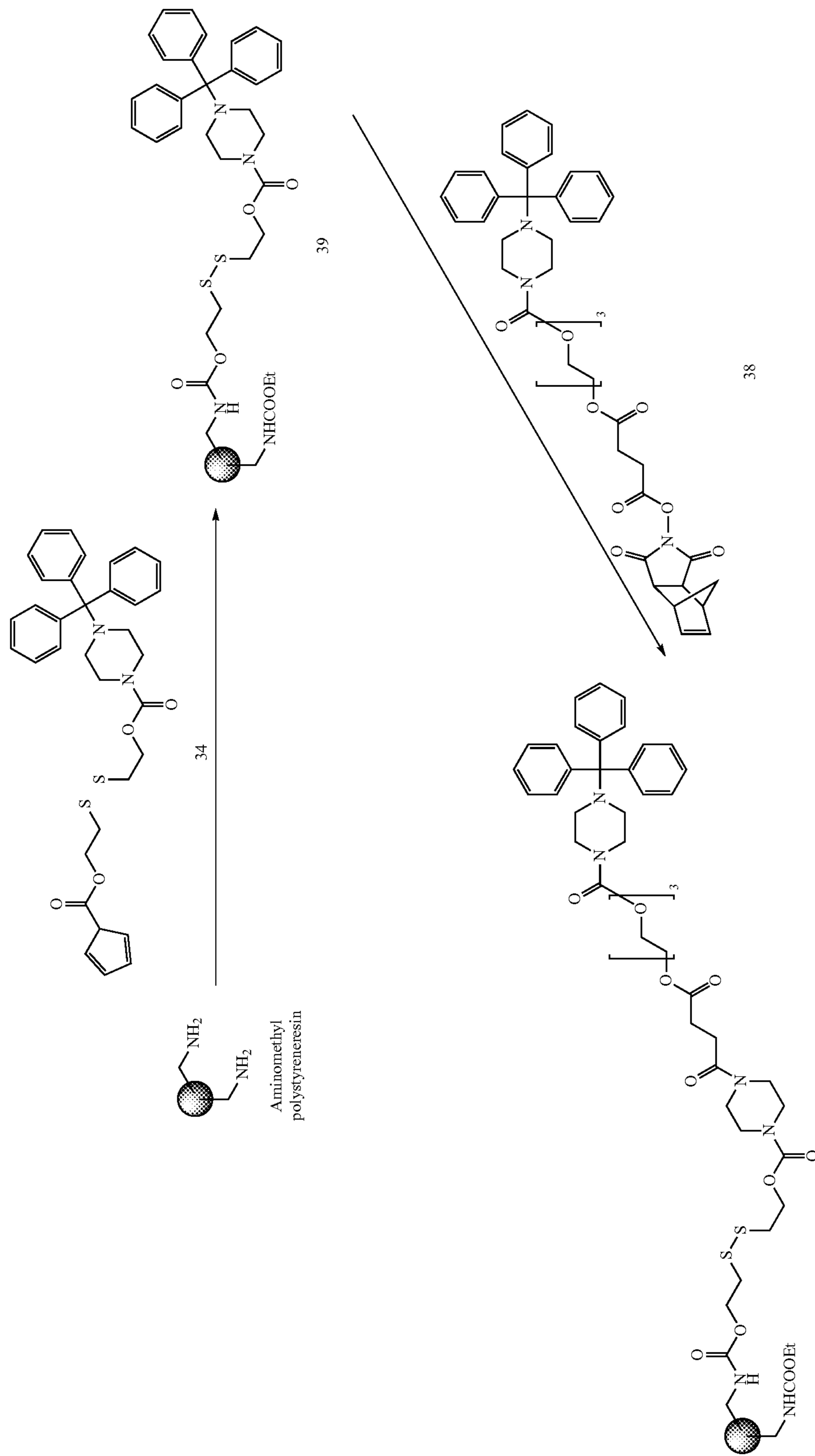
Scheme 3: Preparation of the Solid Support for Synthesis of Morpholino Oligomers
