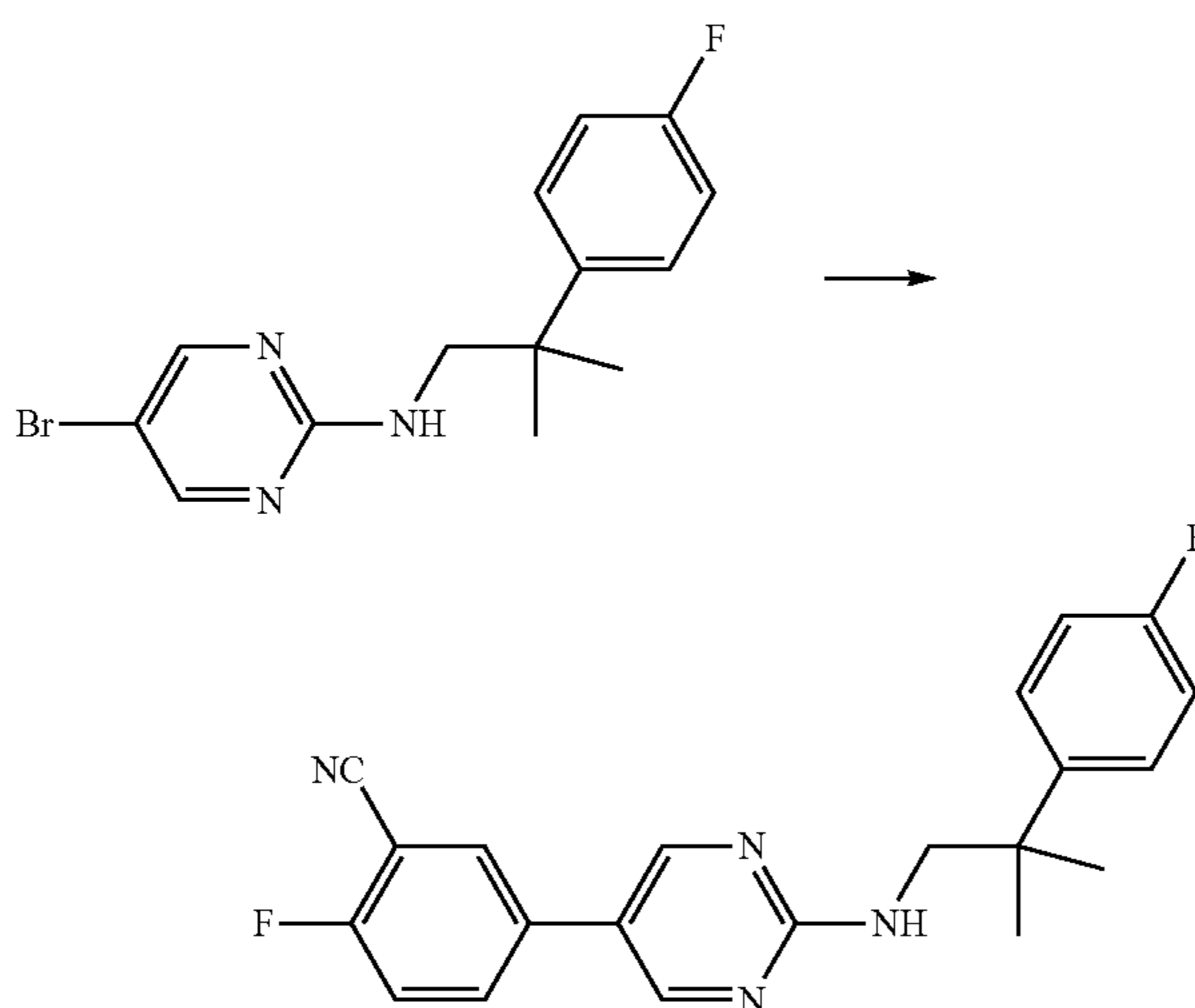
2-Fluoro-5-(2-(2-(4-fluorophenyl)-2-methylpropylamino)pyrimidin-5-yl)benzonitrile
