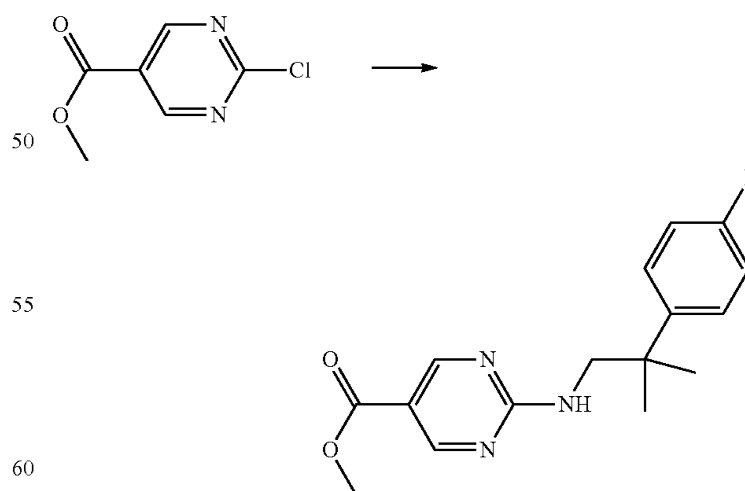
2-Fluoro-5-(2-(2-(4-fluorophenyl)-2-methylpropylamino)pyrimidin-5-yl)benzonitrile
