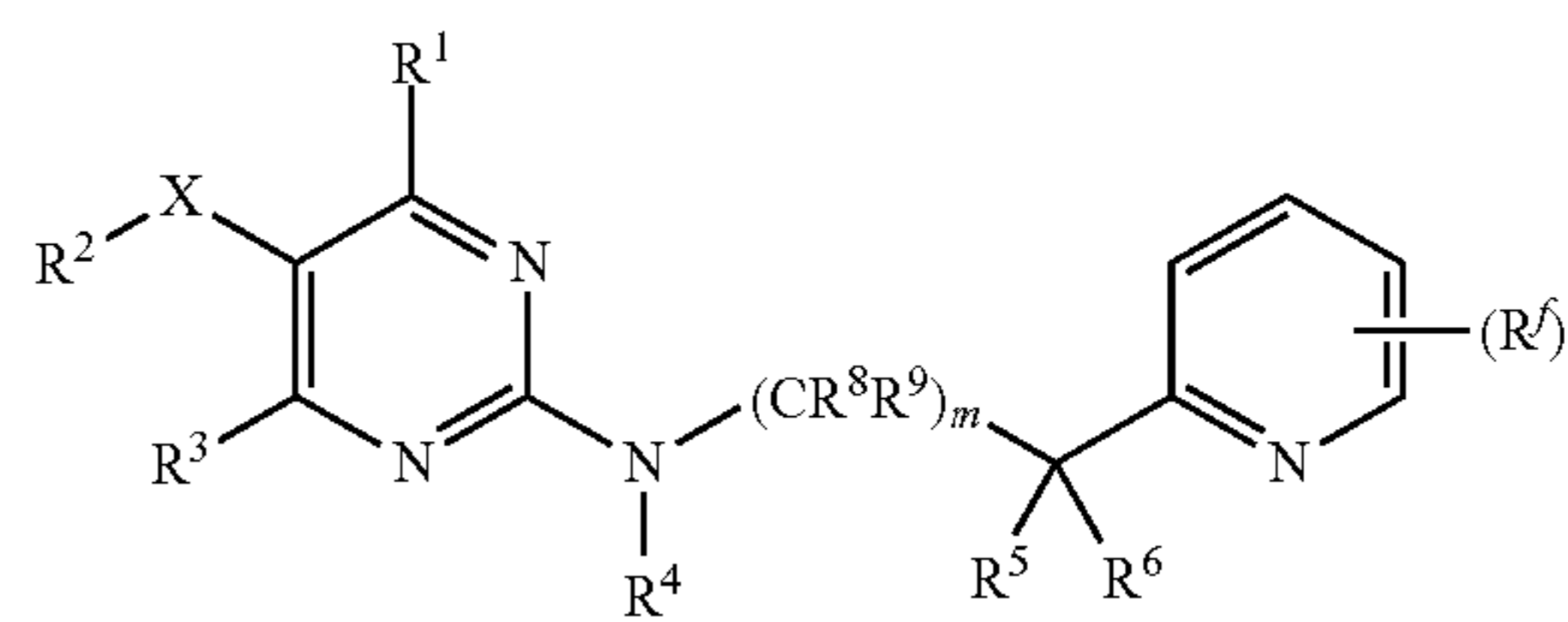
Formula IX
