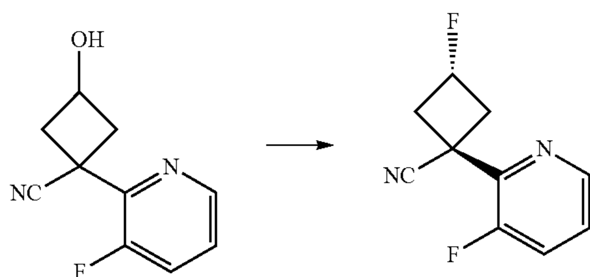
trans-3-Fluoro-1-(3-fluoropyridin-2-yl)cyclobutanecarbonitrile
