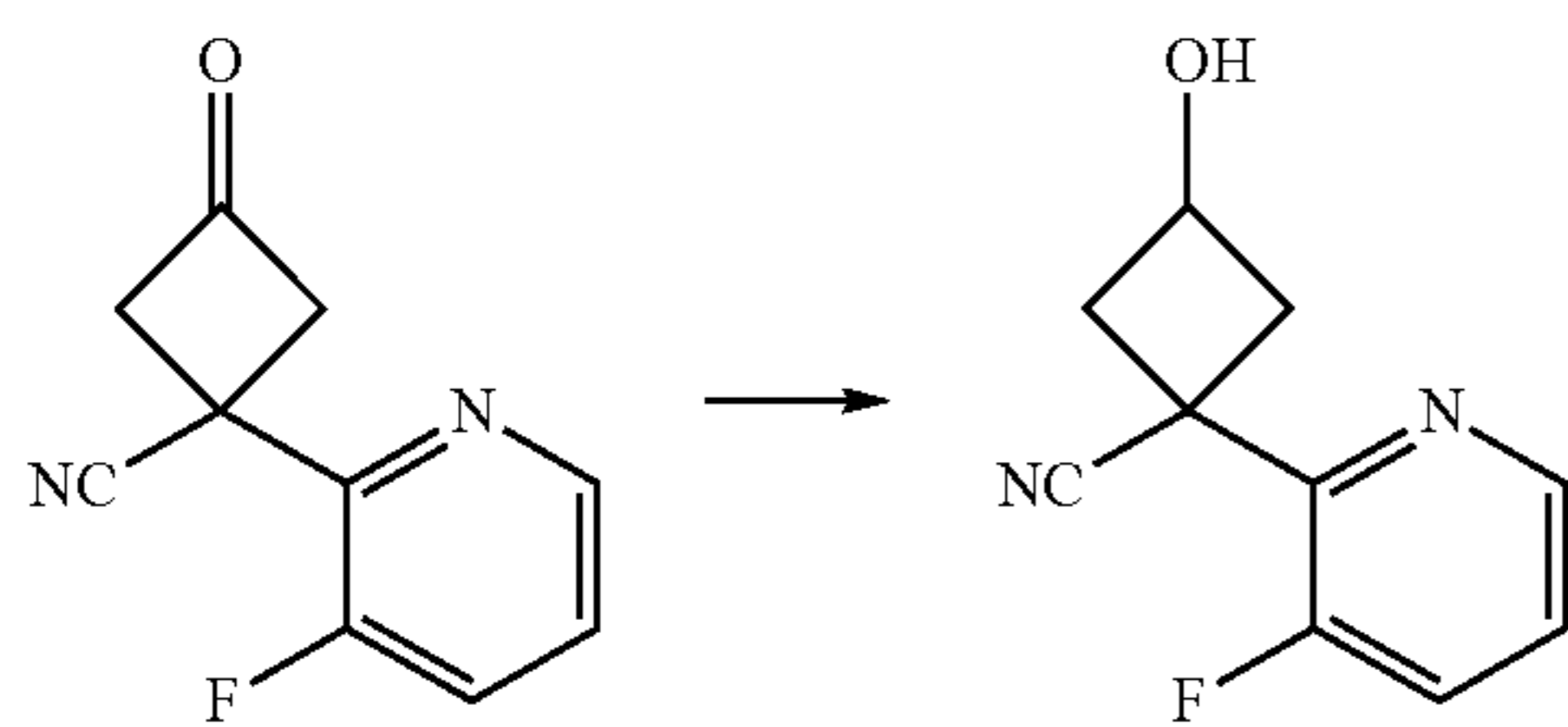
1-(3-Fluoropyridin-2-yl)-3-hydroxycyclobutanecarbonitrile
