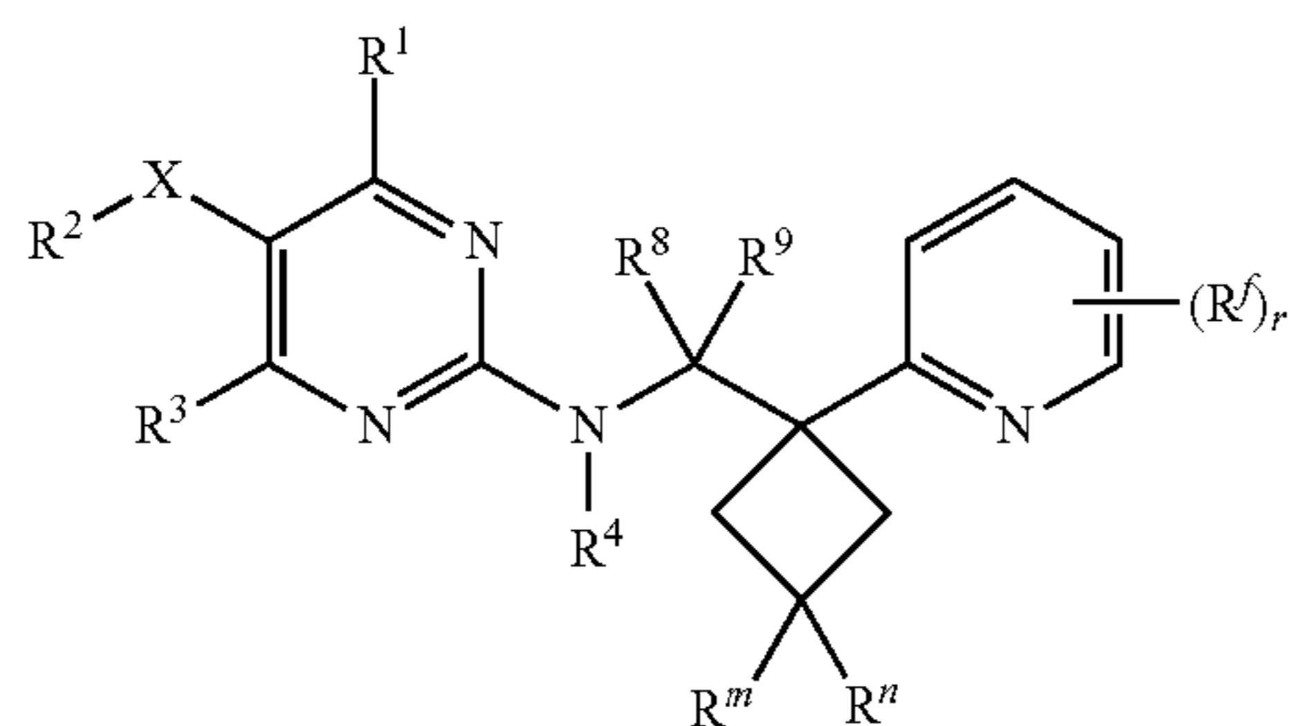
Formula XI(b)
