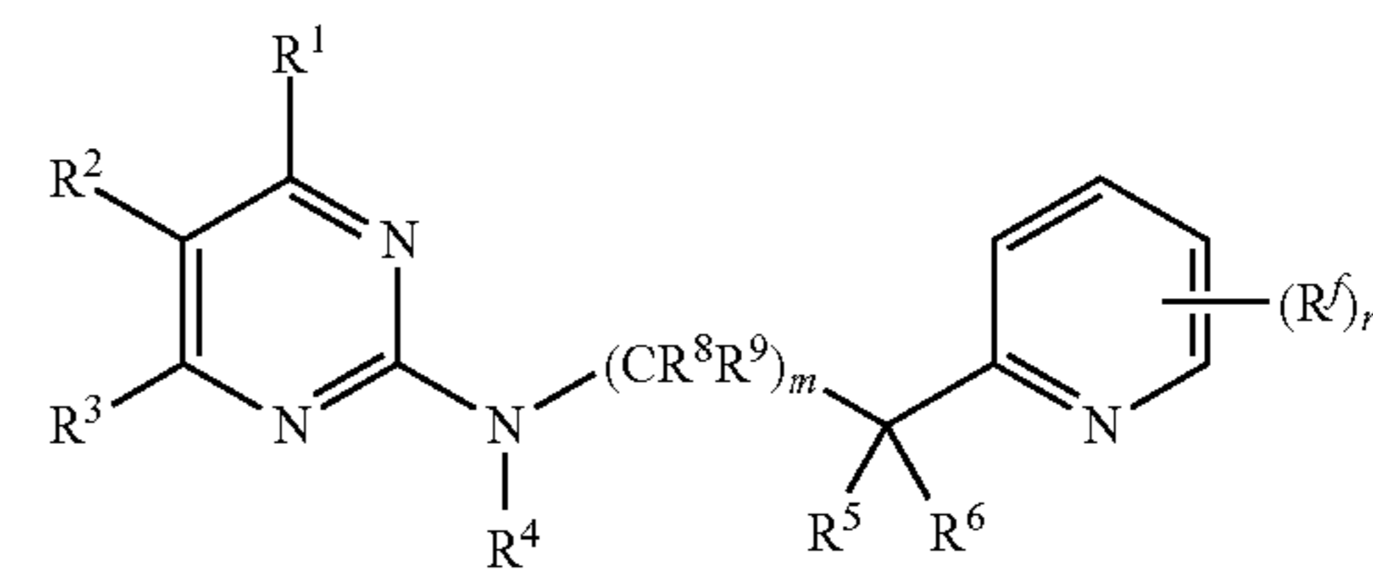
Formula XII(l)
