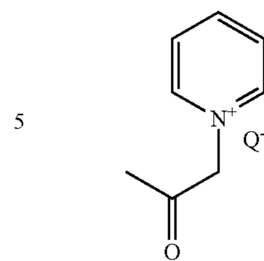
Salt of 1-(2-Oxo-propyl)pyridinium
