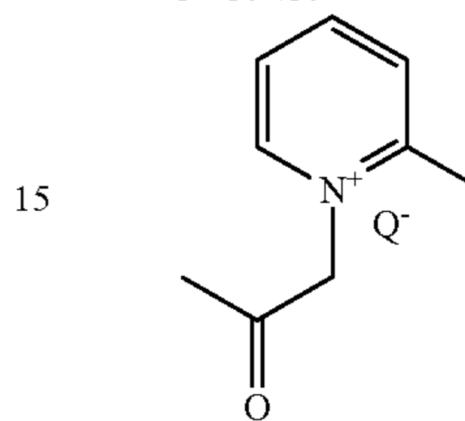
Salt of 2-Methyl-1-(2-Oxo-propyl)-pyridinium
