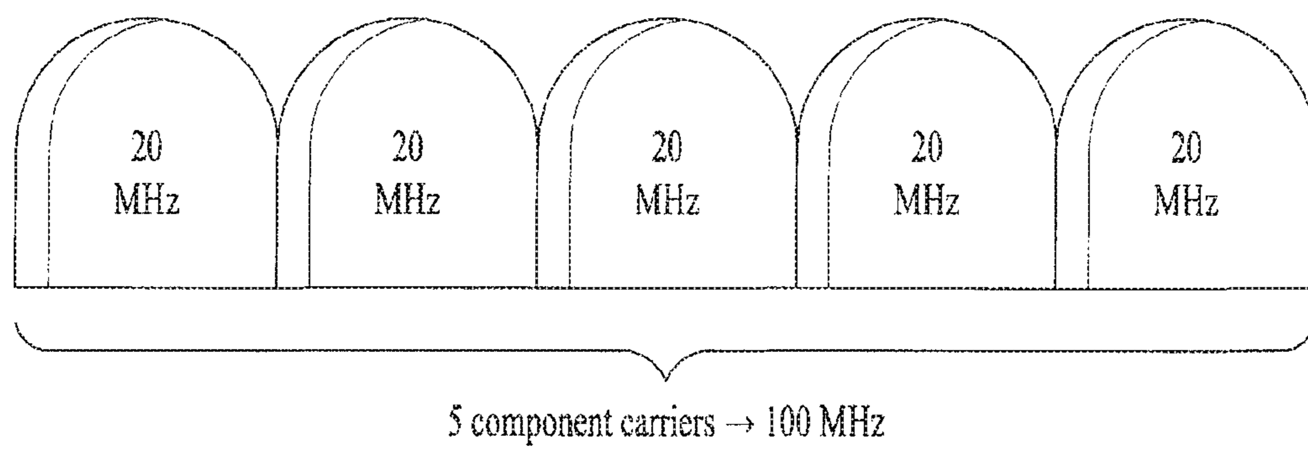
Component carrier
